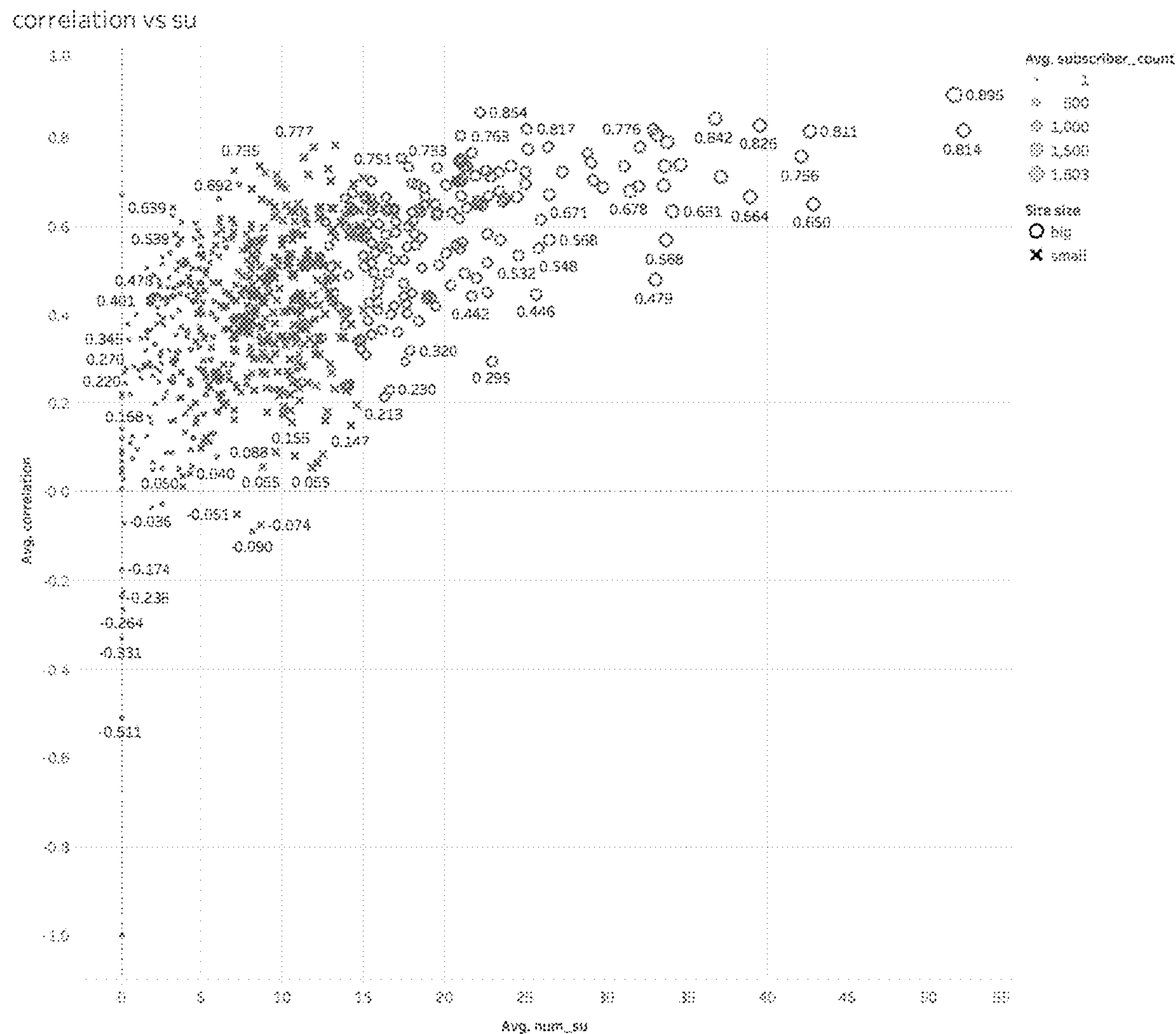
Average of num_su vs. average of correlation. Size shows average of subscriber_count. Shape shows details about Site size. The marks are labeled by average of correlation. Details are shown for site. The data is filtered on time_stamp, which ranges from 21/8/2019 00:00:00 to 27/9/2019 00:00:00. The view is filtered on site, which excludes 0 and 65881.
