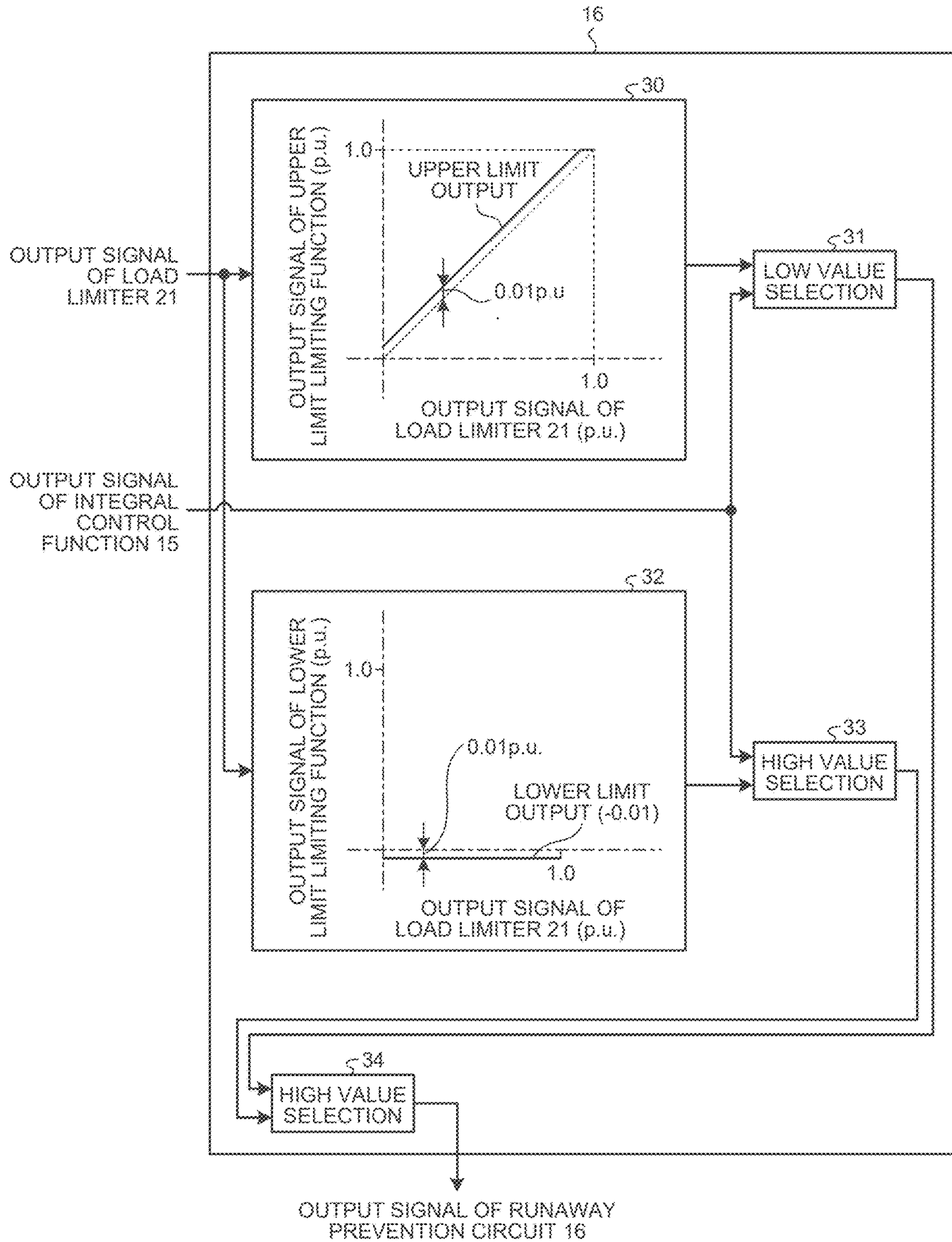
FIG.8 (PRIOR ART)
