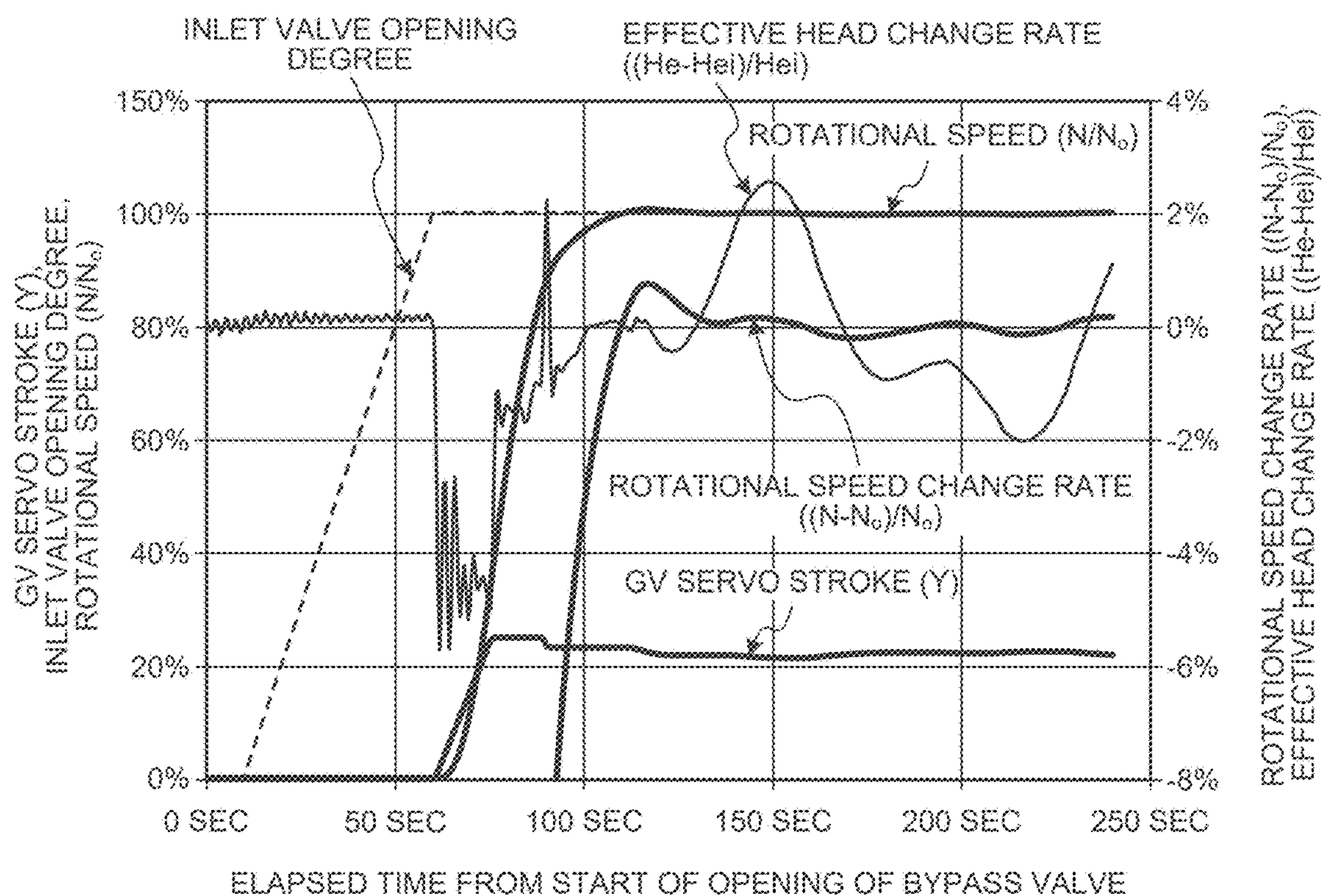
FIG.12 (PRIOR ART)
