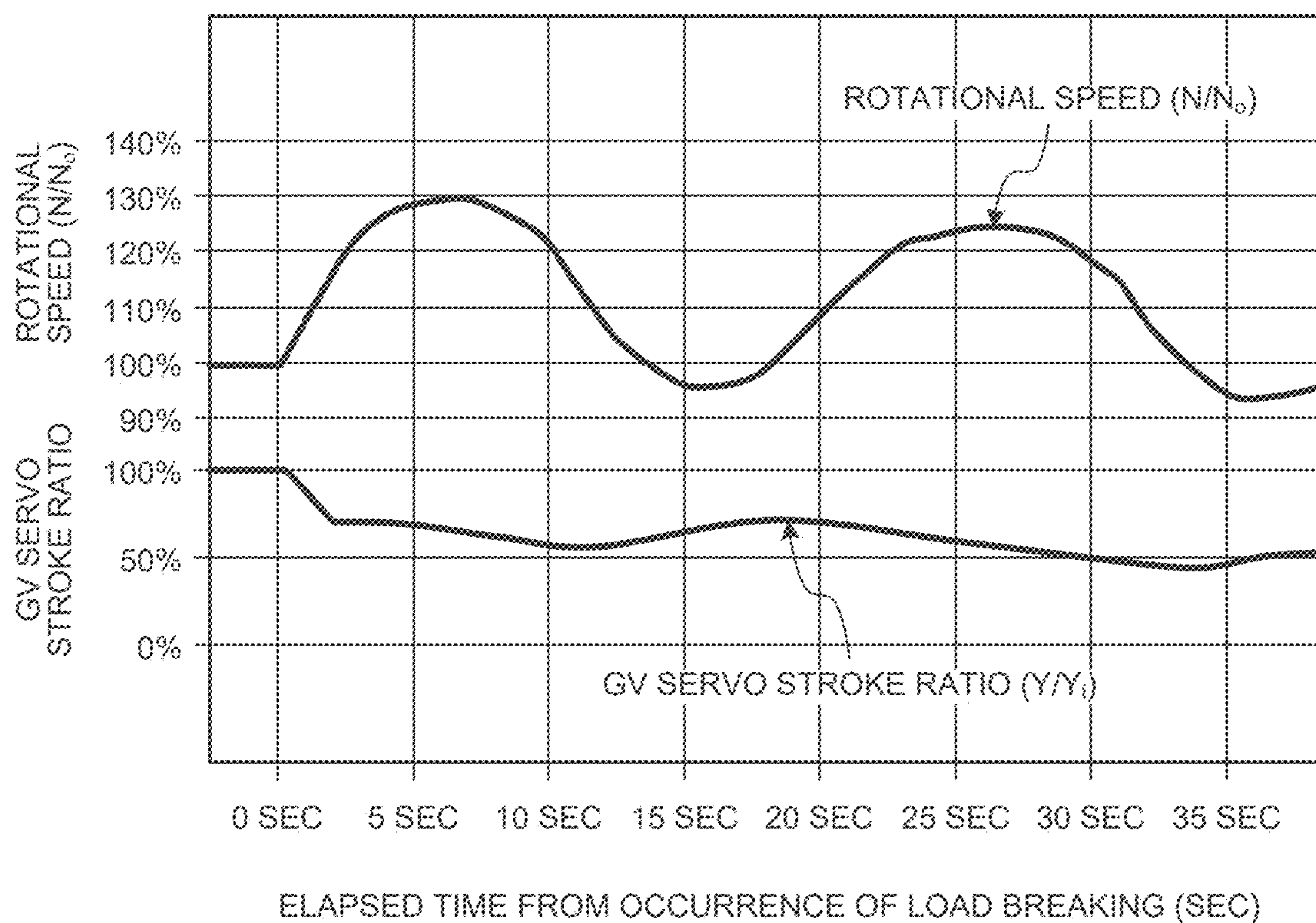
FIG.10 (PRIOR ART)
