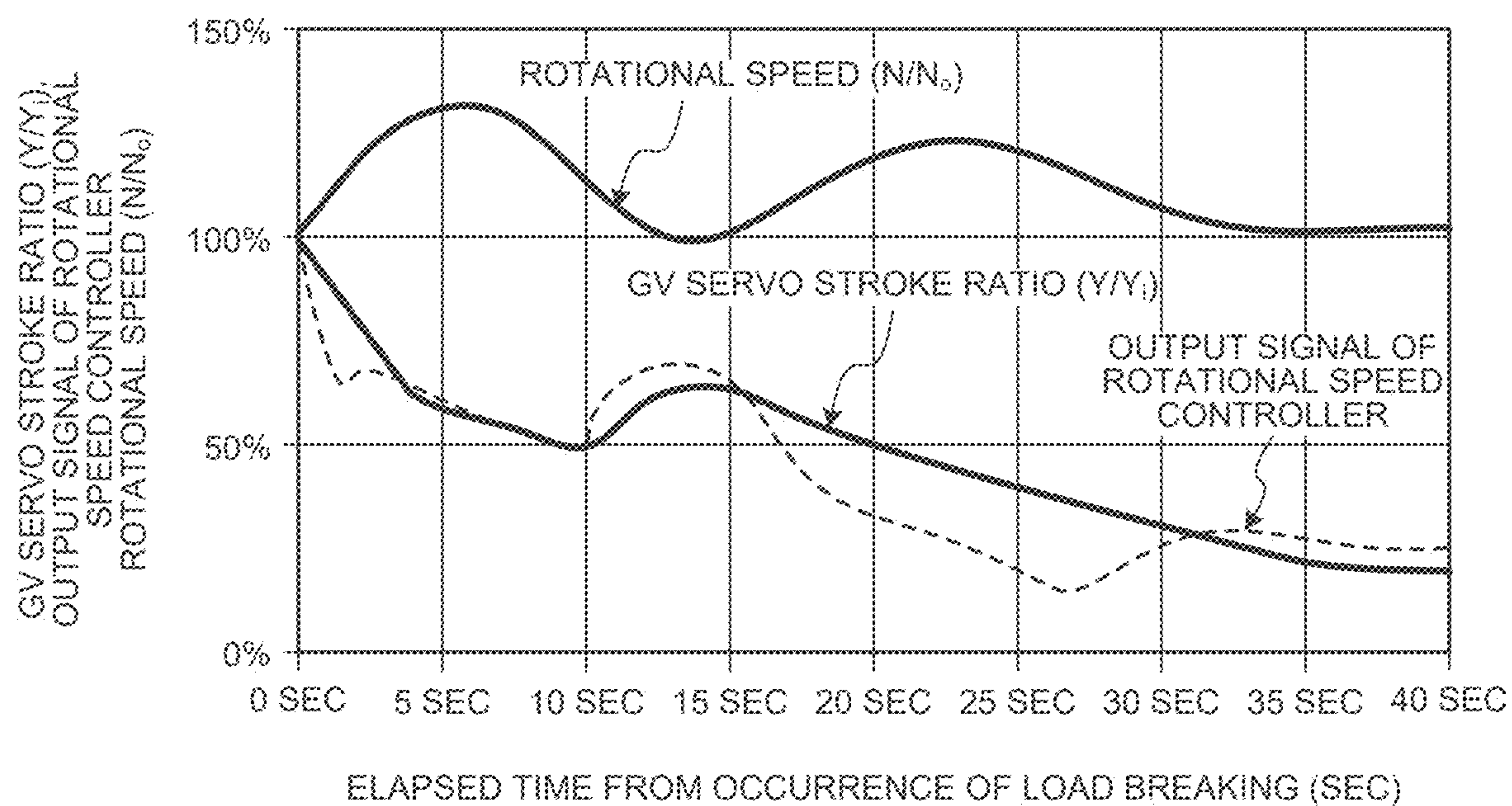
FIG.11 (PRIOR ART)
