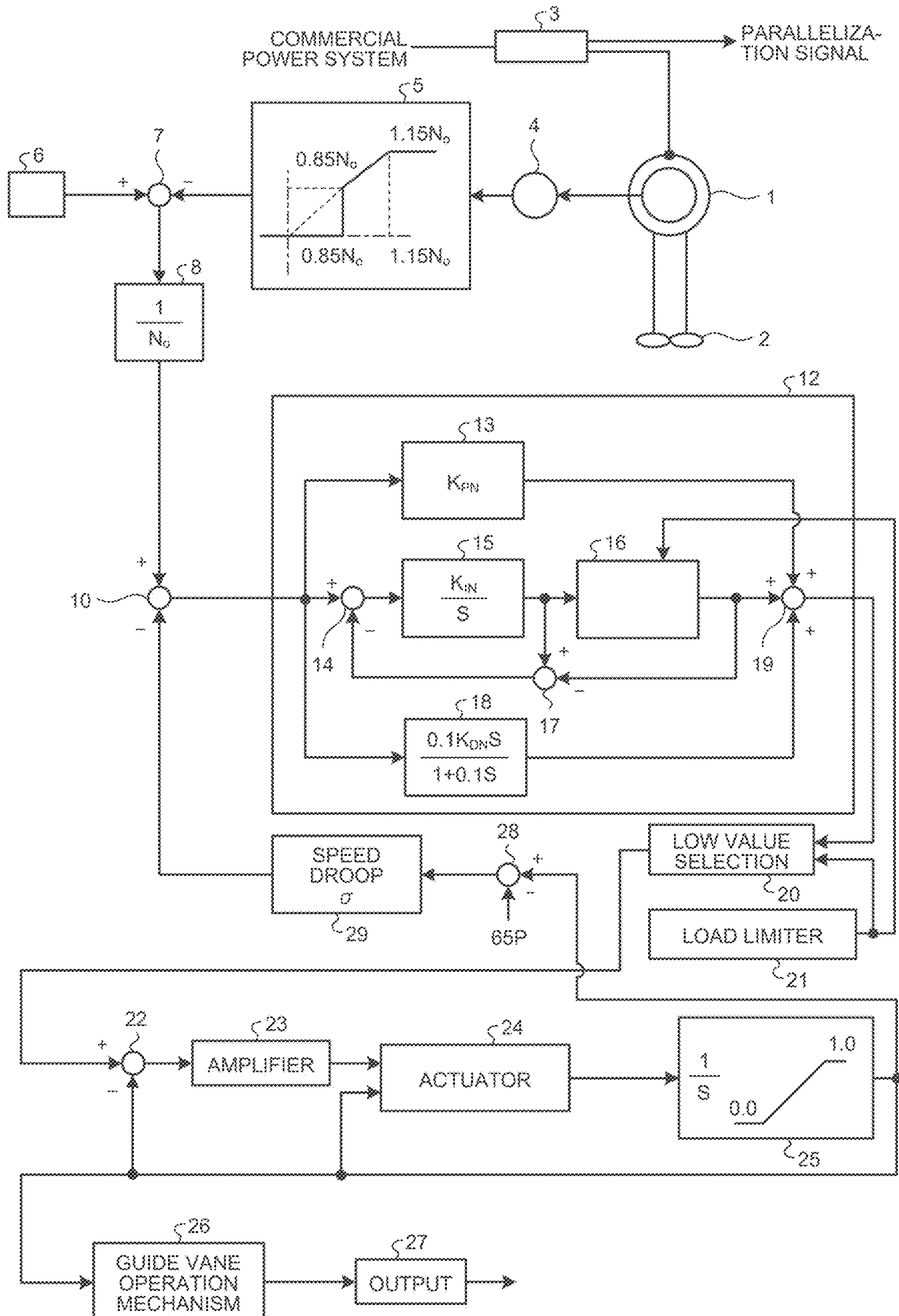
FIG. 7 (PRIOR ART)
