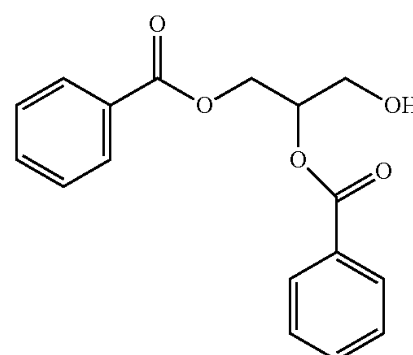
Glyceryl Di-Benzoate
