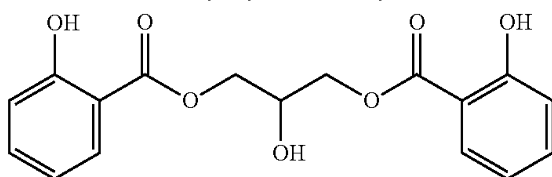
Glyceryl Di-Salicylate
