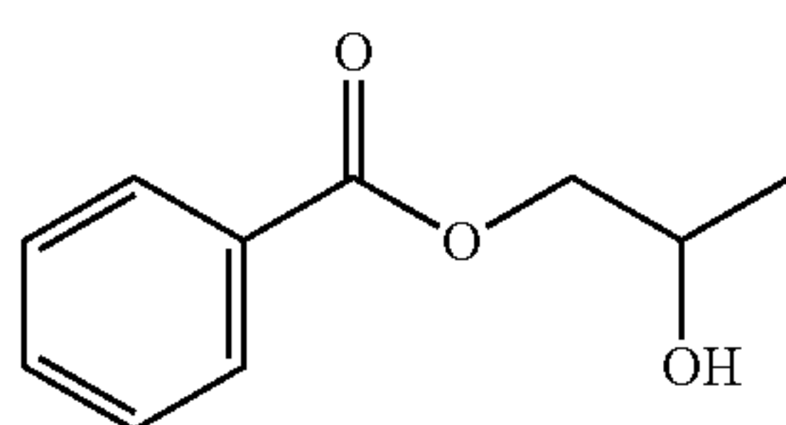
Propylene Glycol Mono-Benzoate
