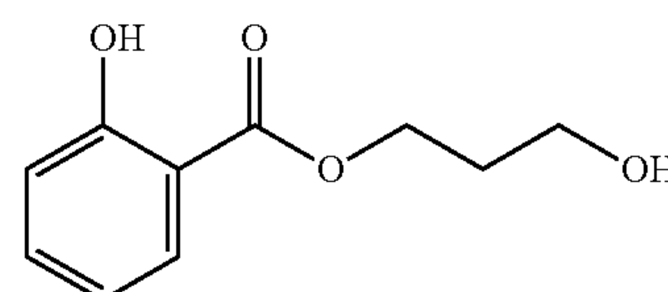
Propylene Glycol Mono-Salicylate
