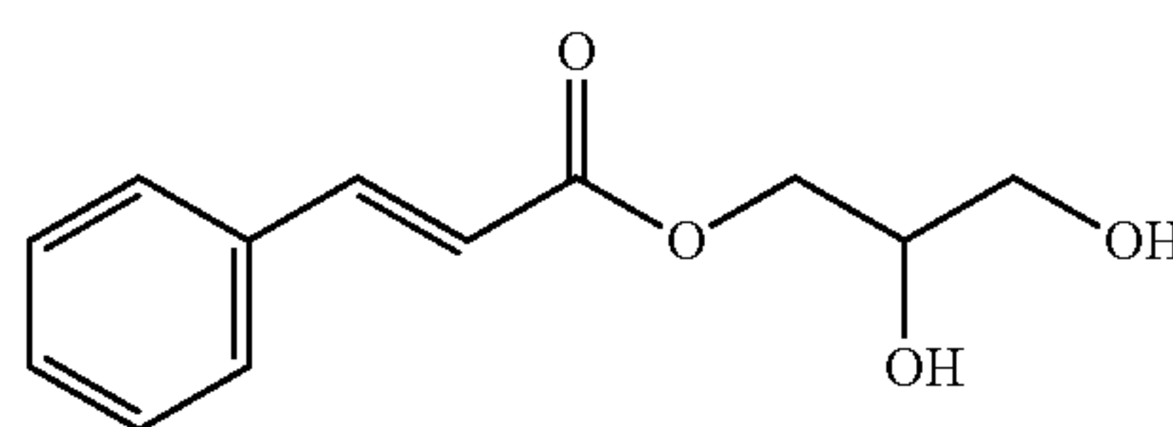
Glyceryl Mono-Cinnamate
