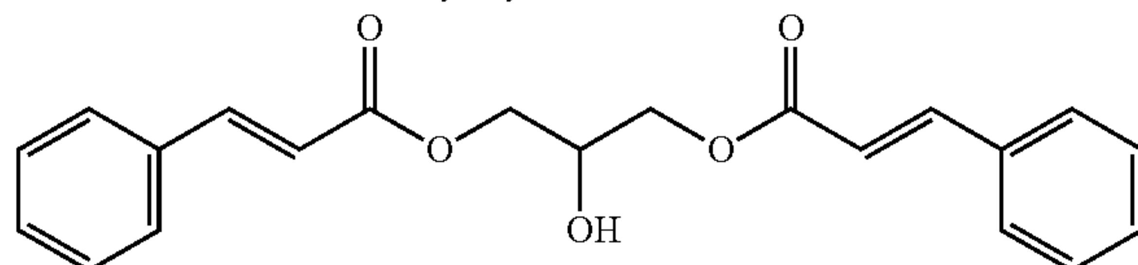
Glyceryl Di-Cinnamate
