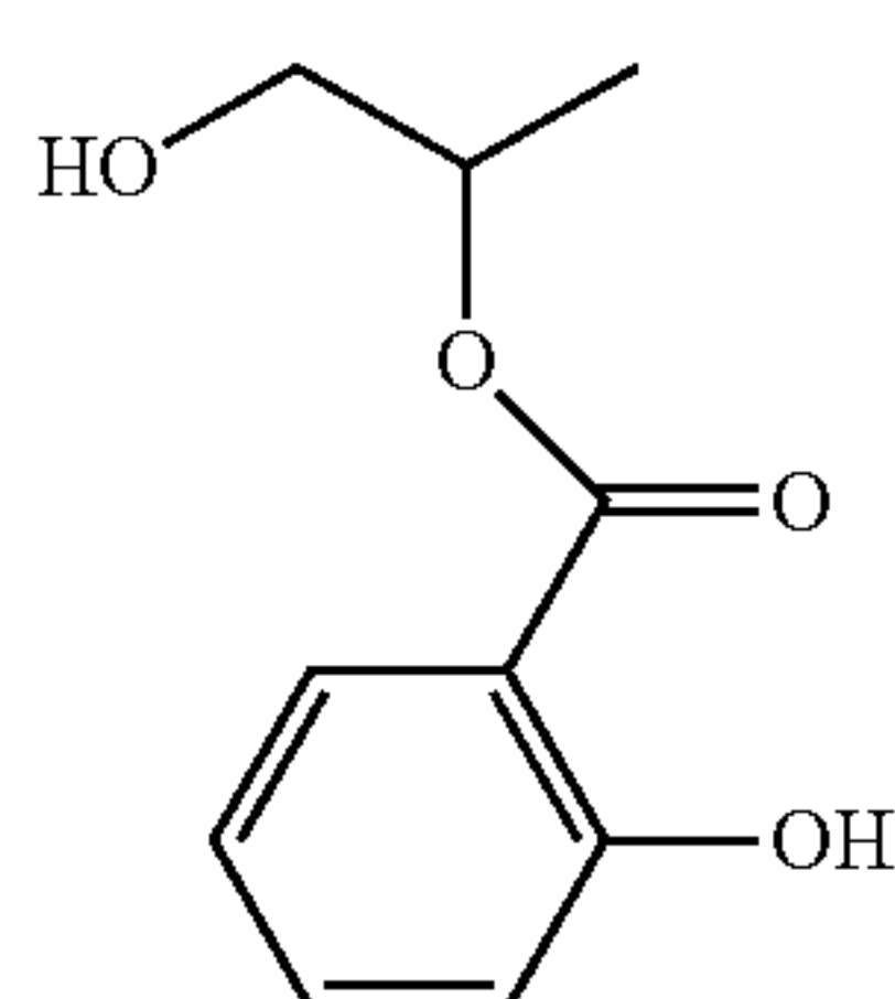
Propylene Glycol Mono-Salicylate
