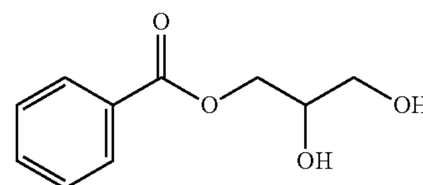
Glyceryl Mono-Benzoate
