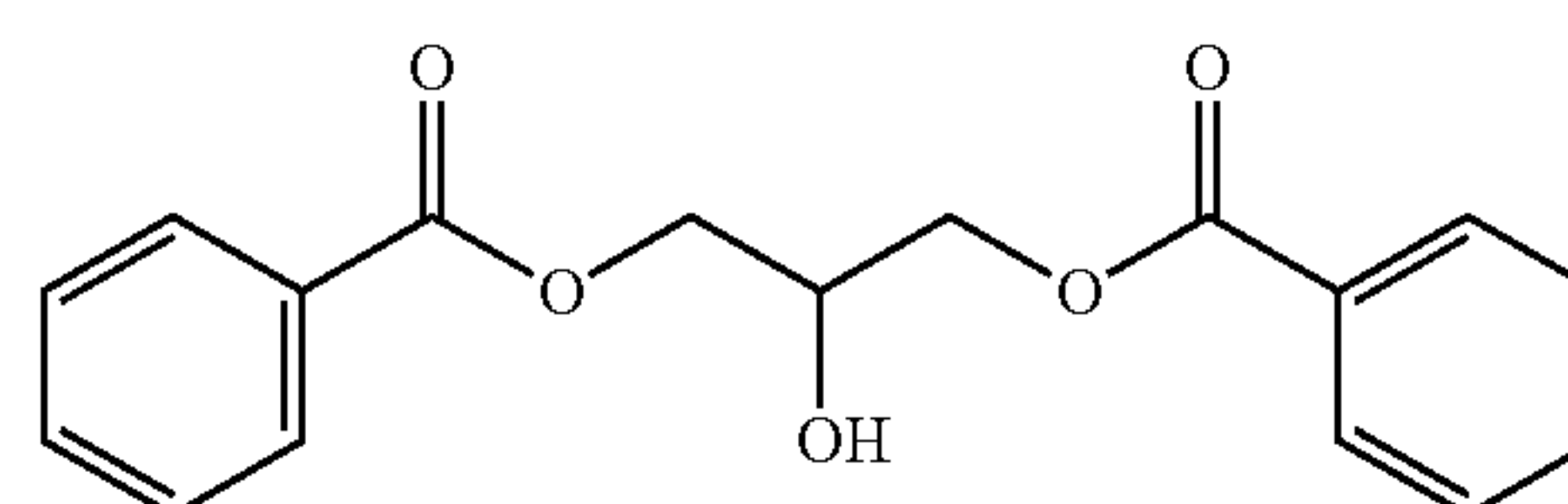
Glyceryl Di-Benzoate
