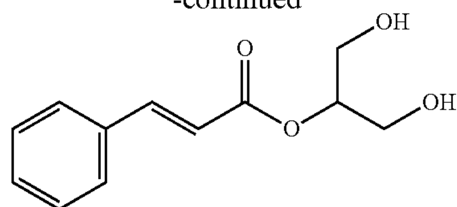
Glyceryl Mono-Cinnamate
