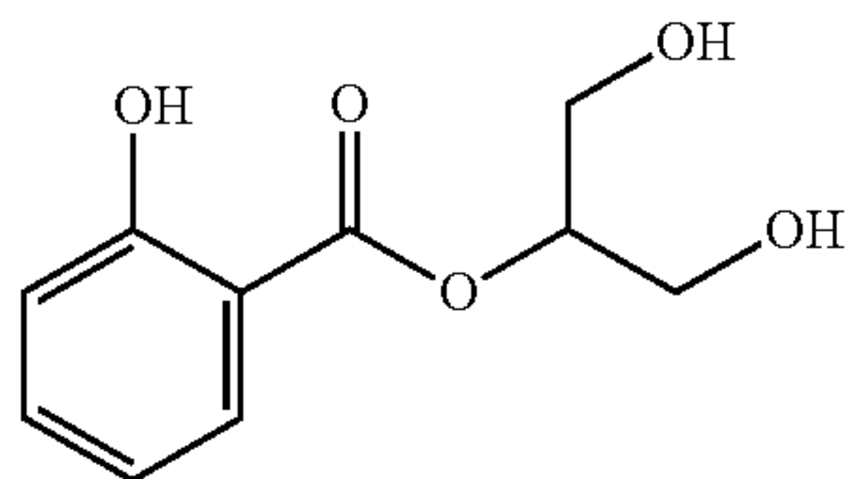
Glyceryl Mono-Salicylate
