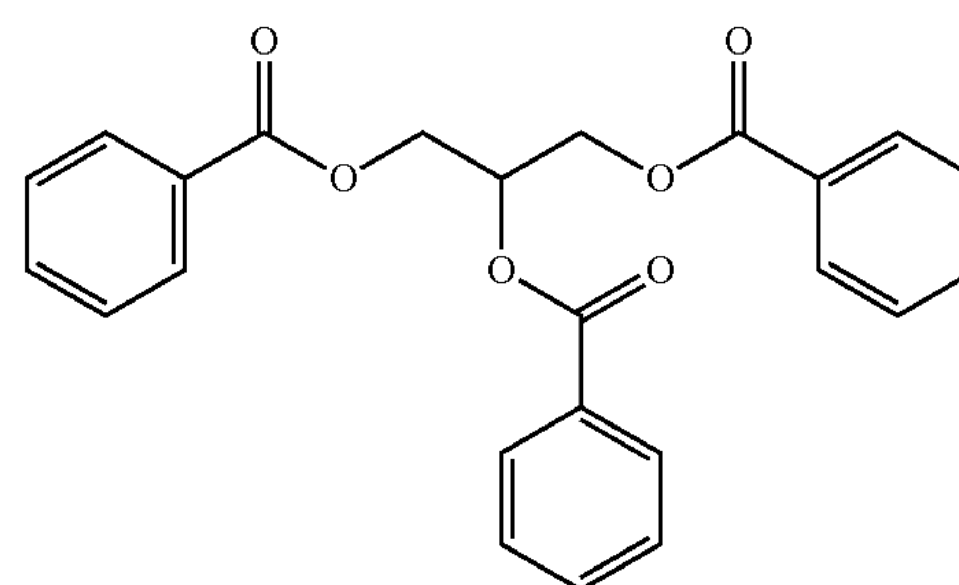
Glyceryl Tri-Benzoate
