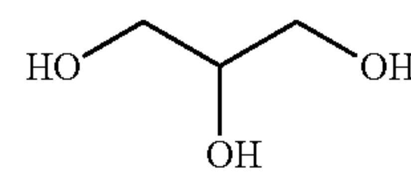
Glycerol
