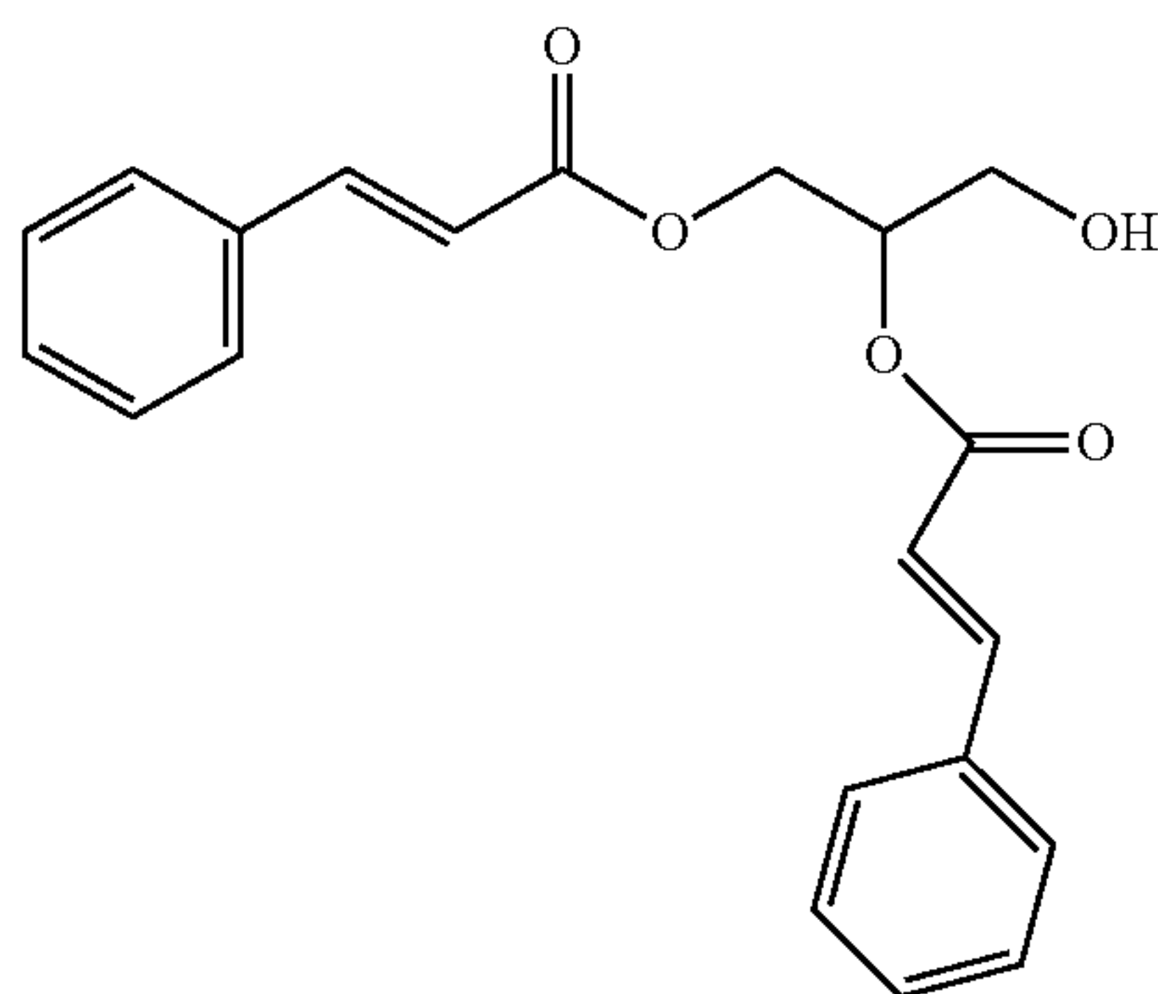
Glyceryl Di-Cinnamate
