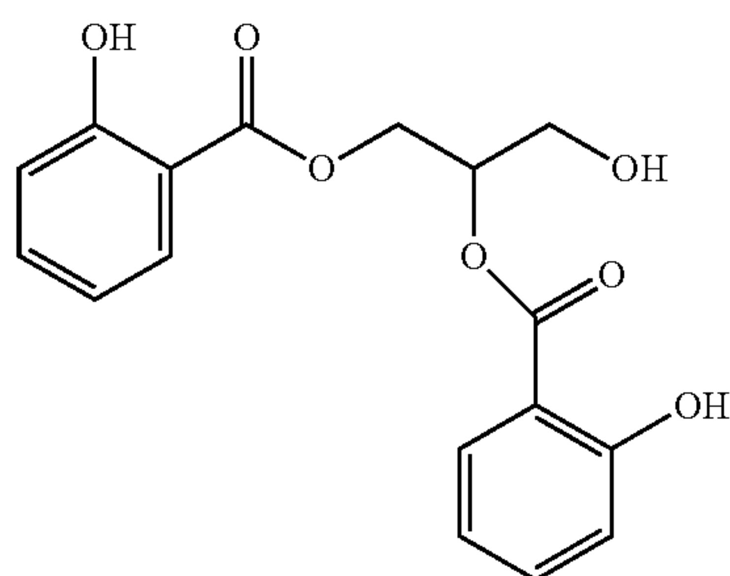
Glyceryl Di-Salicylate
