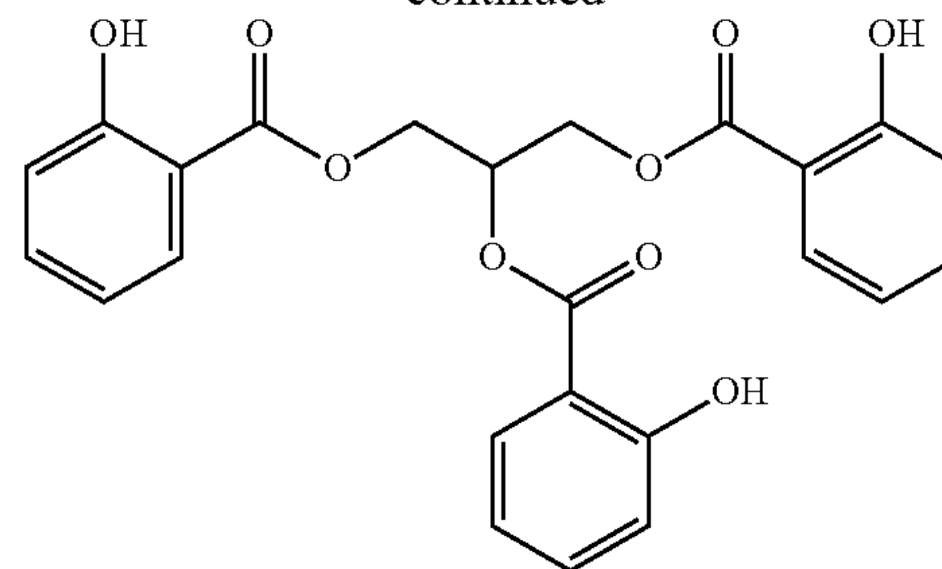
Glyceryl Tri-Salicylate
