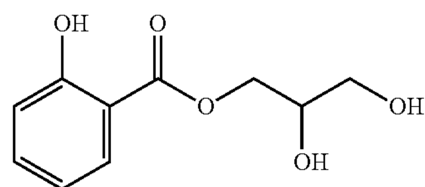
Glyceryl Mono-Salicylate
