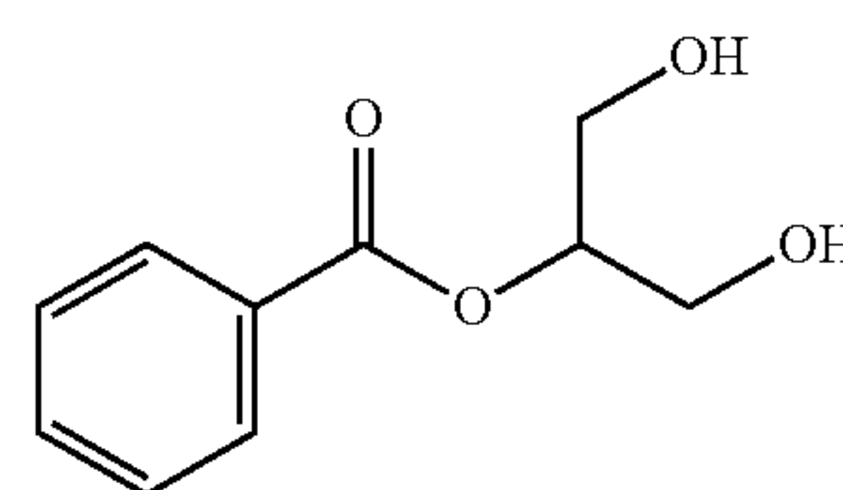
Glyceryl Mono-Benzoate
