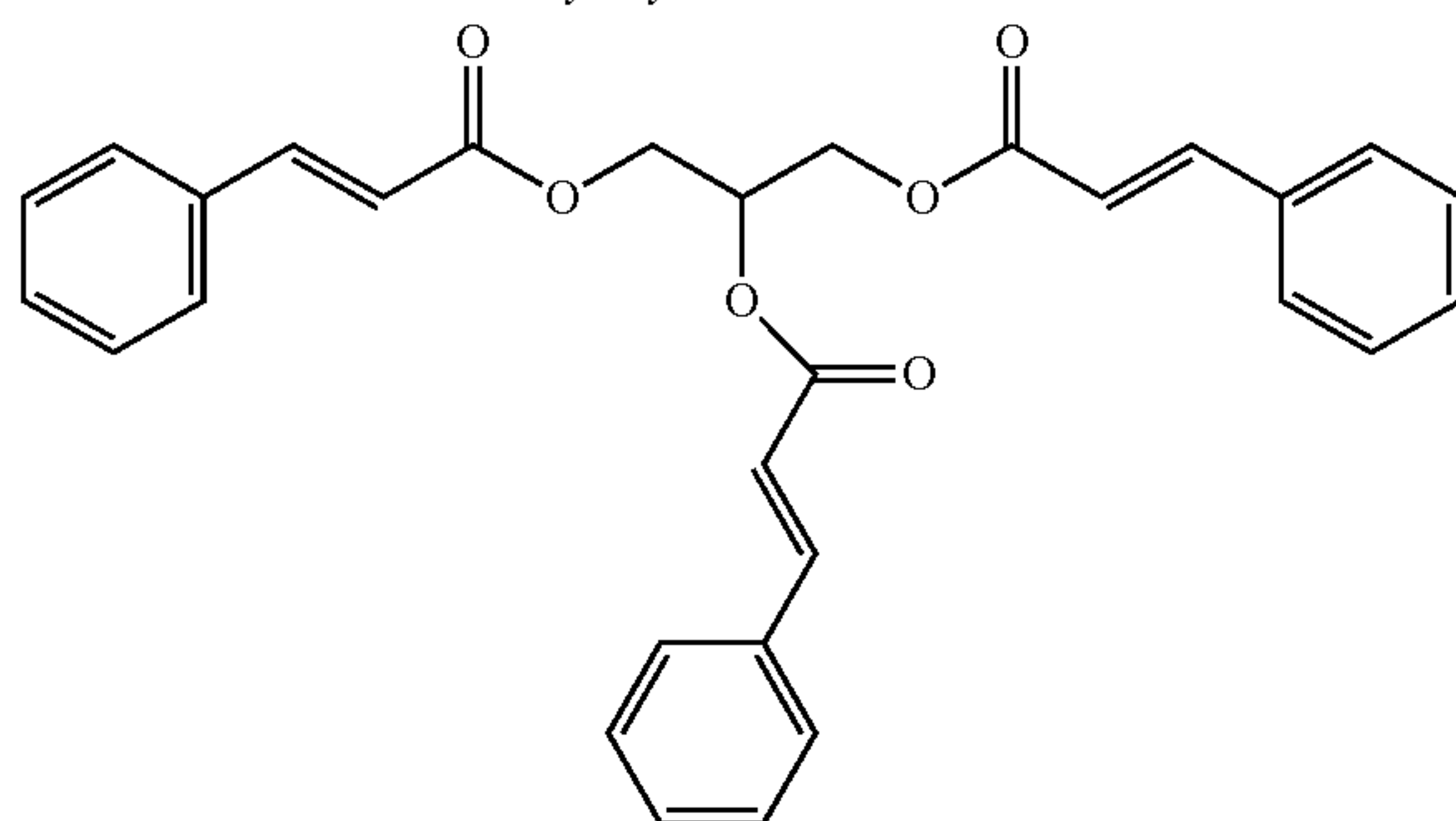
Glyceryl Tri-Cinnamate
