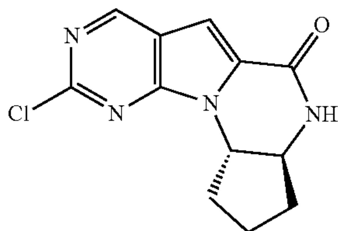
tert-butyl N-[(1S,2S)-2-[(5-bromo-2-chloro-pyrimidin-4-yl)amino]cyclopentyl]carbamate
