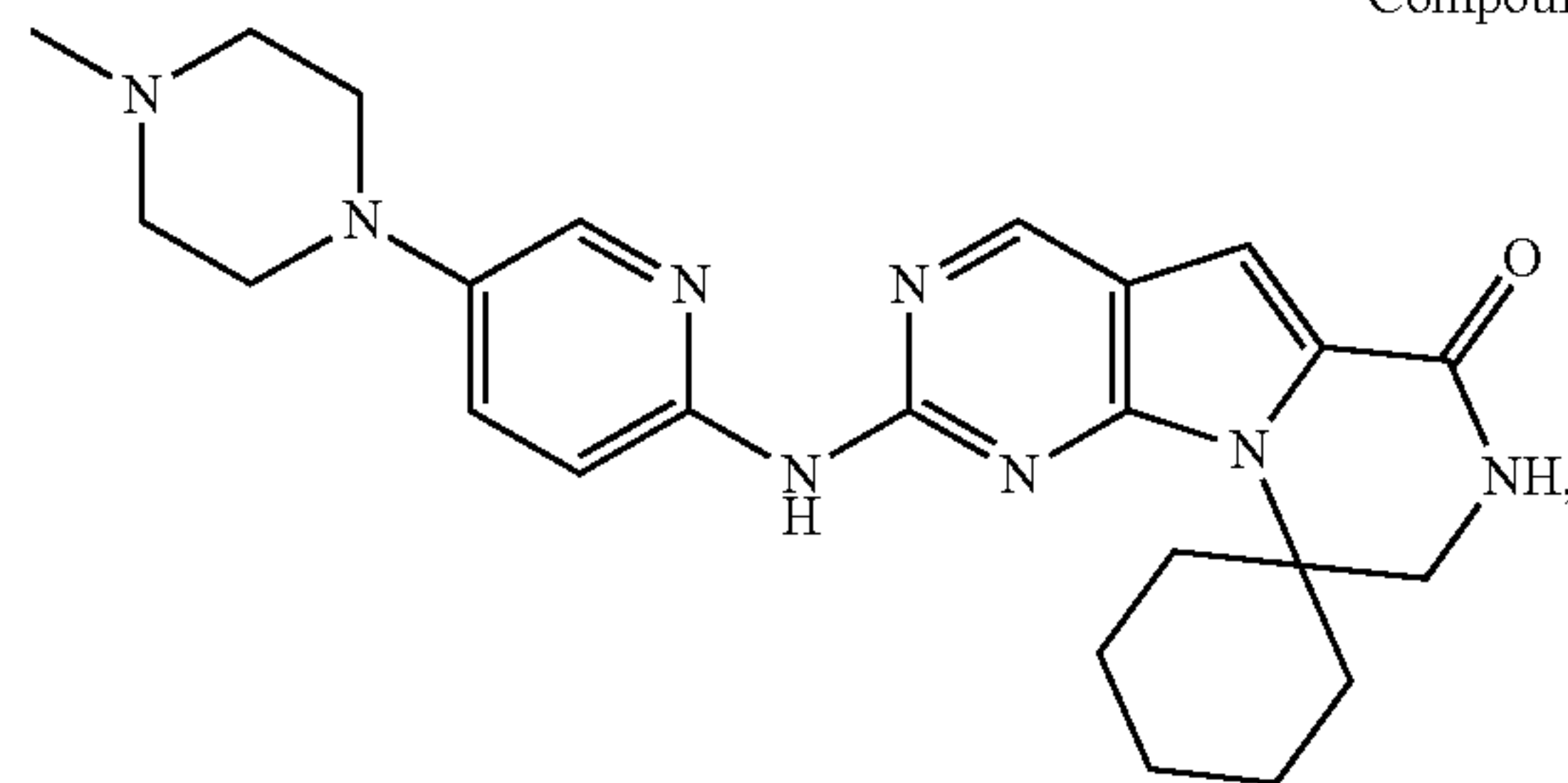
Compound T
