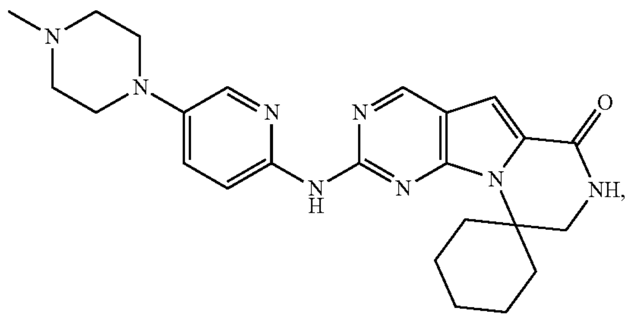
Compound T
