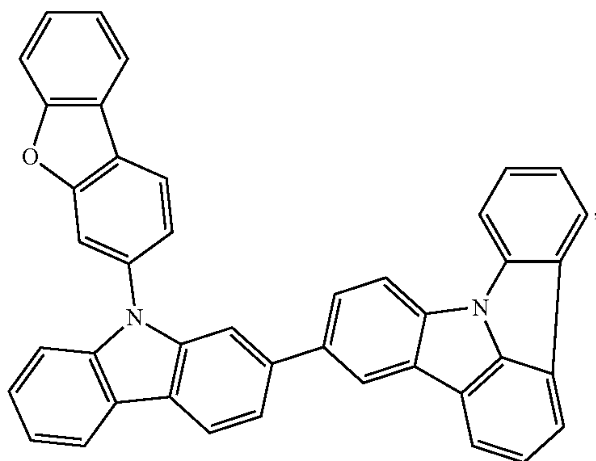
Compound E5
