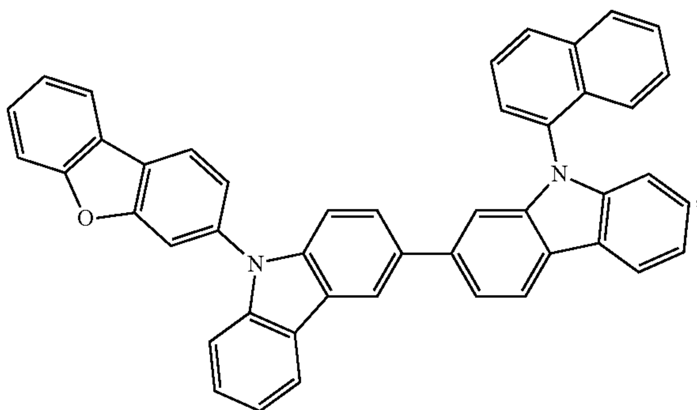
Compound A17
