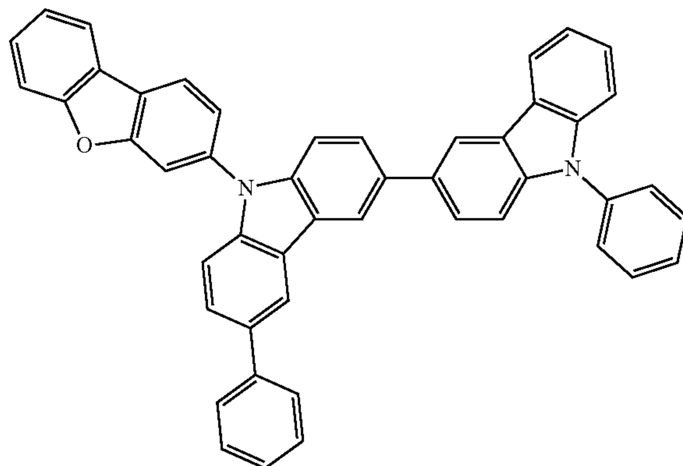
Compound A25
