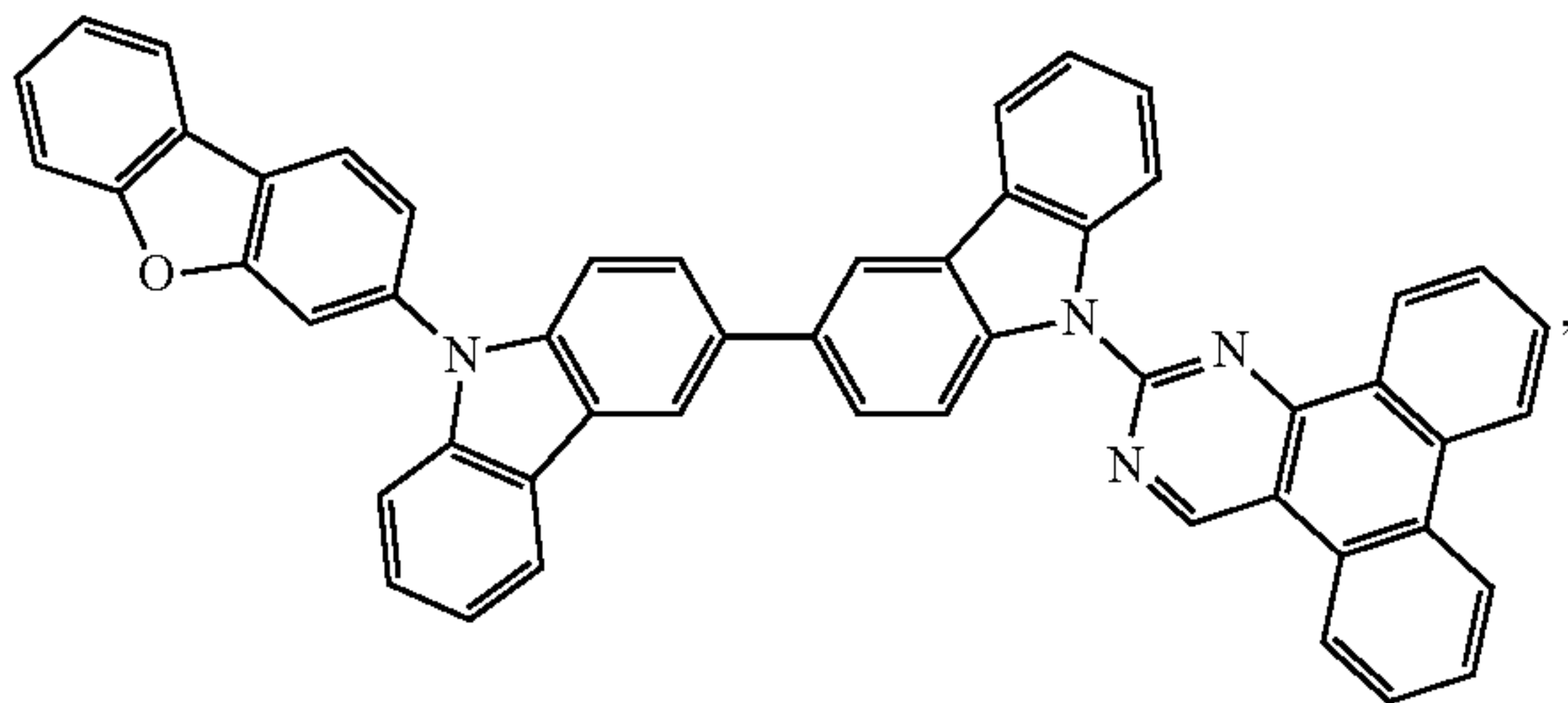
Compound A36
