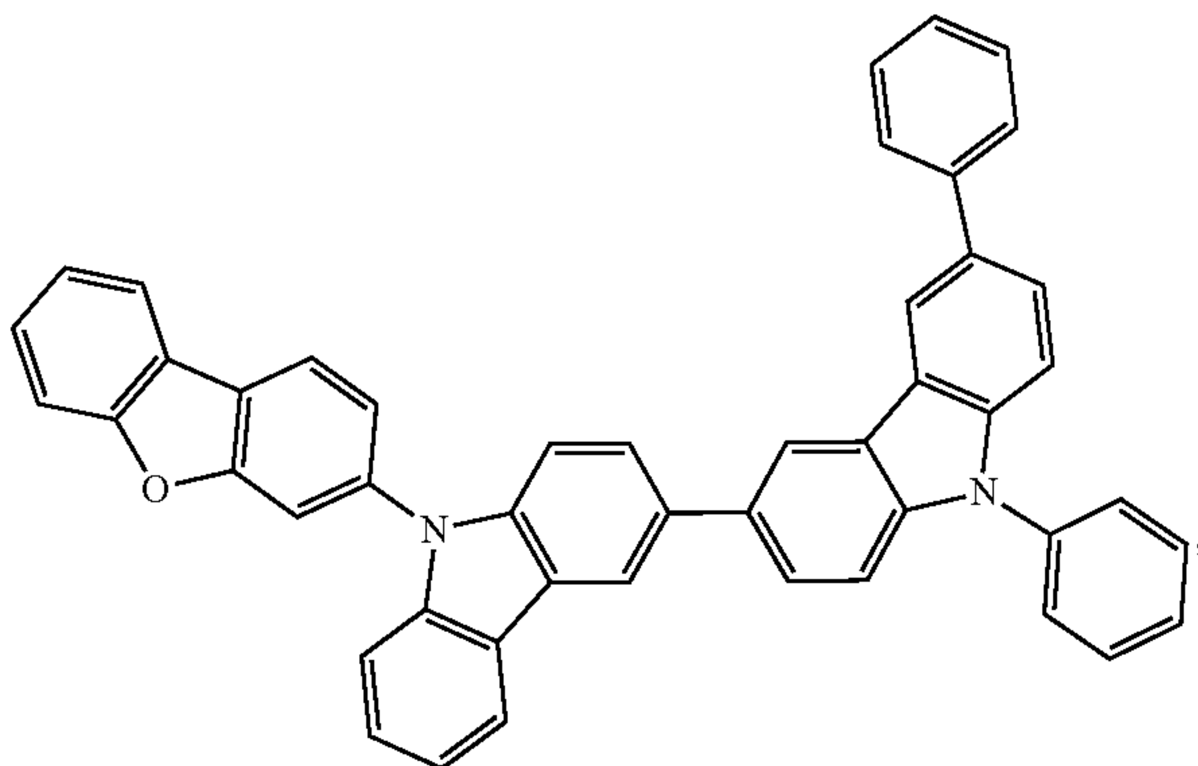
Compound A23
