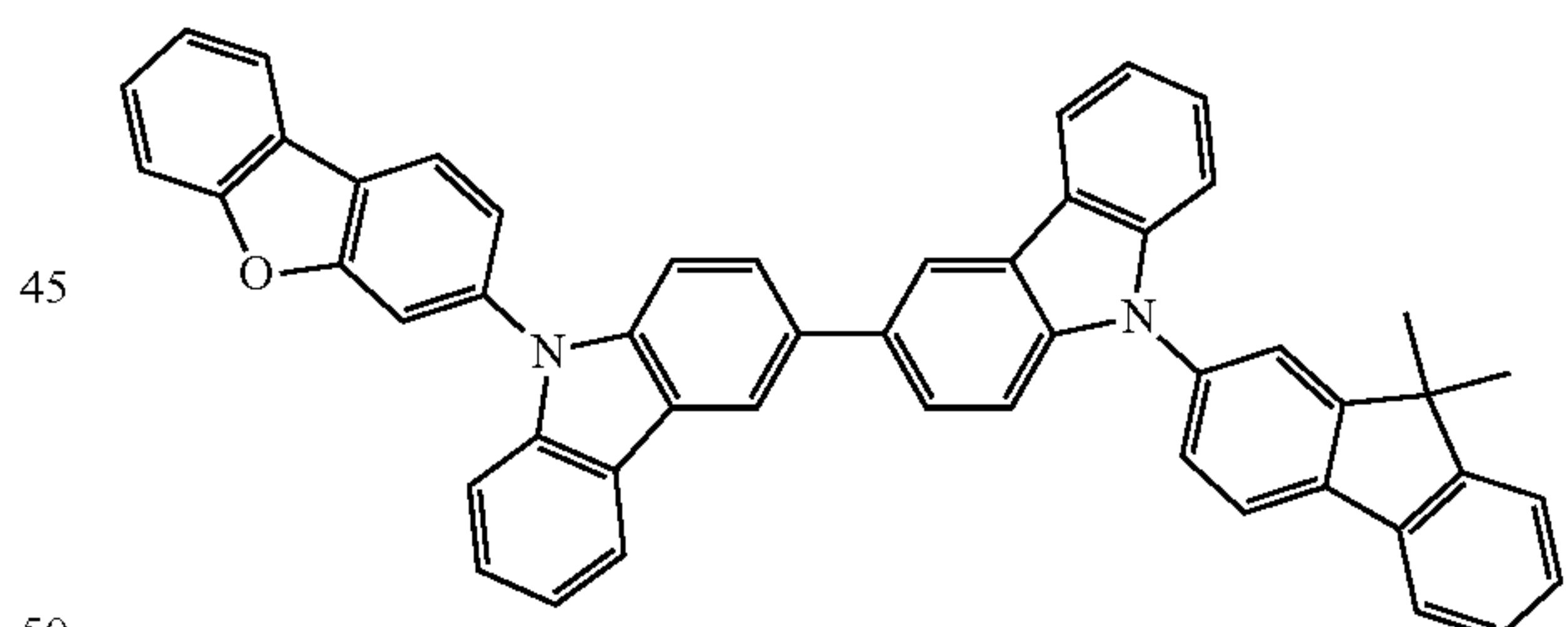
Compound A9
