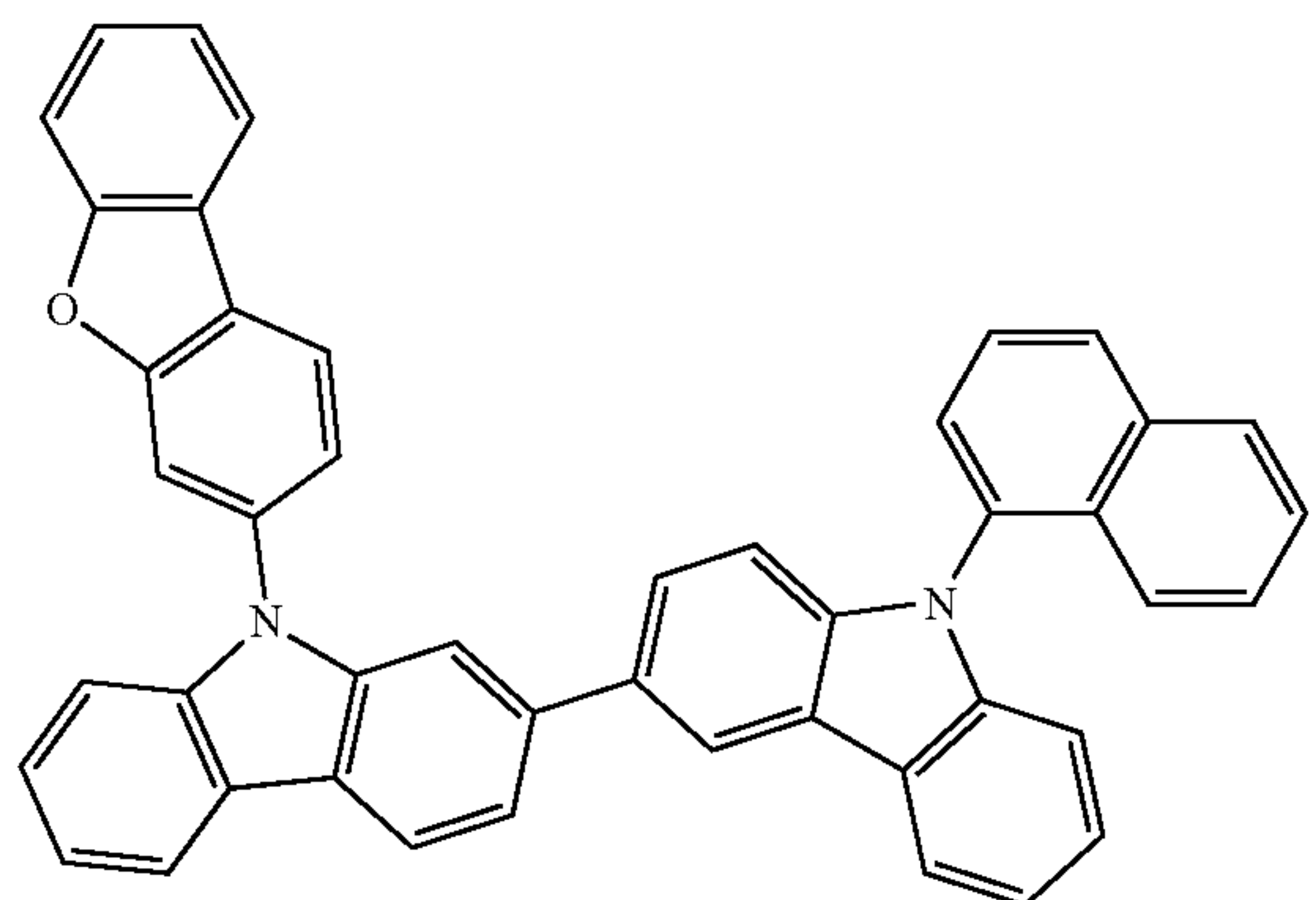
Compound A18
