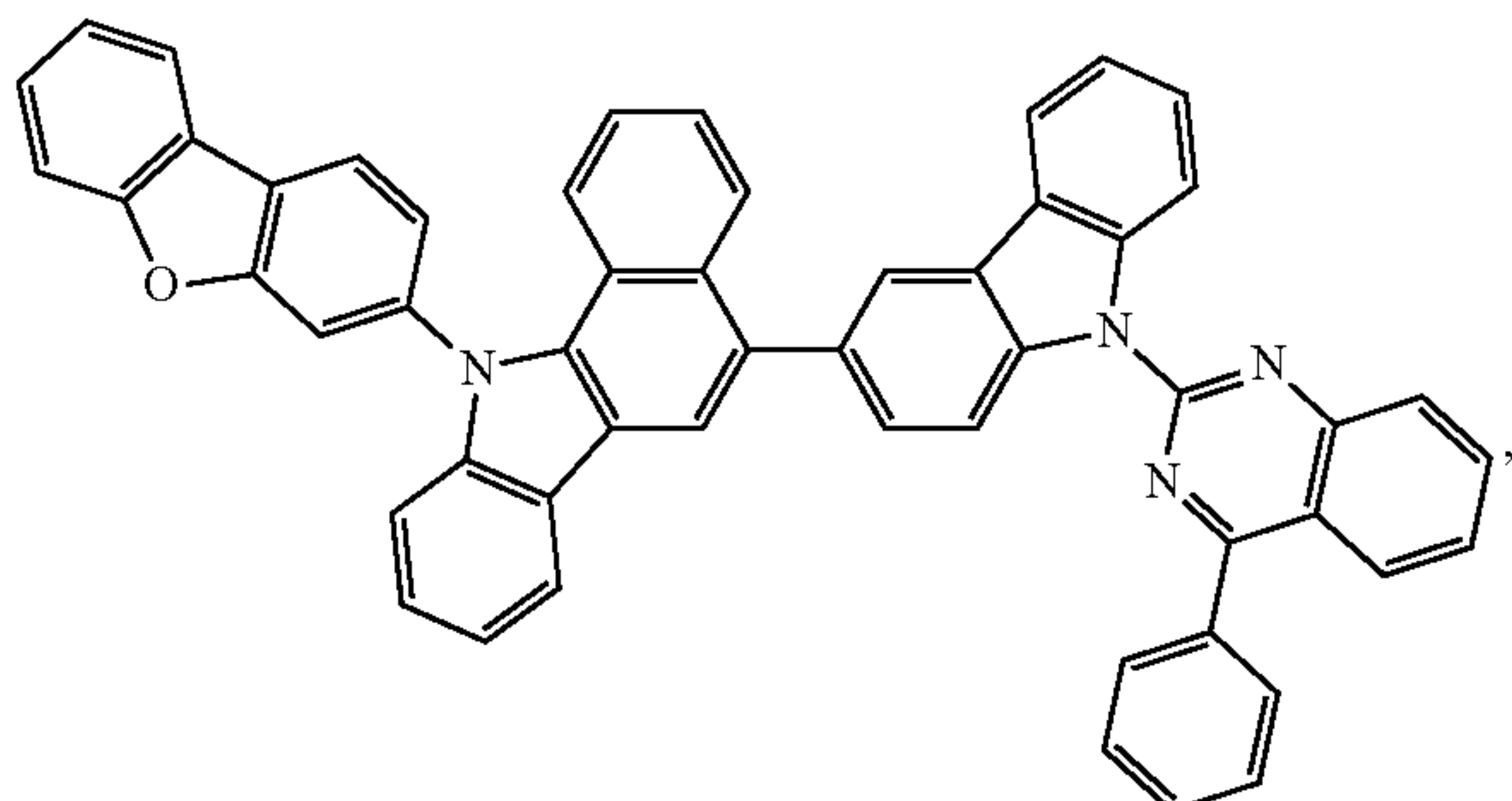
Compound A35
