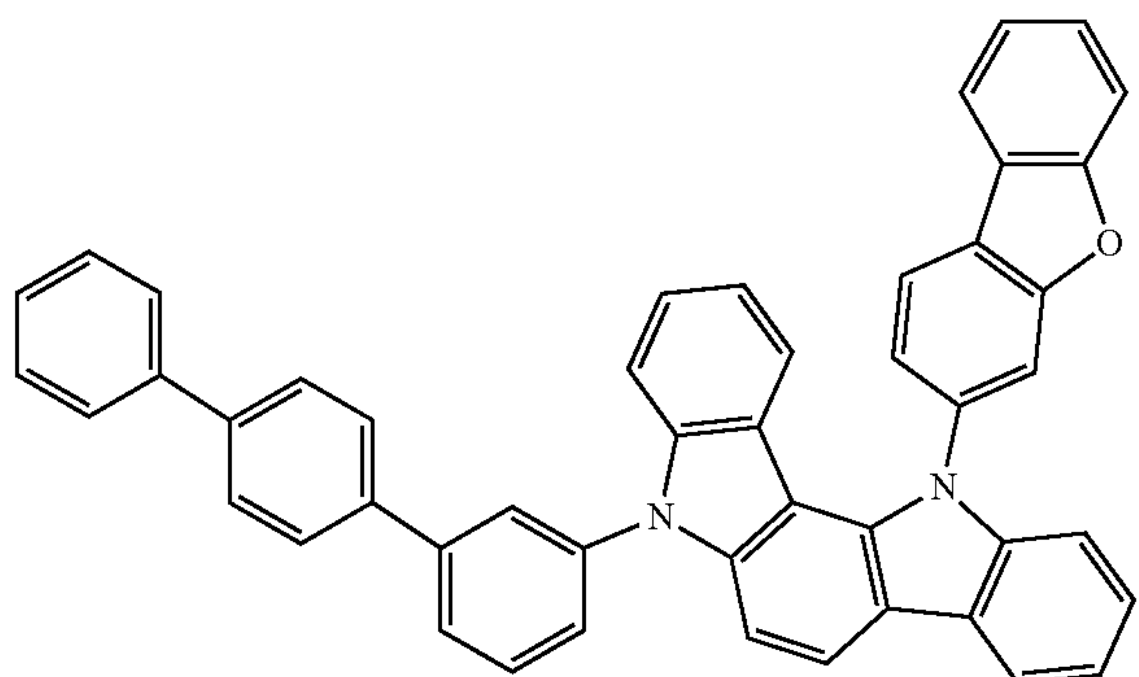
Compound B5
