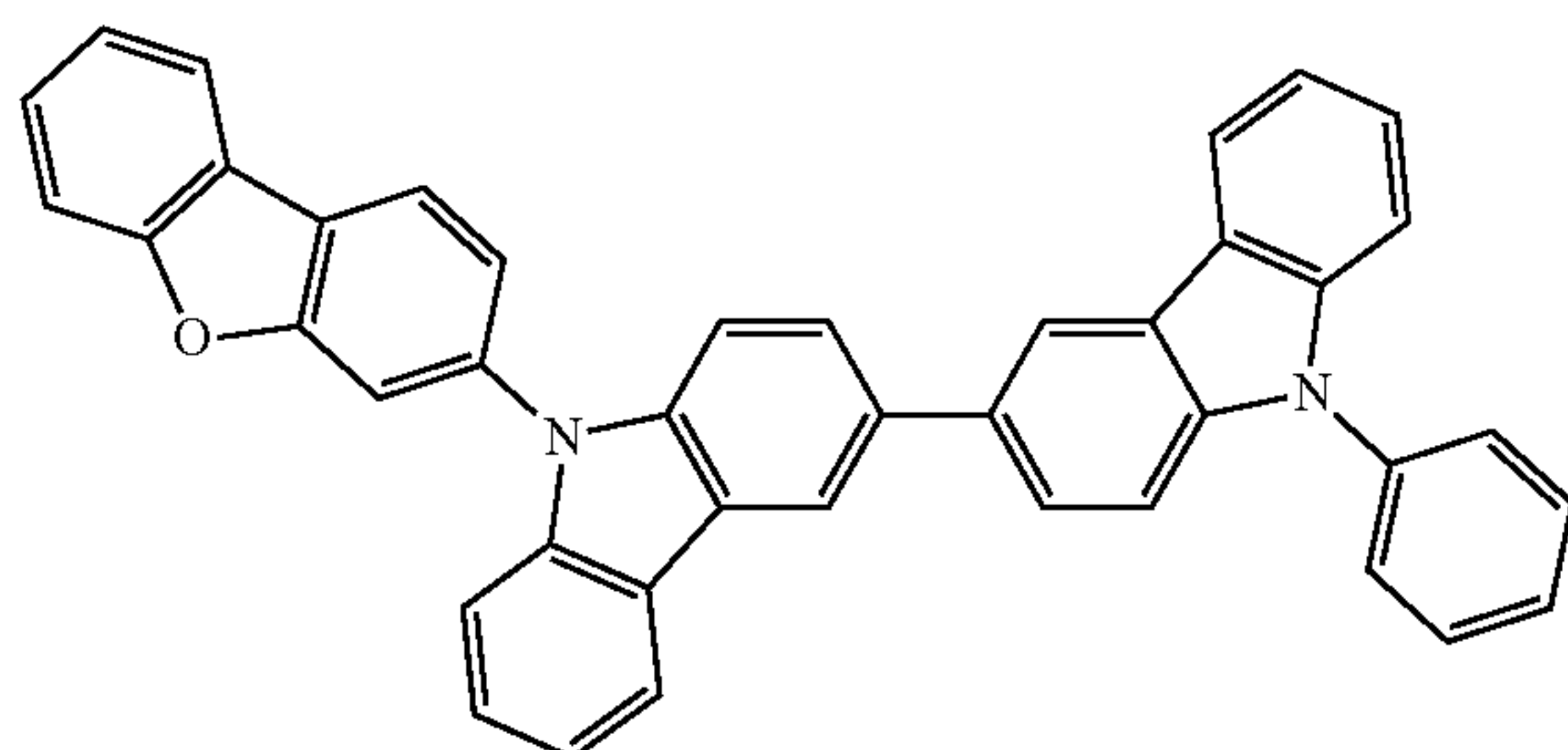
Compound A1
