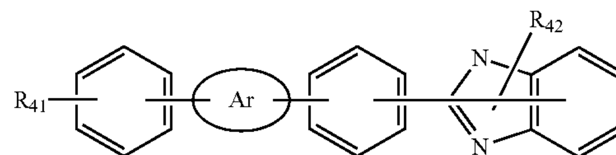
Chemical Formula 9
