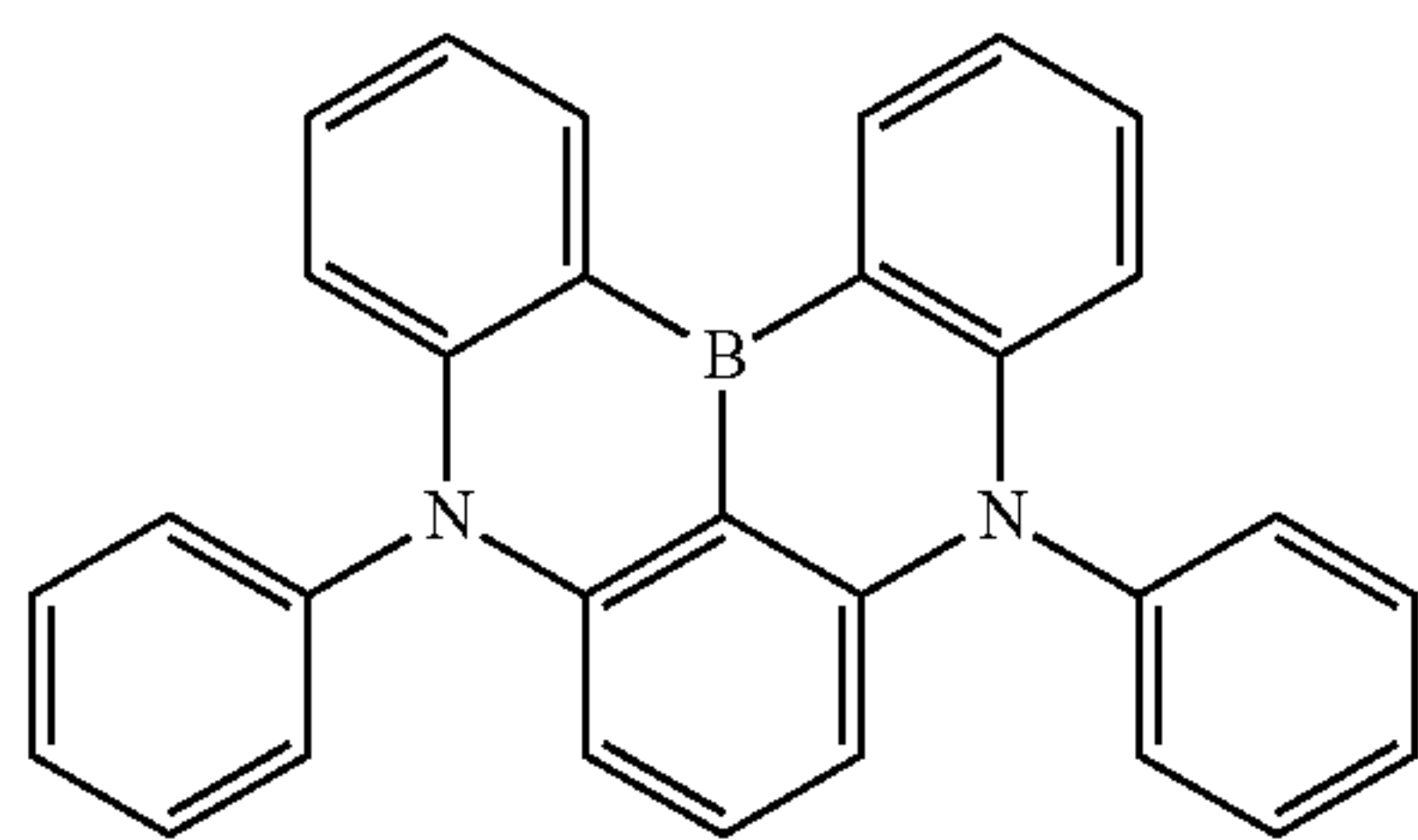
Chemical Formula 4
