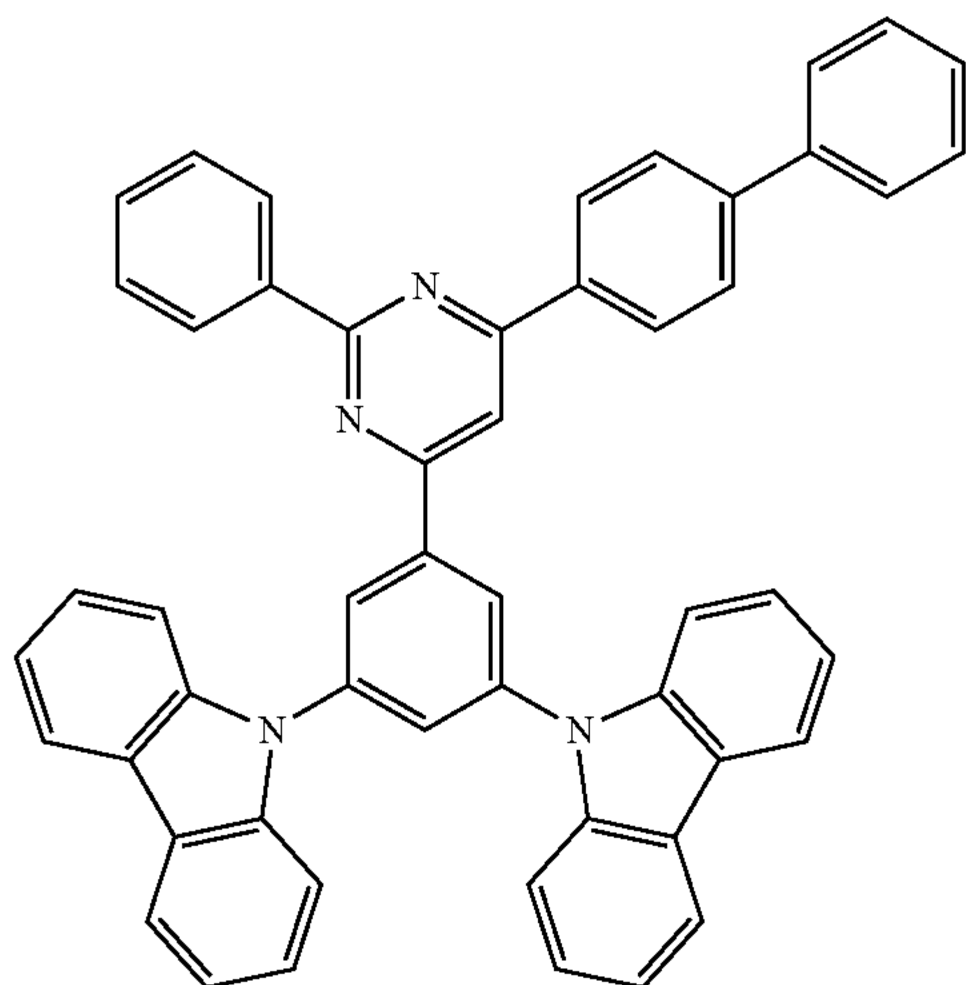
Chemical Formula 8
