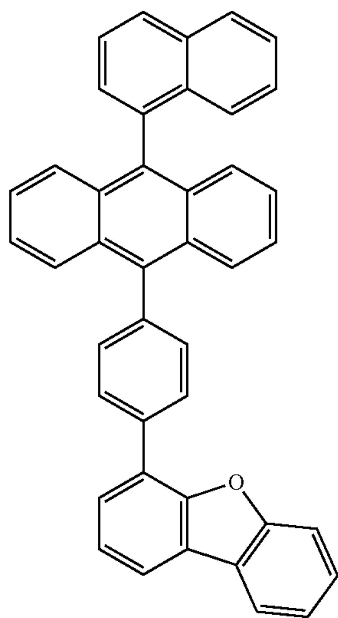
Host 4
