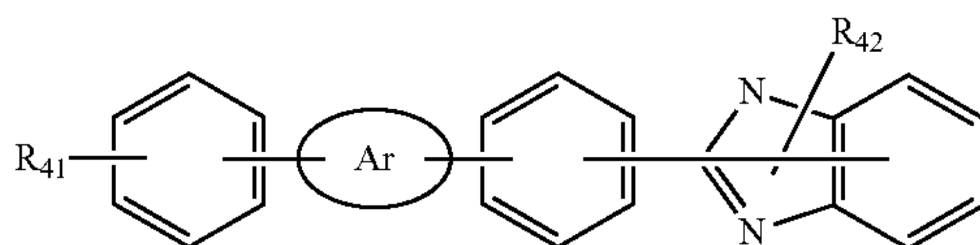
Chemical Formula 9
