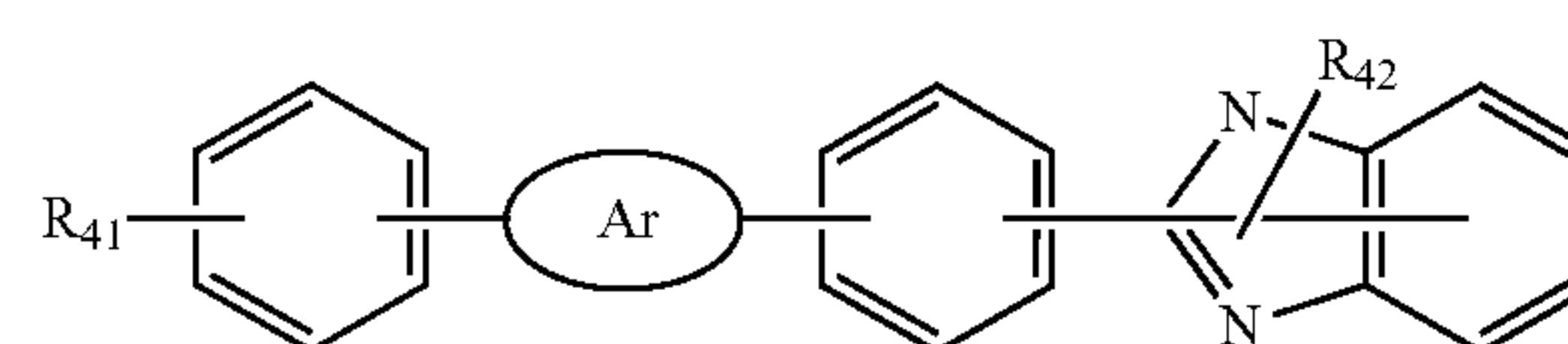
Chemical Formula 9
