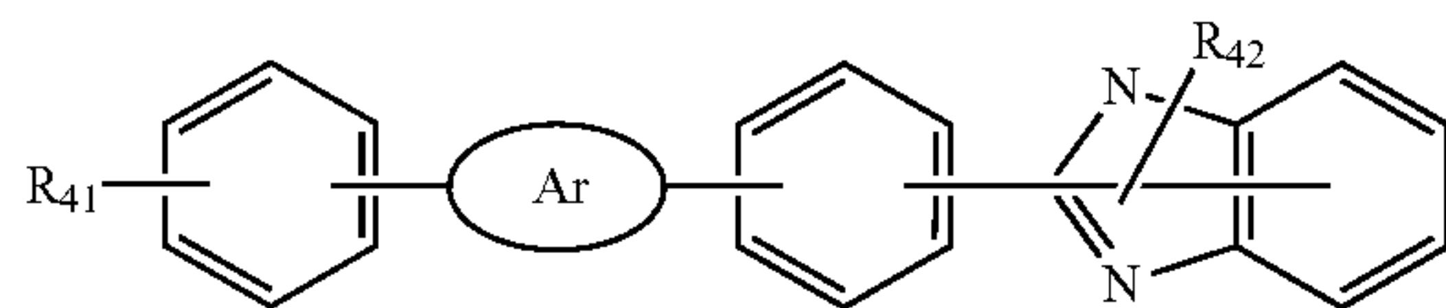
Chemical Formula 9
