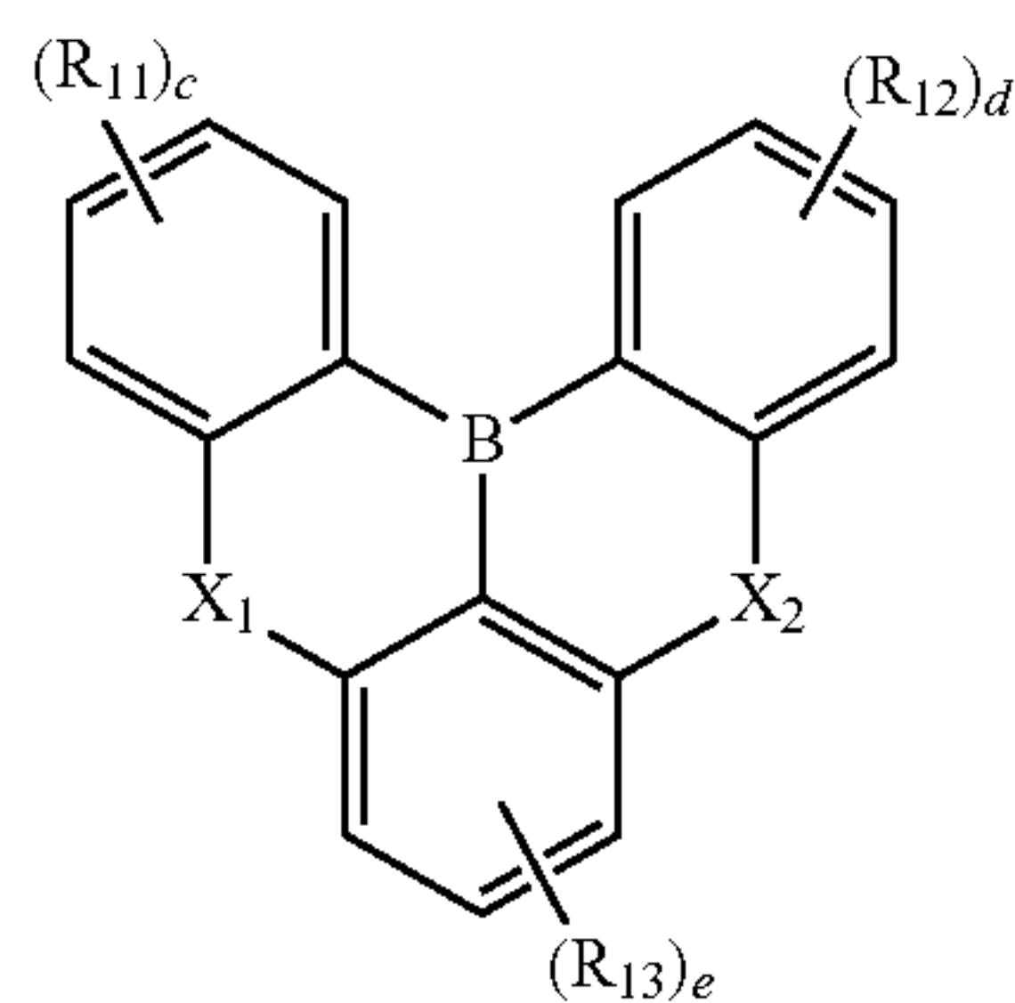
Chemical Formula 3
