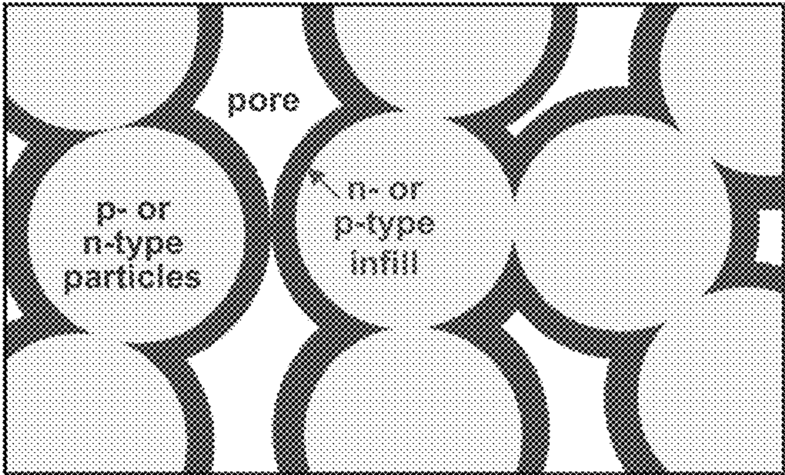
Infilled Compact
