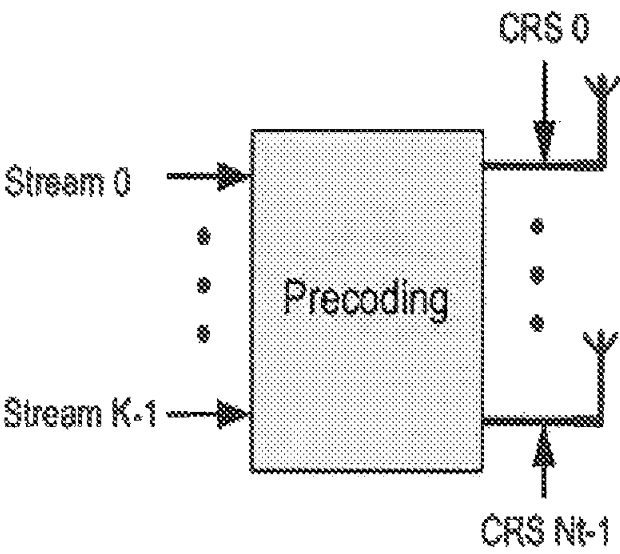
Figure 5 - Non-precoded cell-specific RS
