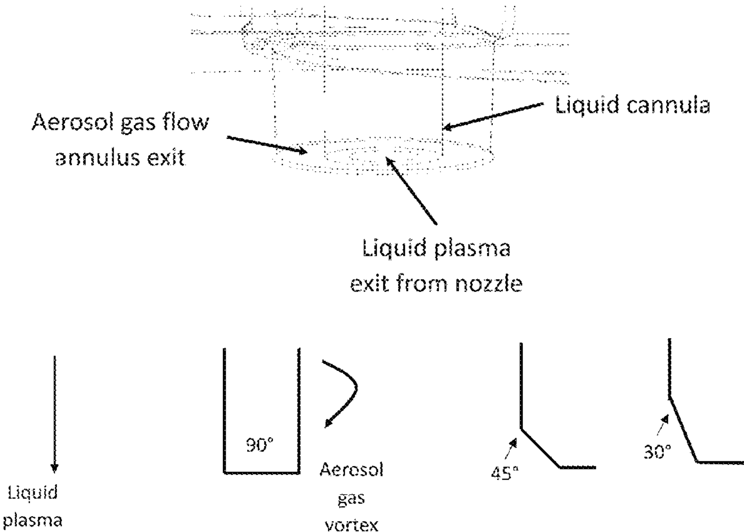
Liquid flow existing nozzle assembly
