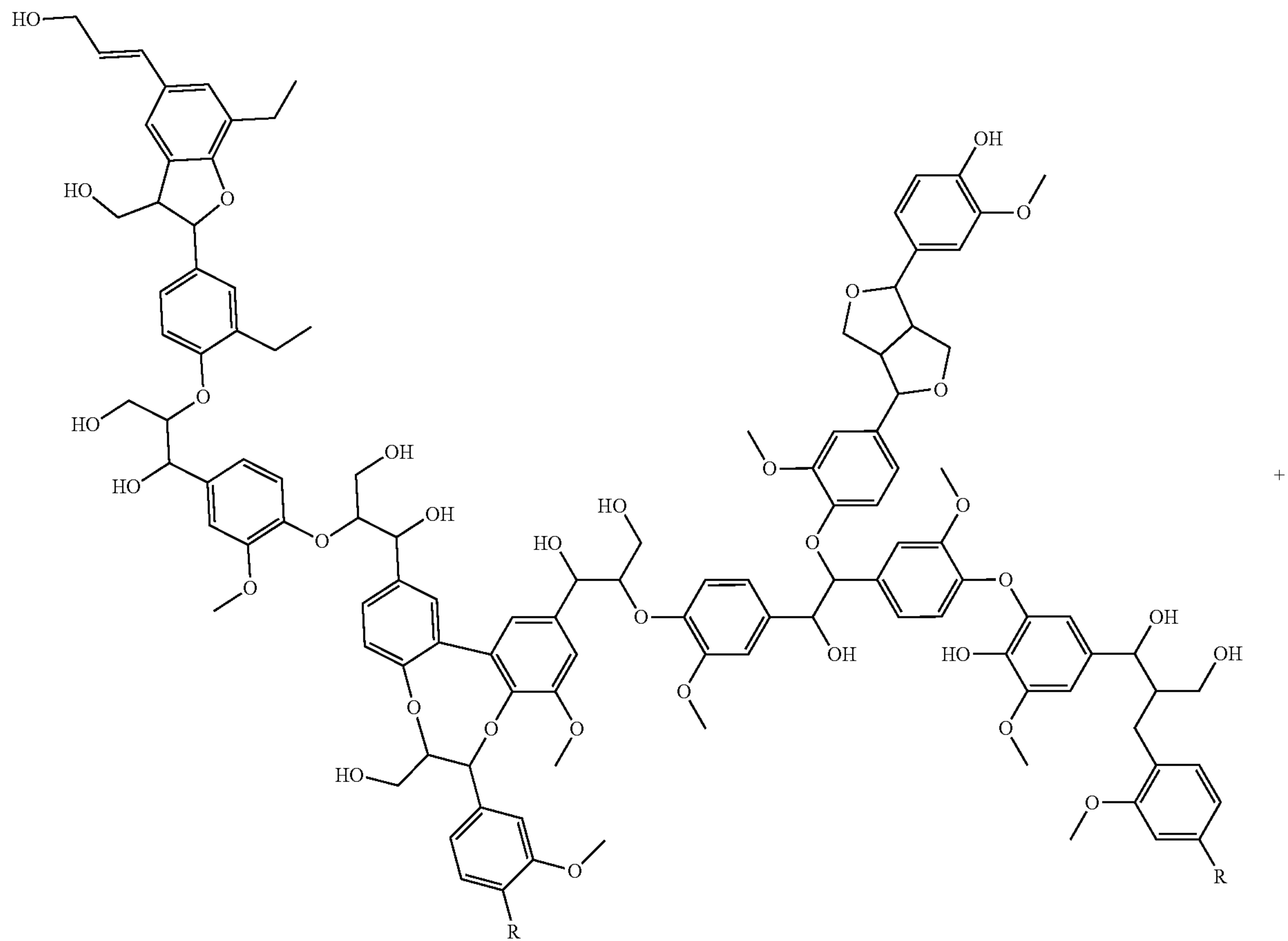
Scheme 7
