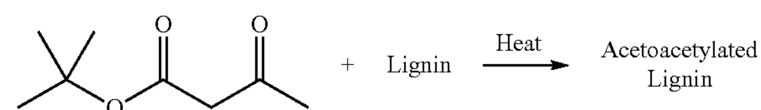
Scheme 5
