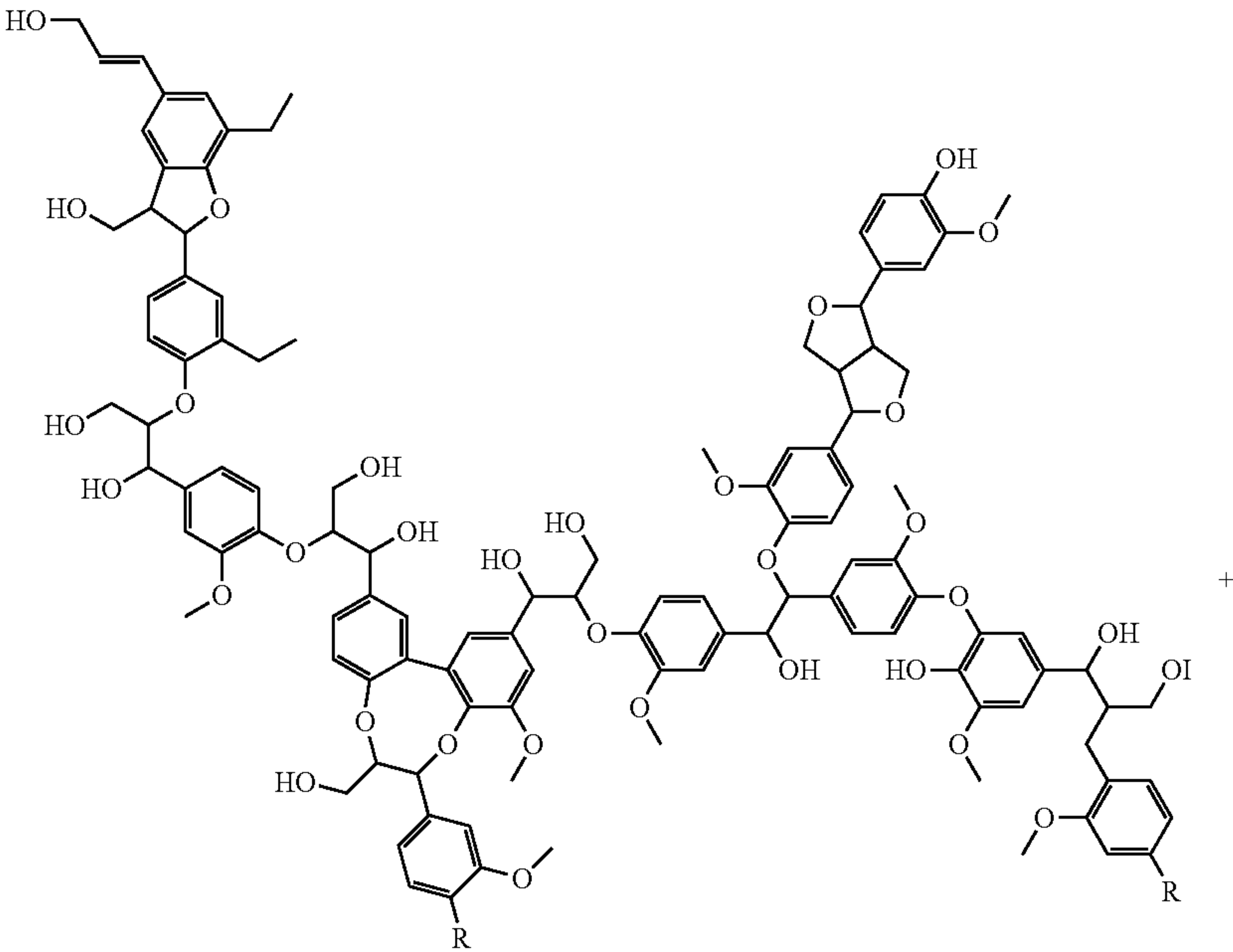
Scheme 12: Acetoacetylation of Kraft lignin.
