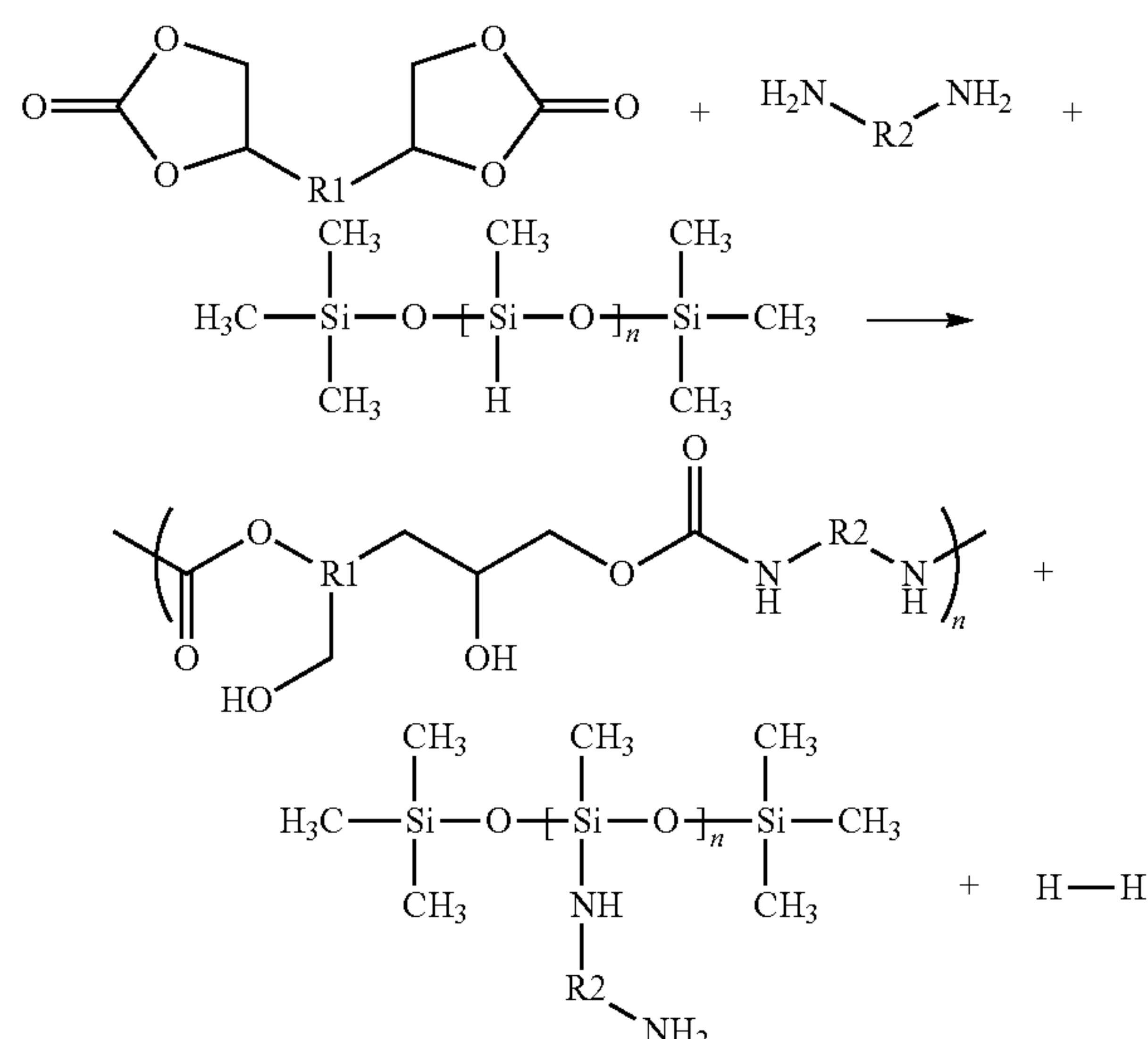
Scheme 3. Reaction Scheme of Polyfunctional Amine and Silane Blowing Agent to Make Polyurethane Foams
