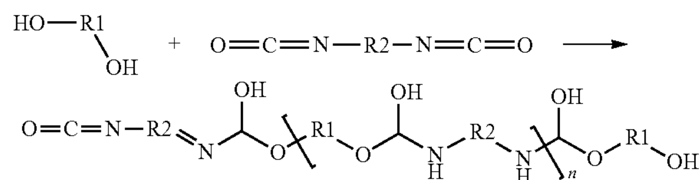
Scheme 2. General Reaction Scheme of Polyurethanes
