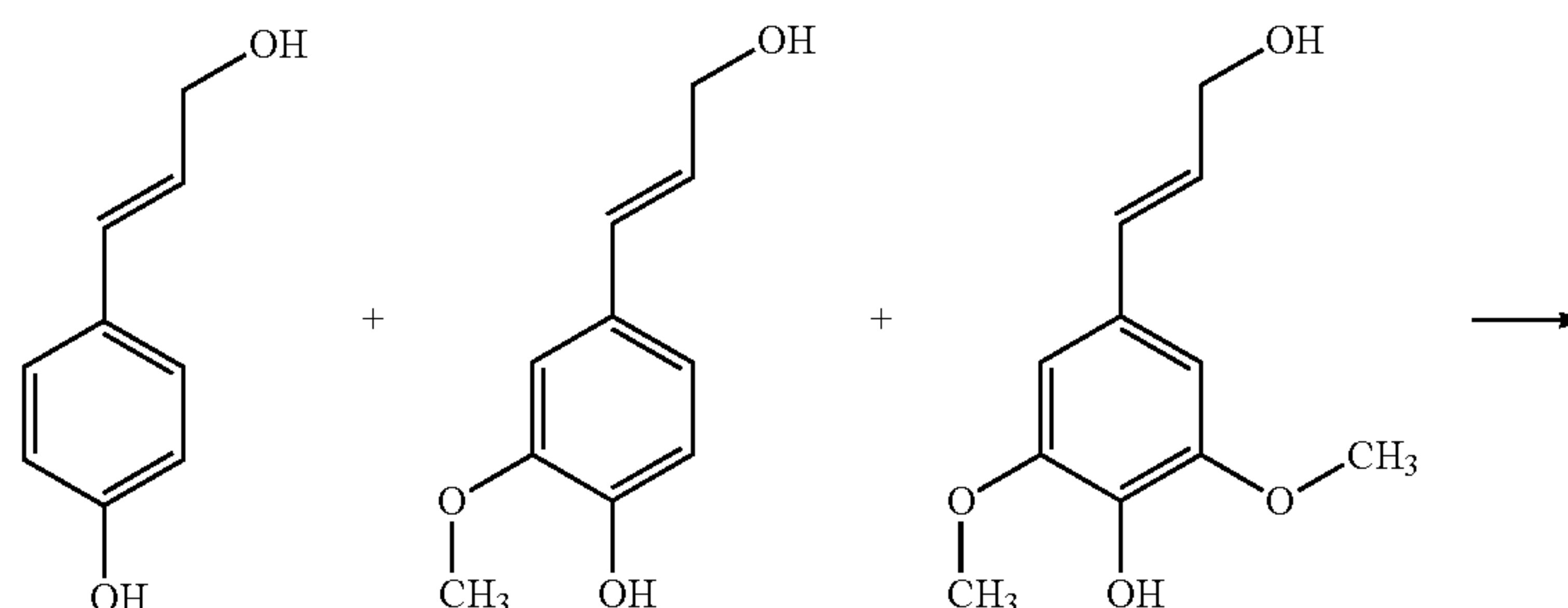
Scheme 1. Reaction Scheme of Radical Polymerization of Lignin Monomers
