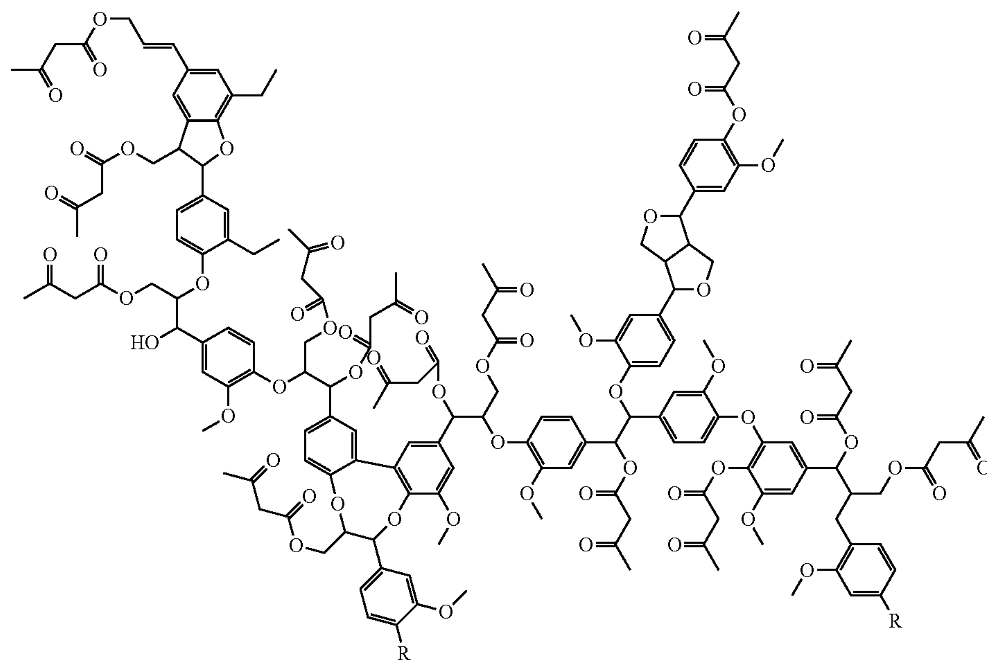
(B) Representative structure of acetoacetylated Kraft Lignin.
