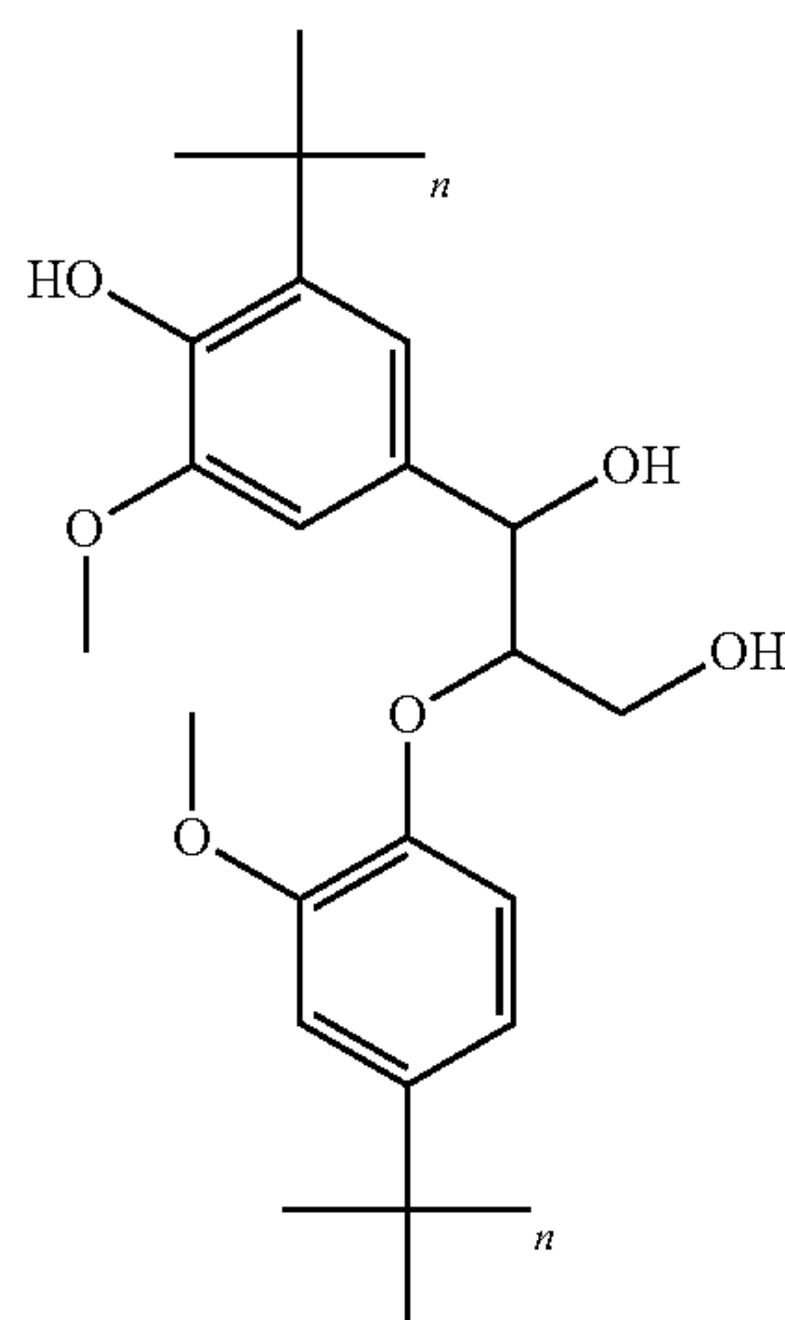
(C) Representative structure of depolymerized lignin.
