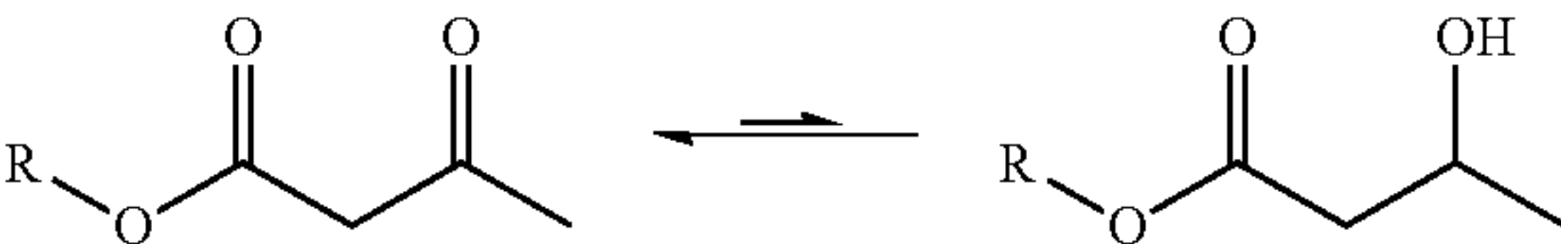
Scheme 13: Keto-enol tautomerization of acetoacetate groups
