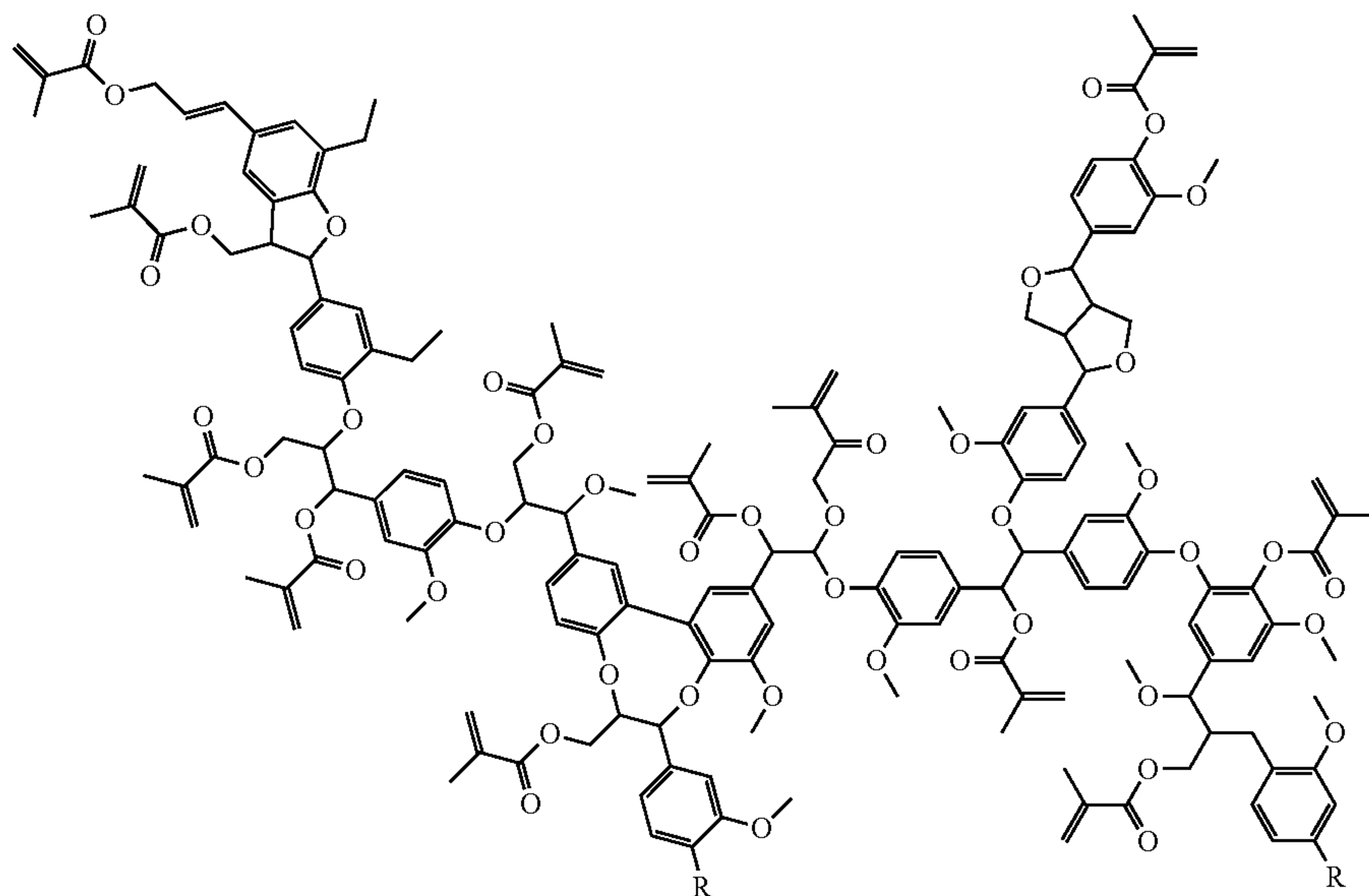
(D) Representative structure of Kraft lignin functionalized with methacrylate groups
