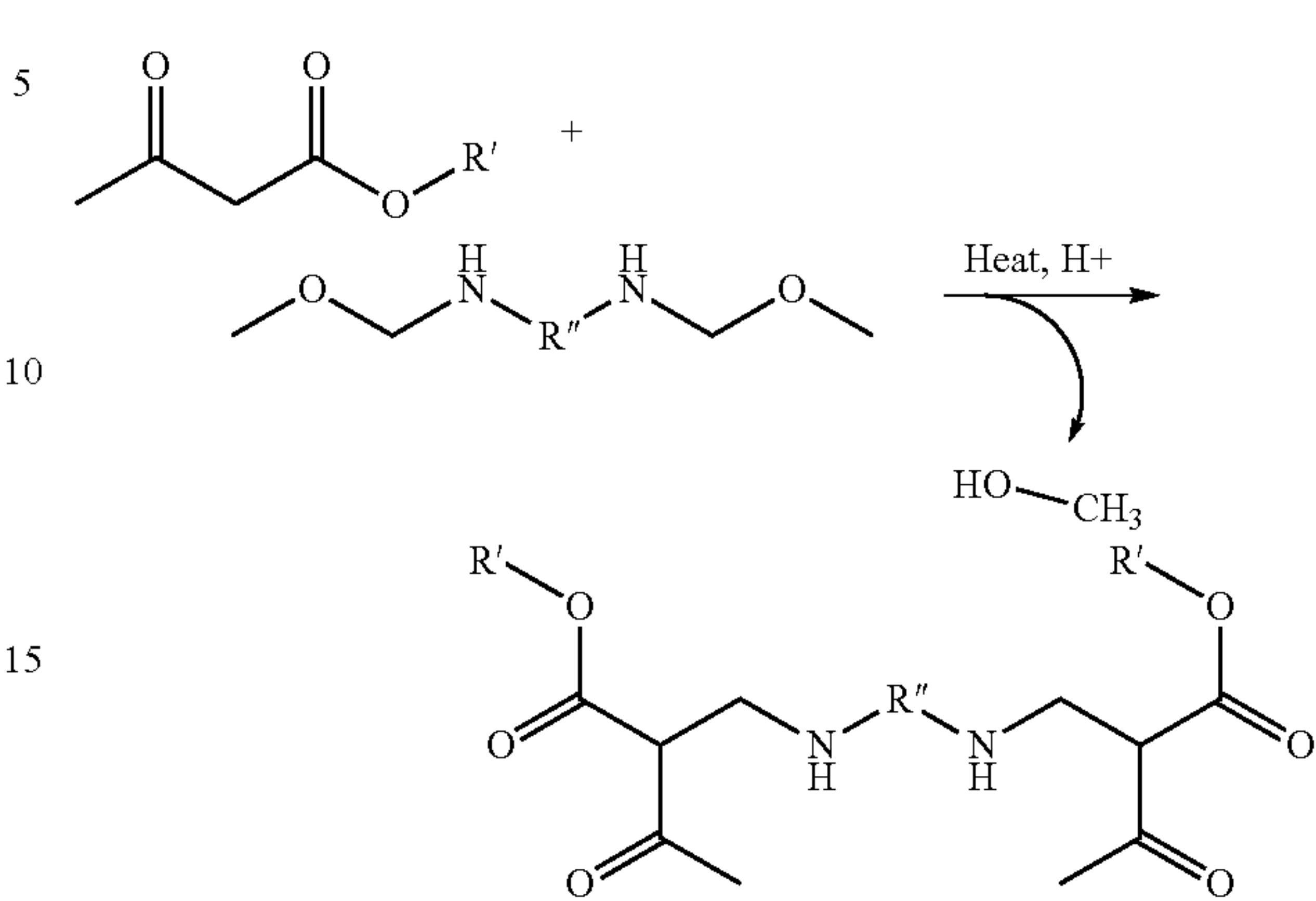
Reaction 5: crosslinking reaction between a melamine and acetoacetate functional groups.
