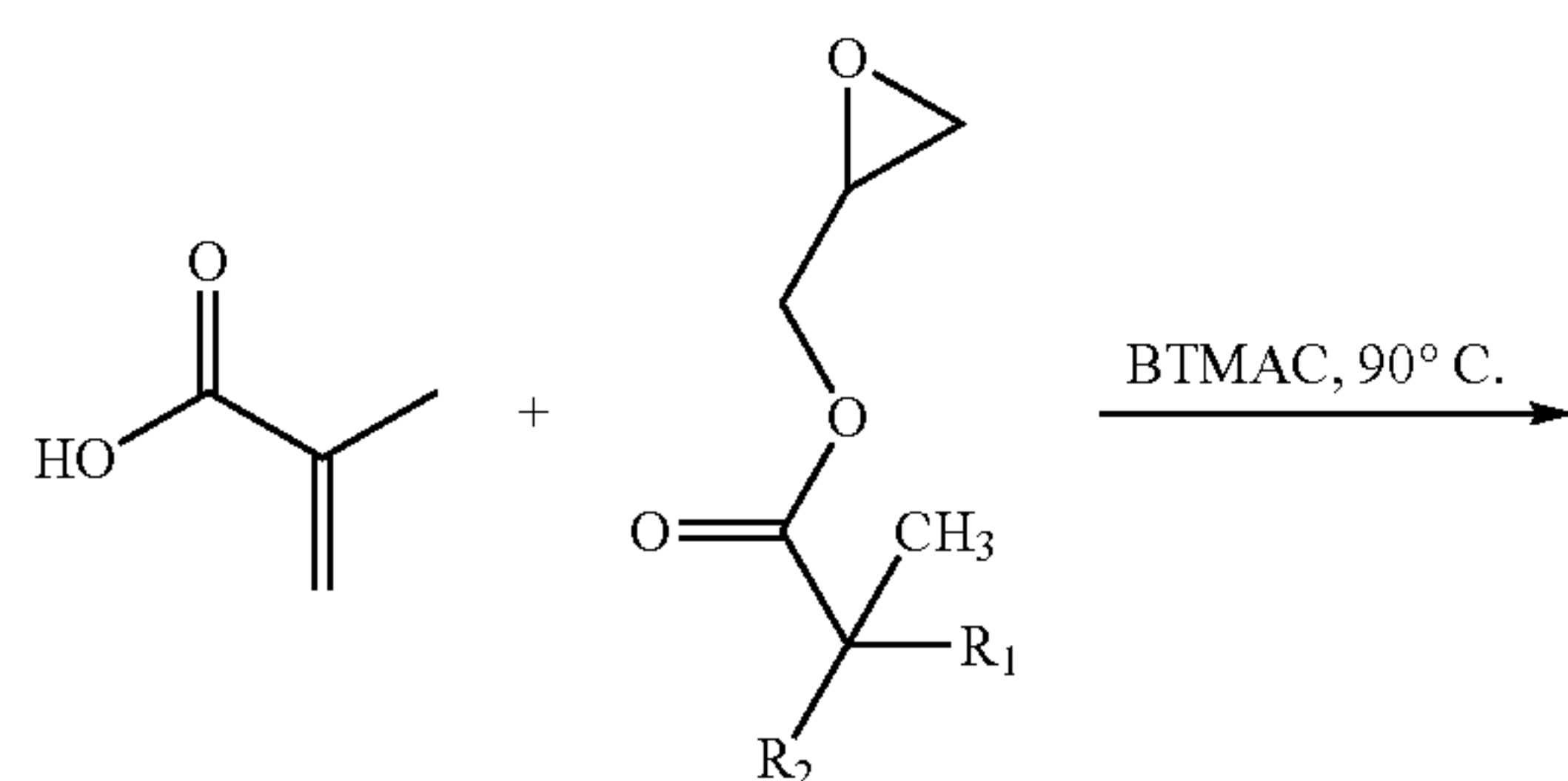
Scheme 10: Reaction of methacrylic acid with Cardura E-10P. R groups on Cardura molecule are, for example, alkyl chains.
