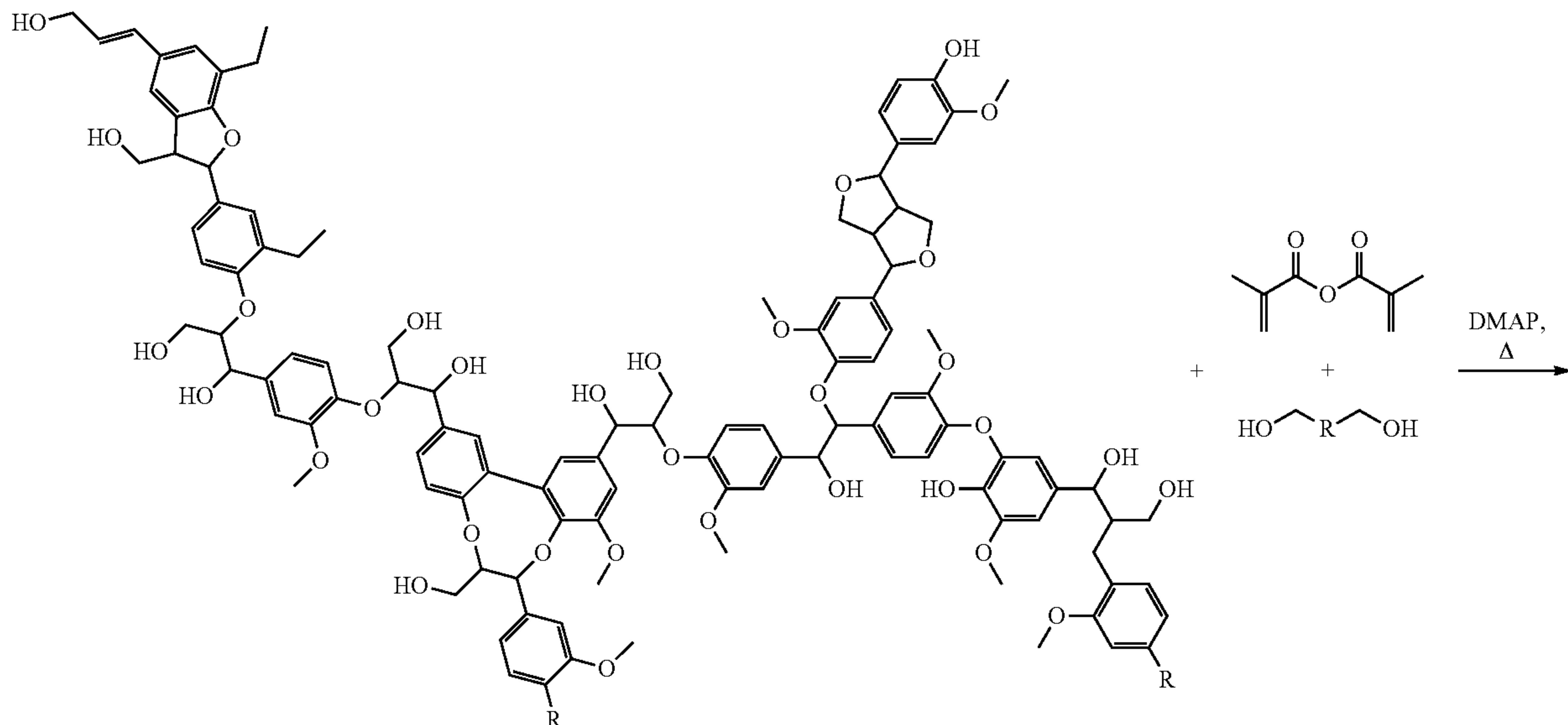
Scheme 9: Resin synthesis to create methacrylate functionalized Kraft Ligin resins.
