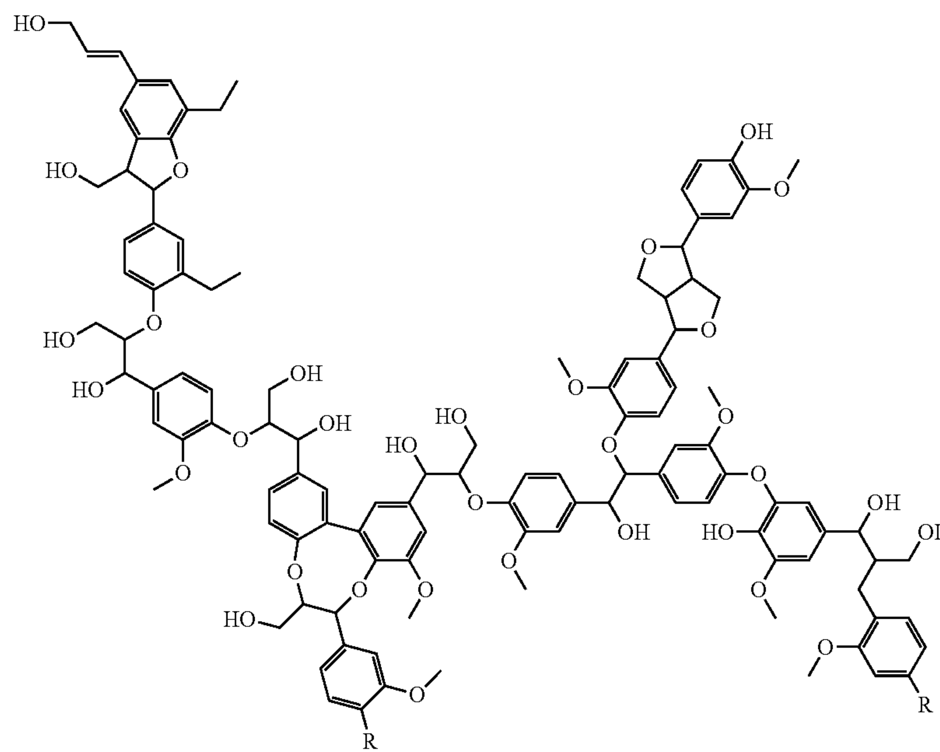
(A) Representative structure of Kraft Lignin.
