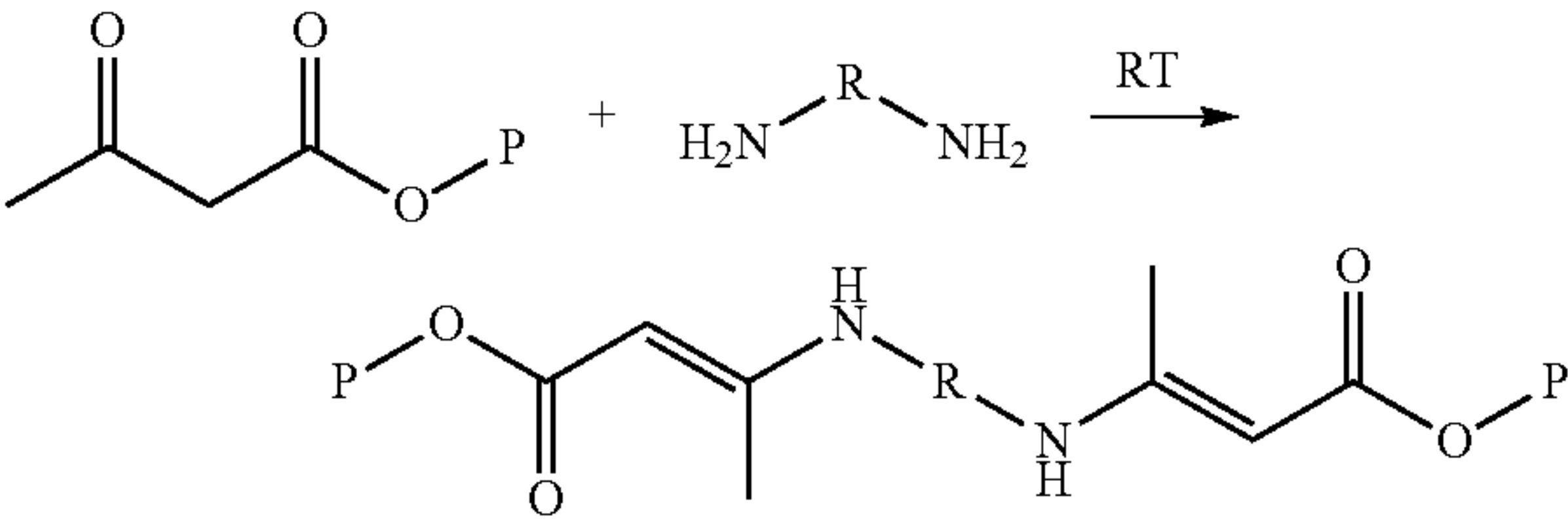
Reaction 6: crosslinking reaction between a diamine and acetoacetate functional groups.
