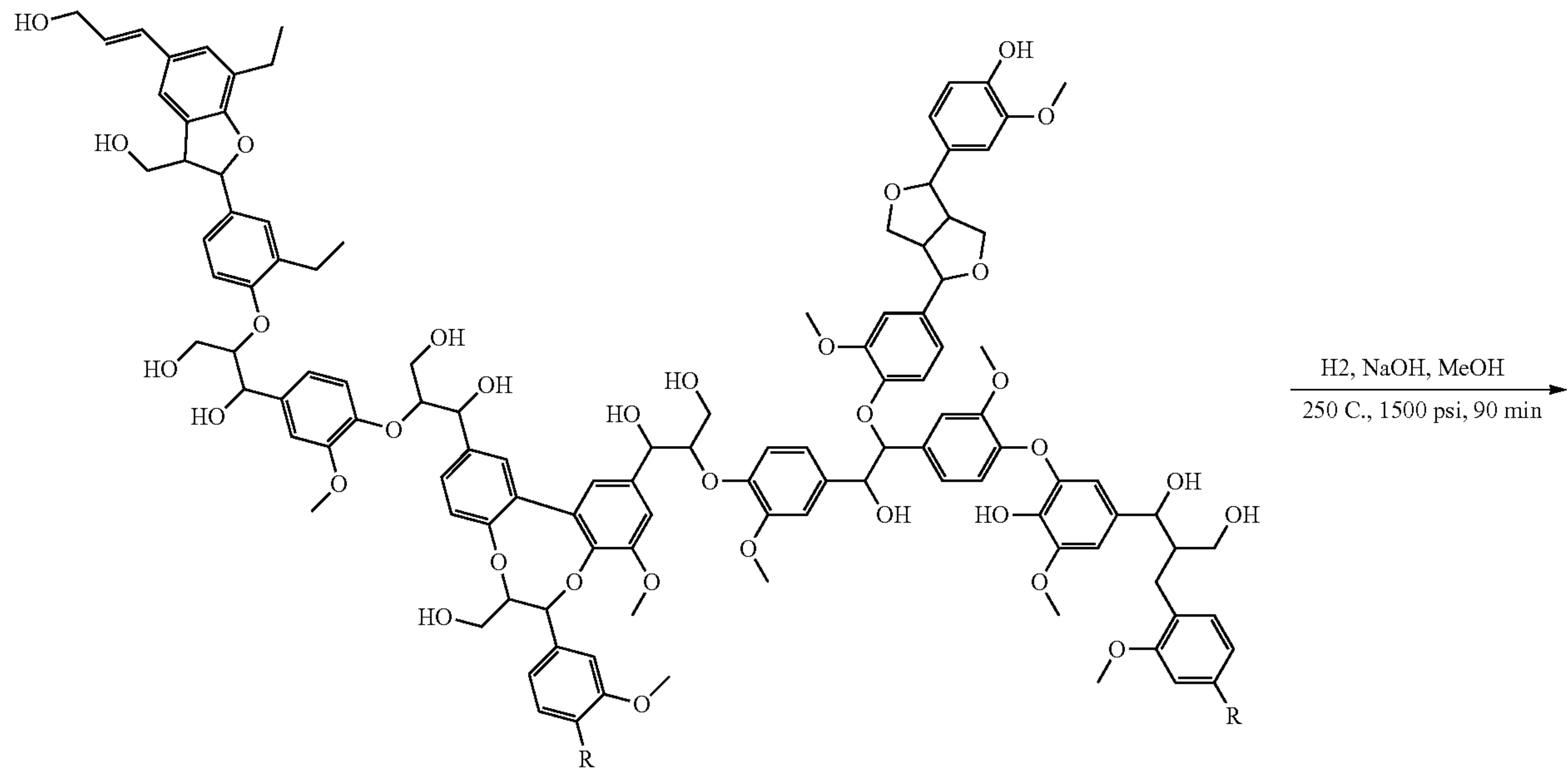
Scheme 11
