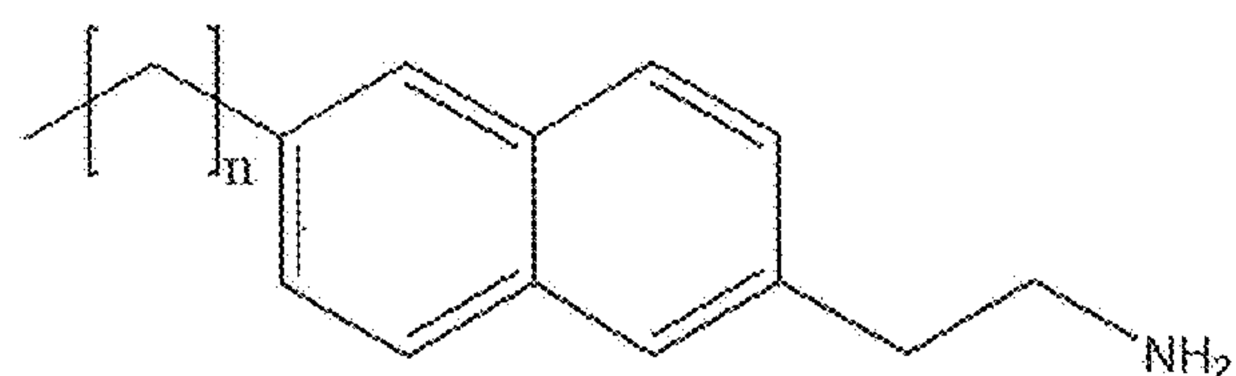
2-Ethylamine-7-alkyl-Naphthalene
