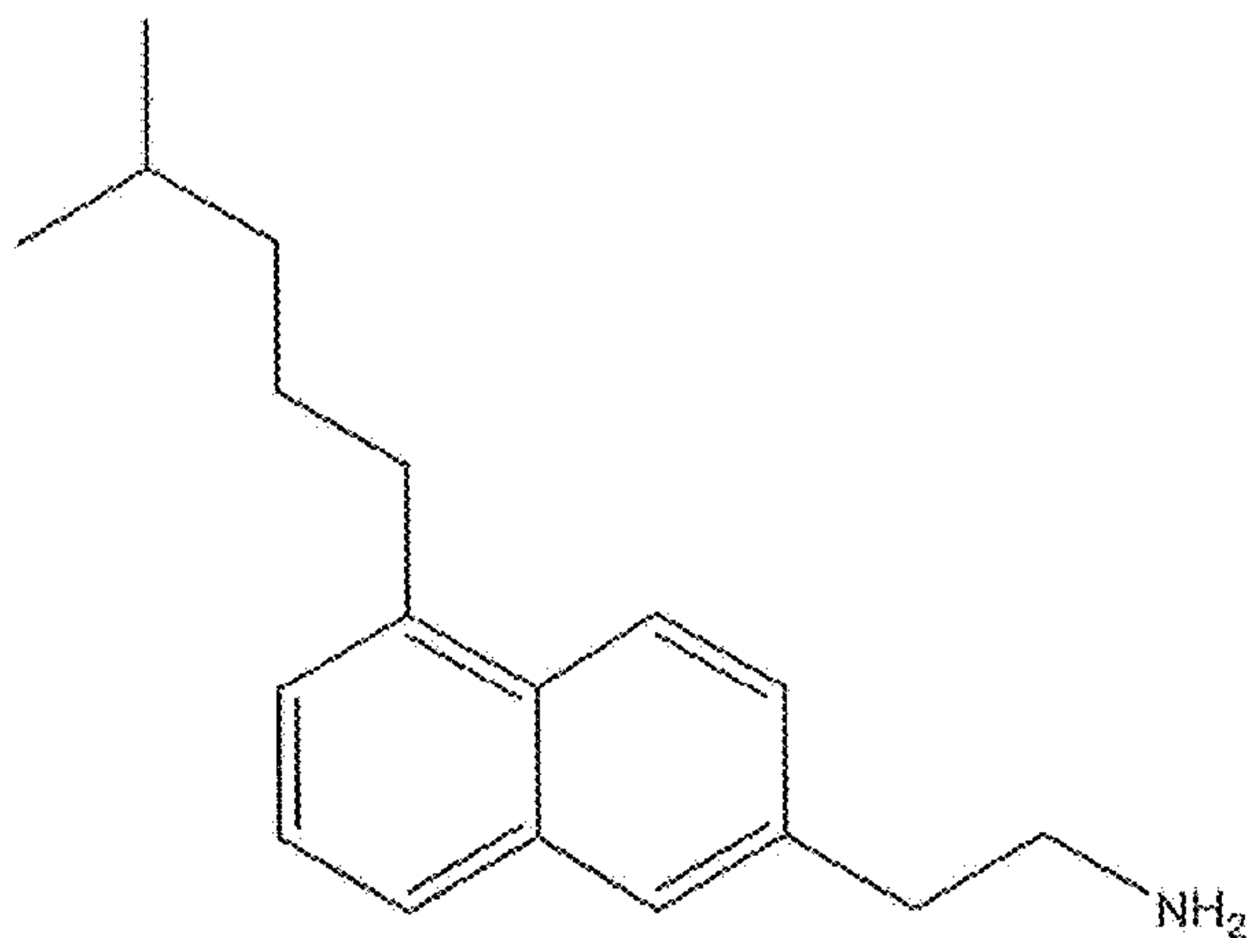
2-(5-[4-Methylpentyl]-2-naphthyl)ethanamine
