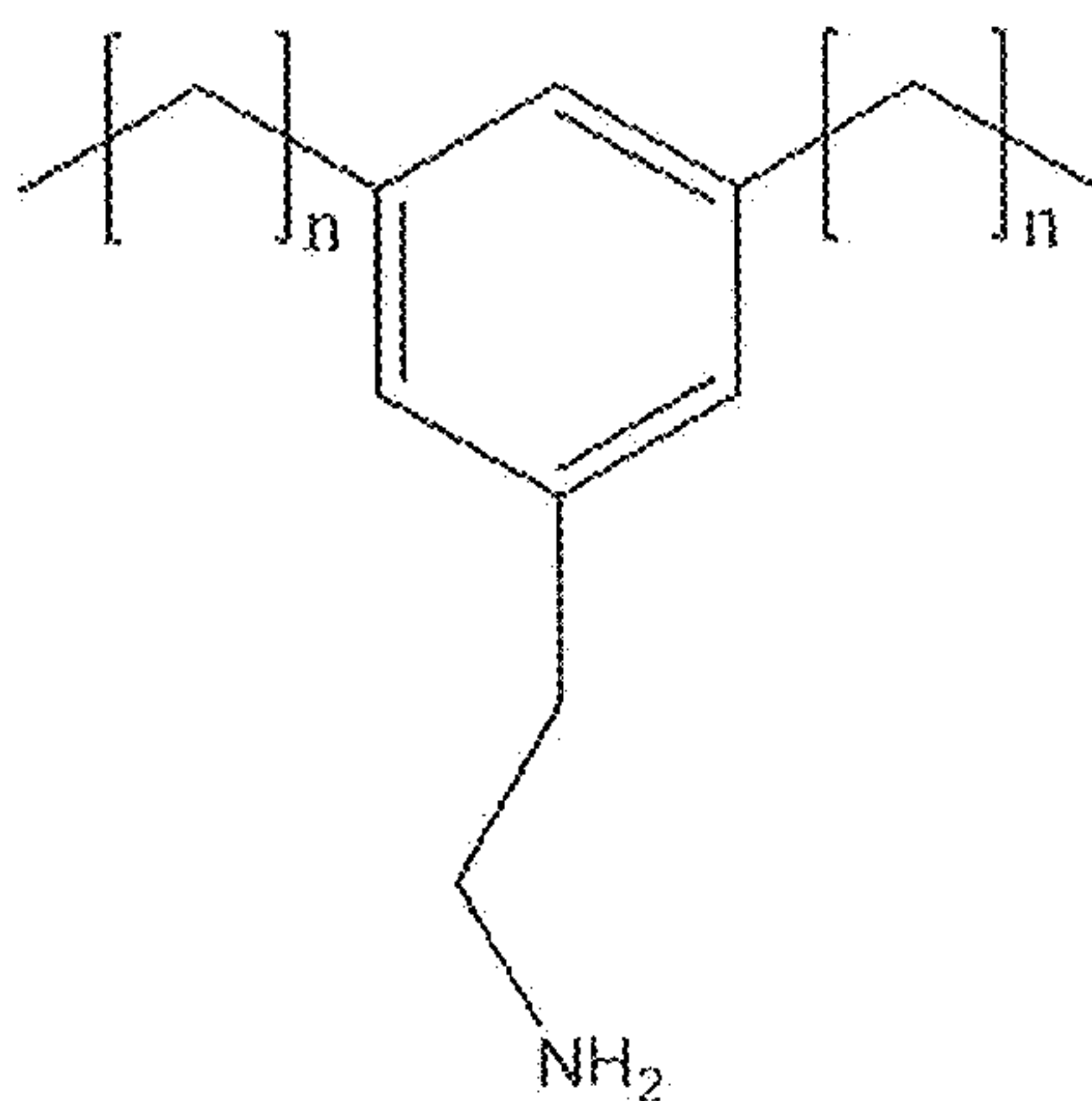
1-(3-alkyl-5-alkyl-2-phenyl)ethanamine
