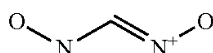
Hydroxy-[(hydroxyamino)methylene]ammonium
