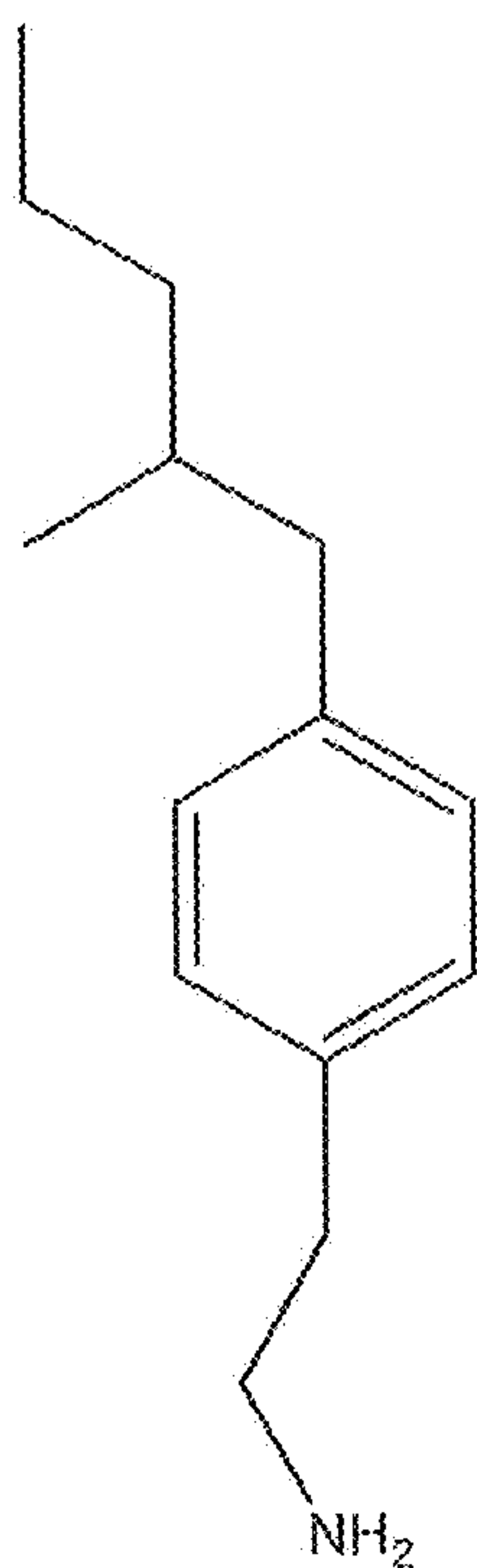
1-[4-(2-Methylpentyl)-2-phenyl]ethanamine
