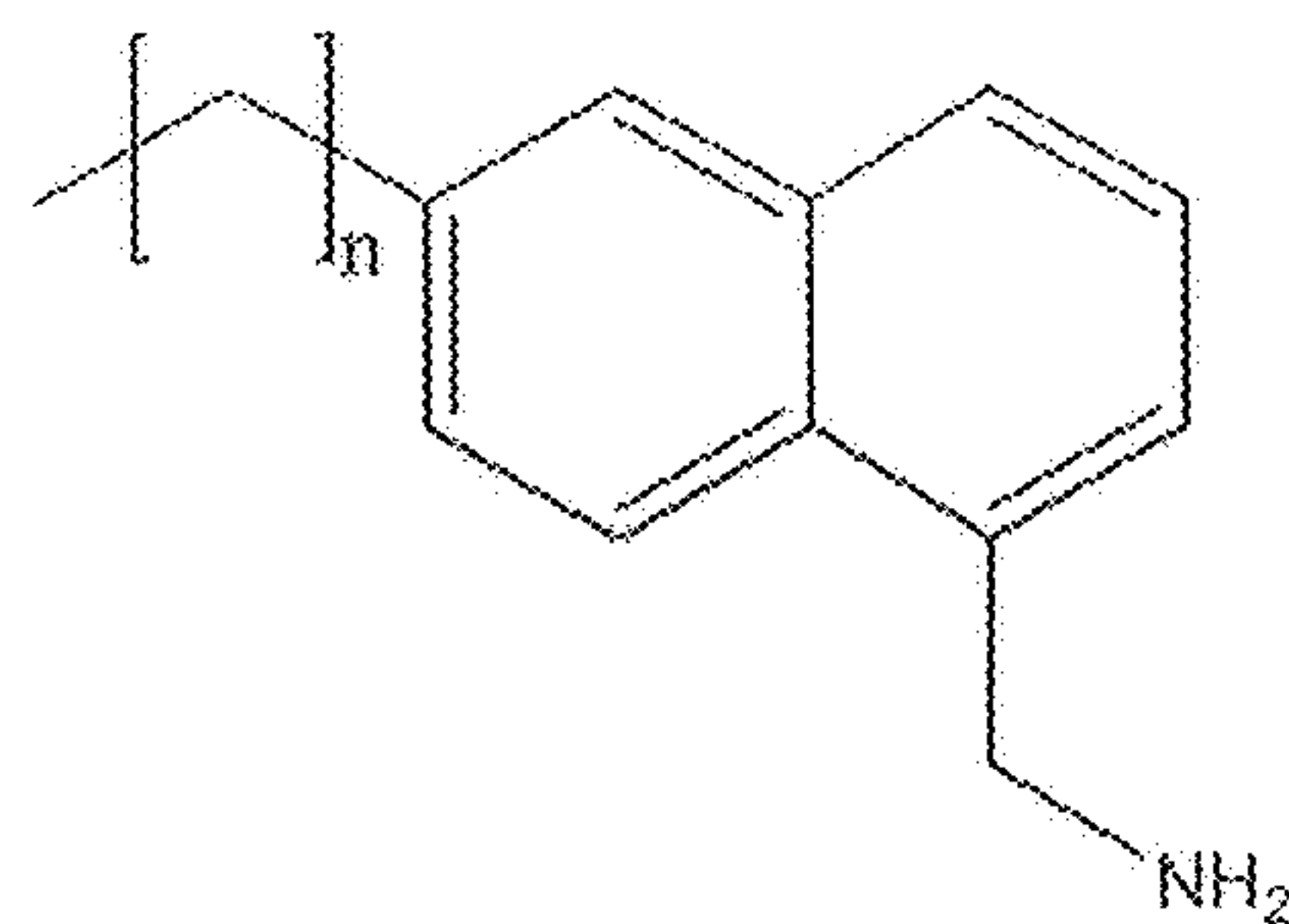
1-Methylamine-7-alkyl-Naphthalene
