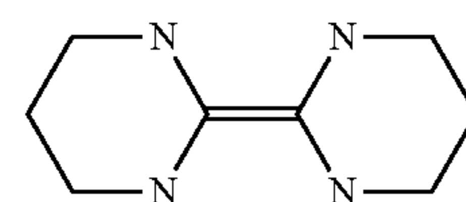
2-hexahydropyrimidin-2-ylidenehexahydropyrimidine
