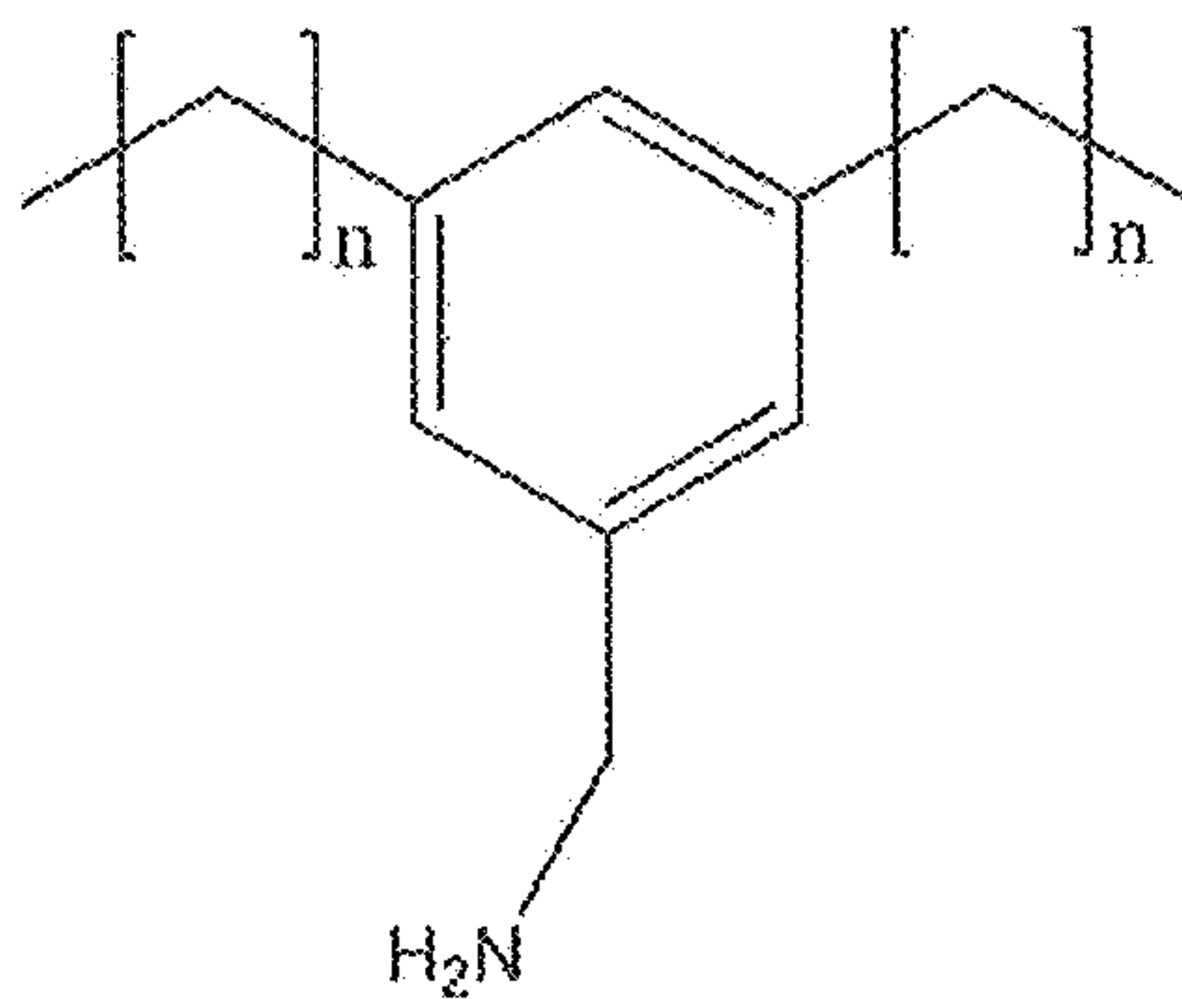
1-(3-alkyl-5-alkylphenyl)methanamine
