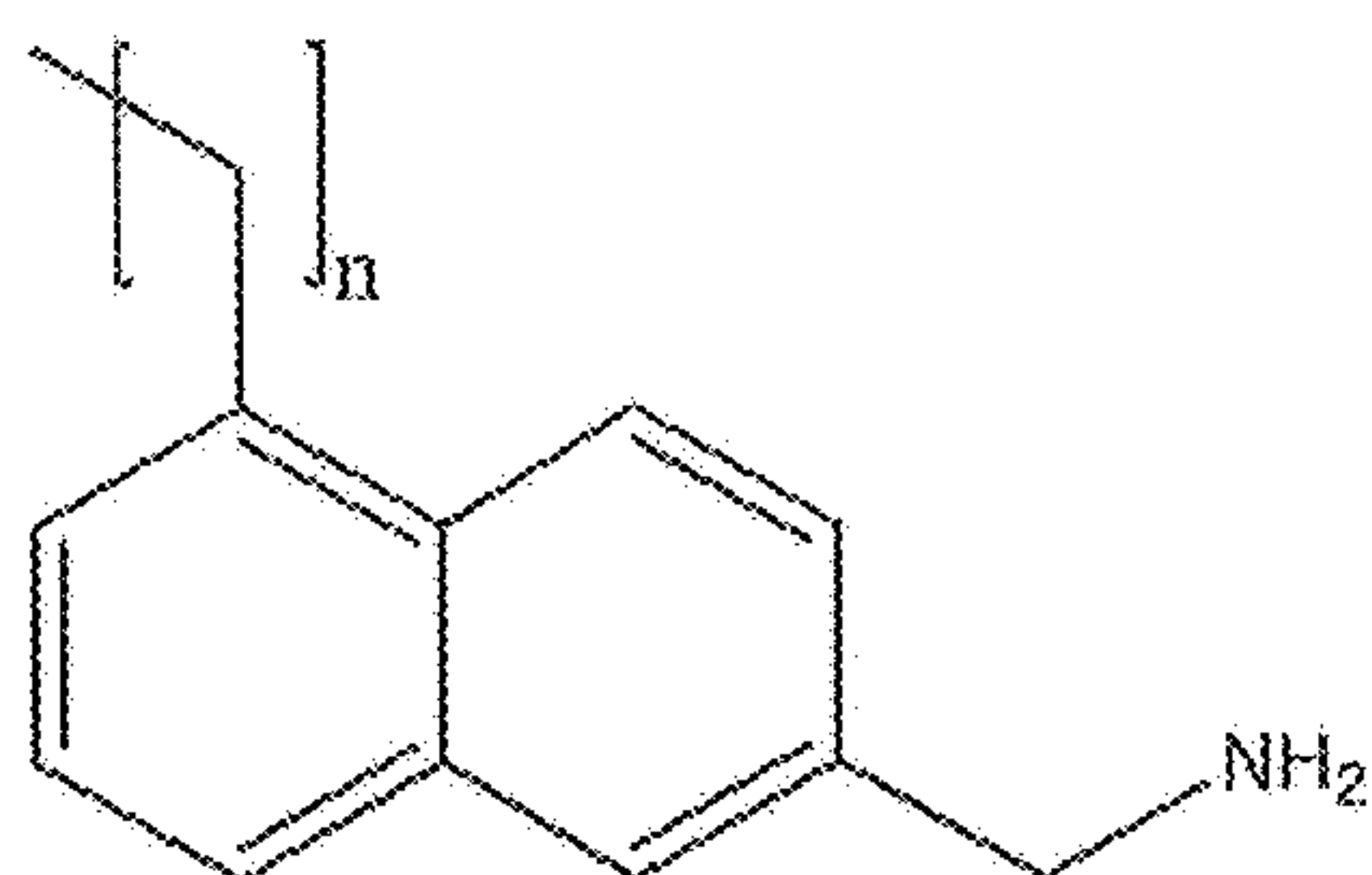
2-Methylamine-6-alkyl-Naphthalene
