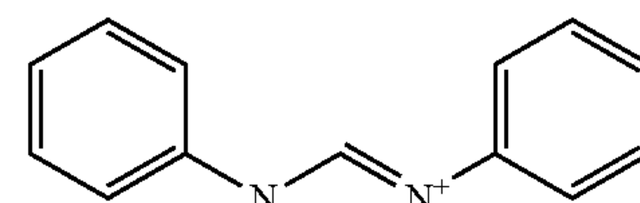
Anilinomethylene(phenyl)ammonium
