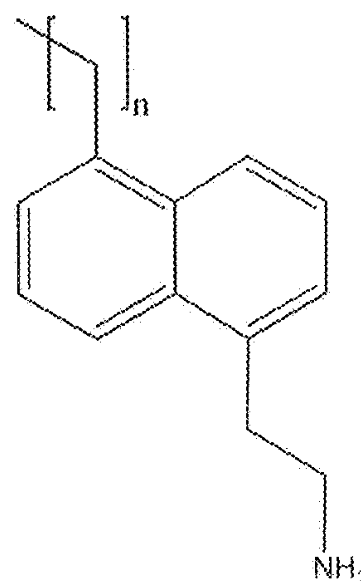
1-Ethylamine-6-alkyl-Naphthalene
