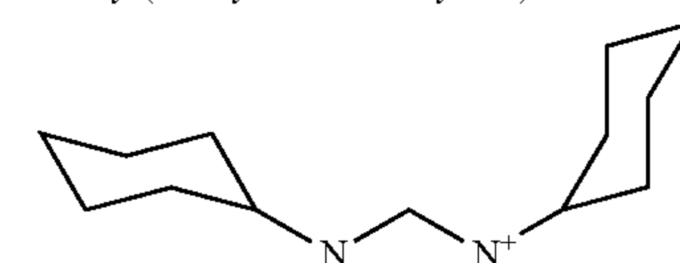
Cyclohexyl-[(cyclohexylamino)methylene]ammonium
