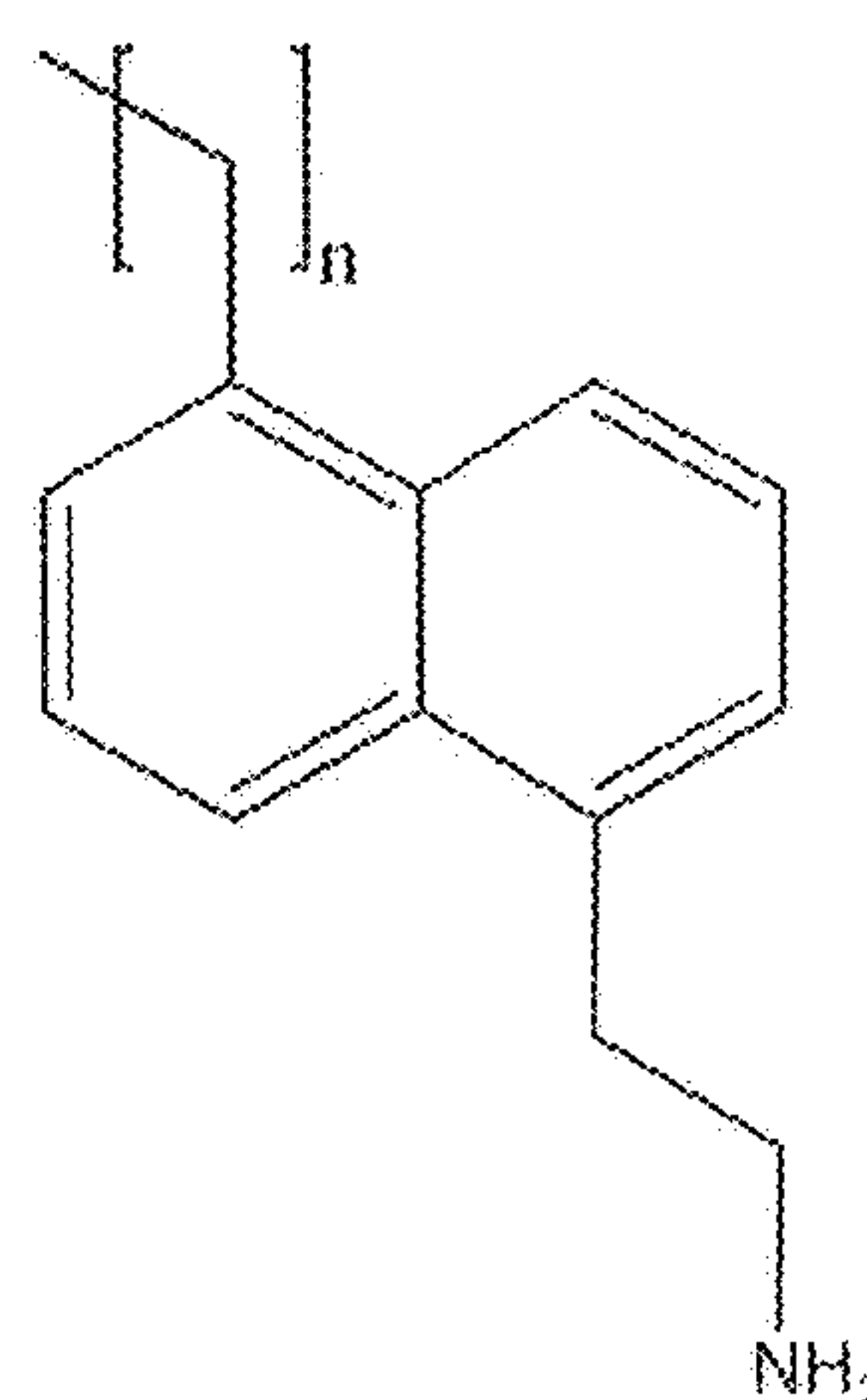
1-Ethylamine-6-alkyl-Naphthalene
