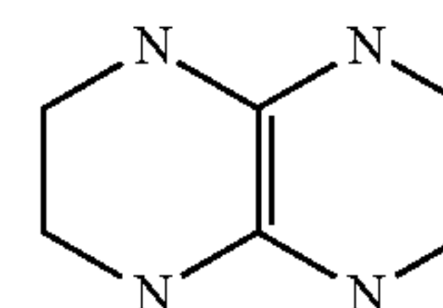
1,2,3,4,5,6,7,8-octahydropyrazino[2,3-b]pyrazine
