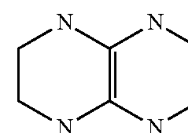
1,2,3,4,5,6,7,8-octahydropyrazino[2,3-b]pyrazine
