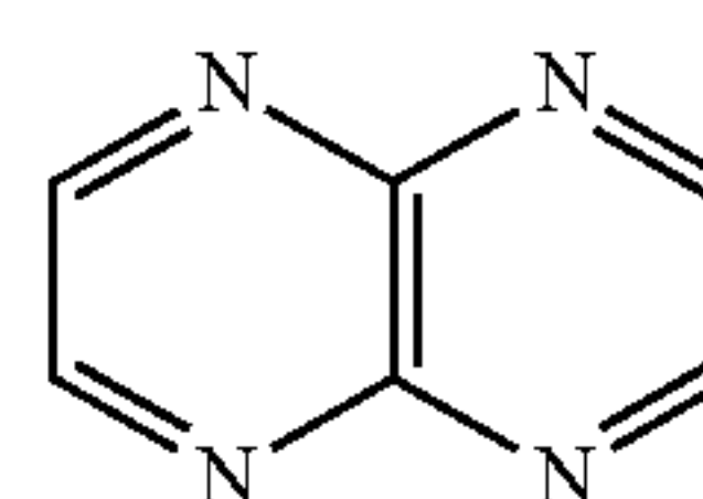
pyrazino[2,3-b]pyrazine
