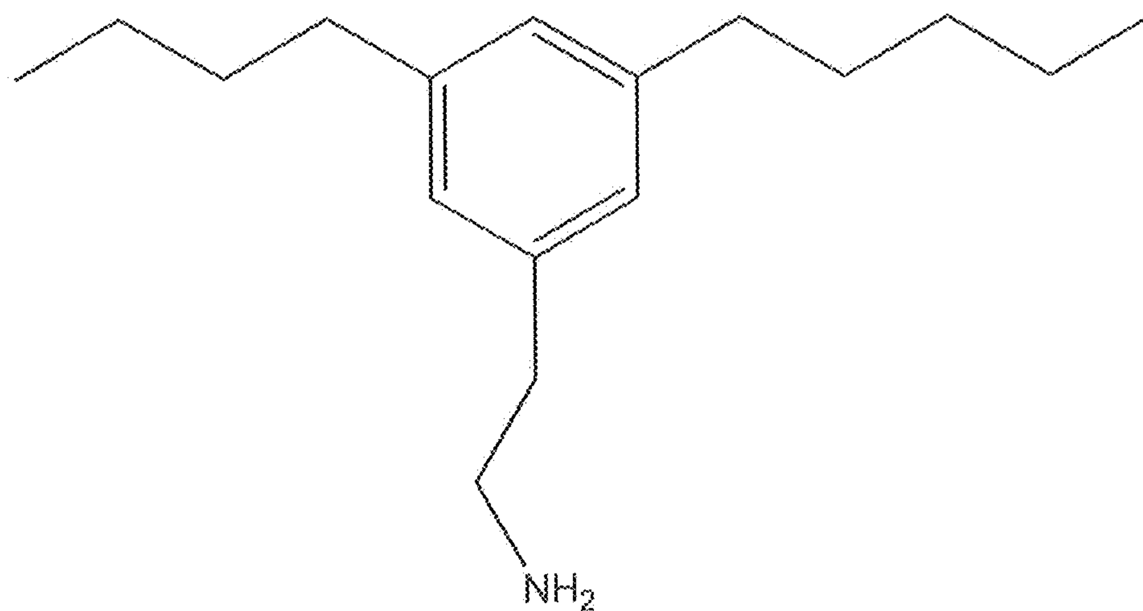
1-(3-Butyl-5-pentyl-2-phenyl)ethanamine
