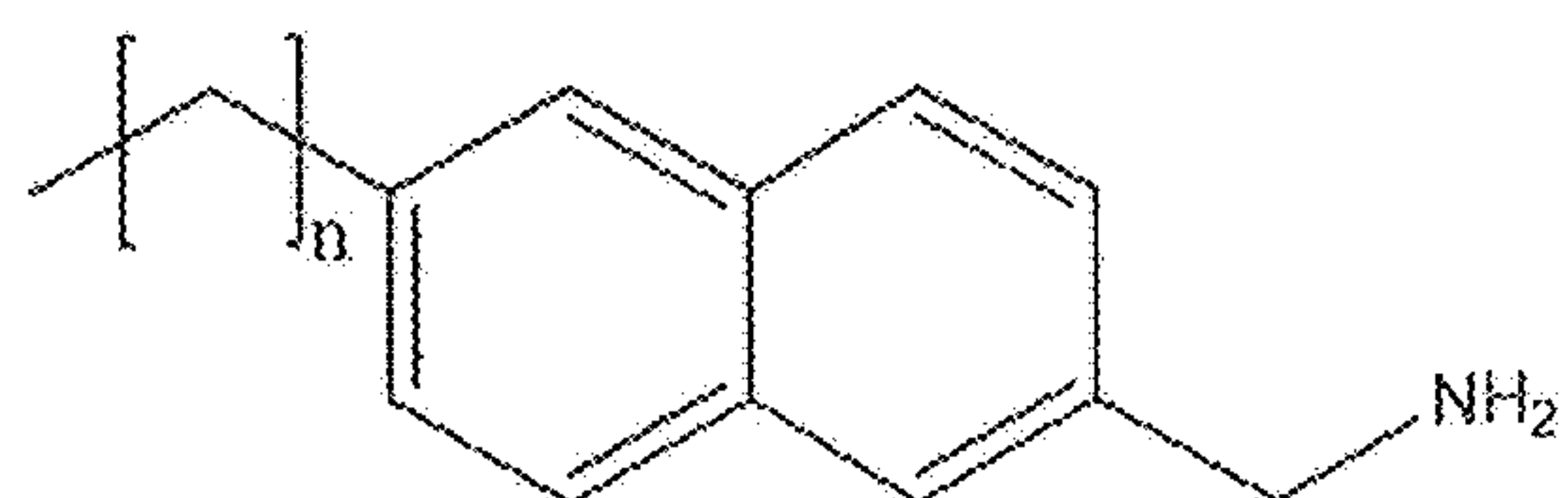
2-Methylamine-7-alkyl-Naphthalene
