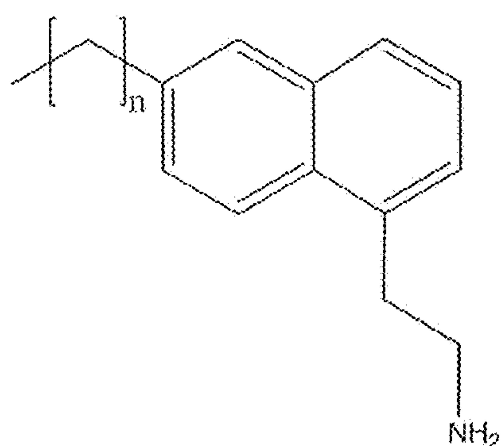
1-Ethylamine-7-alkyl-Naphthalene
