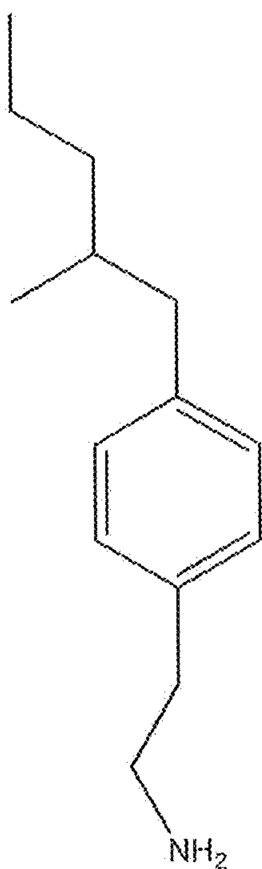
1-[4-(2-Methylpentyl)-2-phenyl]ethanamine
