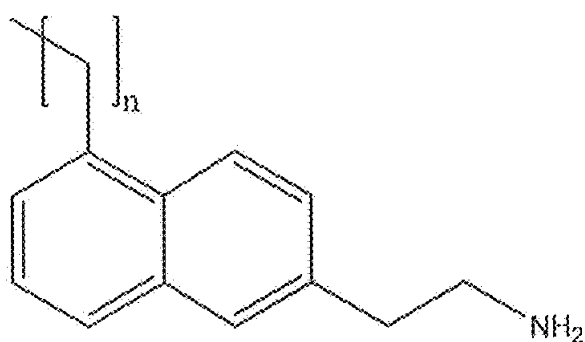
2-Ethylamine-6-alkyl-Naphthalene
