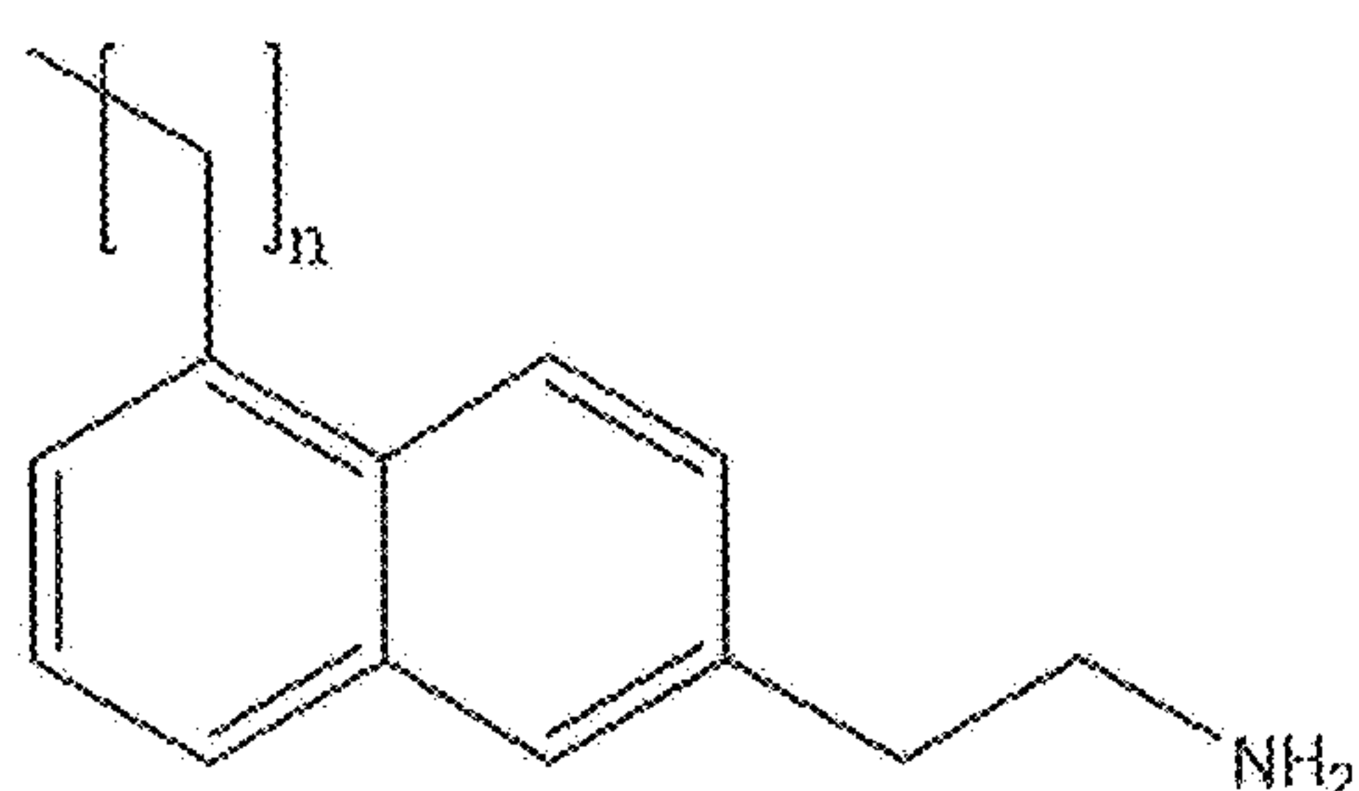
2-Ethylamine-6-alkyl-Naphthalene
