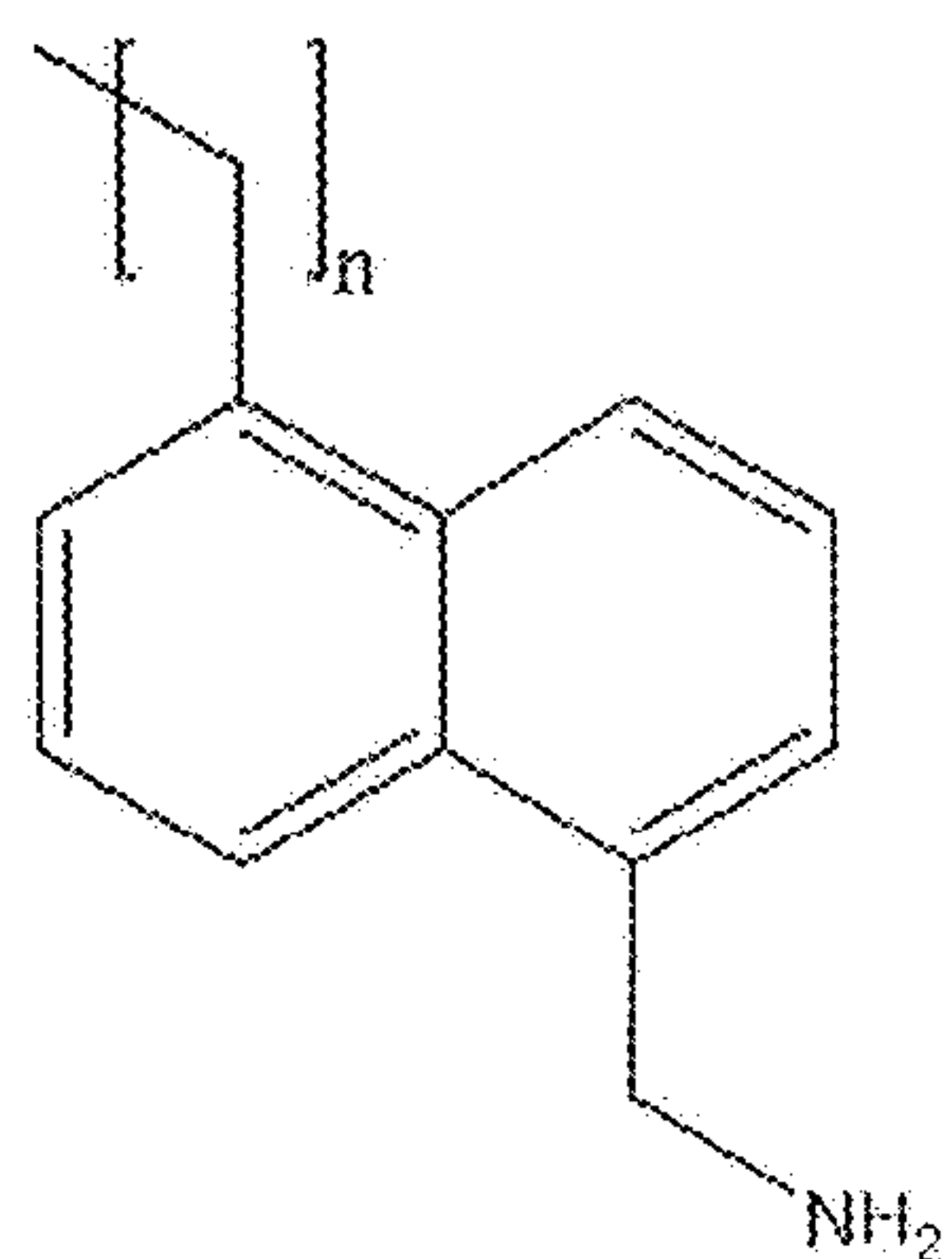
1-Methylamine-6-alkyl-Naphthalene
