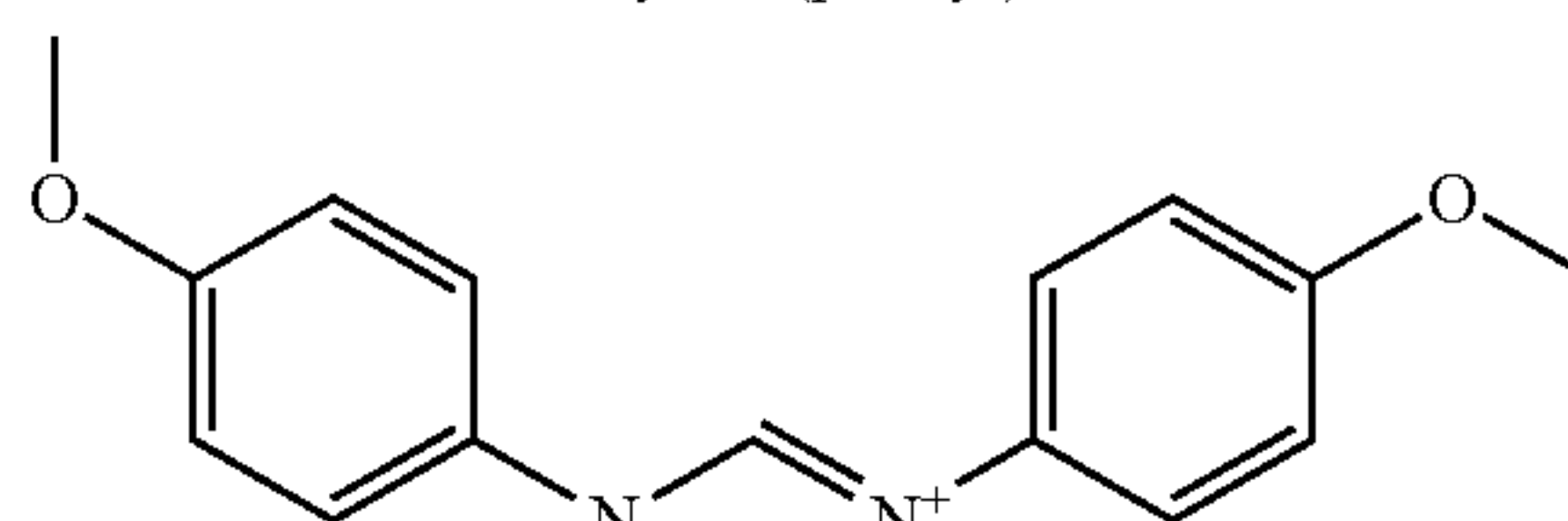
(Methoxyanilino)methylene-(4-methoxyphenyl)ammonium
