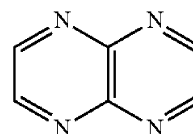
pyrazino[2,3-b]pyrazine
