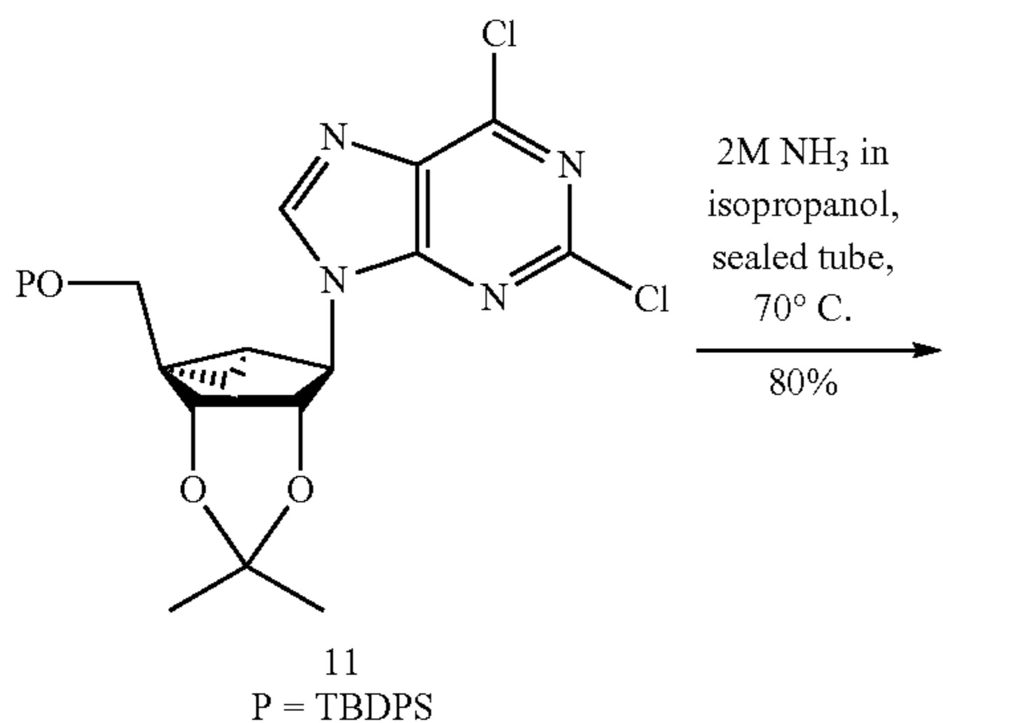
Scheme 2: Synthesis of MRS4322
