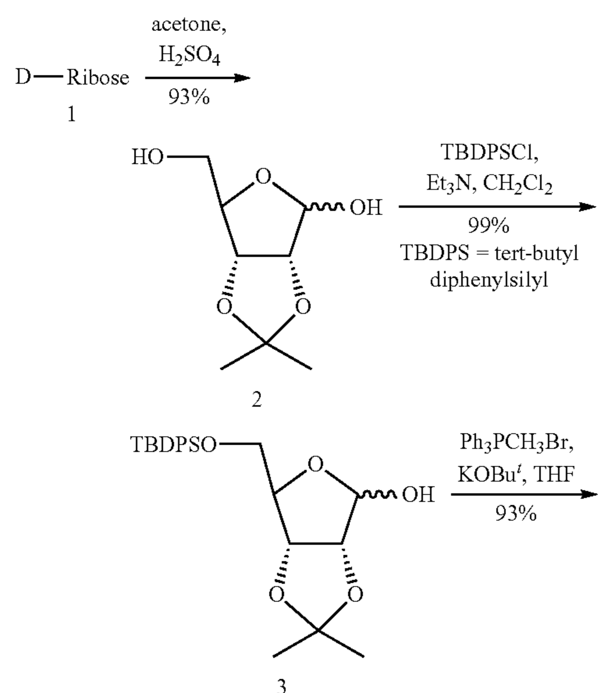
Scheme 1: Synthesis of MRS4322
