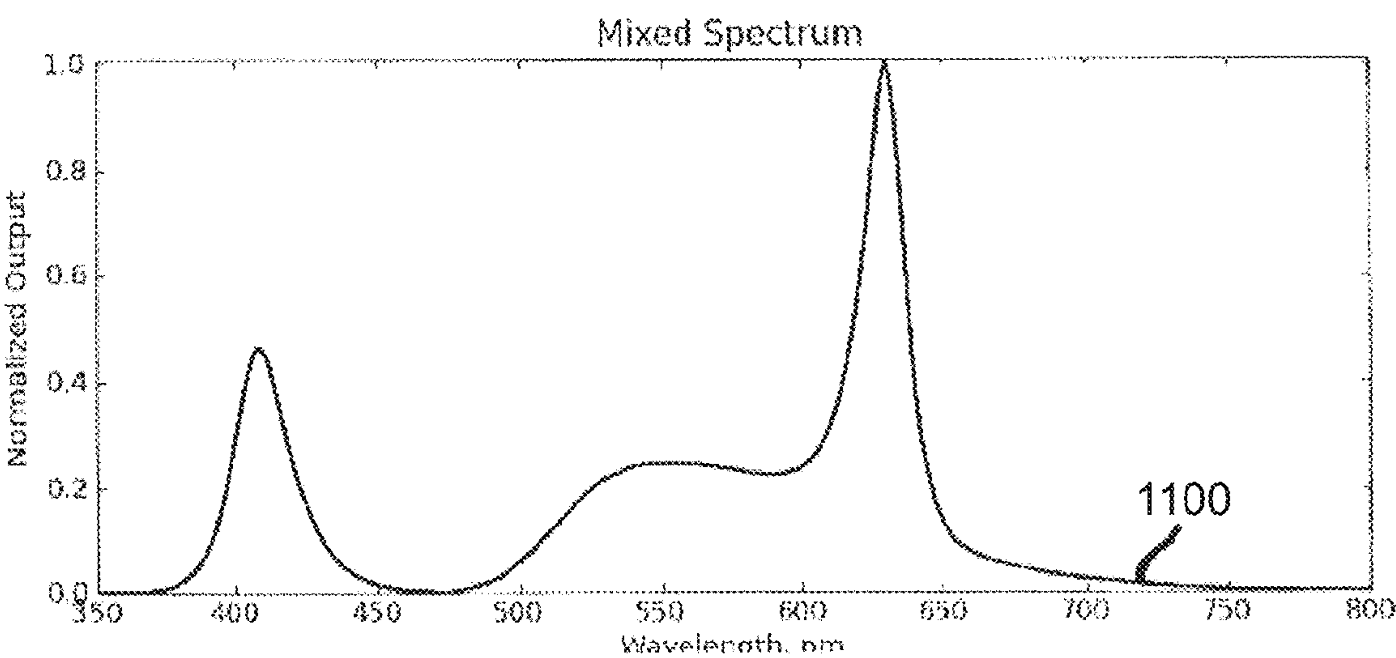
2400K Ch2: Normalized Output vs. Wavelength (nm)
