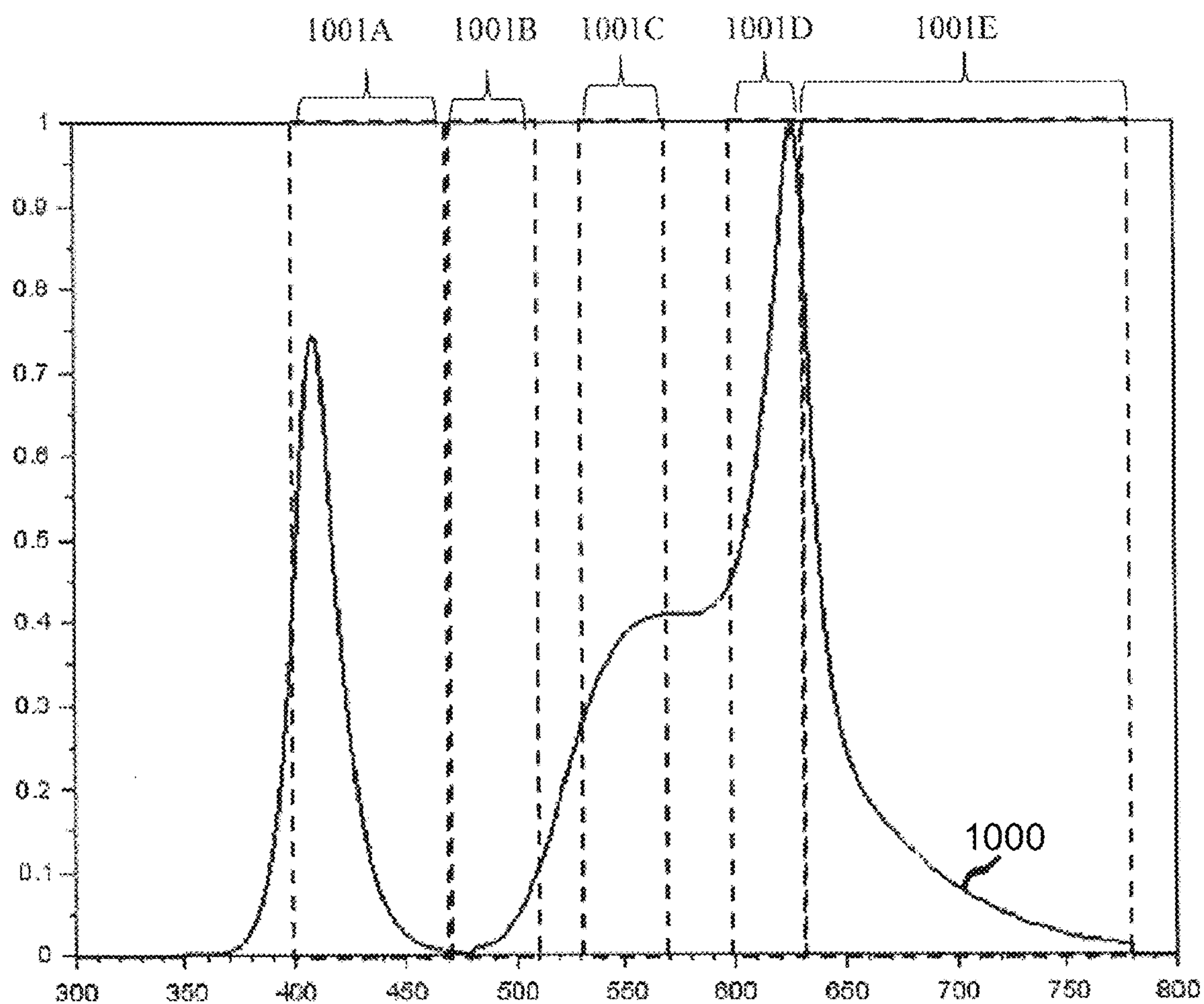
2400K Ch3: Normalized Output vs. Wavelength (nm)
