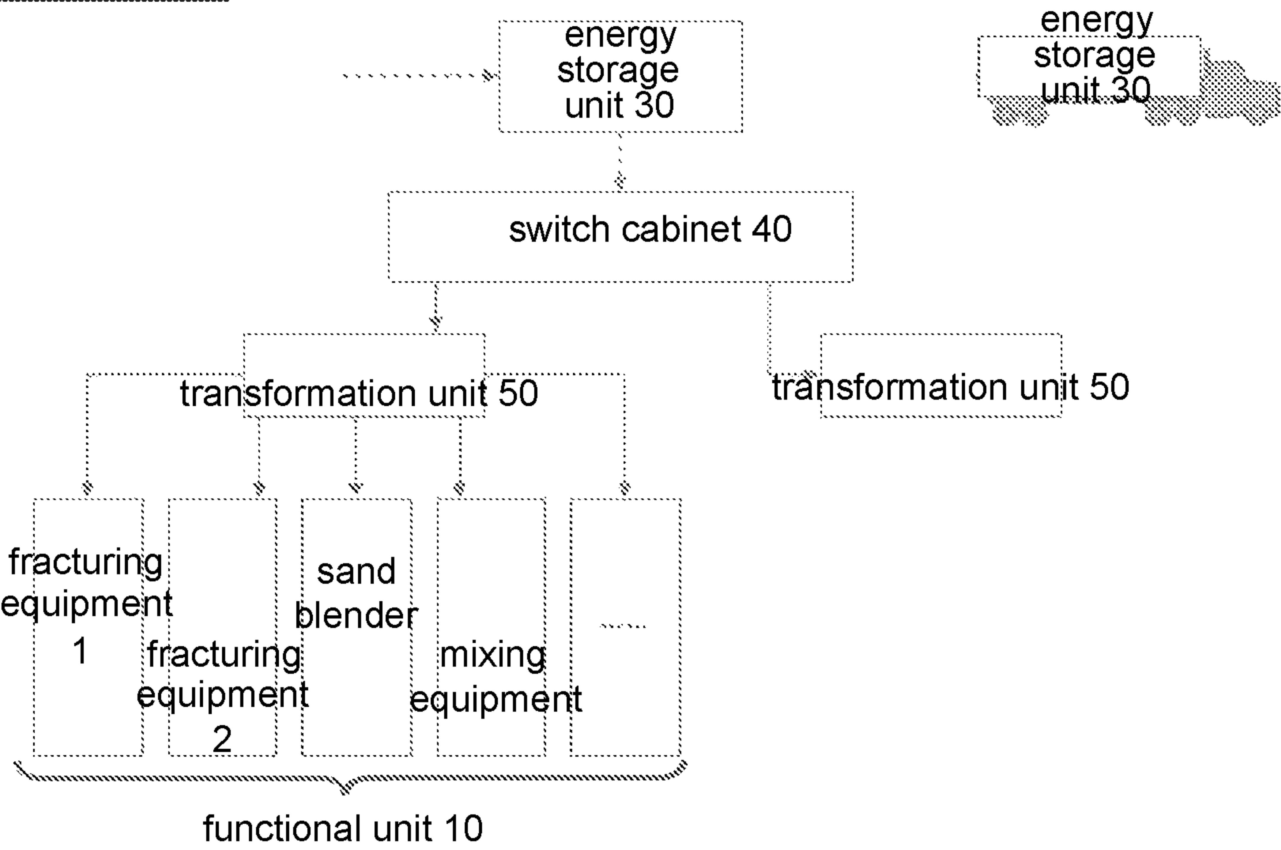
fracturing system 400
