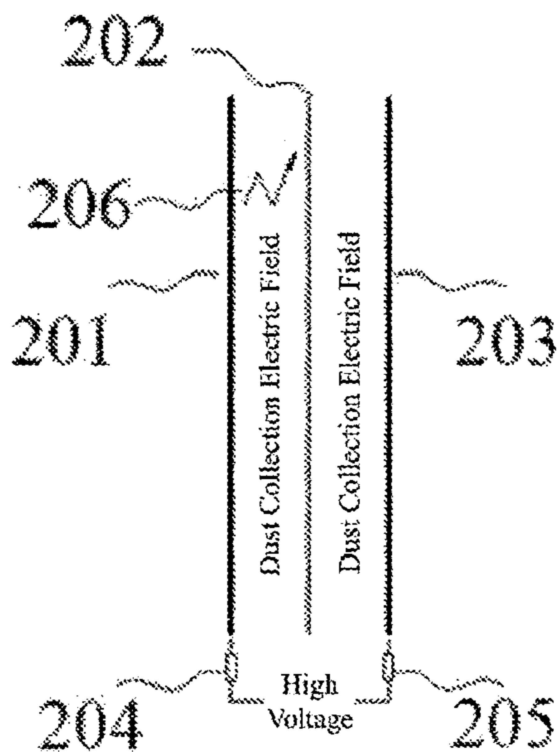
FIG. 2 (PRIOR ART)
