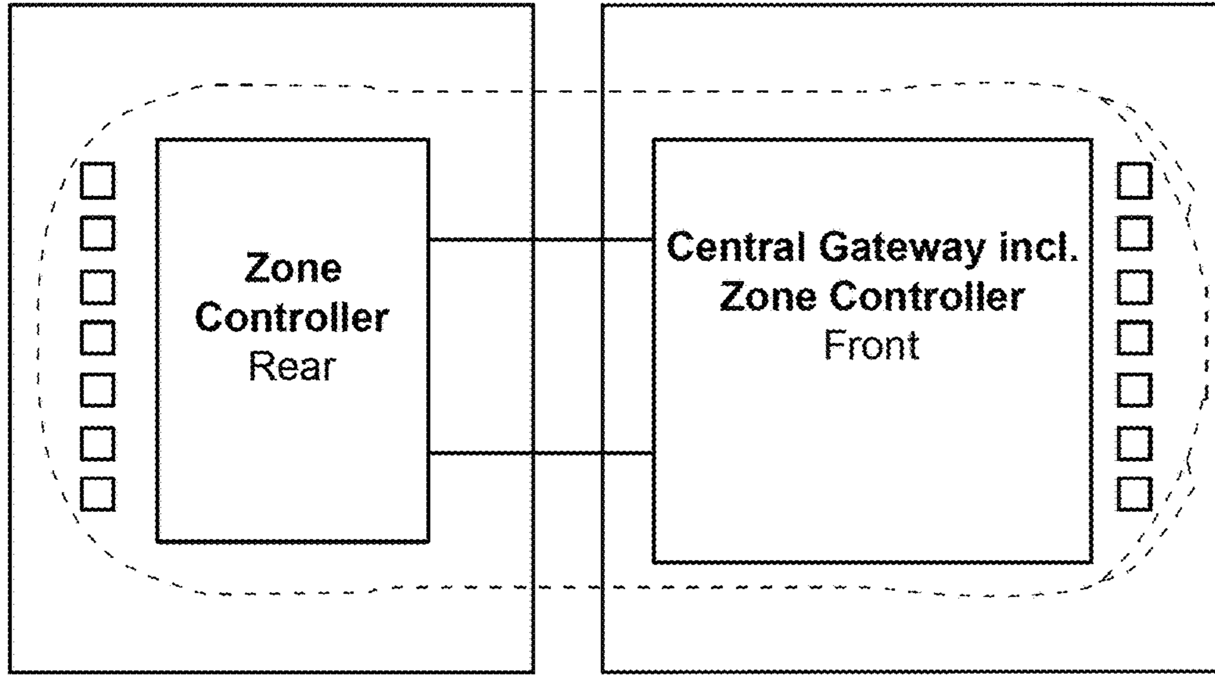
2 - Node Topology
