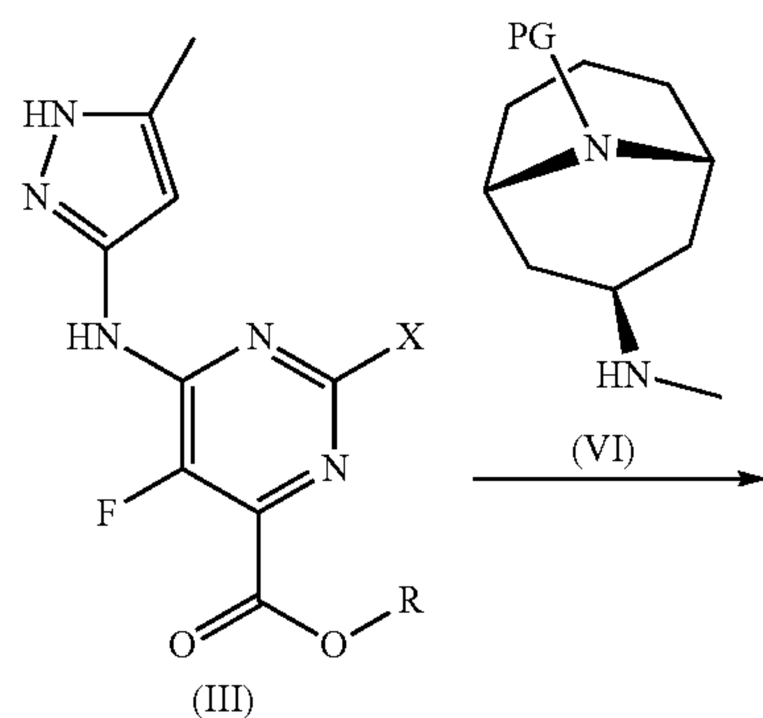
Scheme 2
