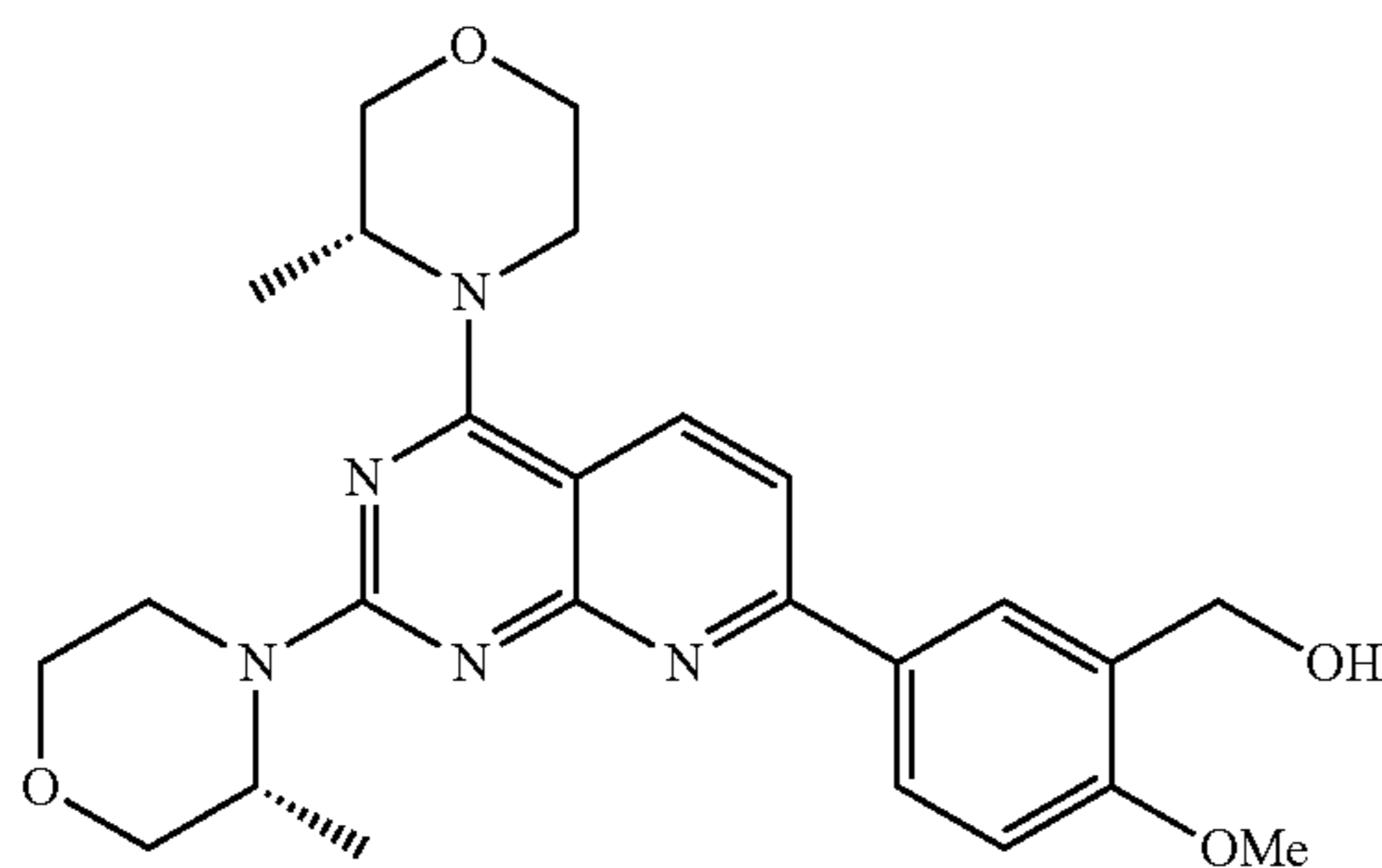
AZD8055
