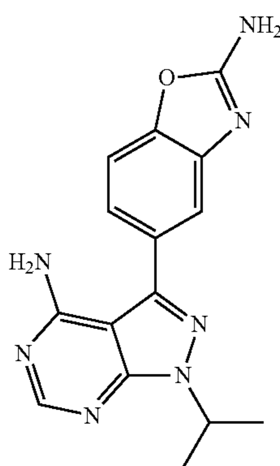
INK128
