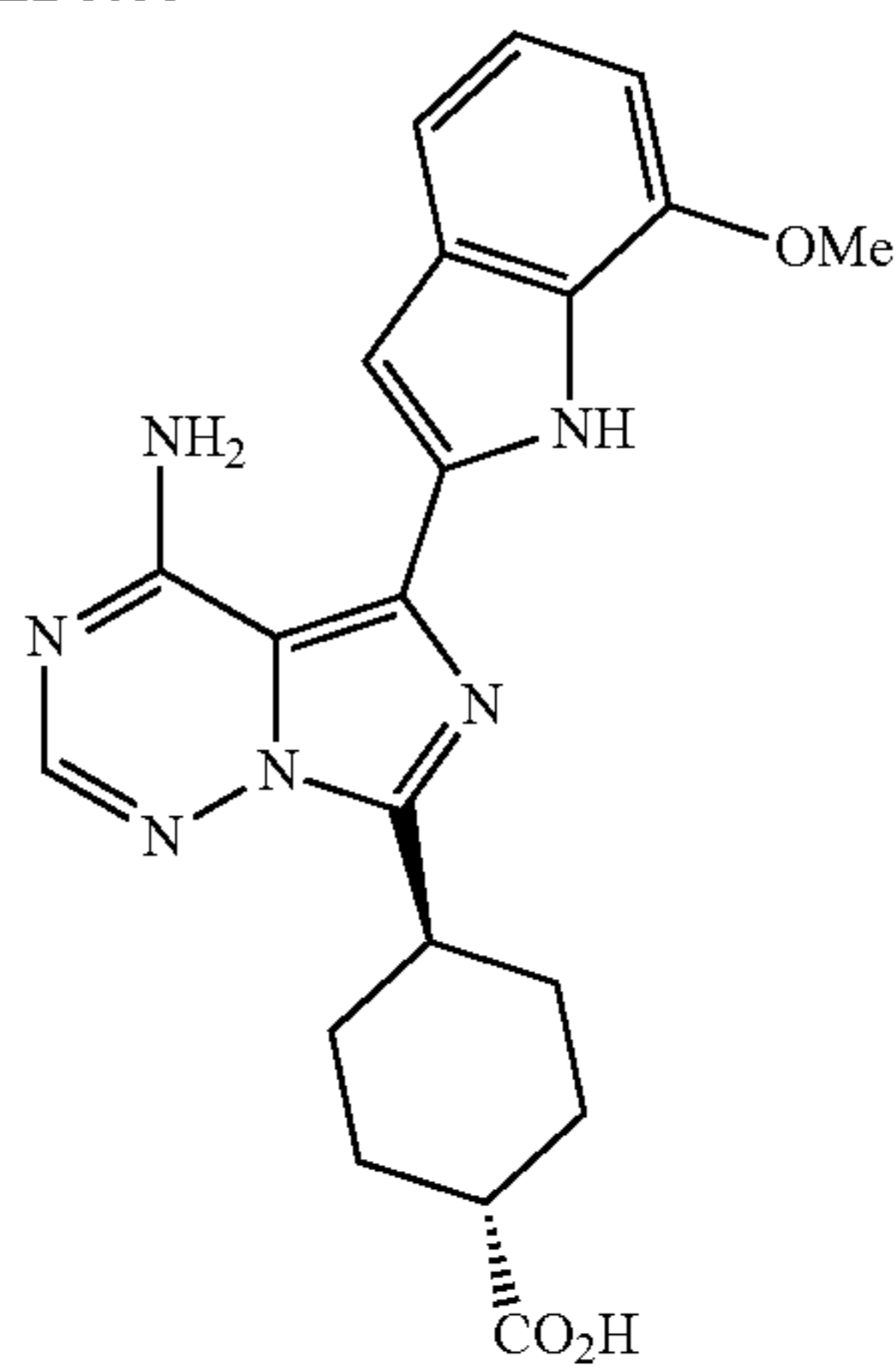
OSI-027
