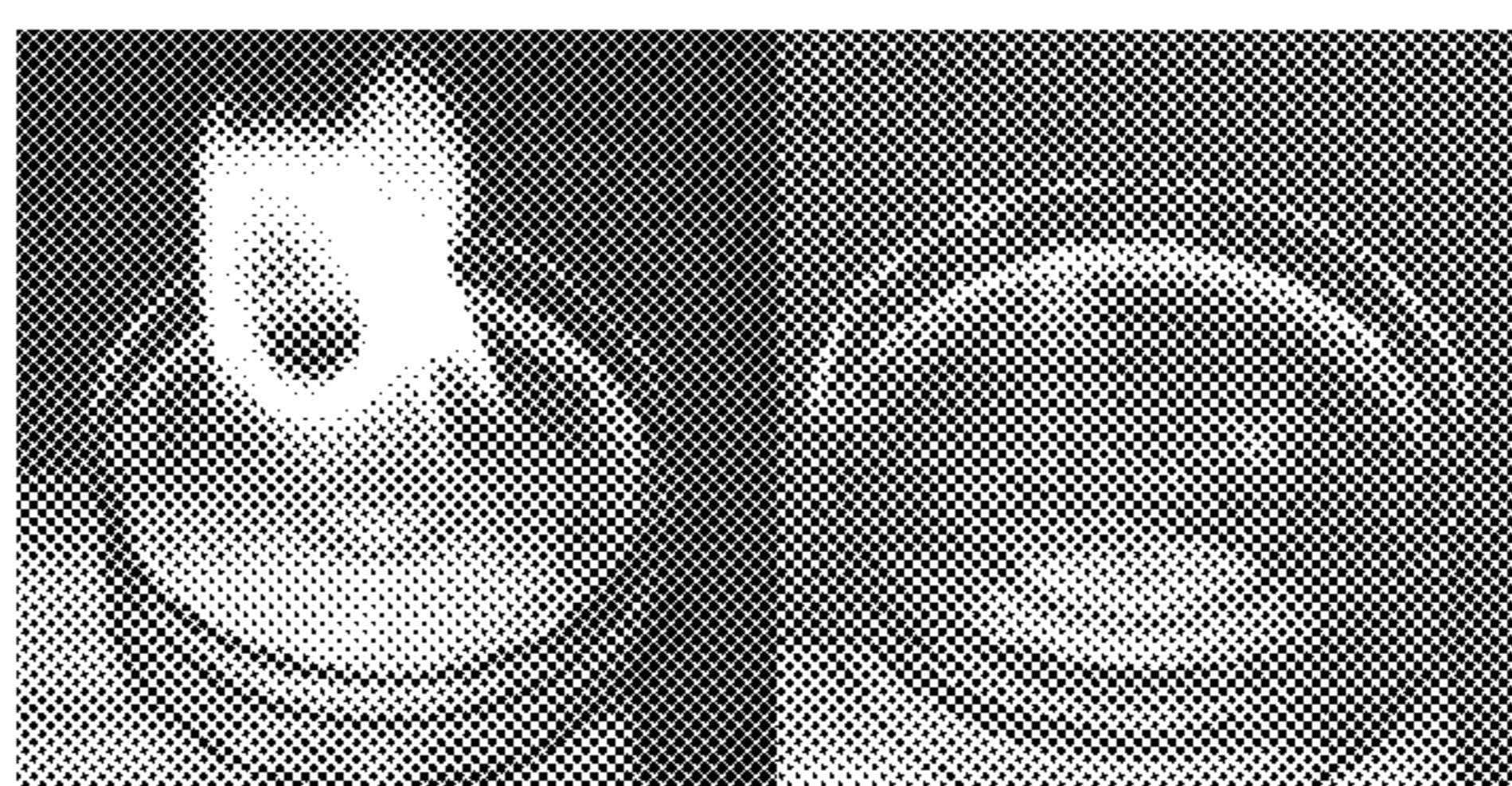
LiTFSI/DME+DOL (1:1) = 0.077 LiTFSI/DME+DOL (1:1) = 0.23
