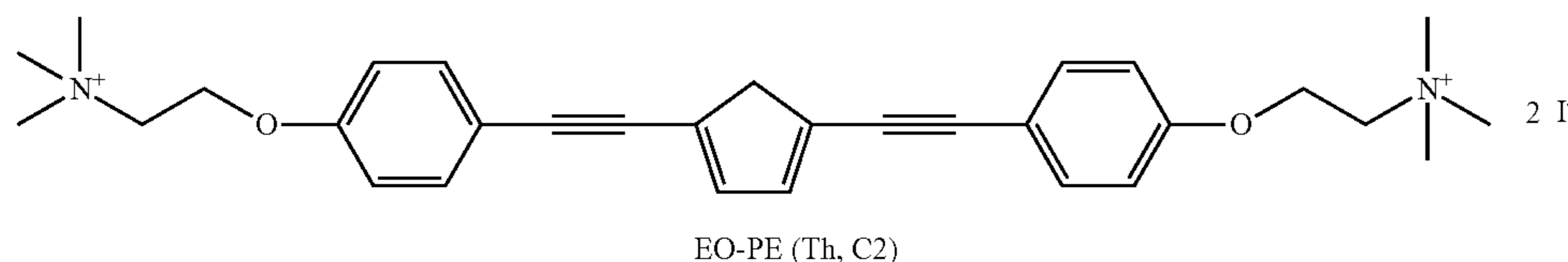
Scheme 1.
