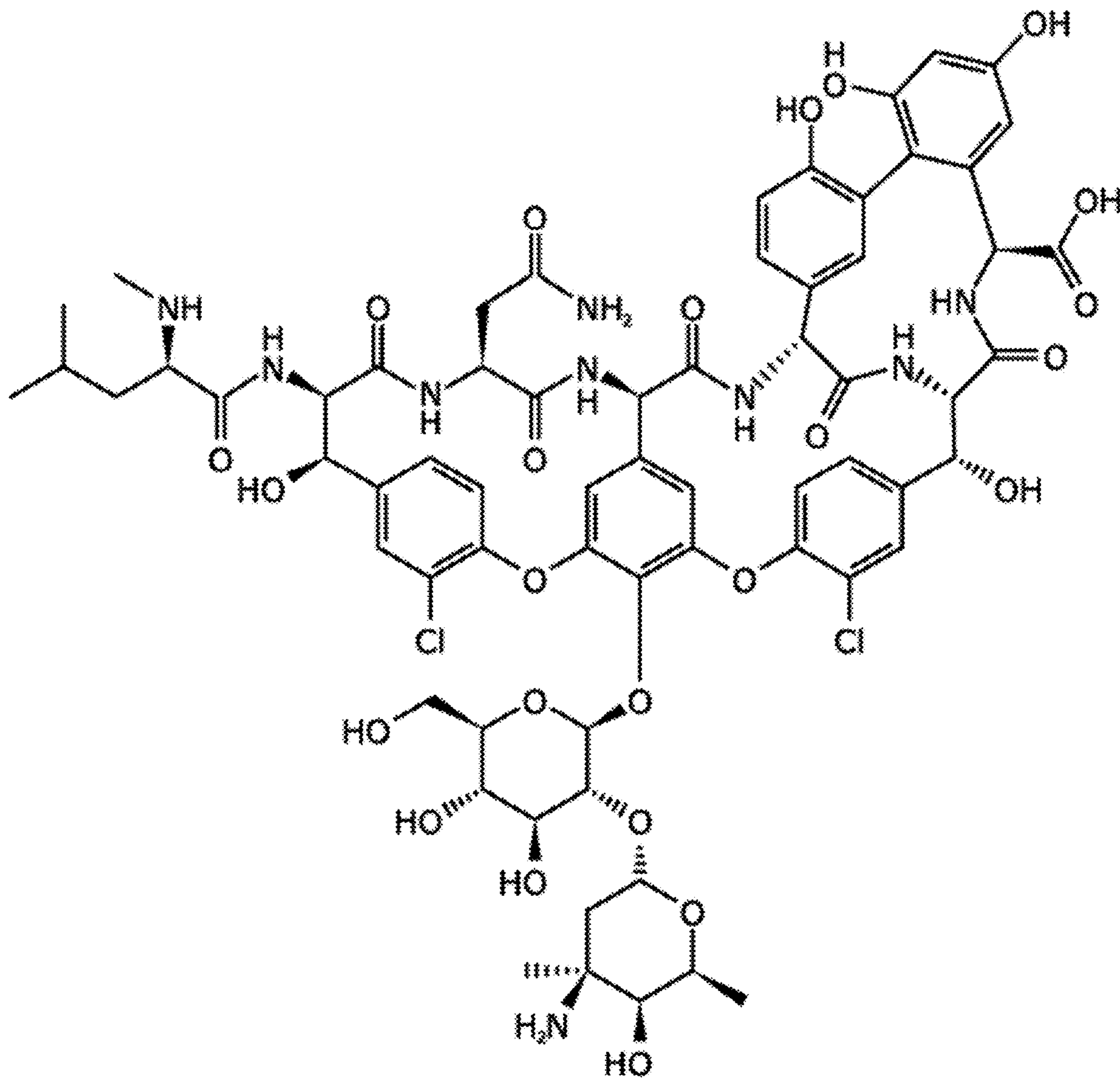
Vancomycin (Formula 1)
