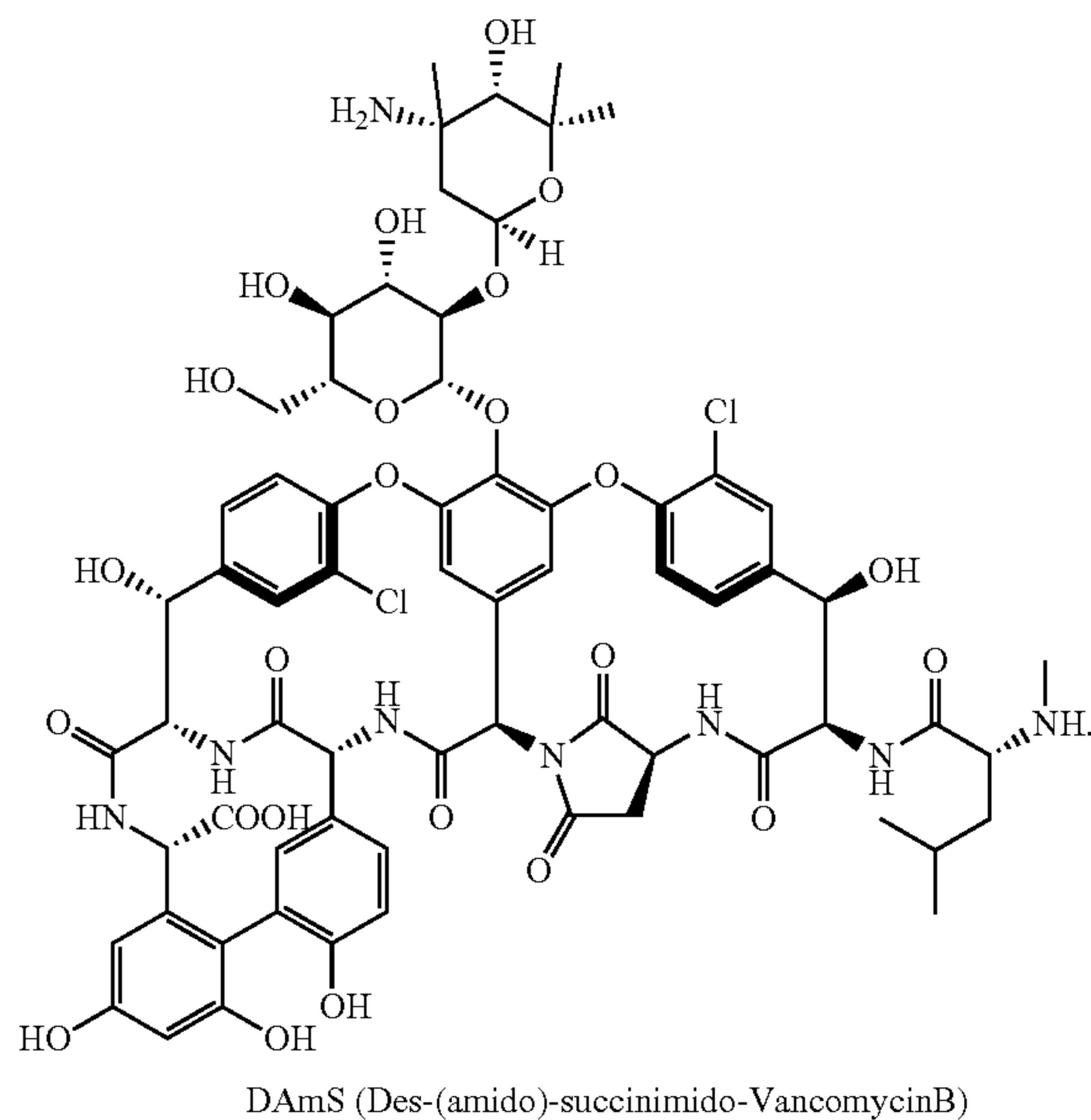
Formula 2
