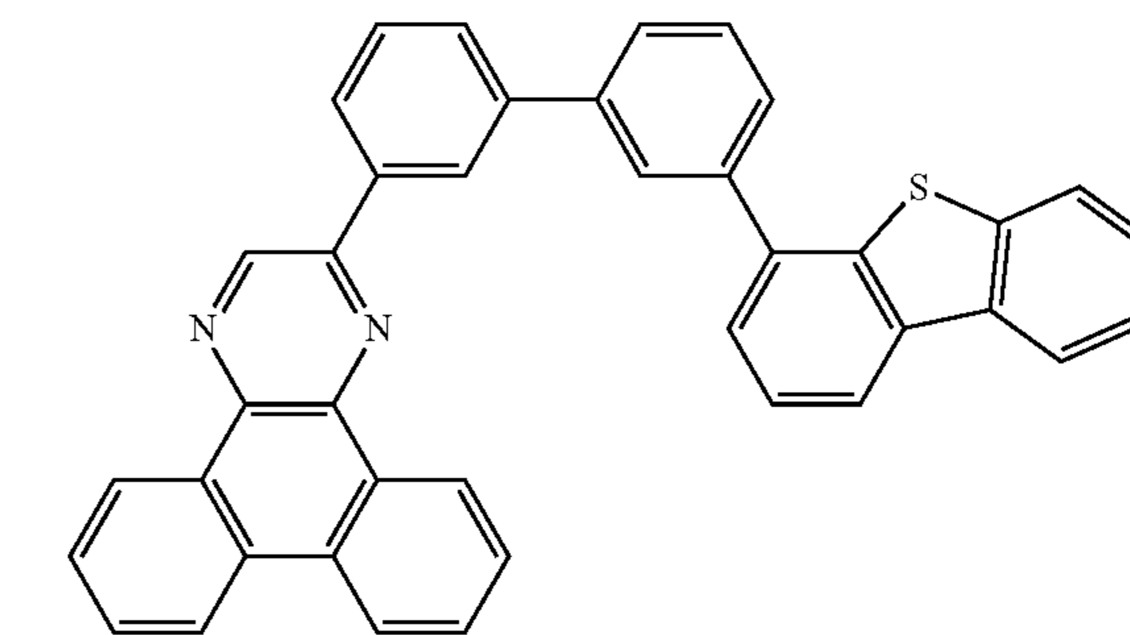
2mDBTBPDBq-II
