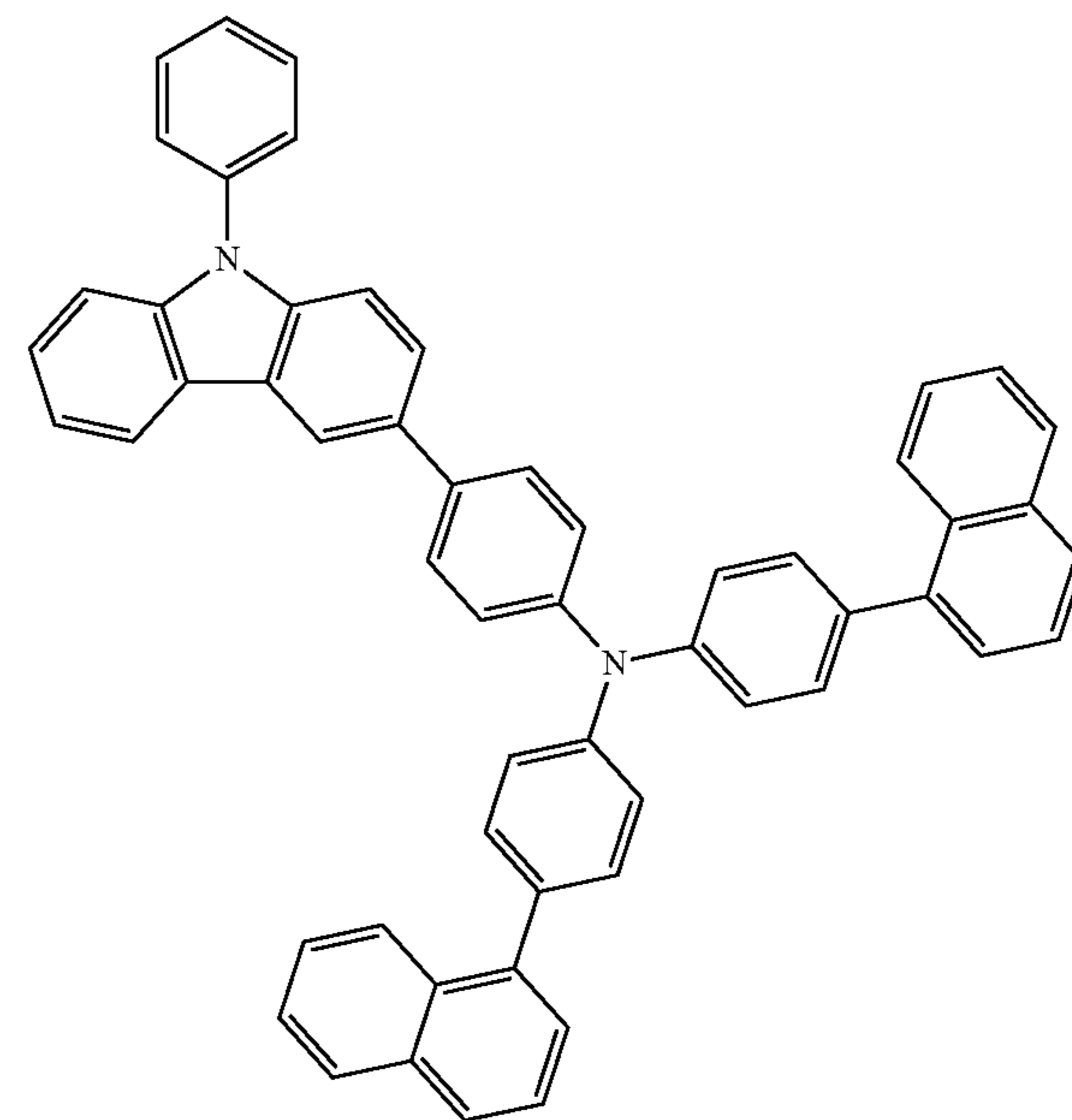
PCBNBB
