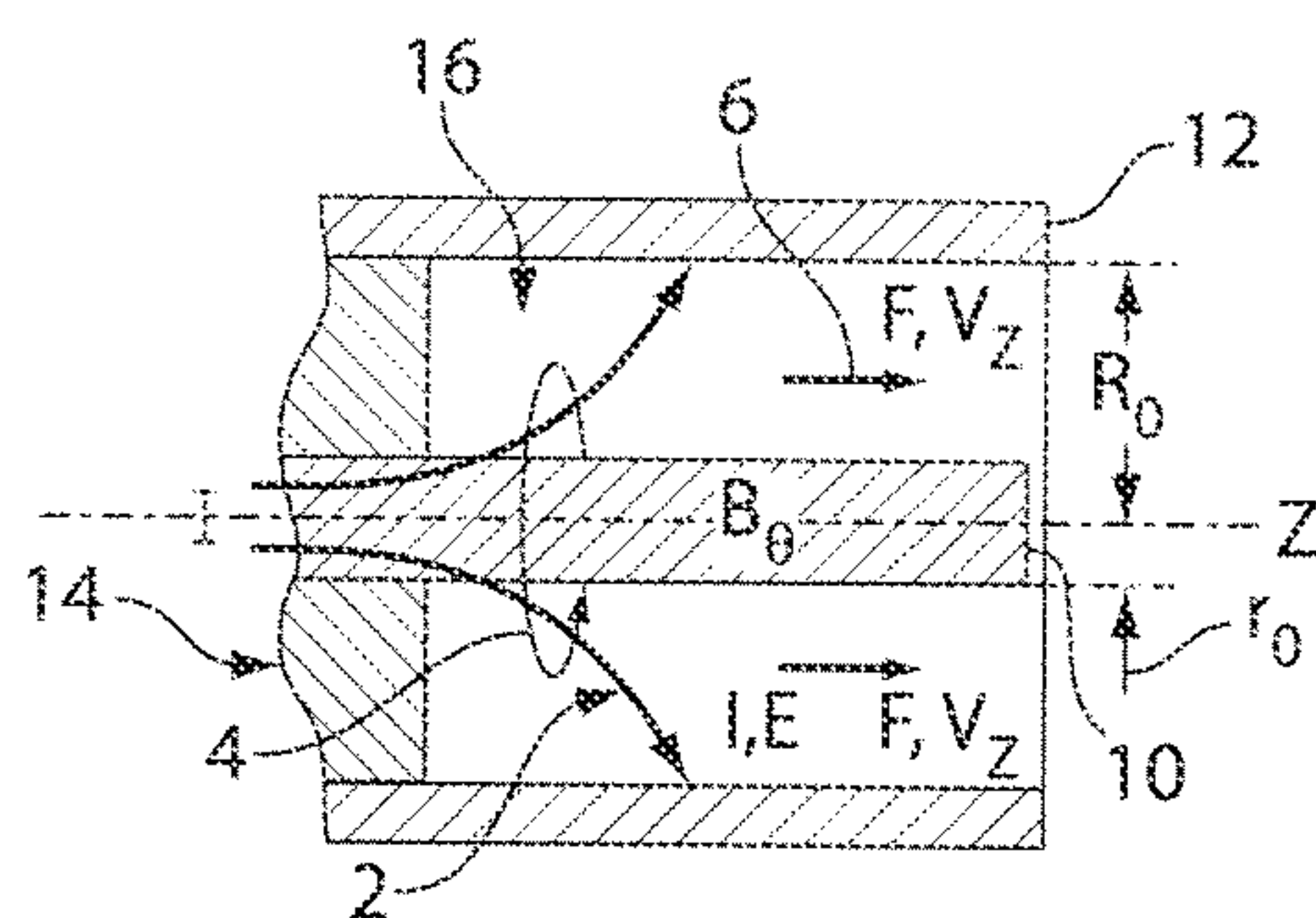
Fig. 1 (Prior Art)
