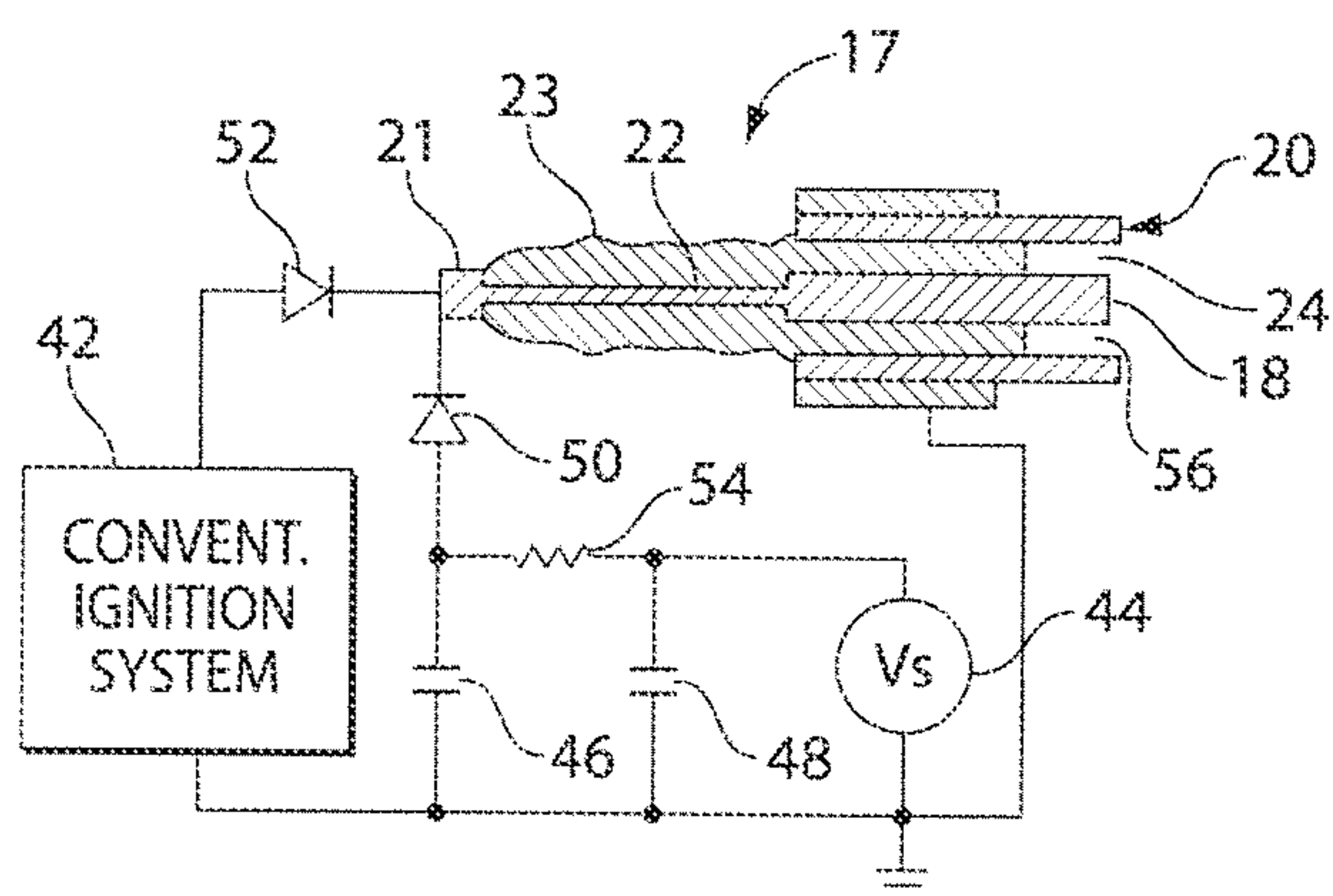
Fig. 2 (Prior Art)
