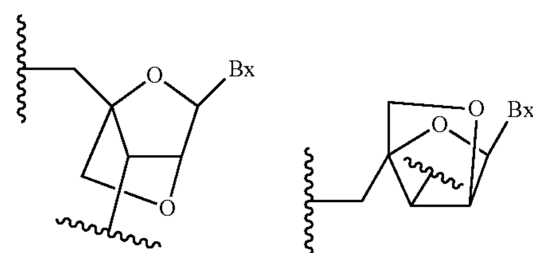
LNA (β-D-configuration) α-L-LNA (α-L-configuration) bridge = 4'-CH 2 -O-2' bridge = 4'-CH 2 -O-2'
