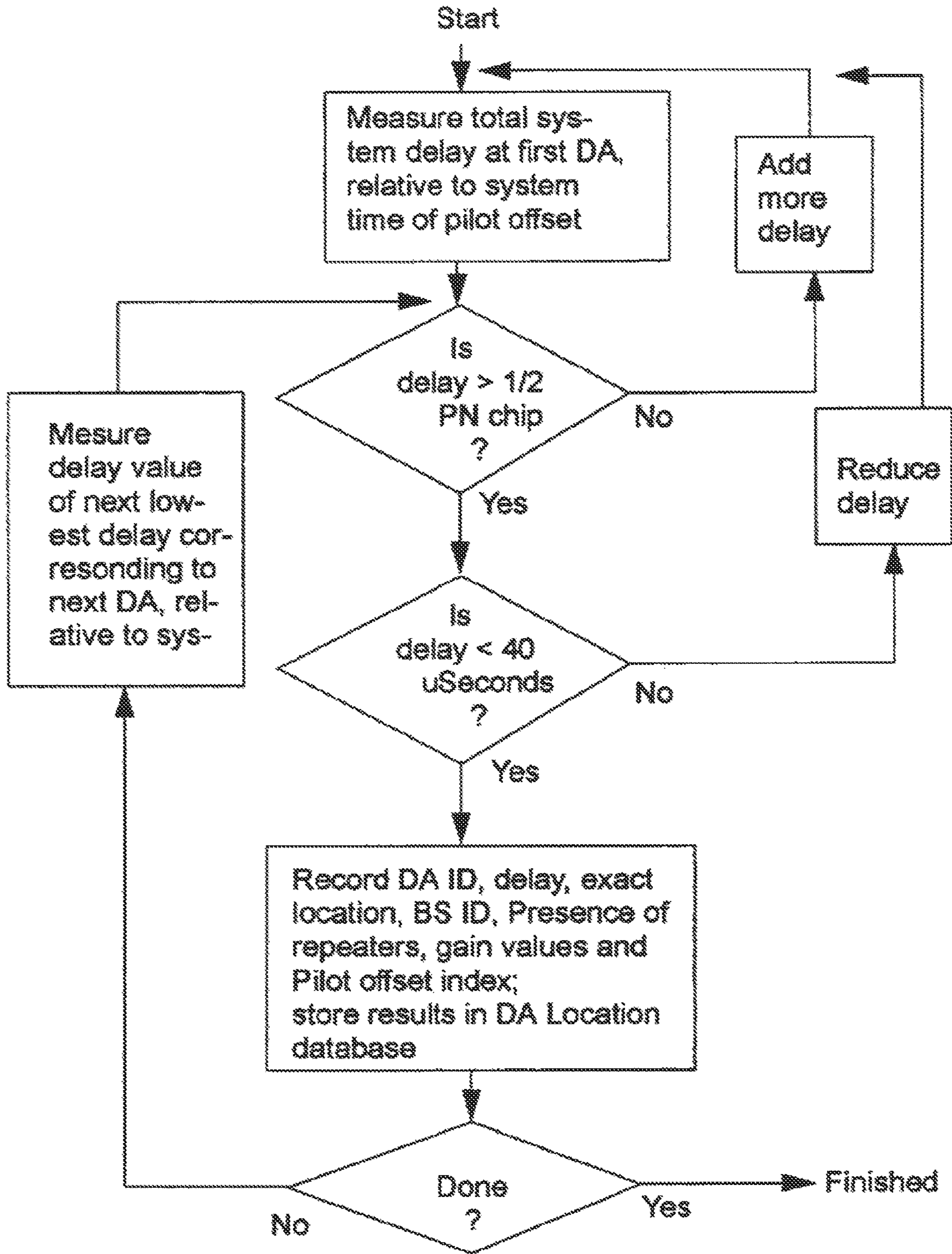
FIG. 8: DA Installation Procedure for Wireless Location
