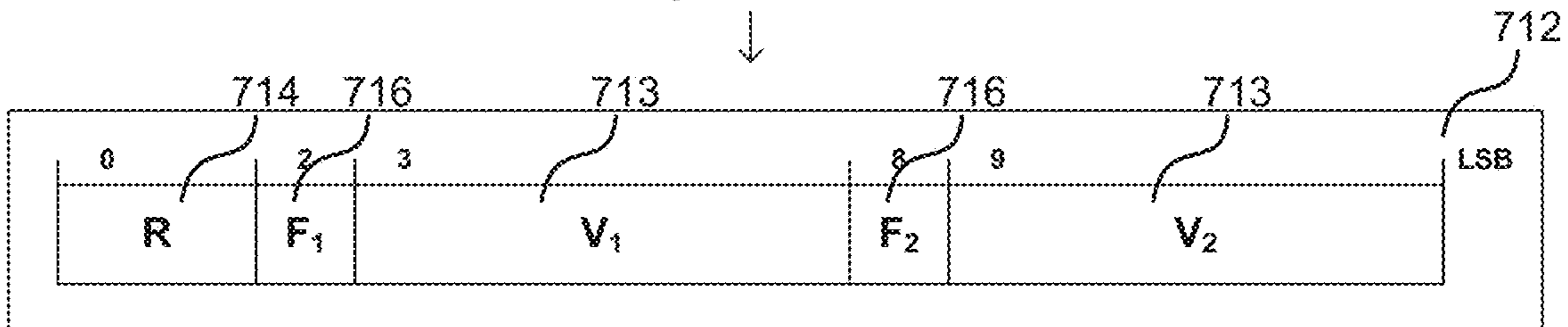
Sub-Block Data Layout
