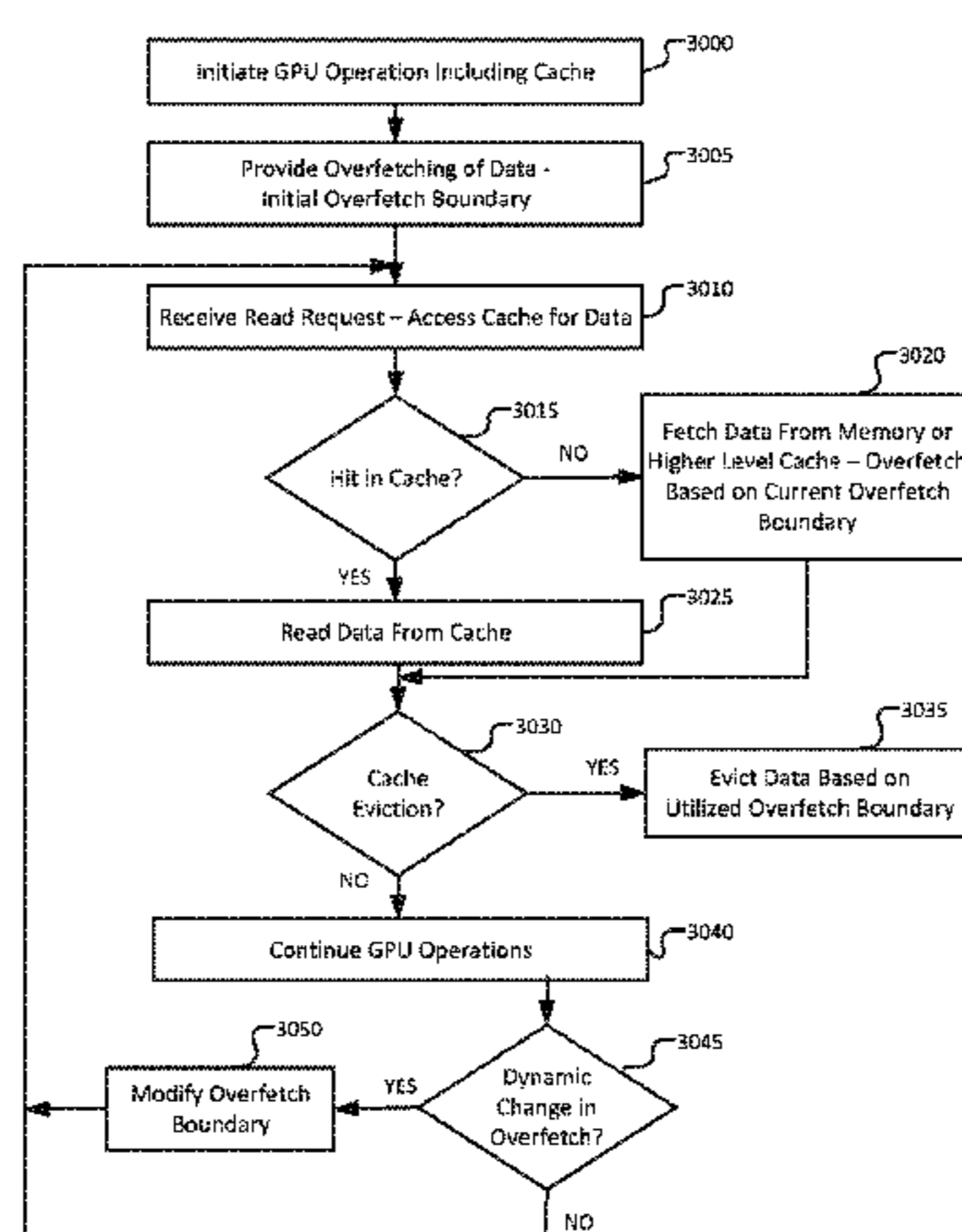
PROCESS FOR DYNAMIC OVERFETCHING OF CACHE LINES
