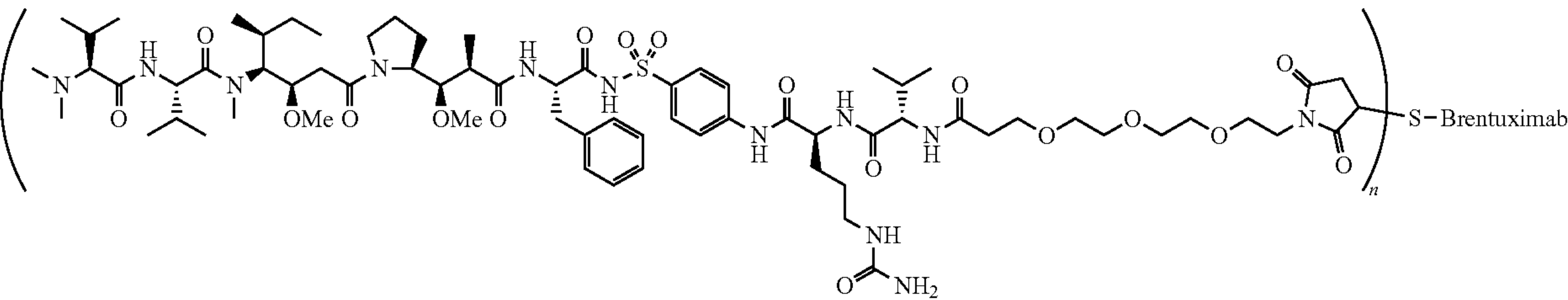
B-MTvc-Compound 11
