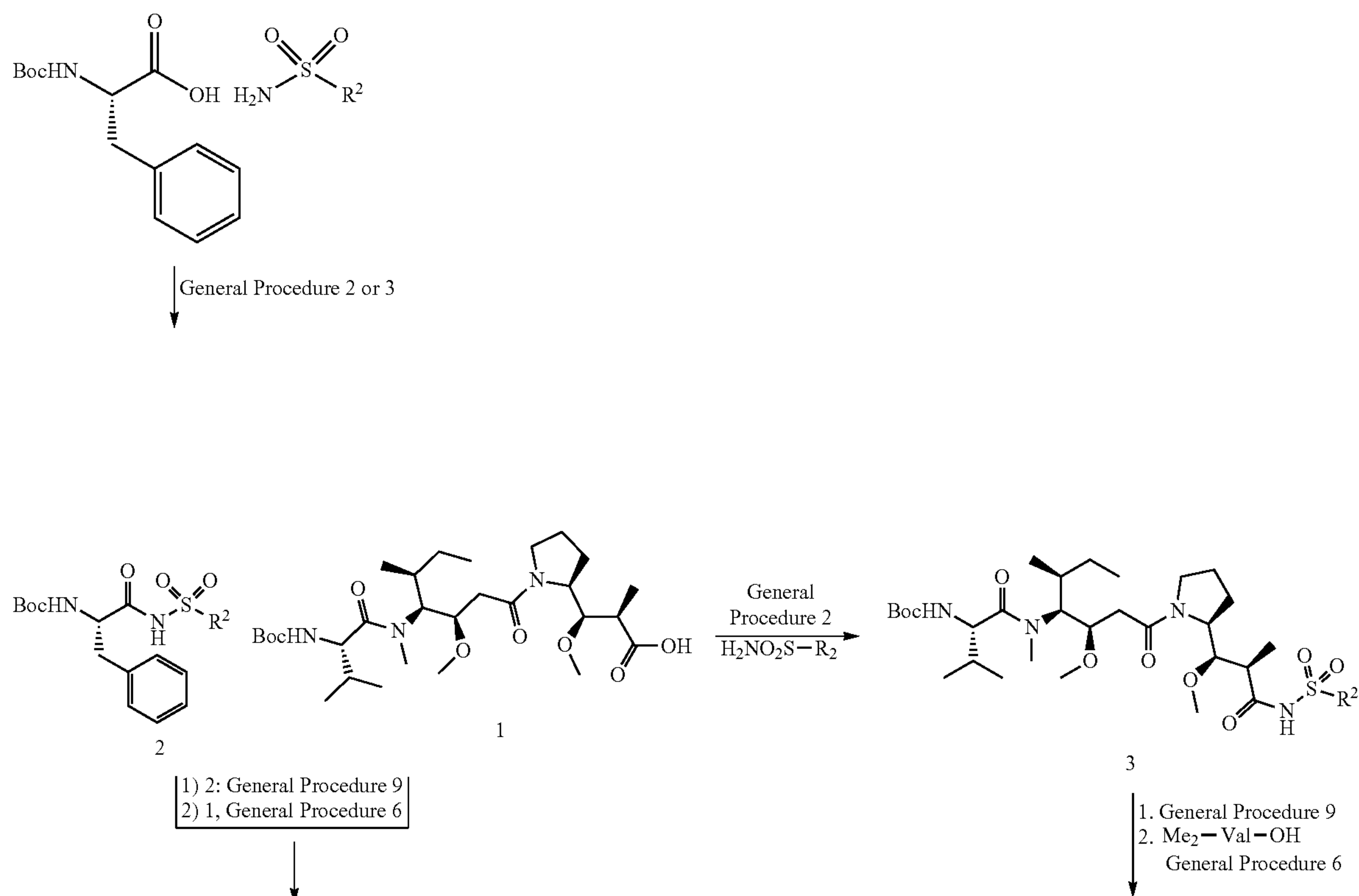
Synthetic Scheme A
