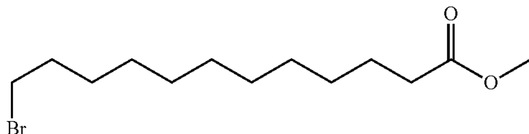
Methyl 12-bromododecanoate
