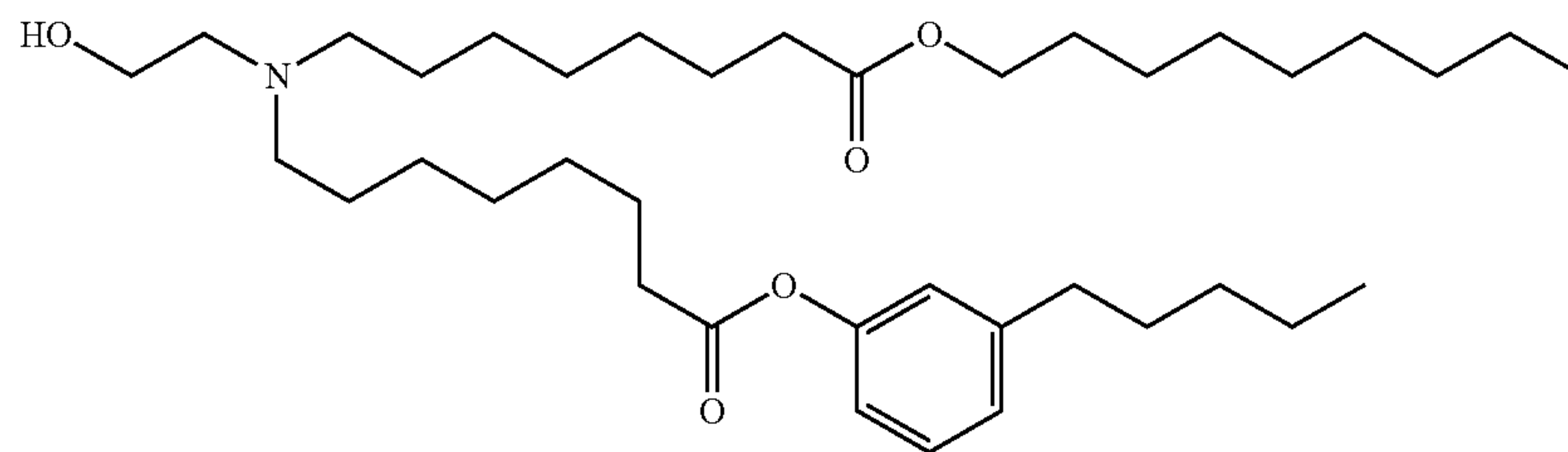
Nonyl 8-((2-hydroxyethyl)(8-oxo-8-(3-pentylphenoxy)octyl)amino)octanoate
