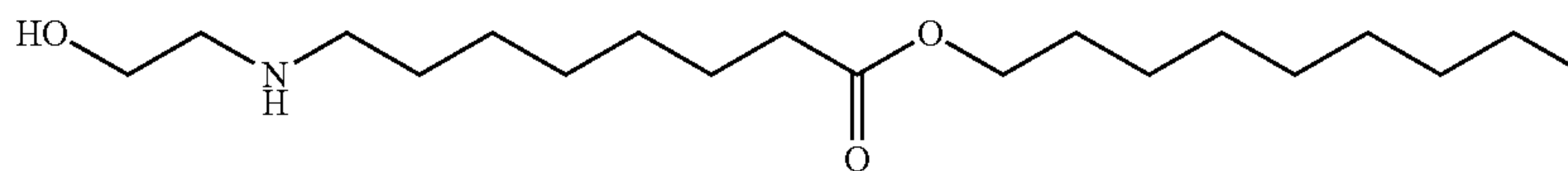
Nonyl 8-((2-hydroxyethyl)amino)octanoate
