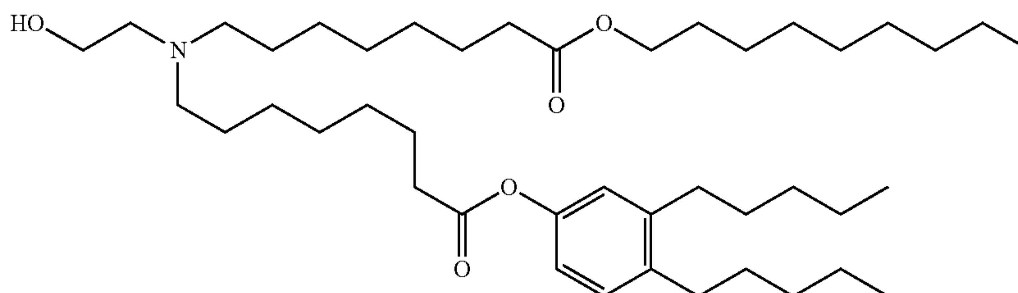
3,4-Dipentylphenyl 8-((2-hydroxyethyl)(8-(nonyloxy)-8-oxooctyl)amino)octanoate
