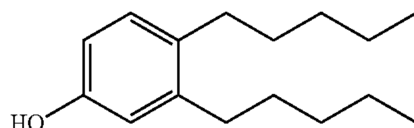
3,4-Dipentylphenol
