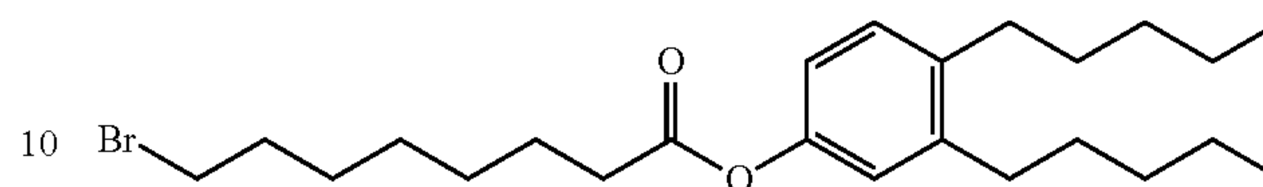
3,4-Dipentylphenyl 8-bromooctanoate
