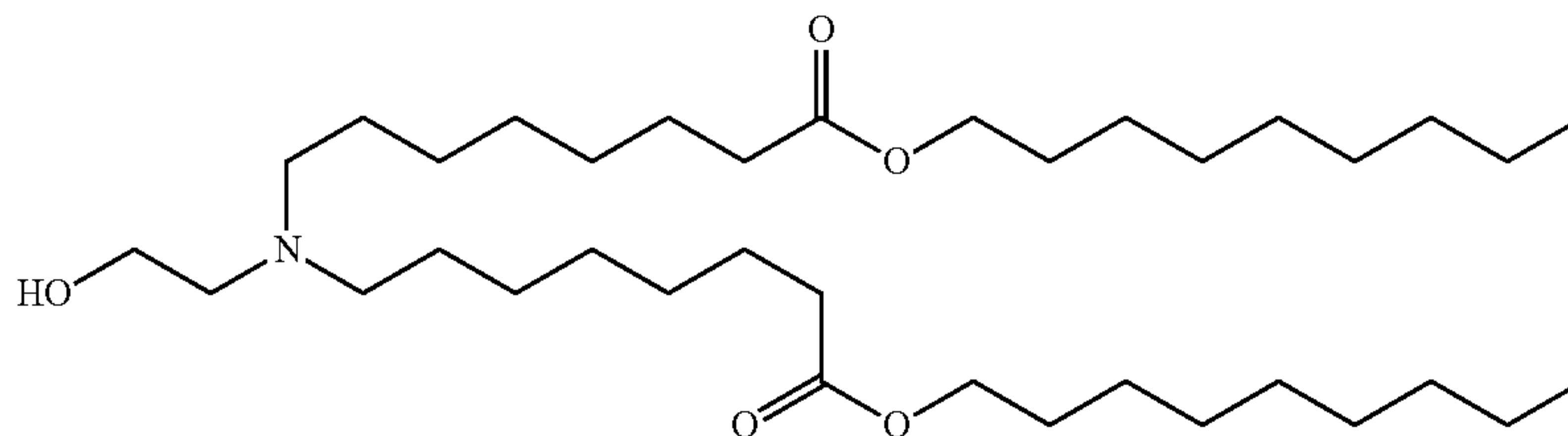
Dinonyl 8,8'-((2-hydroxyethyl)azanediyl)dioctanoate
