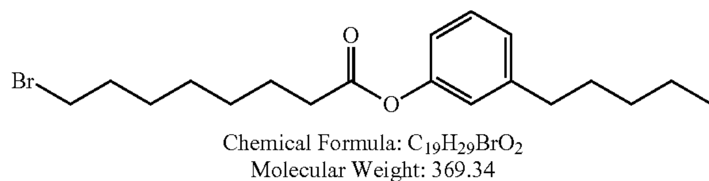
3-Pentylphenyl 8-bromooctanoate
