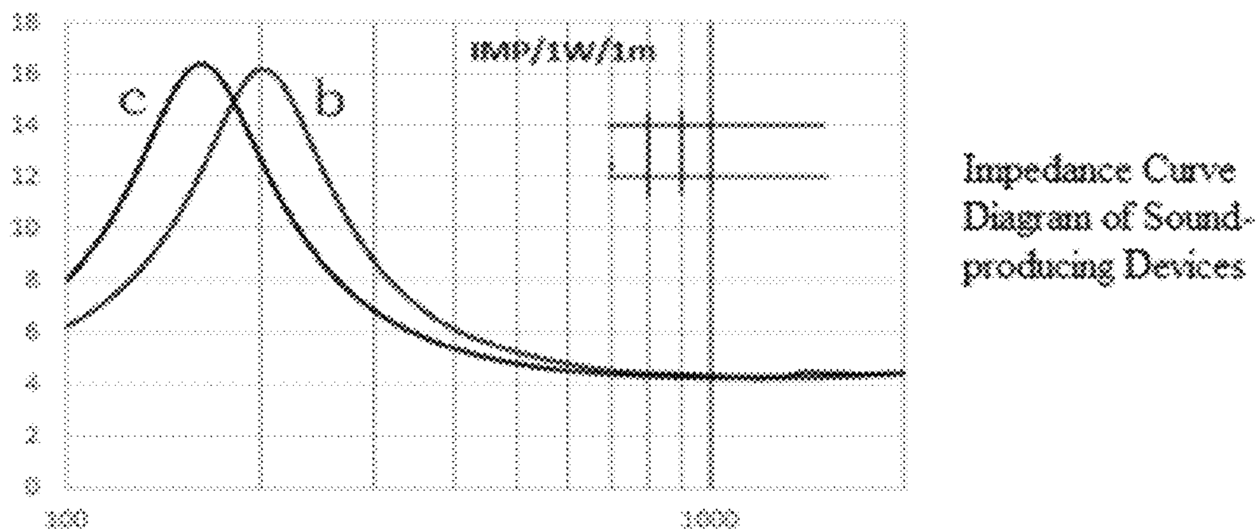
b: A Sound-producing Device Installed with a Prior Art Damper: Resonant Frequency F_0=195Hz c: A Sound-producing Device Installed with the Damper of the Present Disclosure: Resonant Frequency F_0=170Hz
