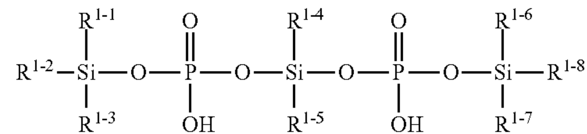
[Chemical Formula 57]
