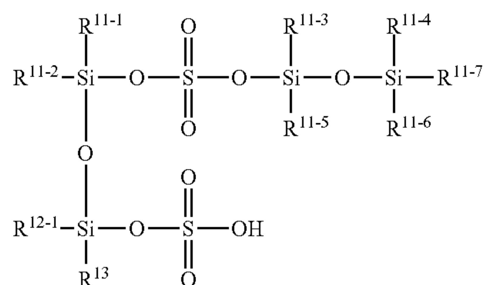
[Chemical Formula 236]
