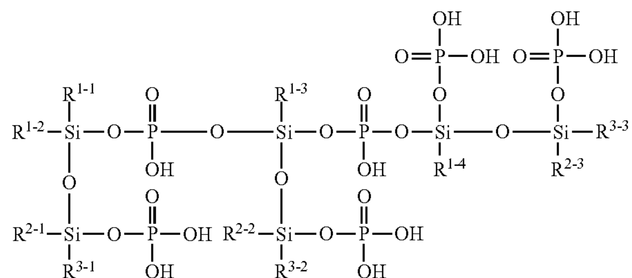
[Chemical Formula 210]
