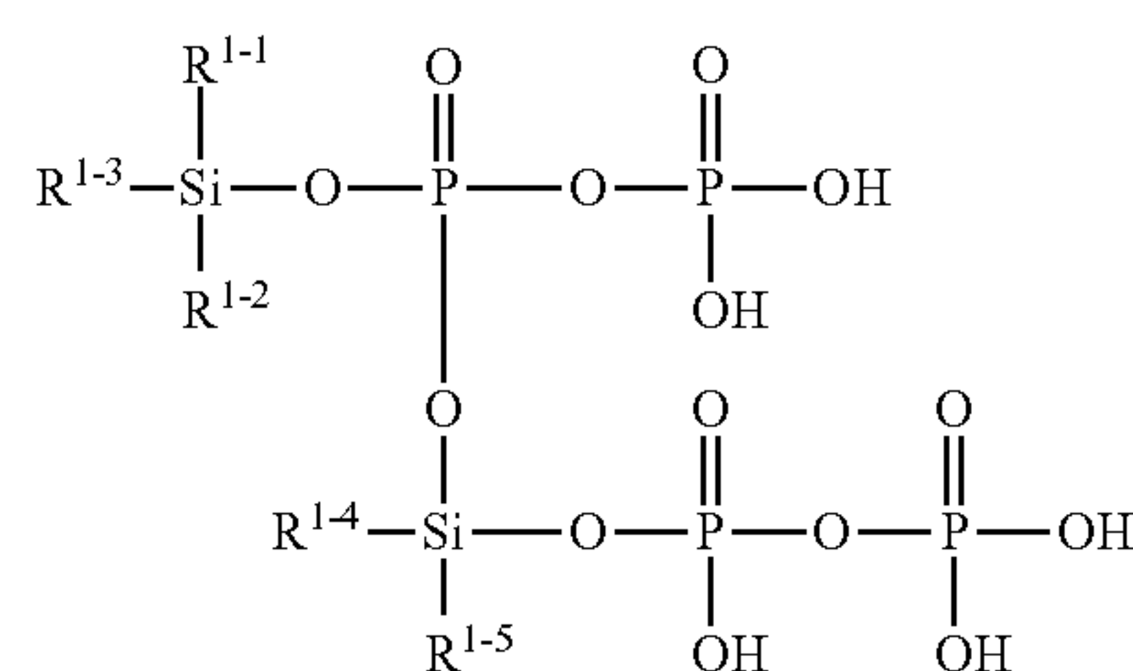
[Chemical Formula 105]
