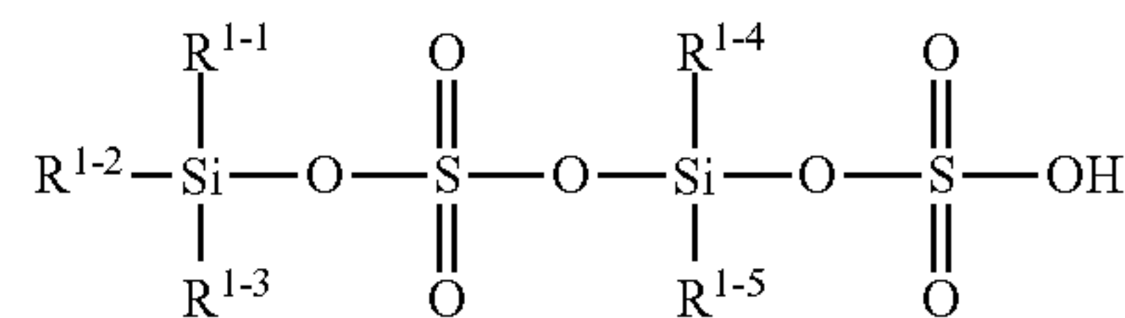
[Chemical Formula 66]
