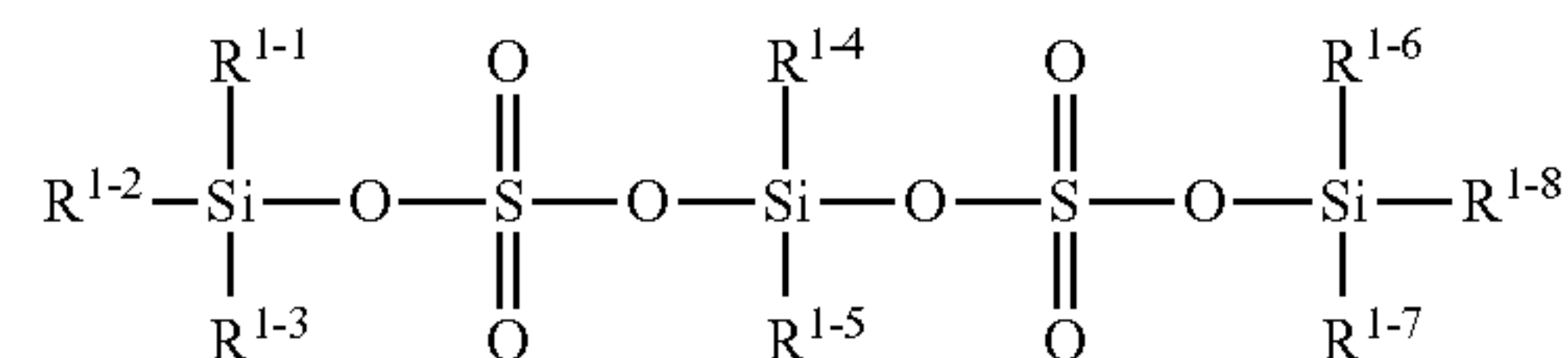
[Chemical Formula 66]
