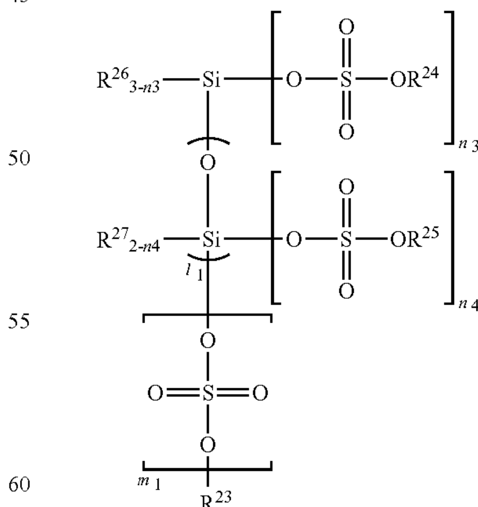
[Chemical Formula 210]
