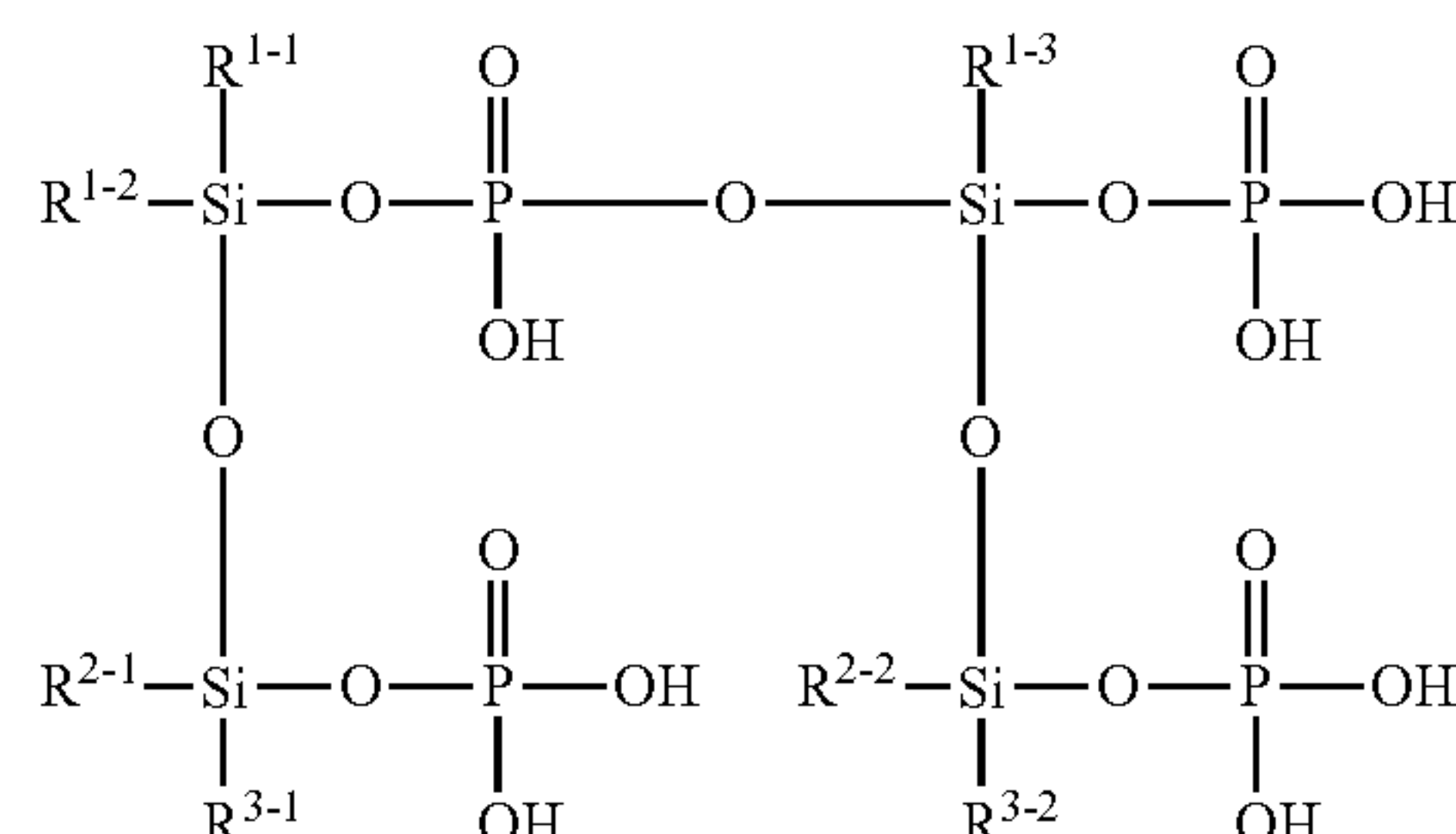
[Chemical Formula 207]
