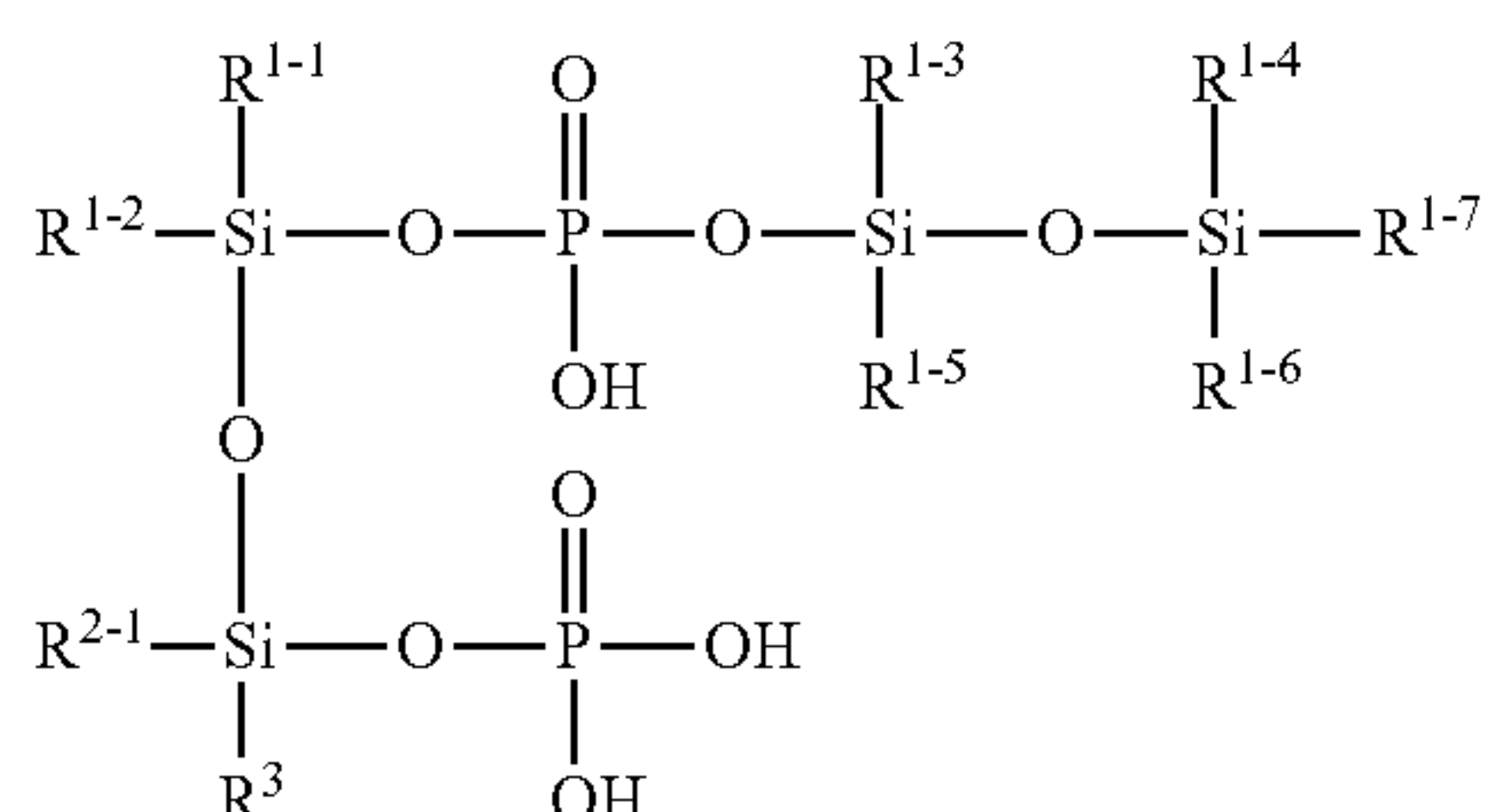
[Chemical Formula 206]
