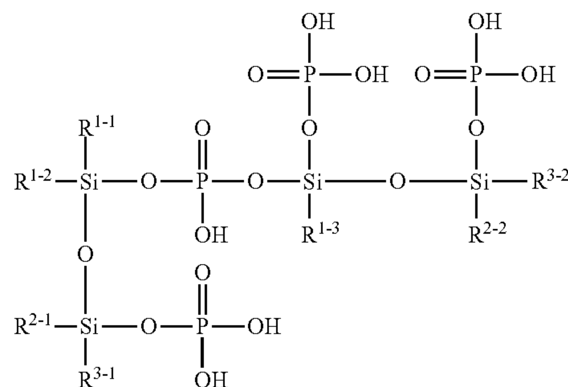
[Chemical Formula 208]
