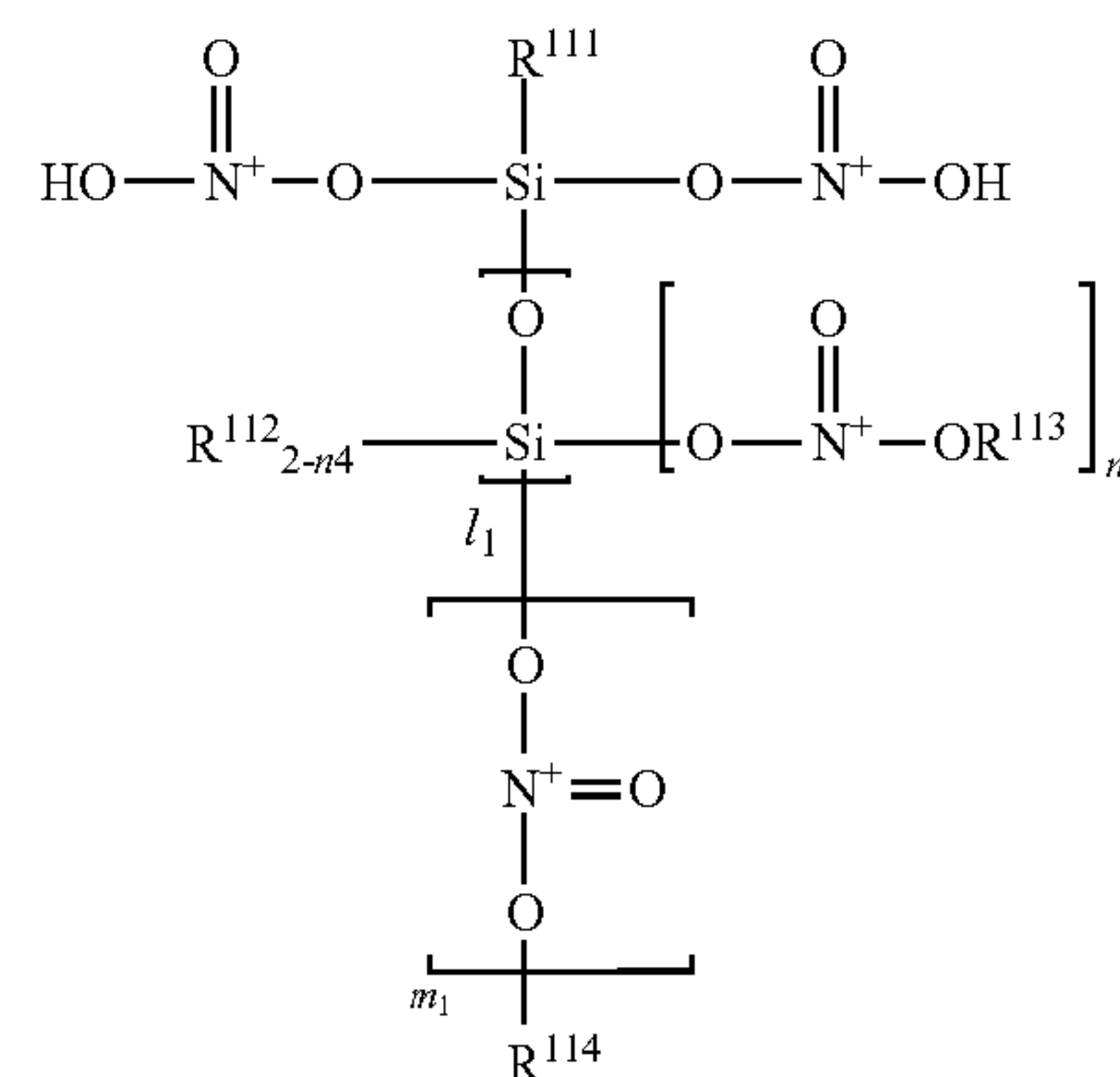
[Chemical Formula C260-1]
