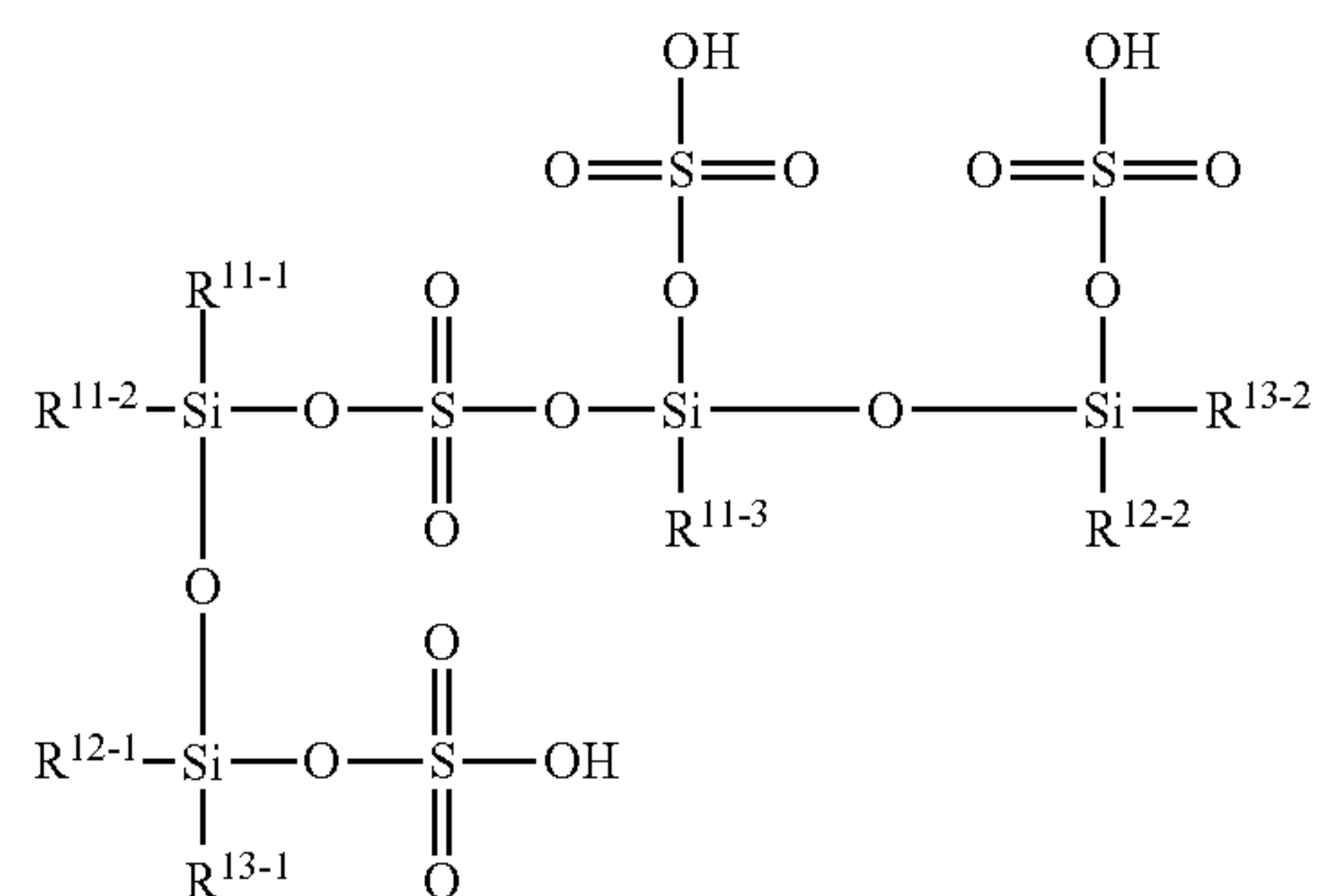
[Chemical Formula 237]
