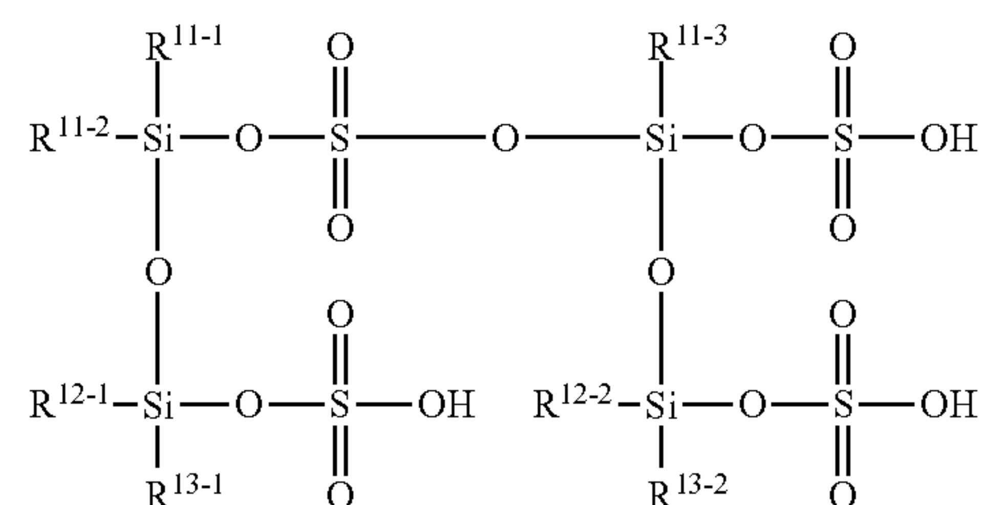
[Chemical Formula 236]
