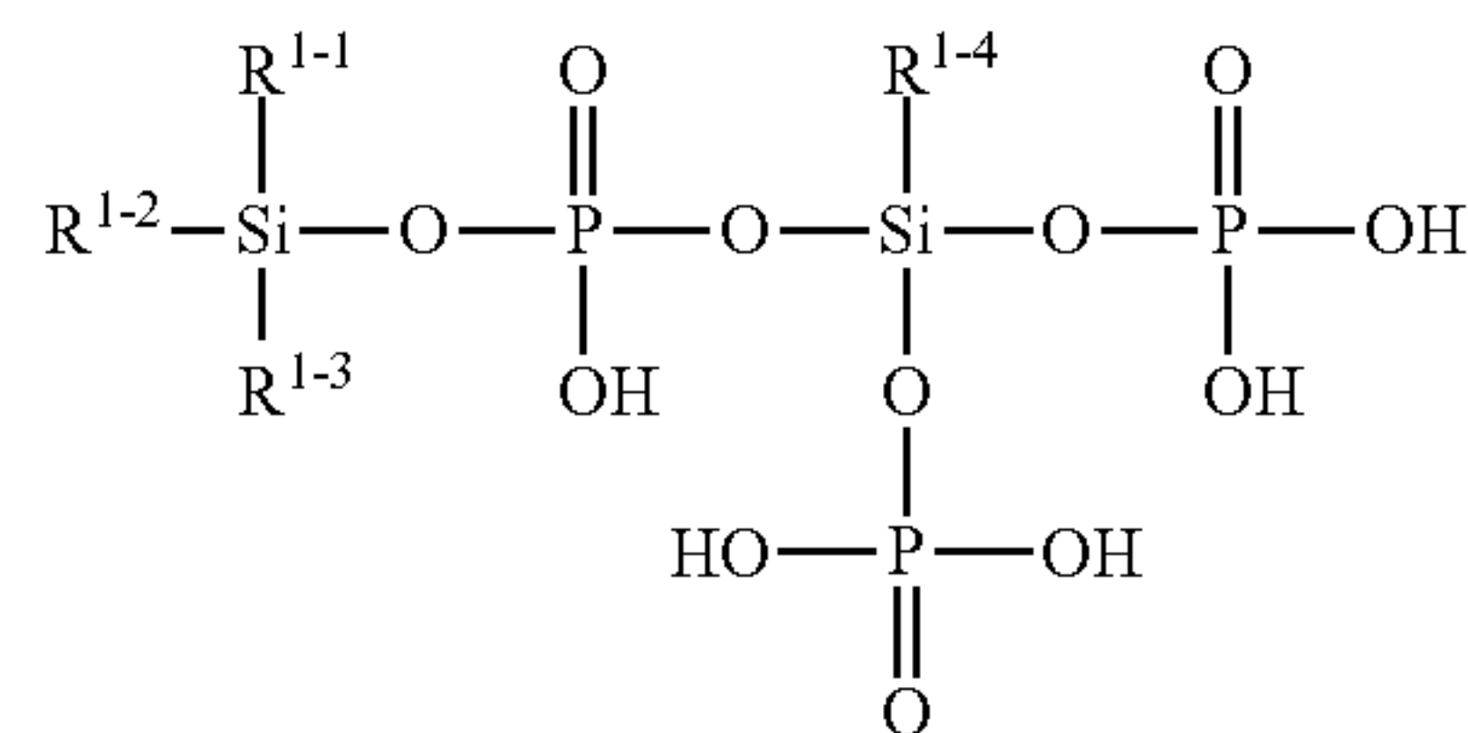
[Chemical Formula 61]
