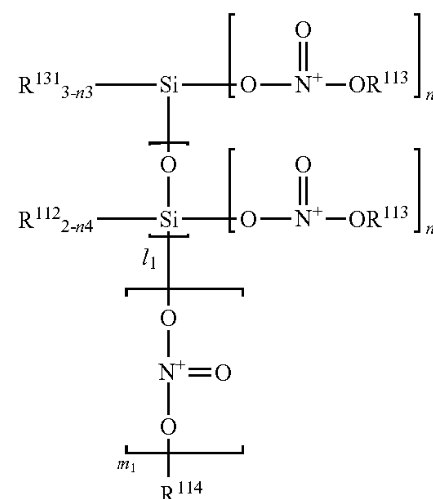
[Chemical Formula C280-1]
