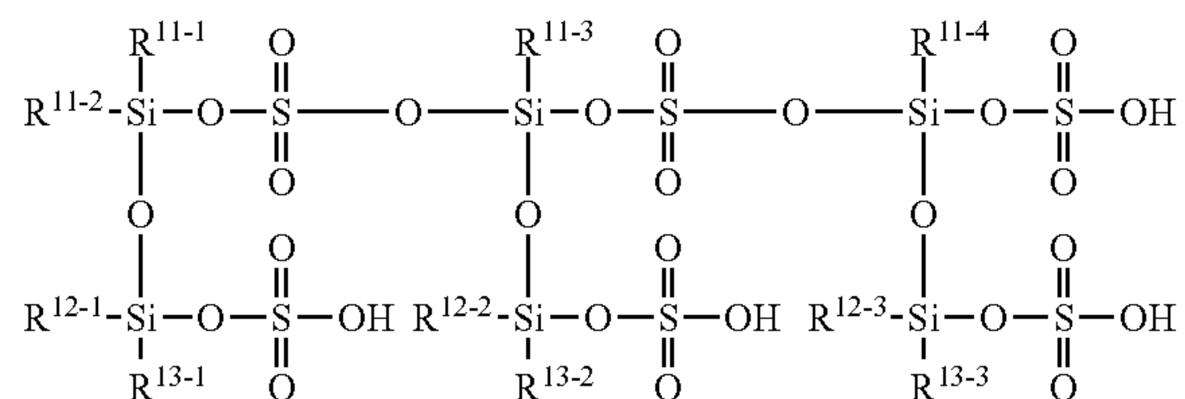
[Chemical Formula 238]
