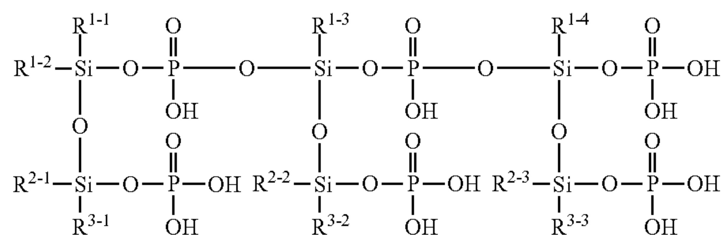
[Chemical Formula 209]
