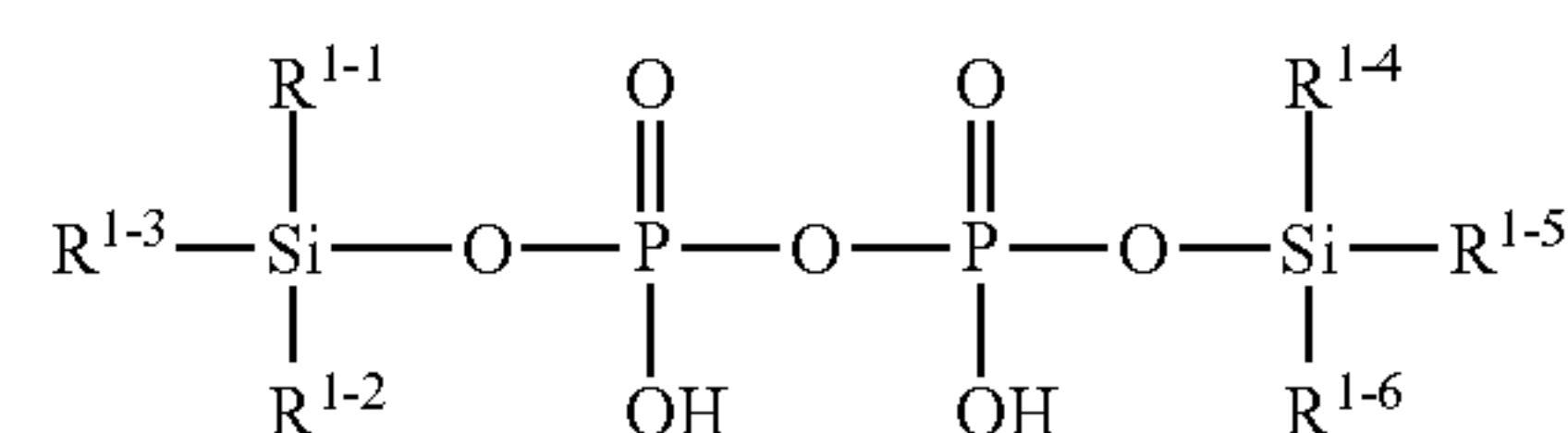
[Chemical Formula 104]
