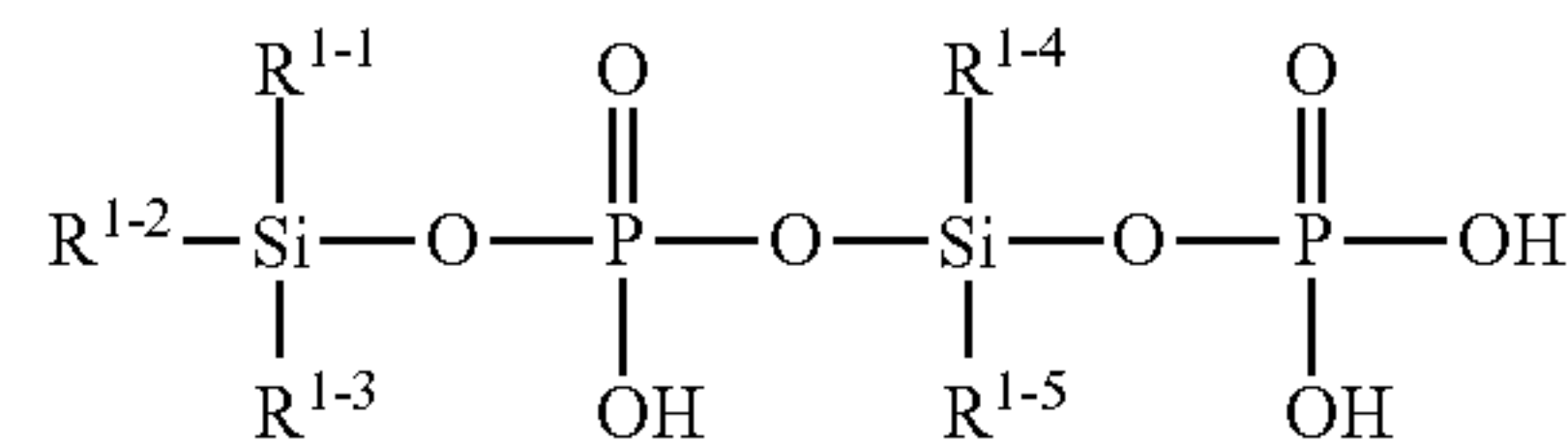
[Chemical Formula 56]
