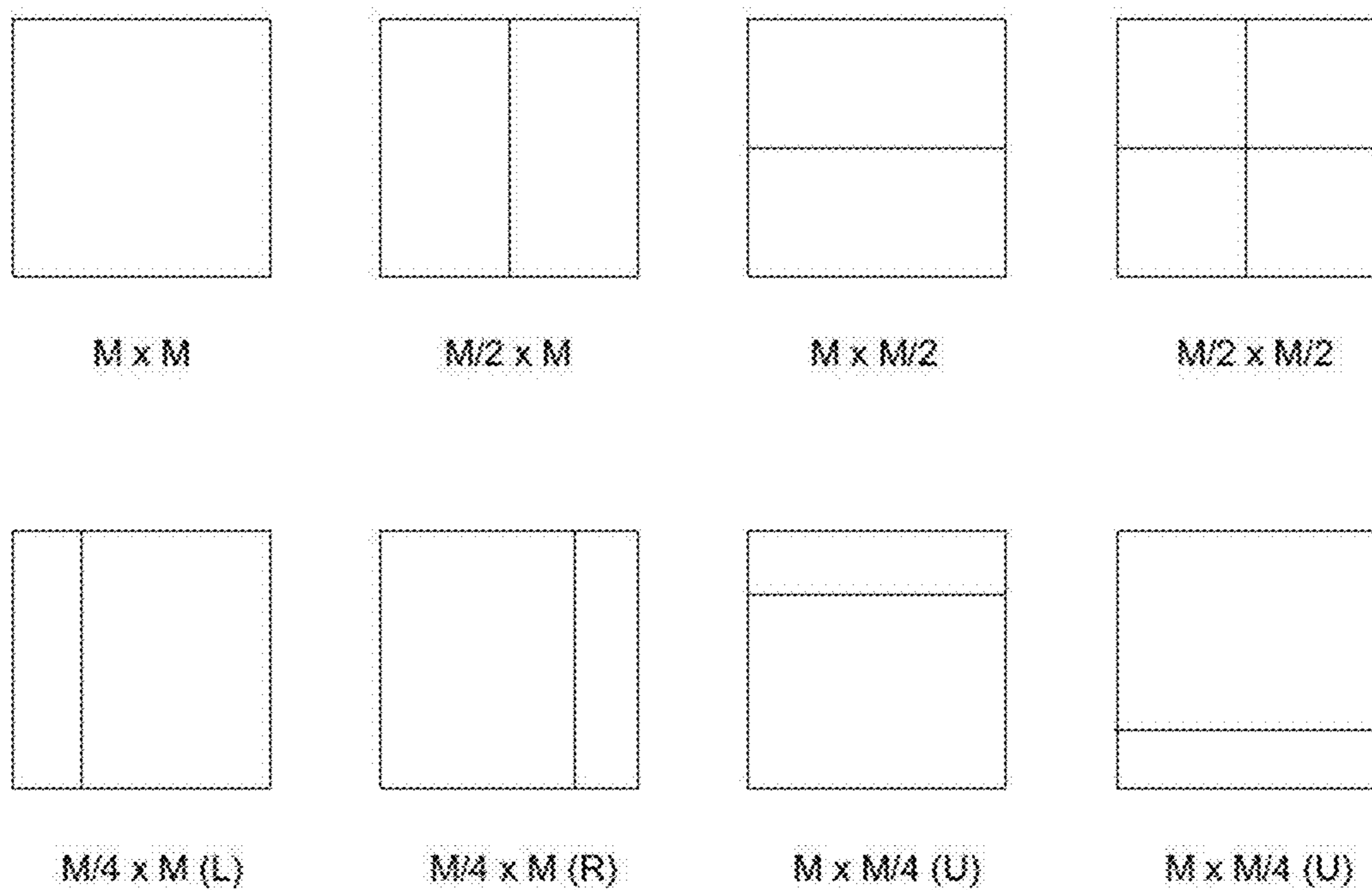
Modes for splitting a CB into PBs, subject to certain size constraints. For intrapicture-predicted CBs, only M \times M and M/2 \times M/2 are supported
