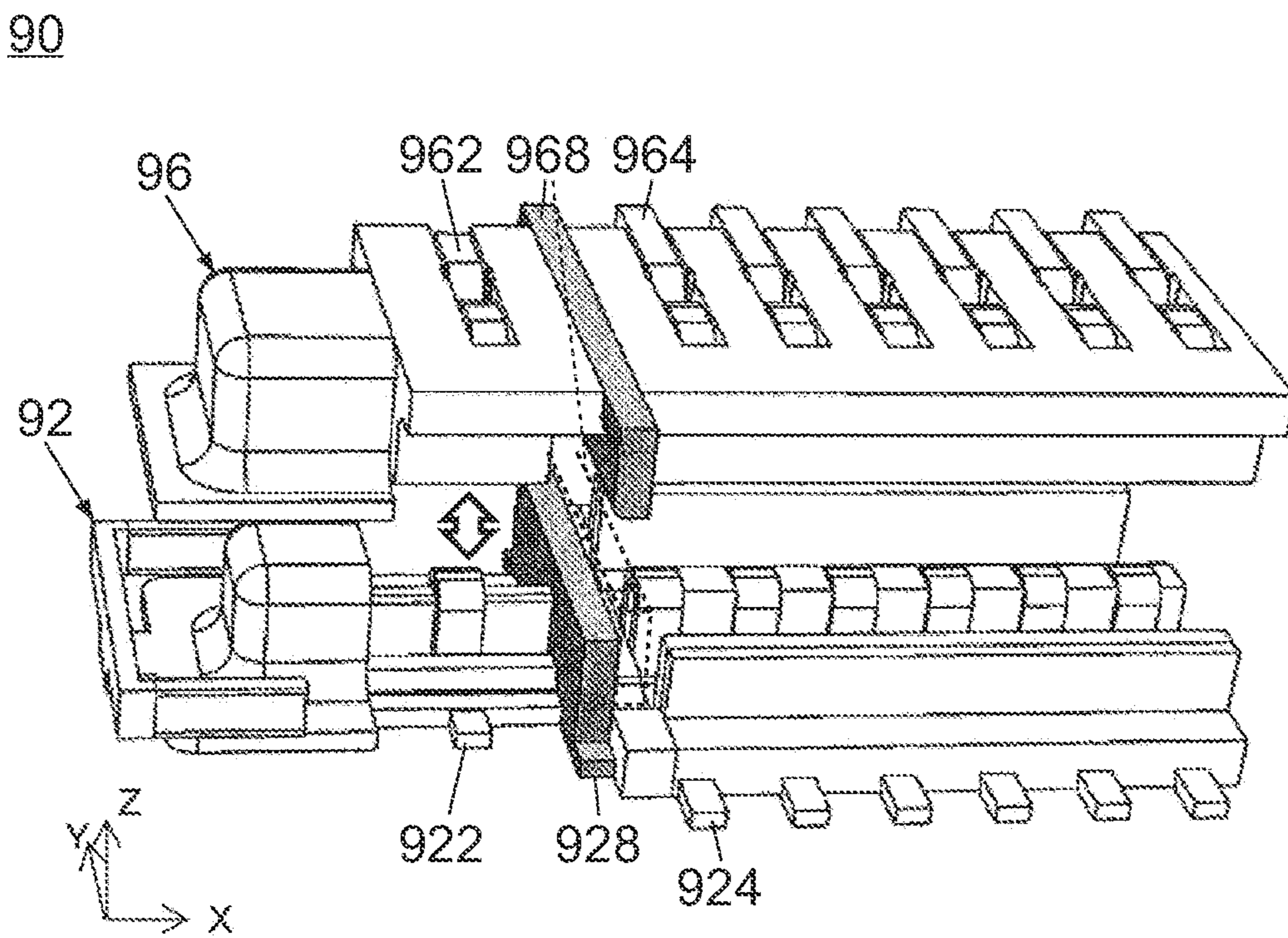
FIG. 14 PRIOR ART
