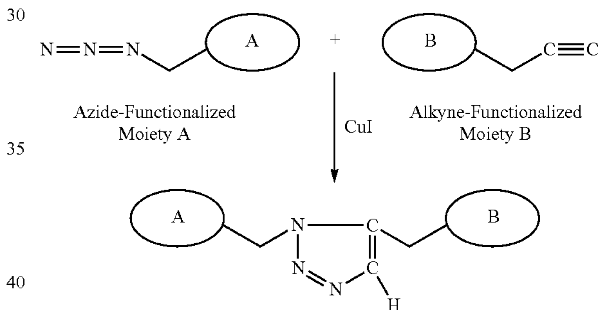
A and B Crosslinked via Triazole Moiety
