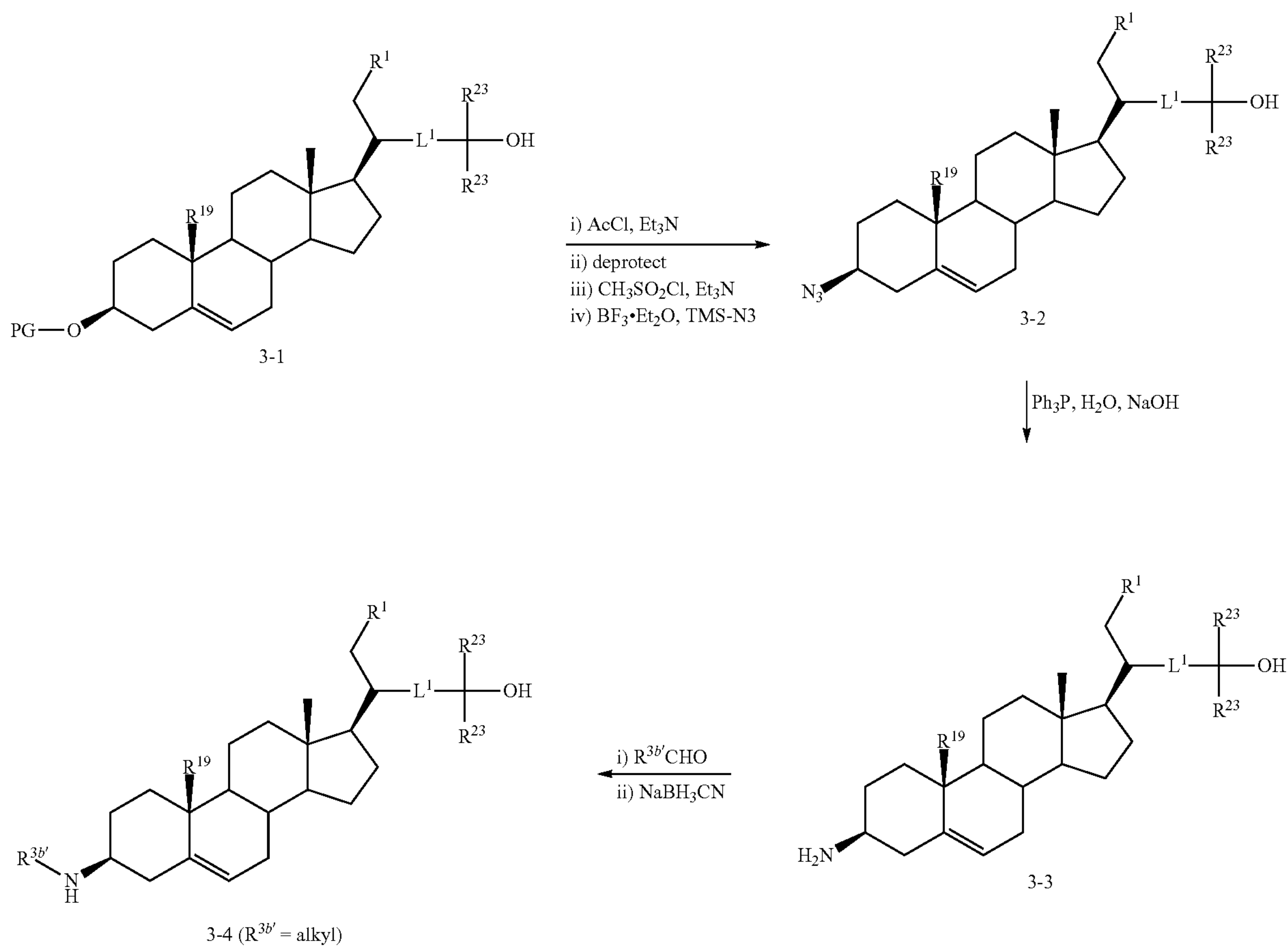
Scheme 3. Synthesis of 3β-Amino- and 3β-alkylamino steroids
