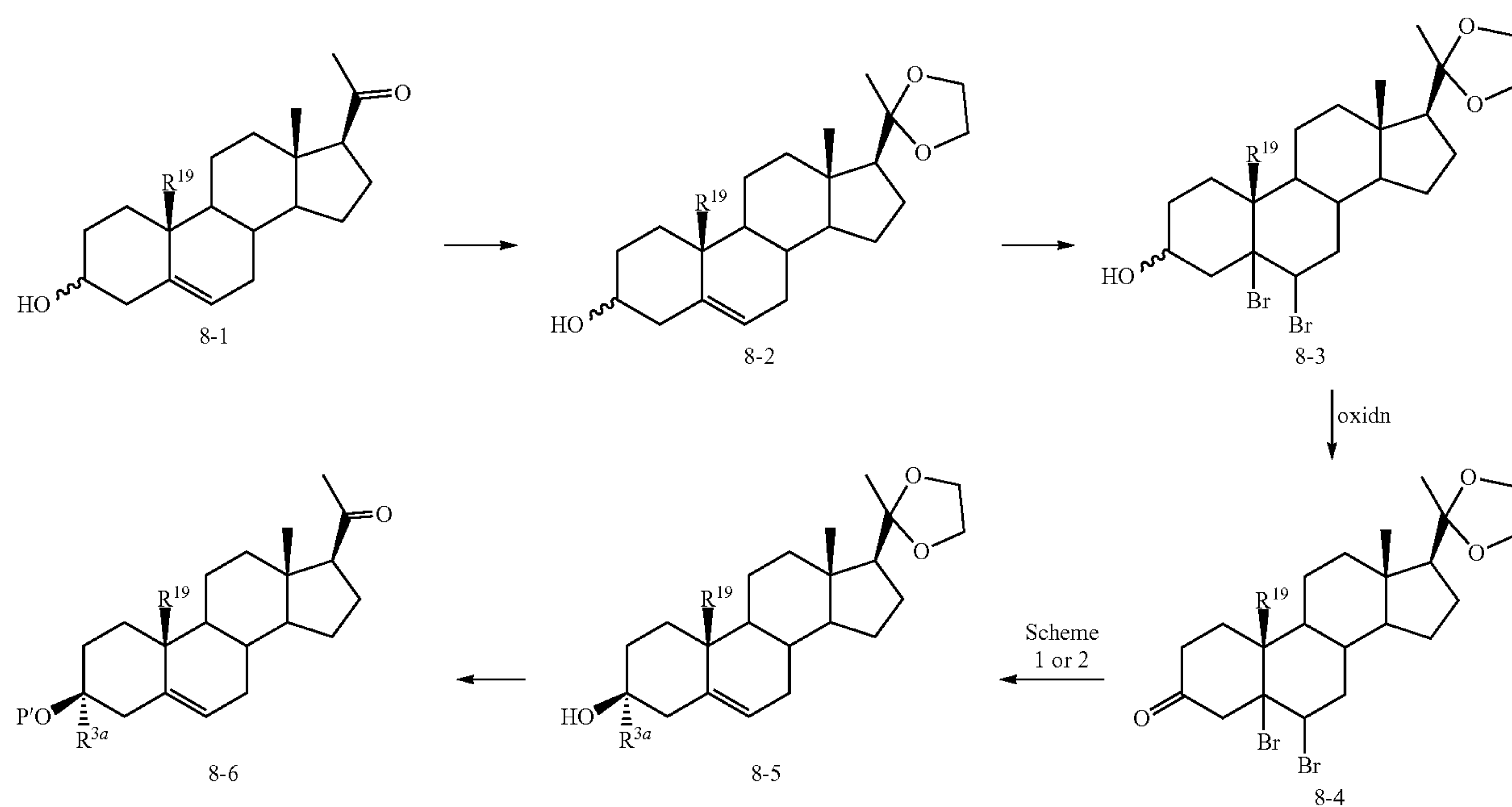
Scheme 8. Synthesis of 3 \alpha -Substituted-3 \beta -hydroxy steroids
