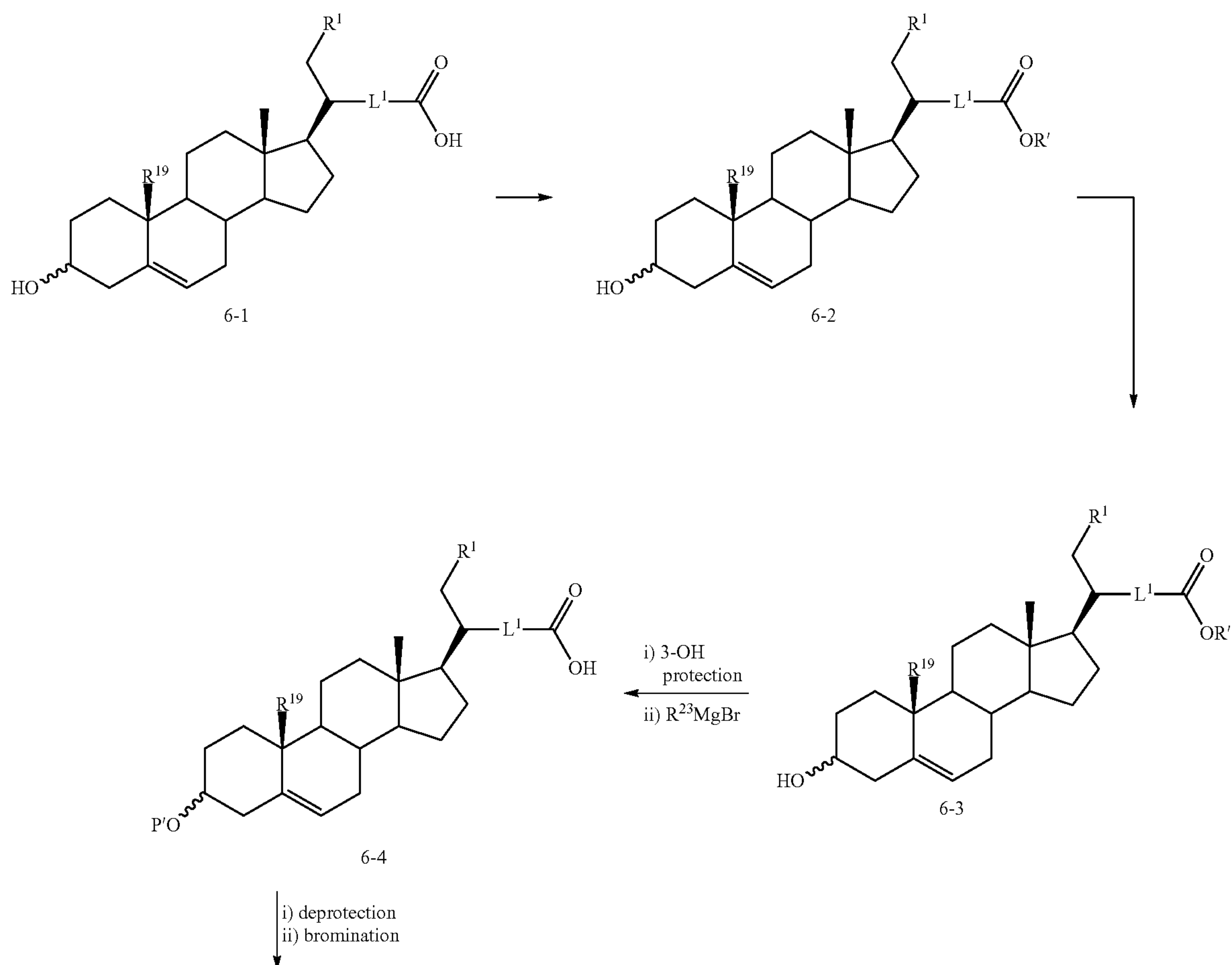
Scheme 6. Synthesis of 3-Oxo Steroids
