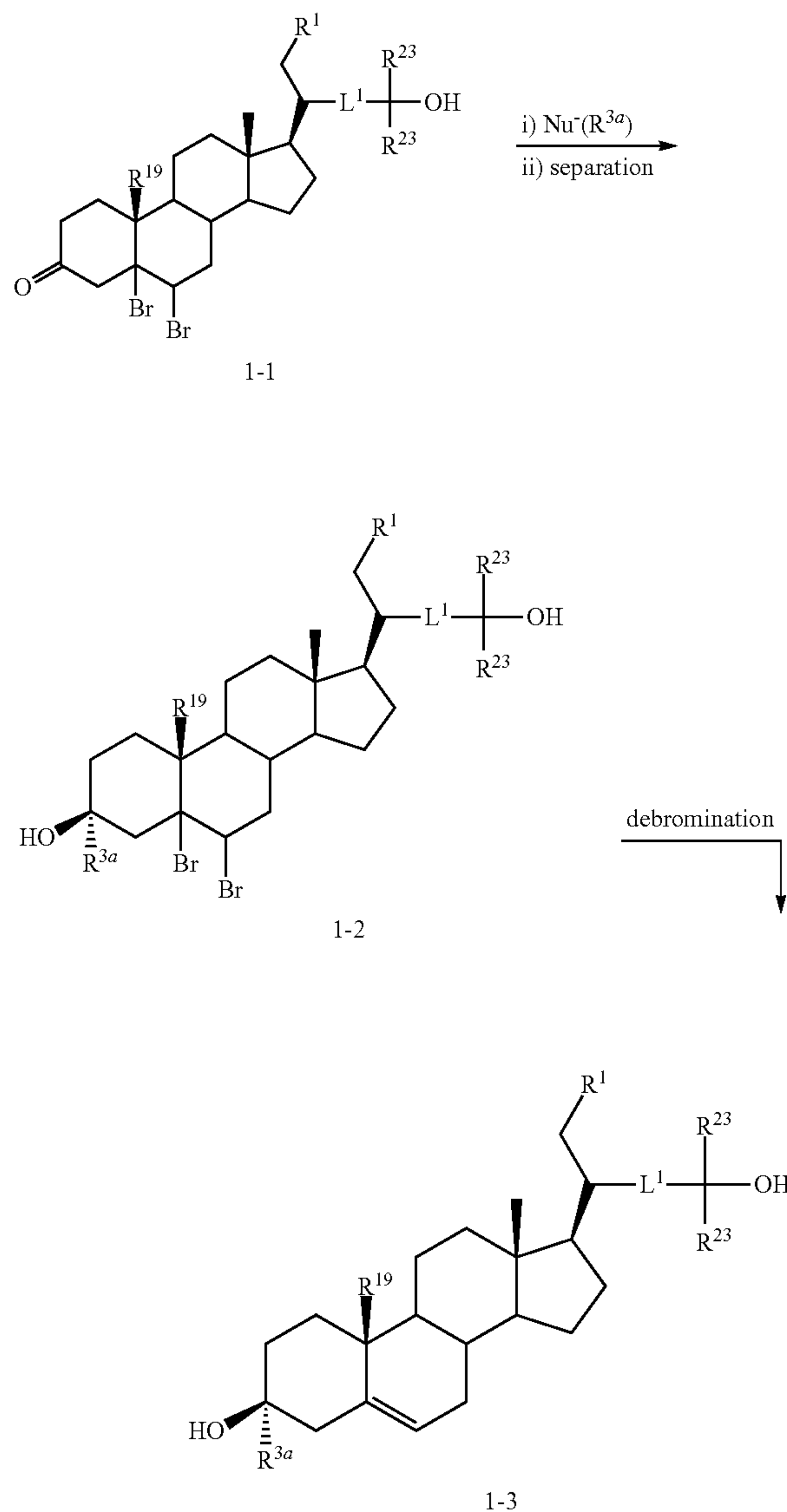
Scheme 1. Synthesis of 3α-Substituted-3β-hydroxy steroids
