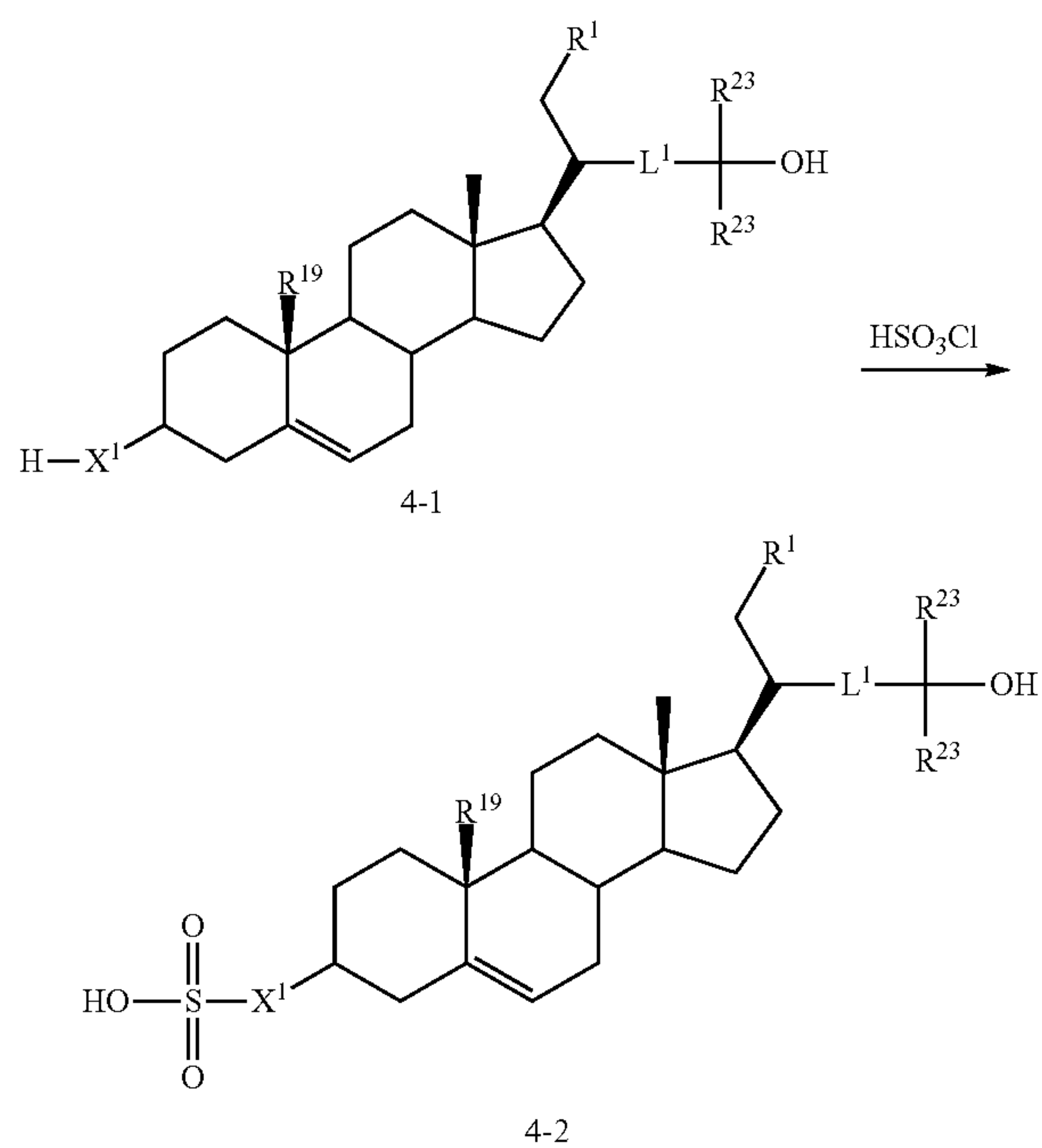
Scheme 4. Synthesis of Steroid sulfates
