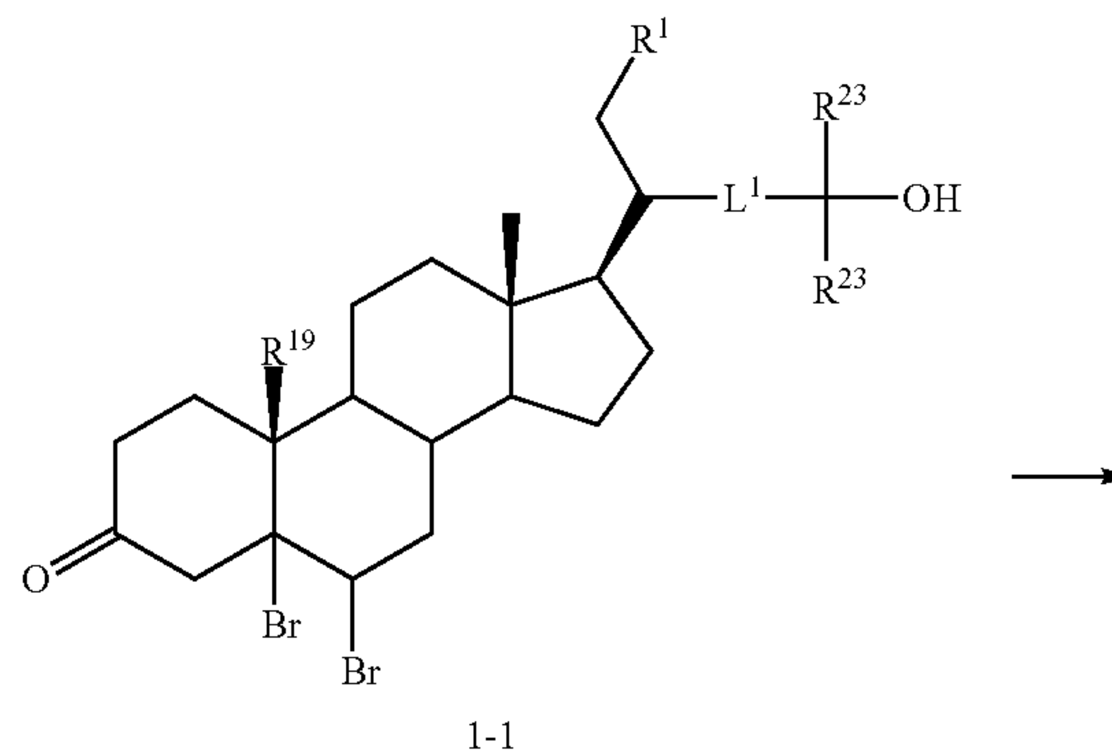
Scheme 2. Synthesis of 3α-Substituted-3β-hydroxy steroids
