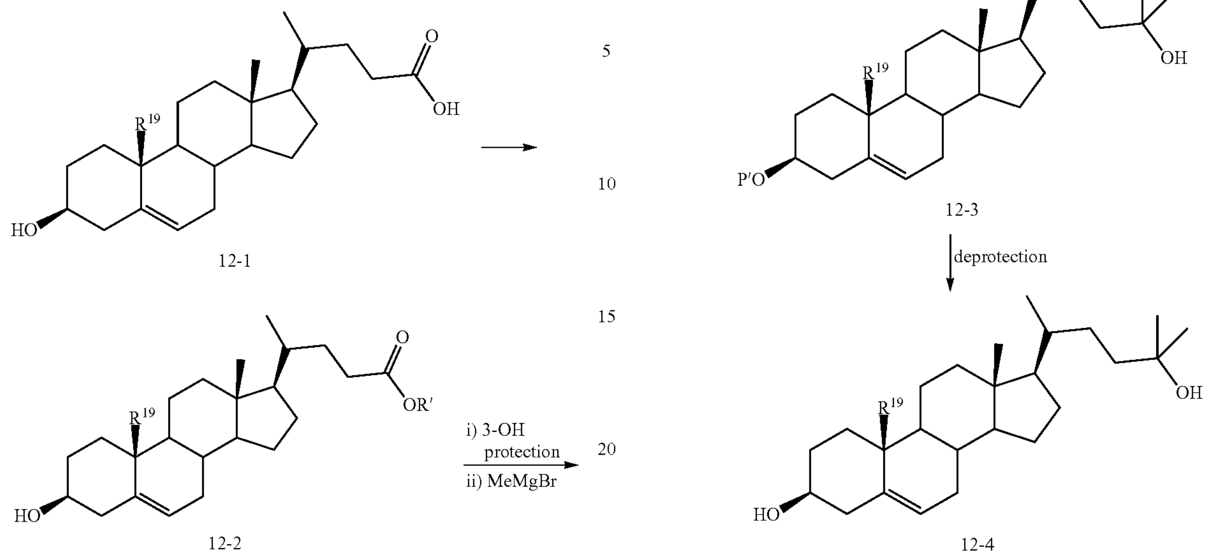
Scheme 12. Synthesis of 3 \alpha -Substituted-3 \beta -hydroxy steroids
