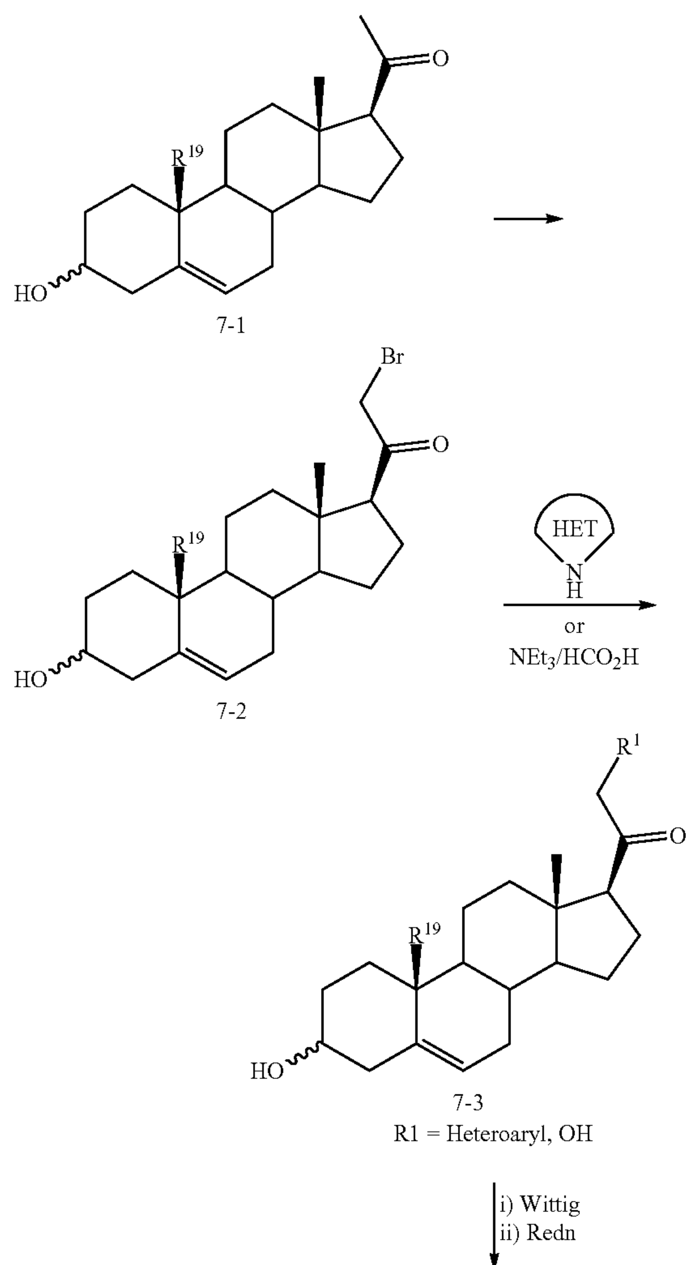
Scheme 7. Synthesis of 21-Heteroaryl-3β-hydroxy steroids
