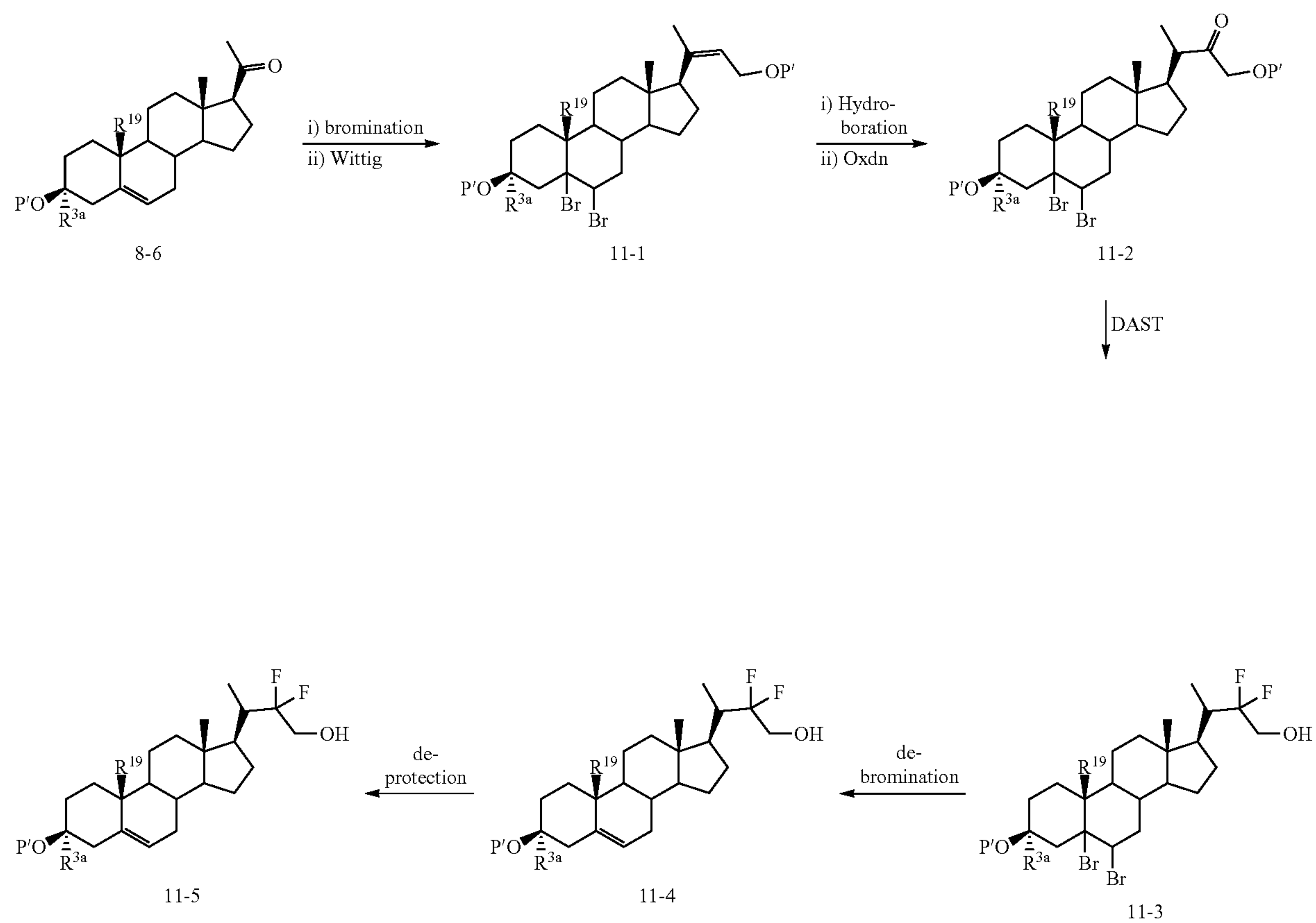
Scheme 11. Synthesis of 3 \alpha -substituted-3 \beta -hydroxy steroids
