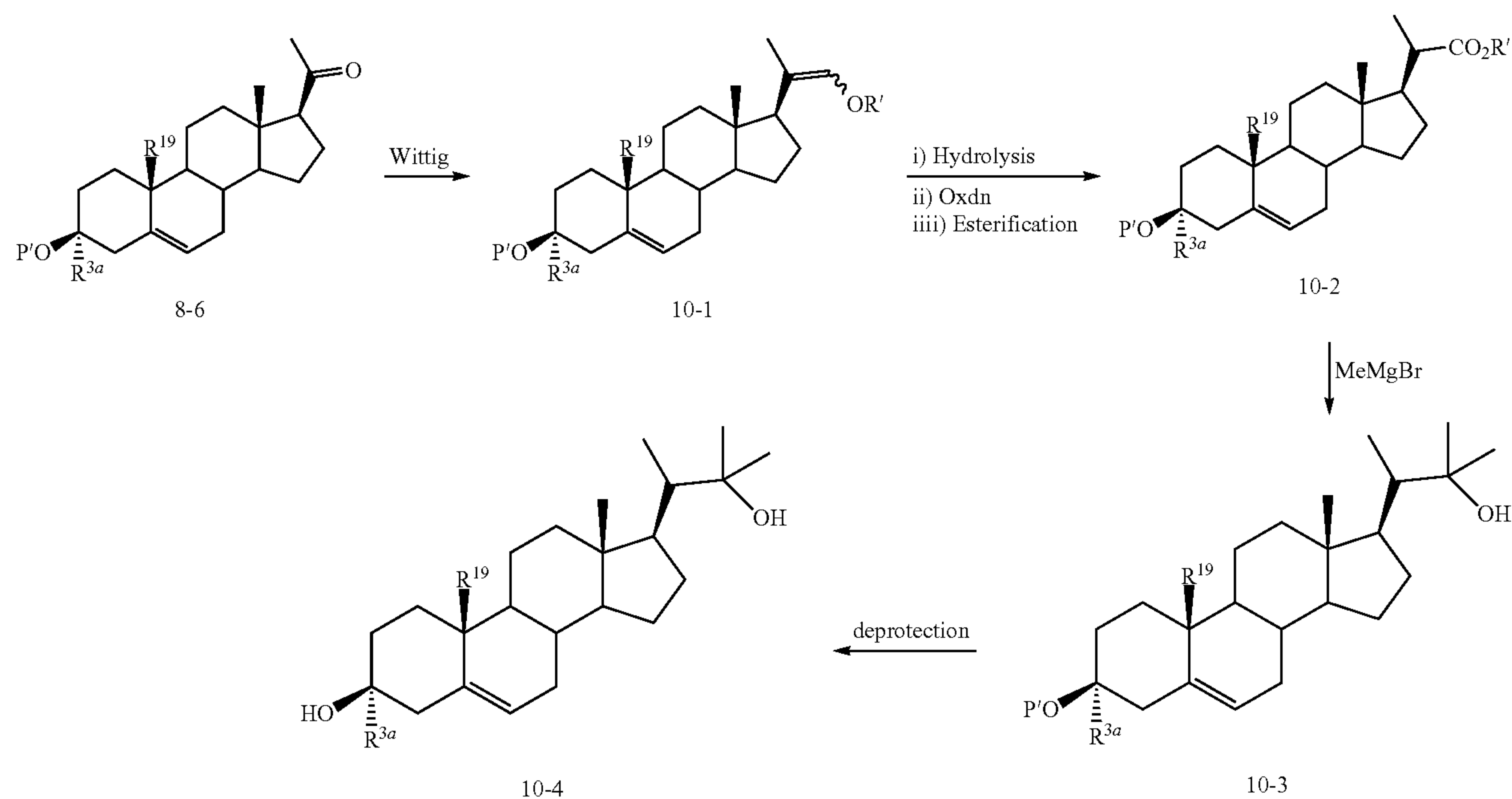
Scheme 10. Synthesis of 3 \alpha -substituted-3 \beta -hydroxy steroids
