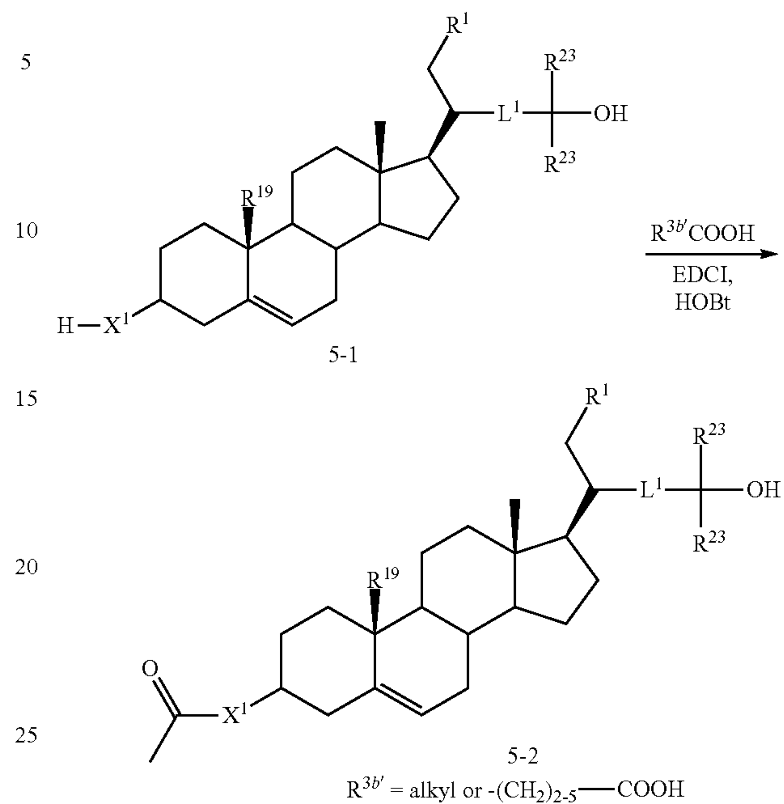
Scheme 5. Synthesis of Steroid 3 \beta -ester and amide
