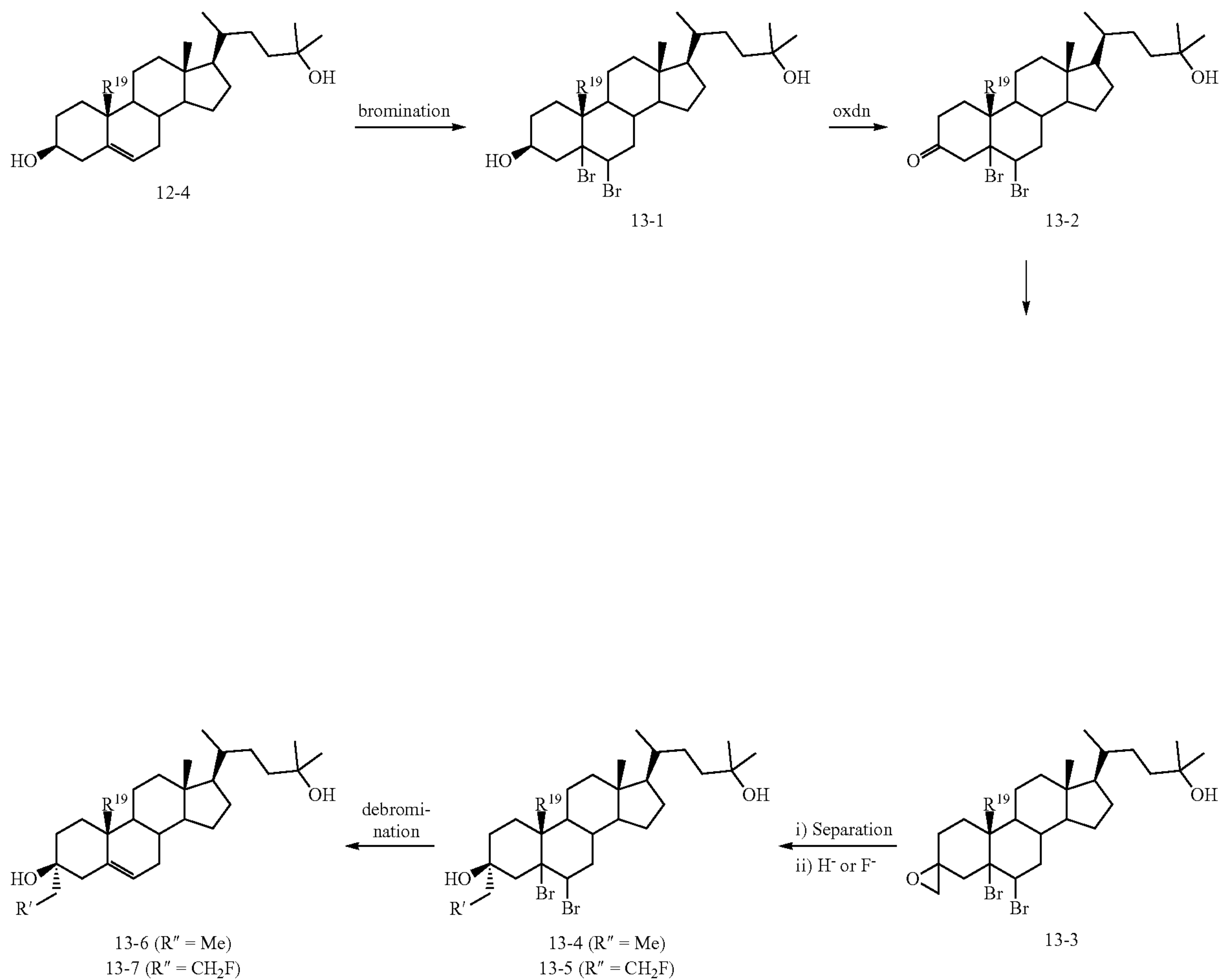
Scheme 13. Synthesis of 3 \alpha -Substituted-3 \beta -hydroxy steroids
