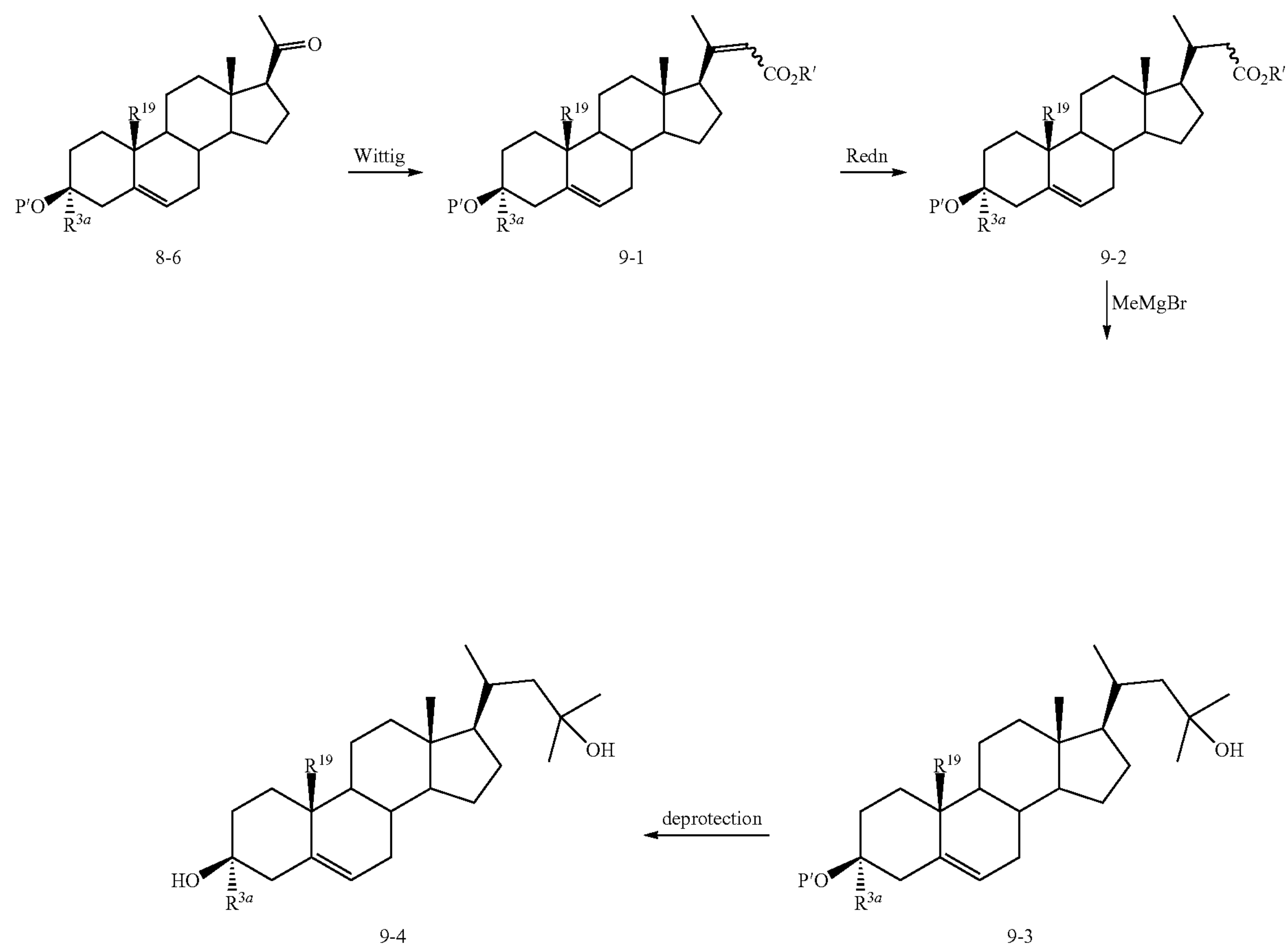
Scheme 9. Synthesis of 3 \alpha -substituted-3 \beta -hydroxy steroids
