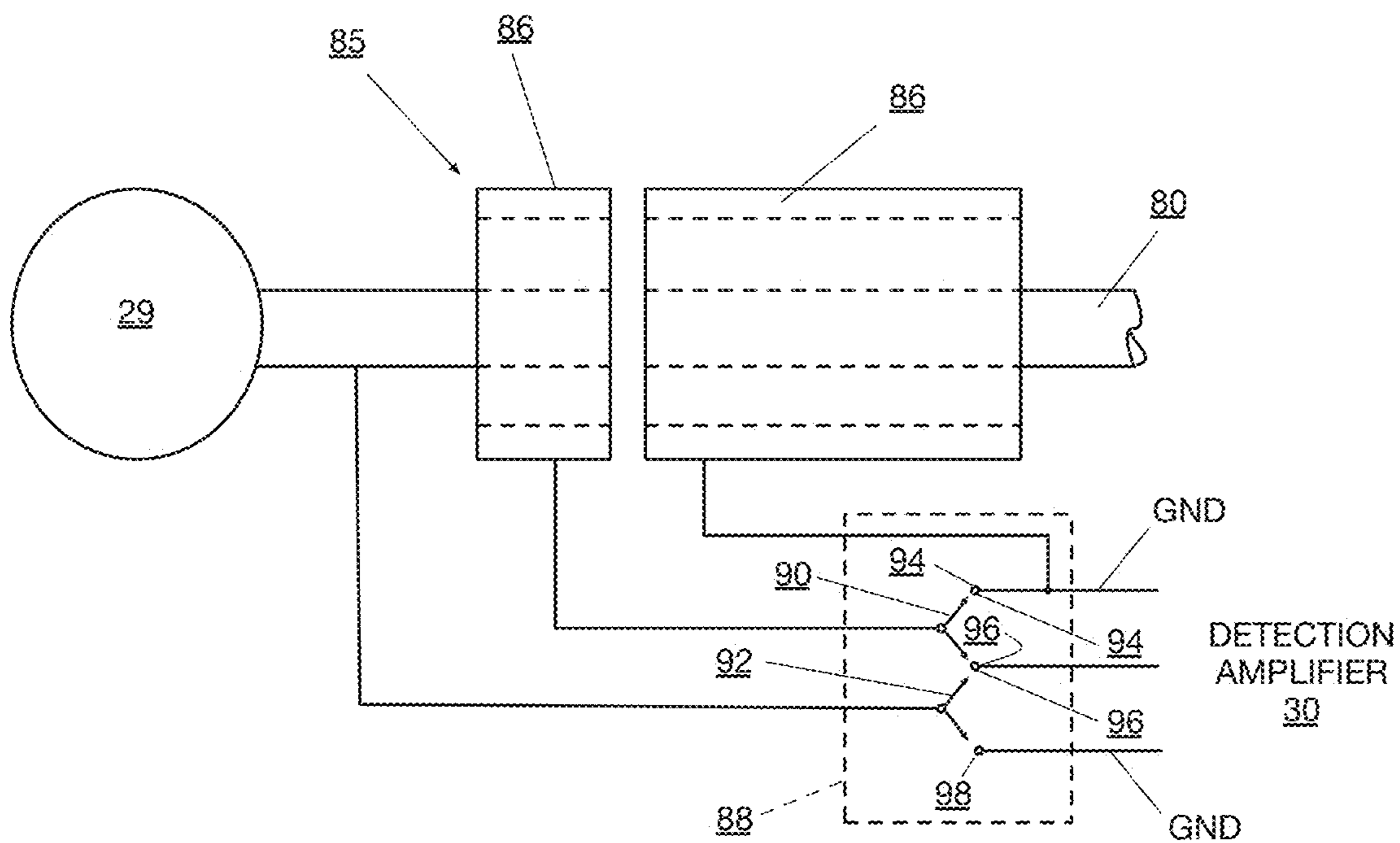
Fig. 42 (PRIOR ART)
