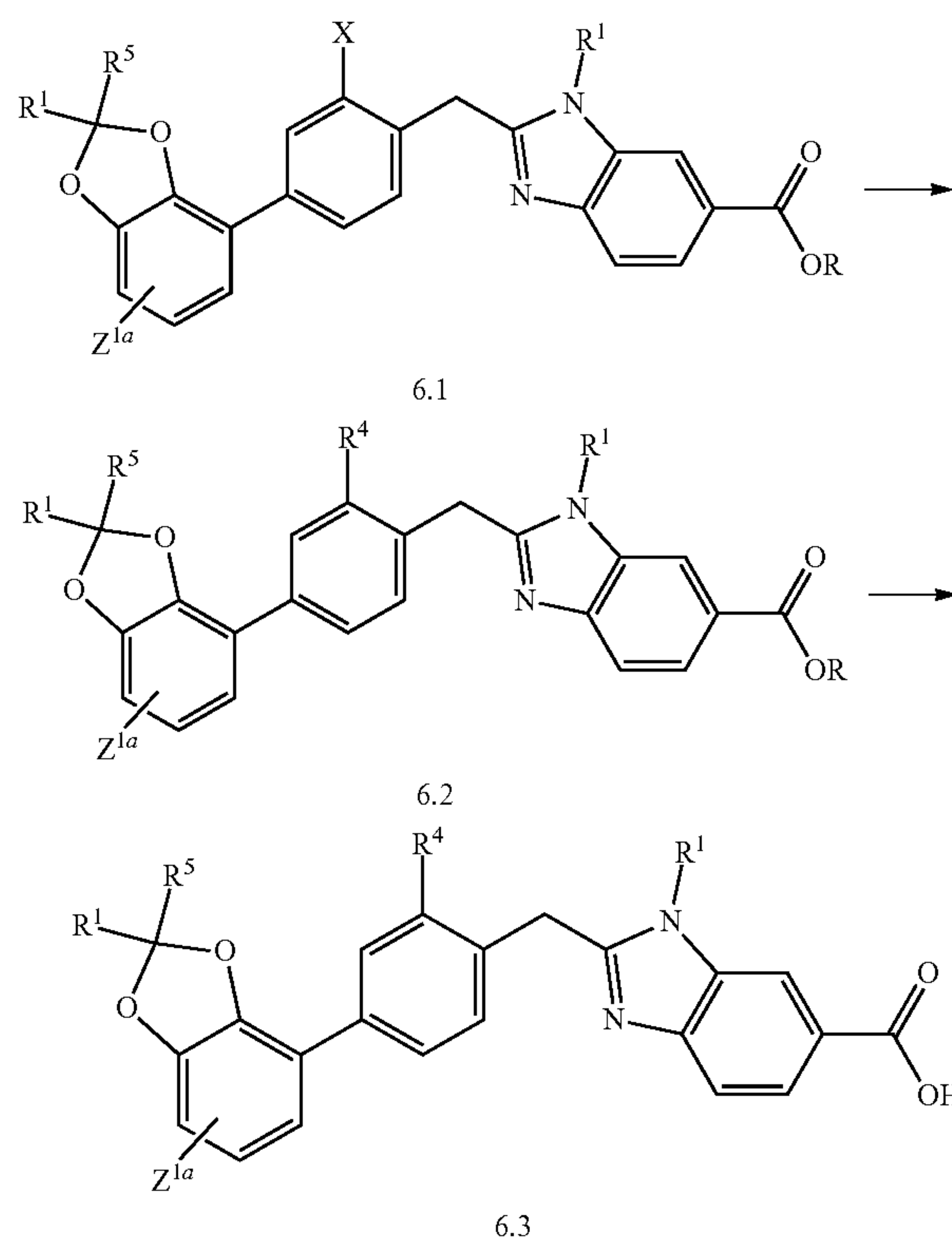
Scheme 6
