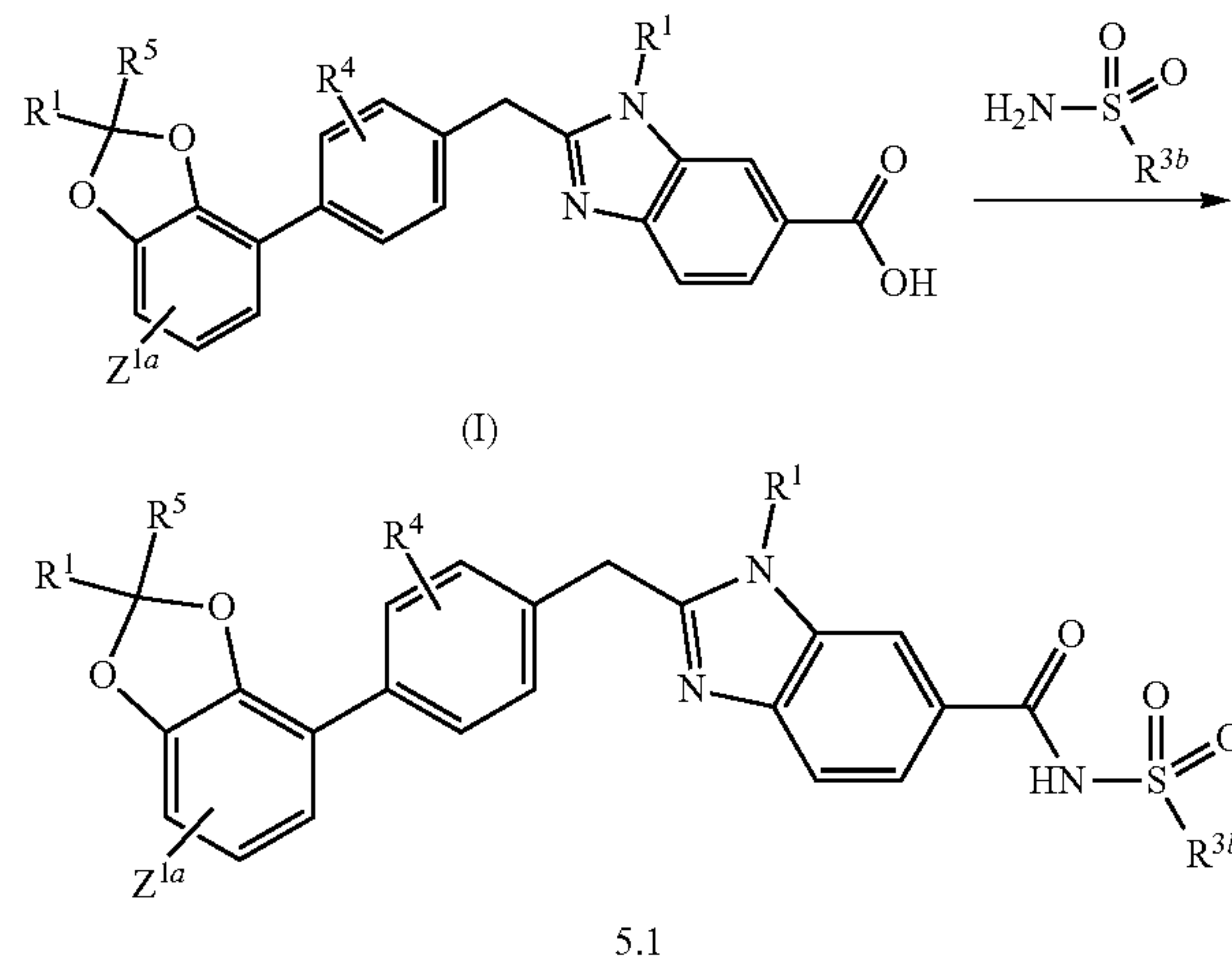
Scheme 5
