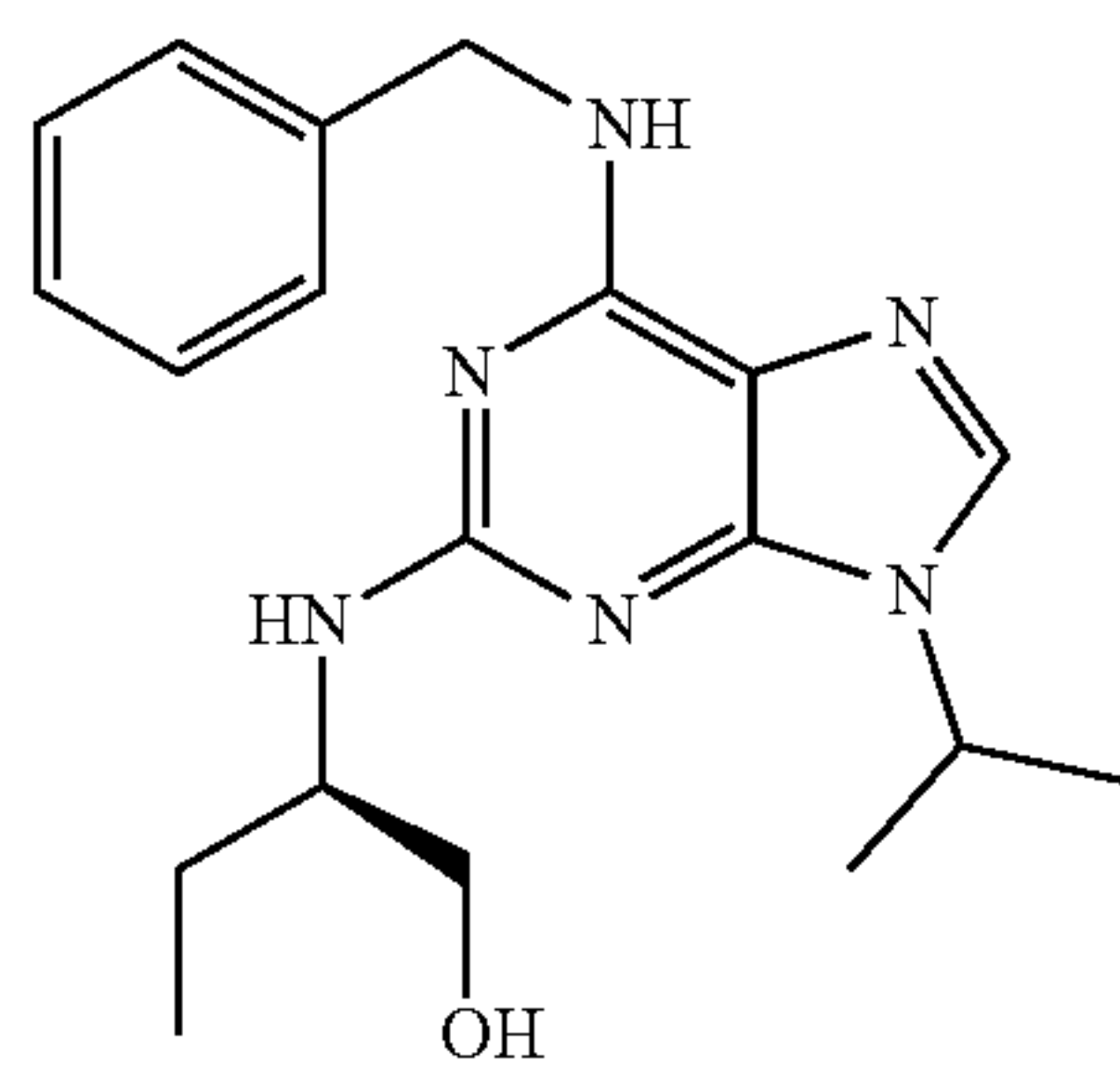
(R)-roscovitine
