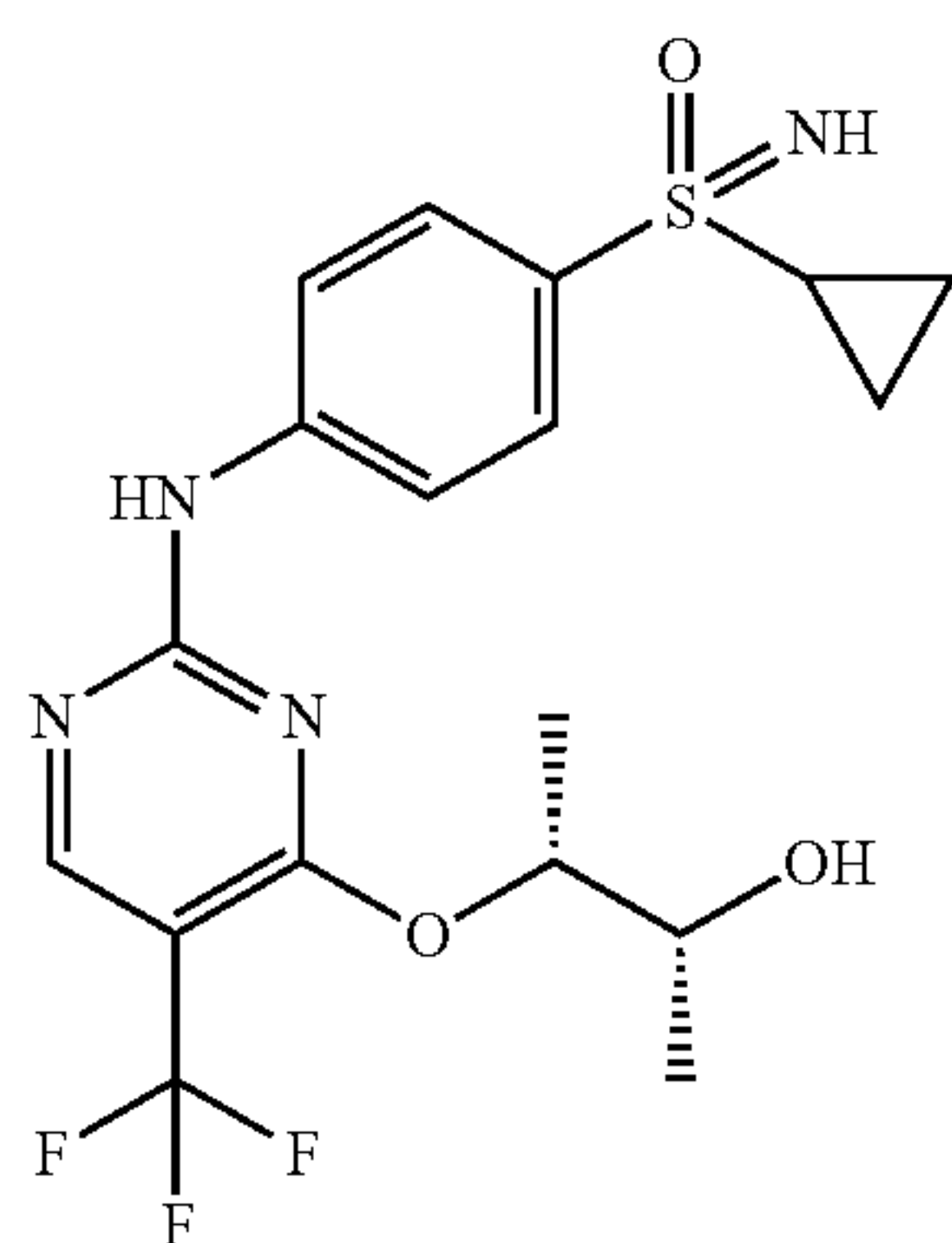
BAY1000394
