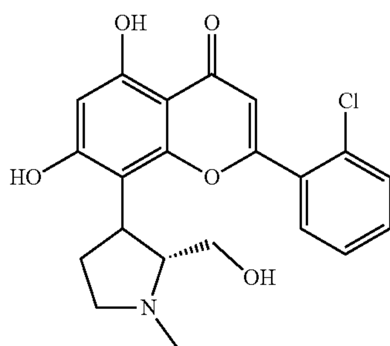
P276-00
