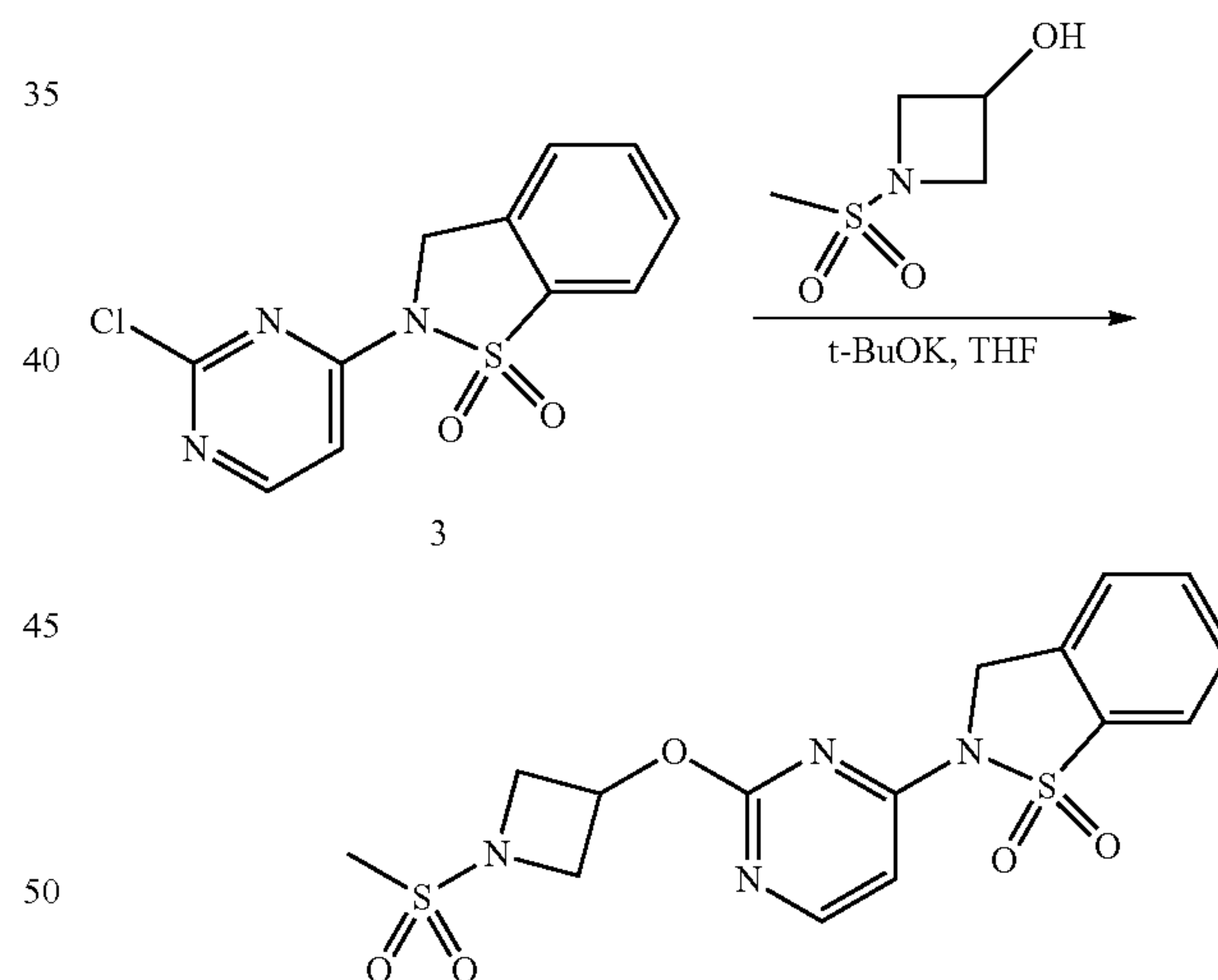
Compound 109
