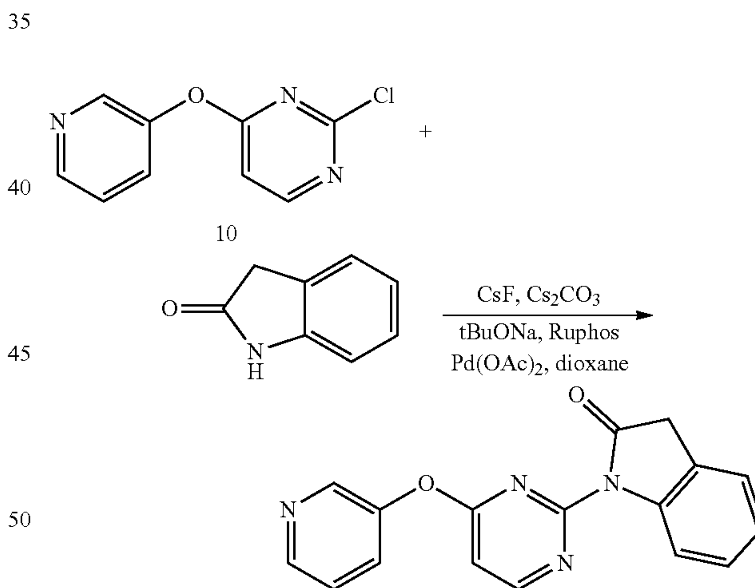
Compound 120
