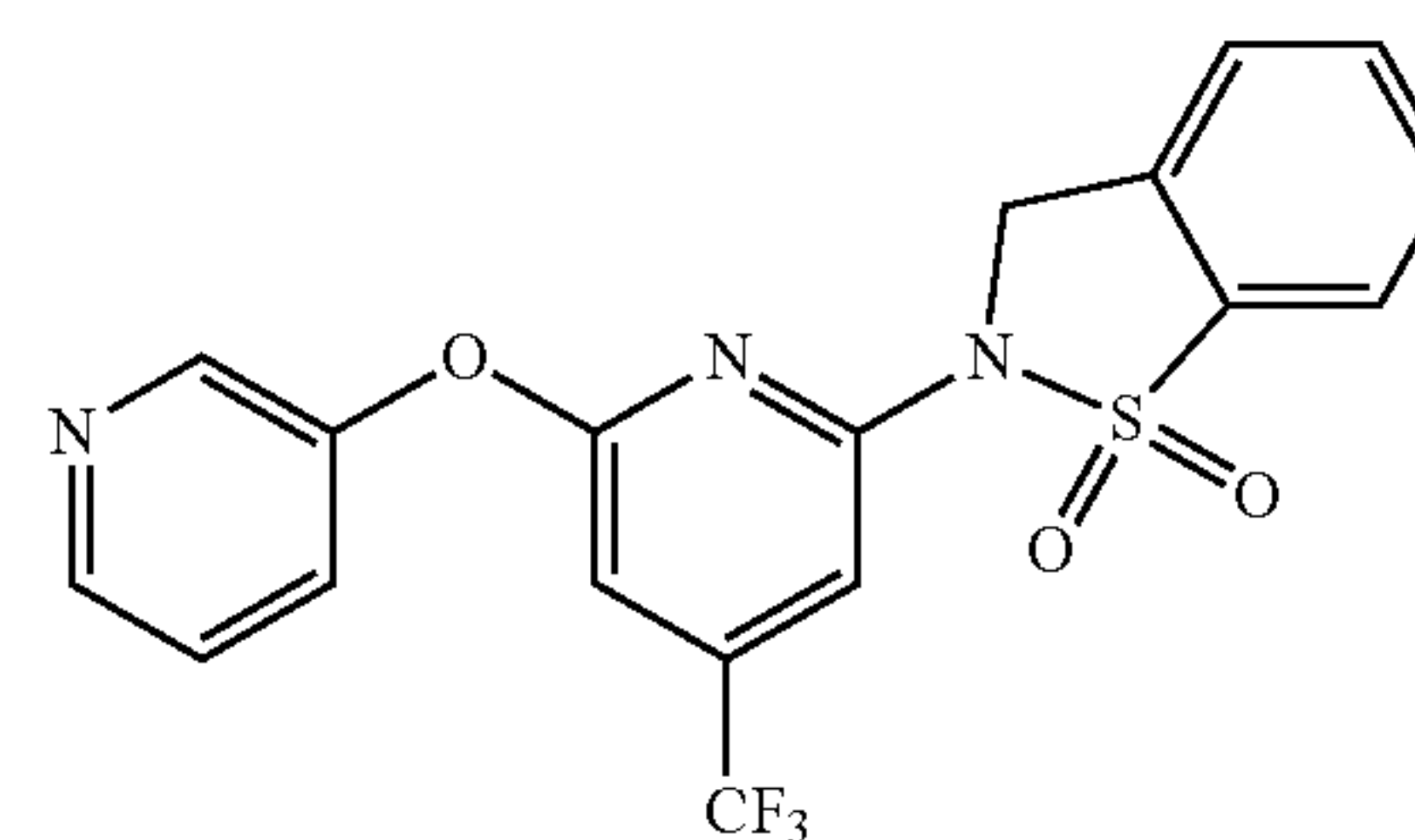
Compound 140
