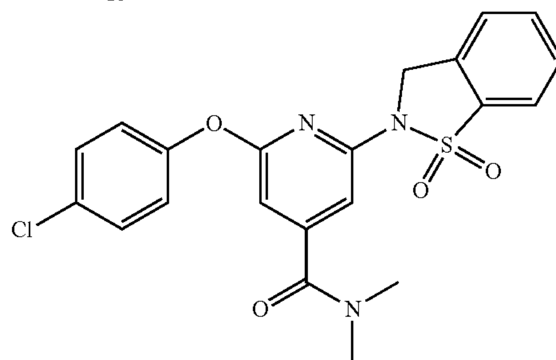
Compound 139
