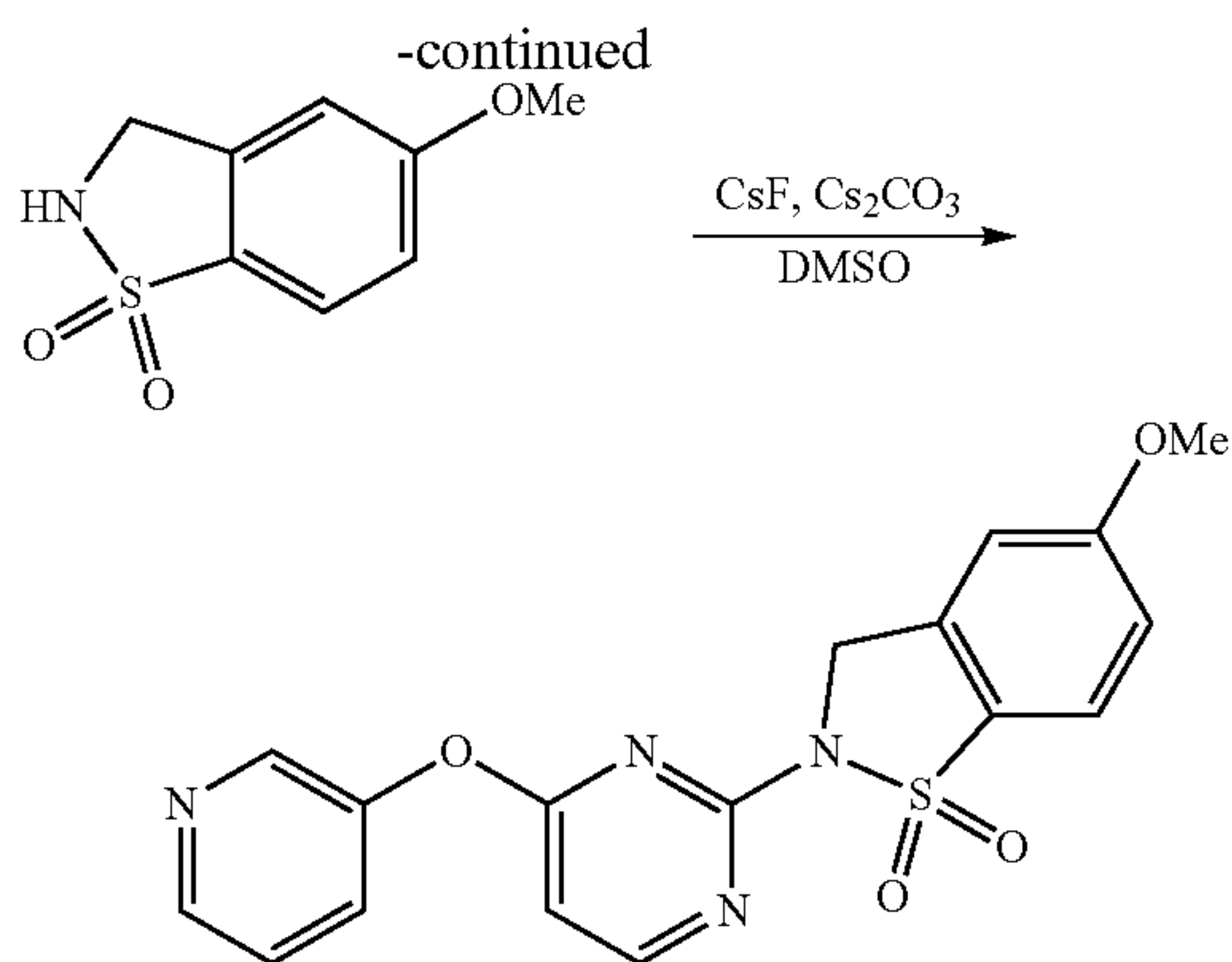
Compound 116
