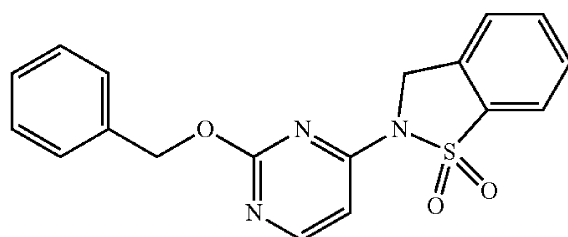
Compound 70
