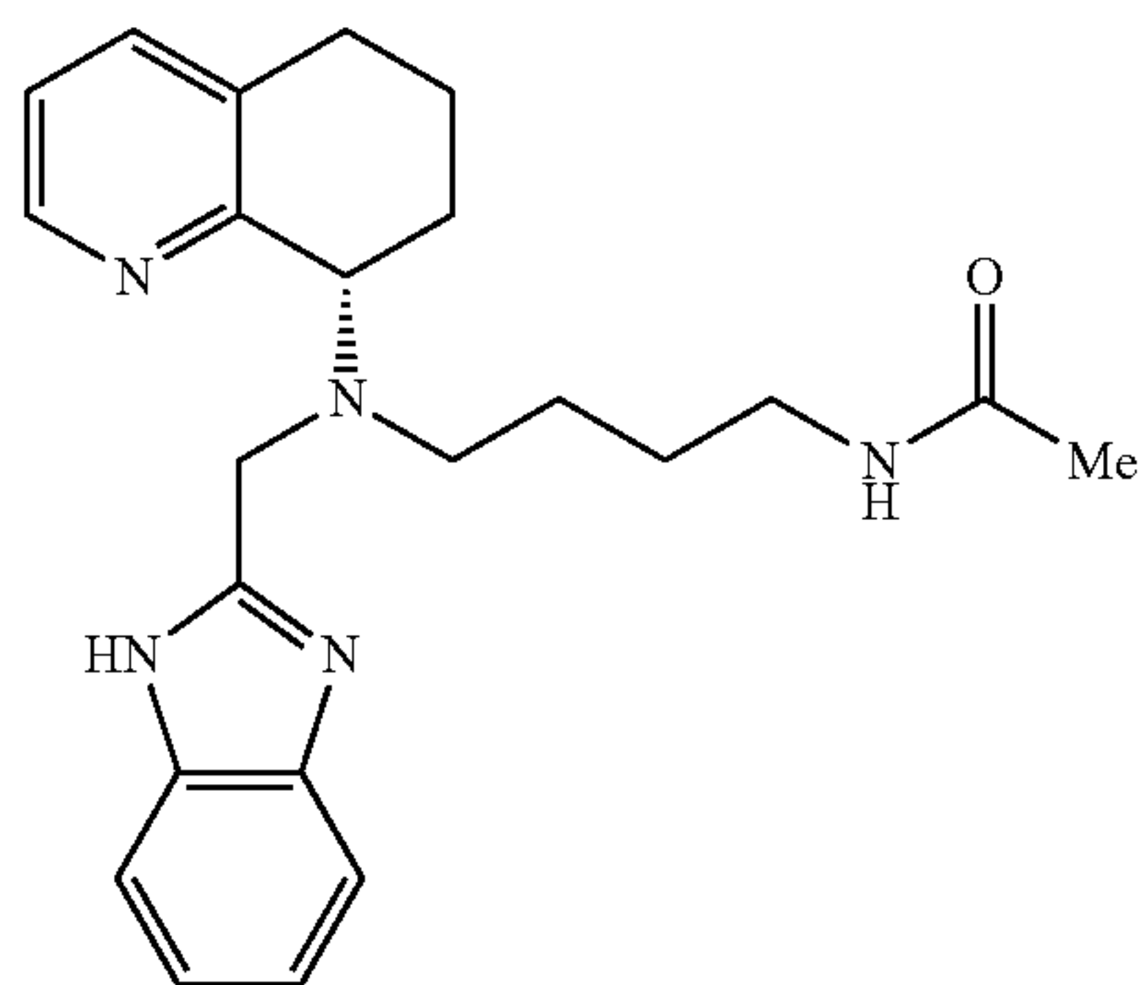
acetamide C
