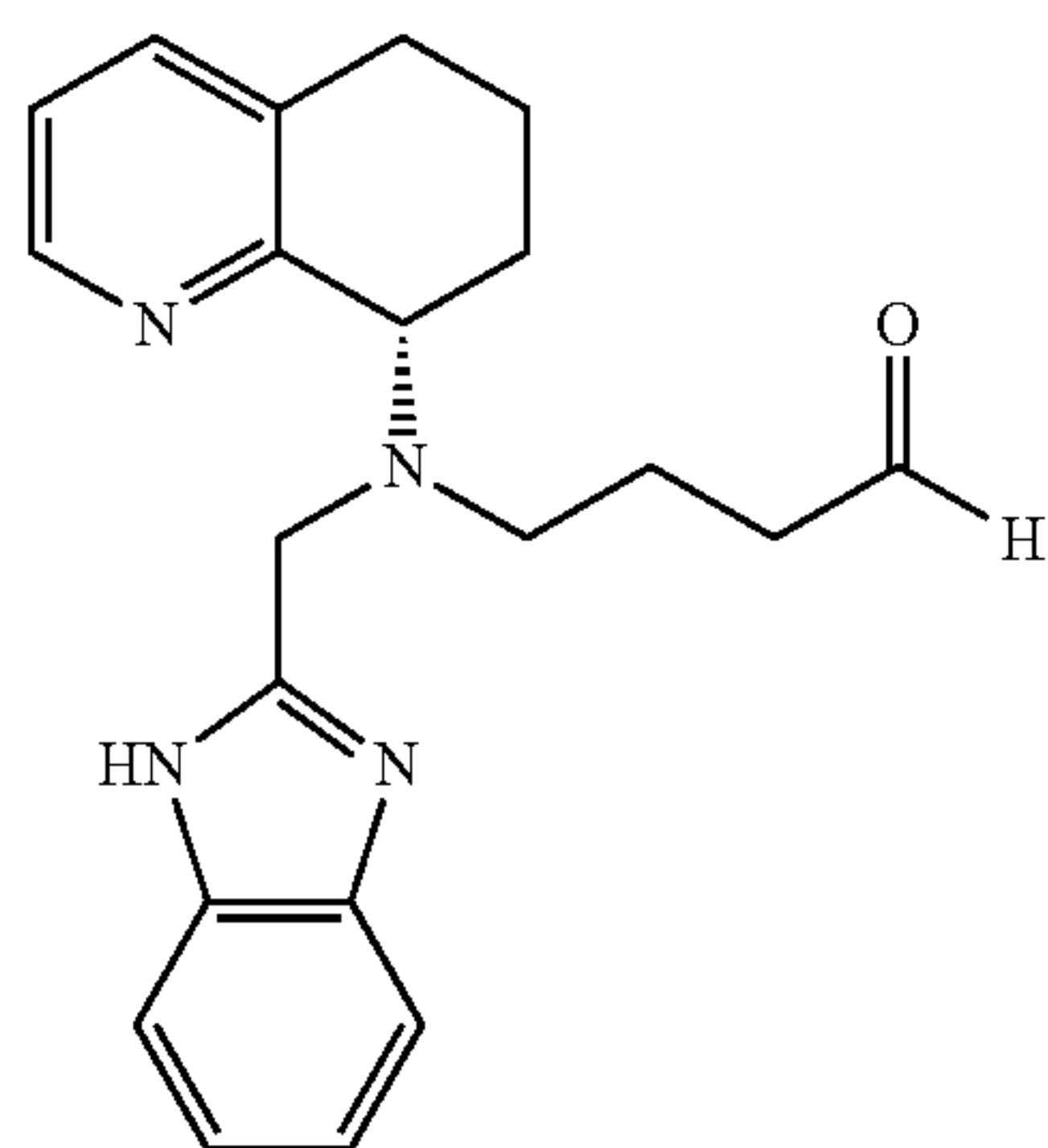
aldehyde D
