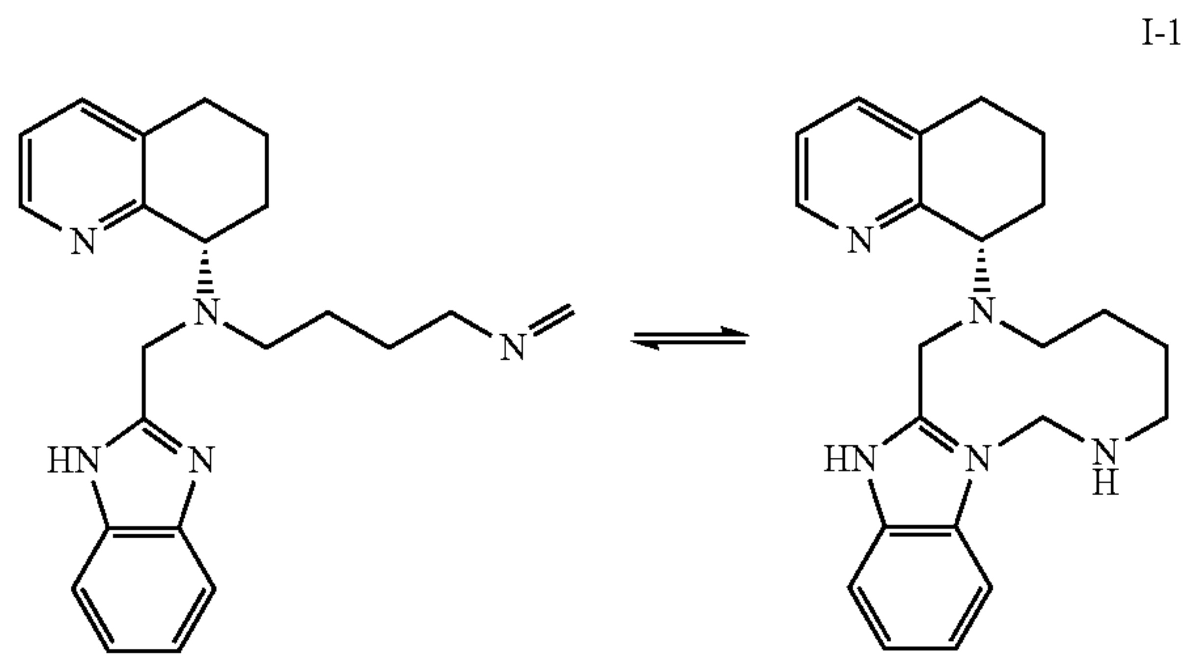
imine A
