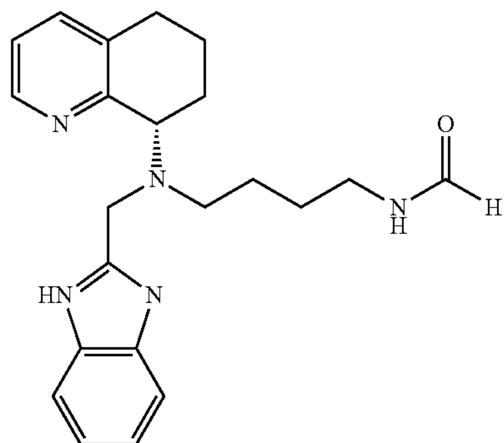
formyl B
