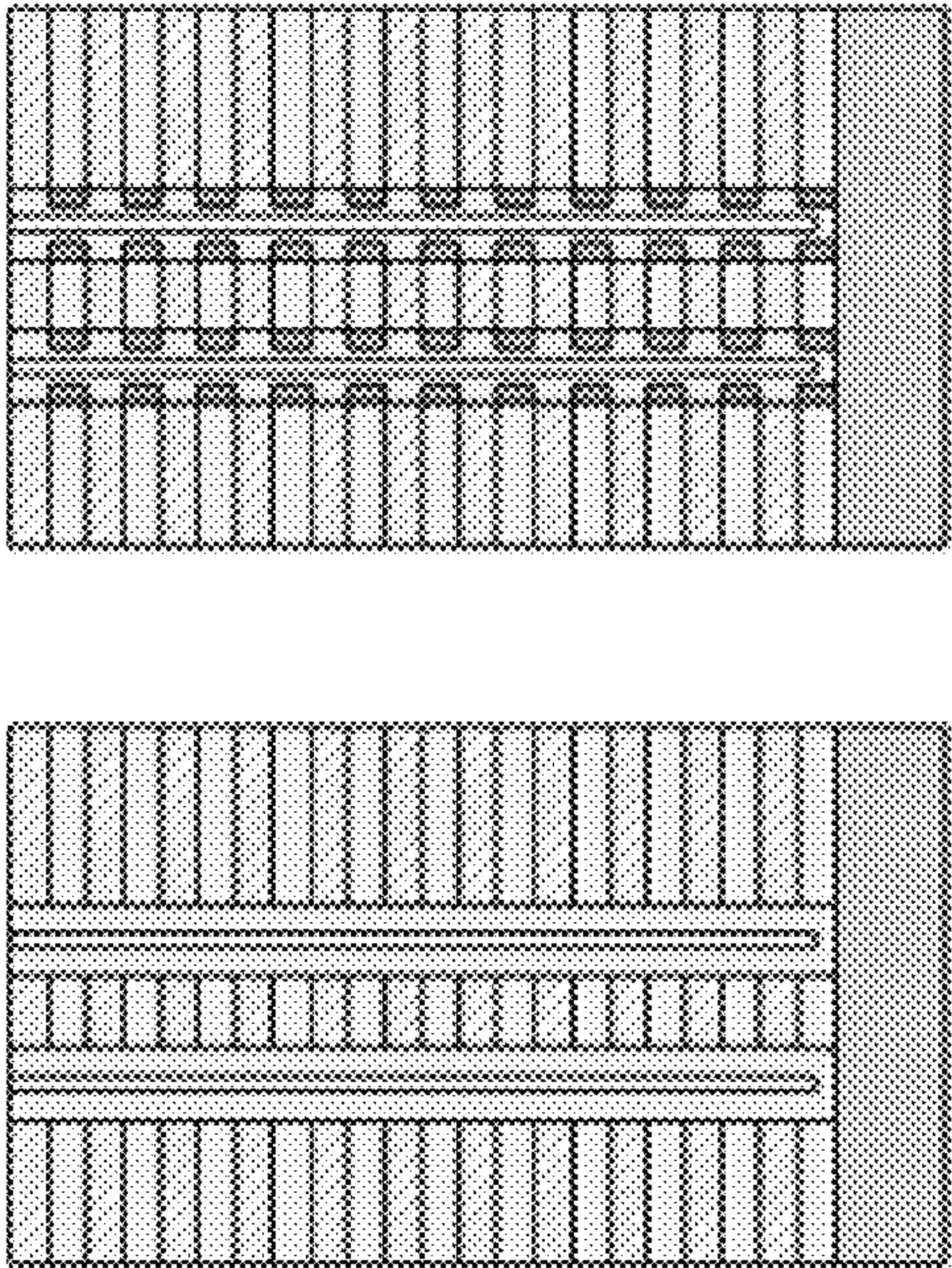
Fig. 4A P doped silicate/Nitride stack Vertical hole for channel
