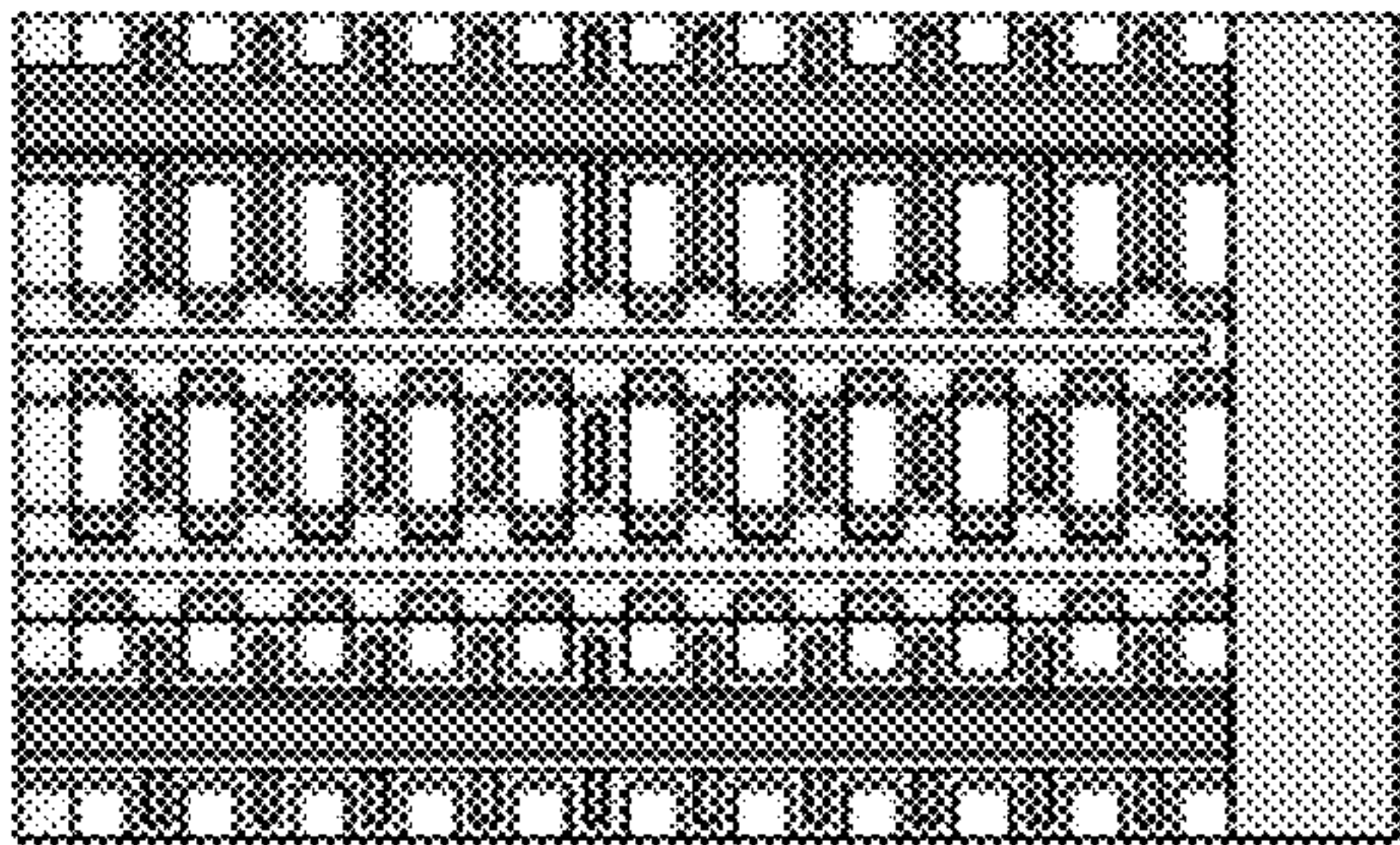
Fig. 4H SiO2 fill and source line contact
