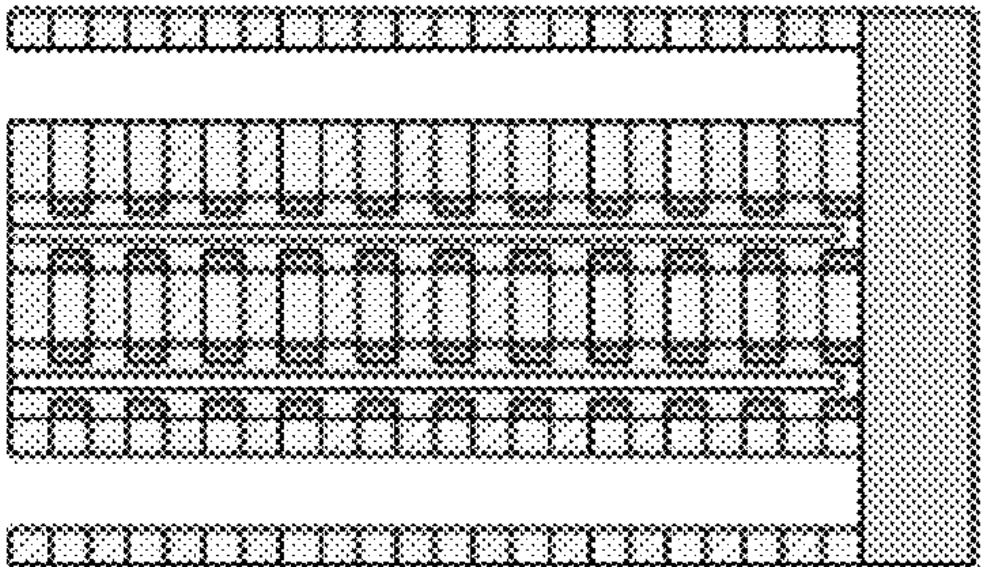
Fig. 4A P doped silicate/Nitride stack Vertical hole for channel
