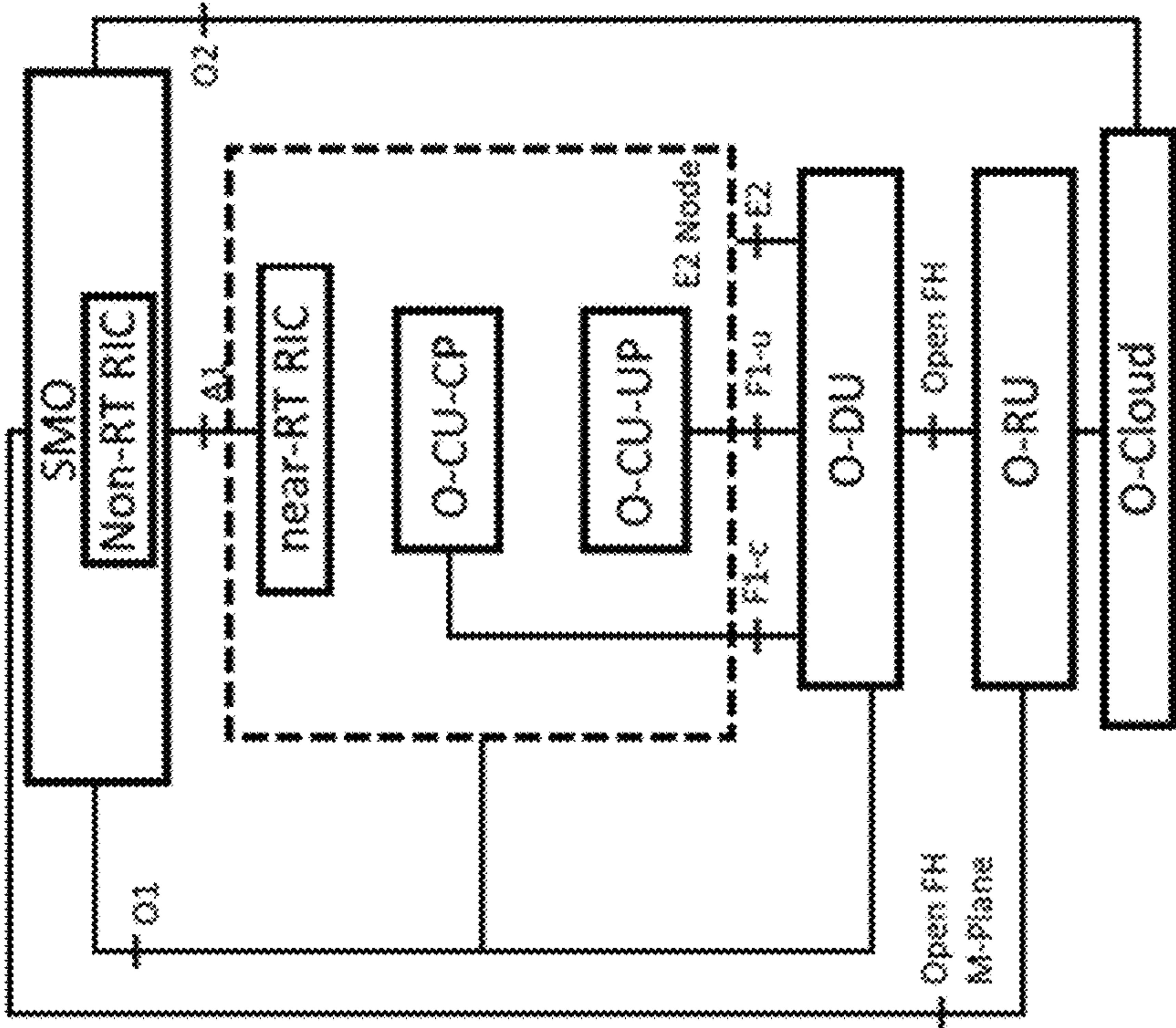
Aggregated near-RT RIC, O-CU-CP, O-CU-UP
