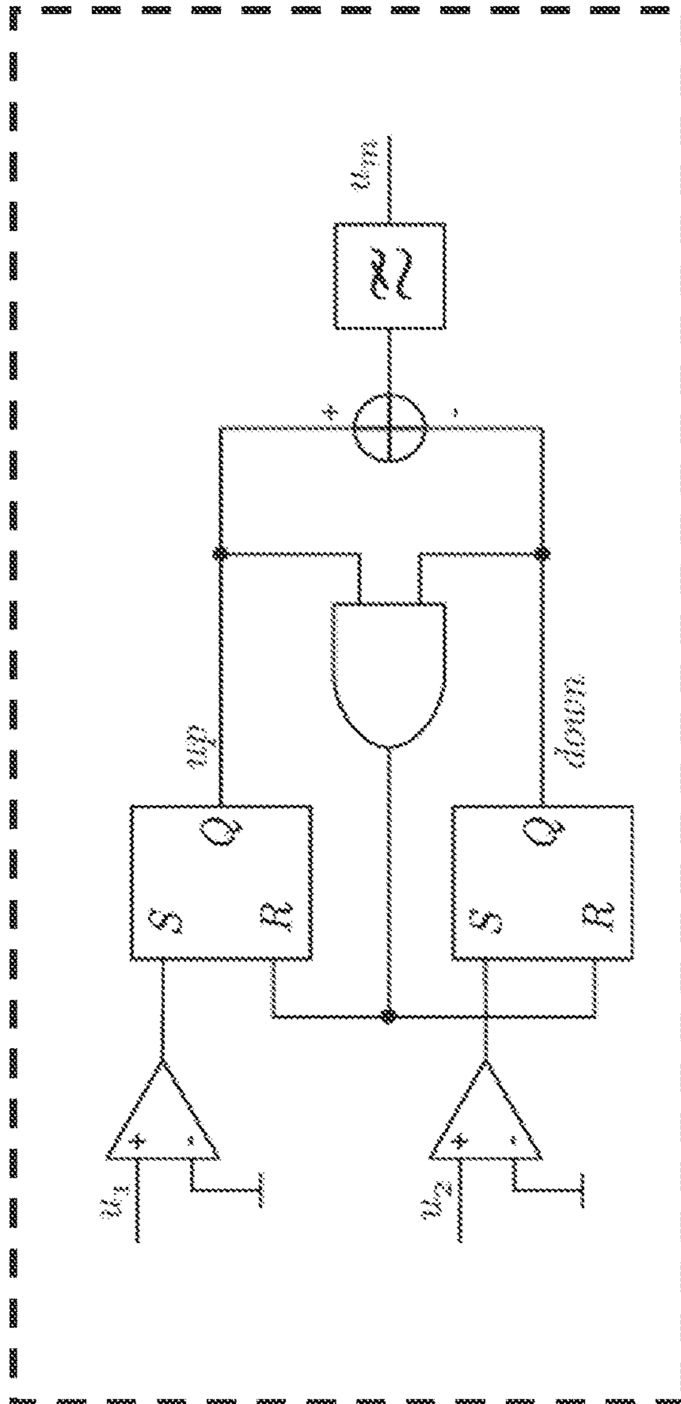
Phase Detector 2206''
