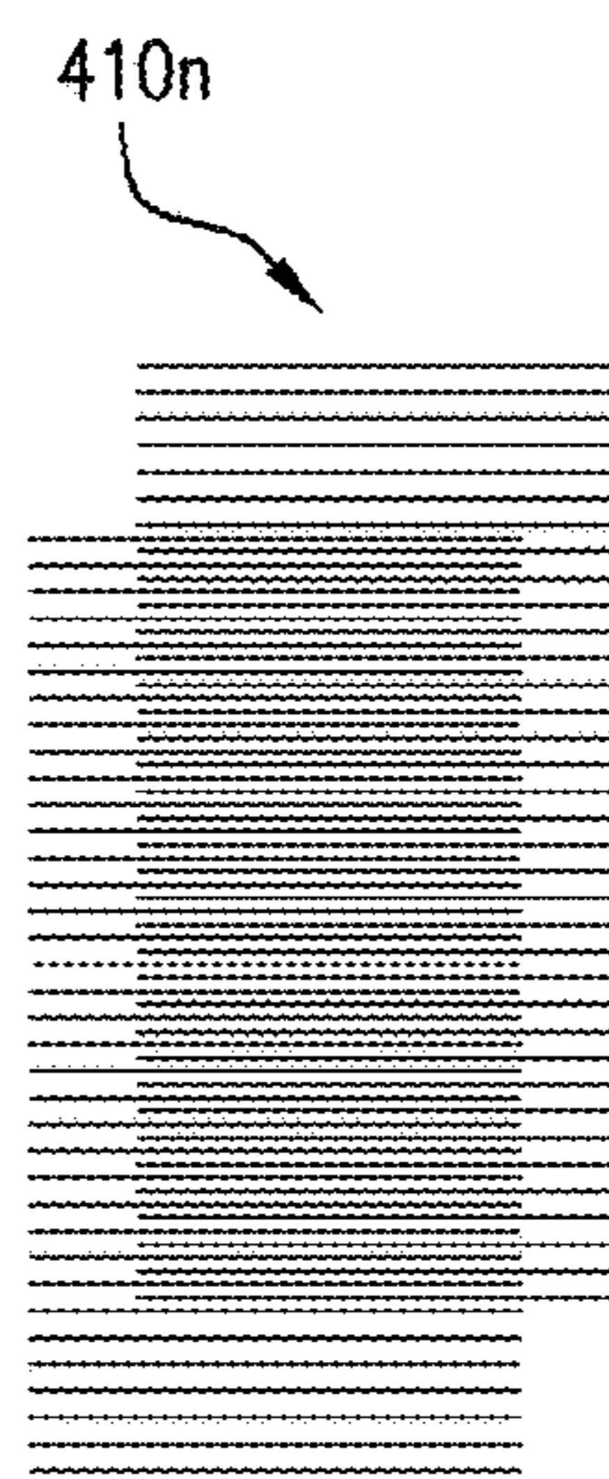
Moiré pattern
