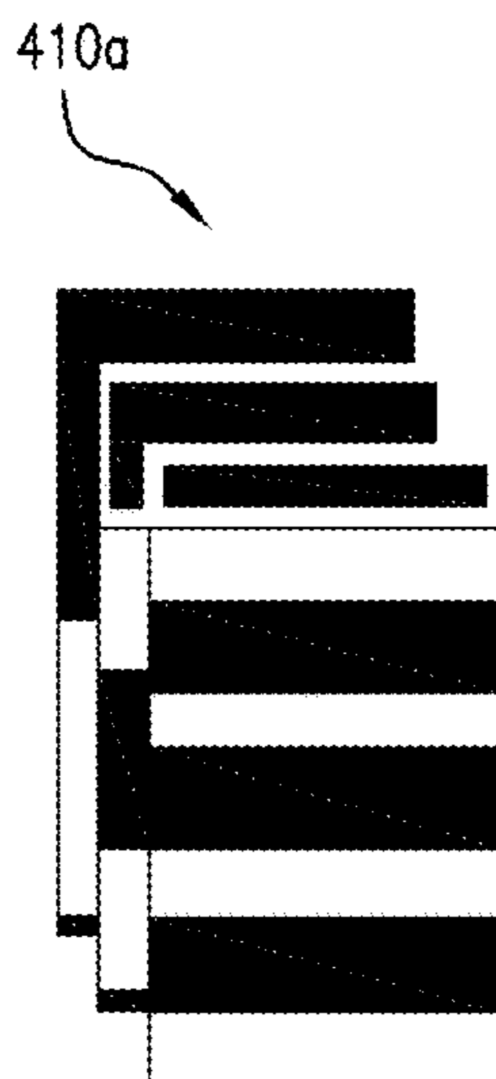
Binary code
