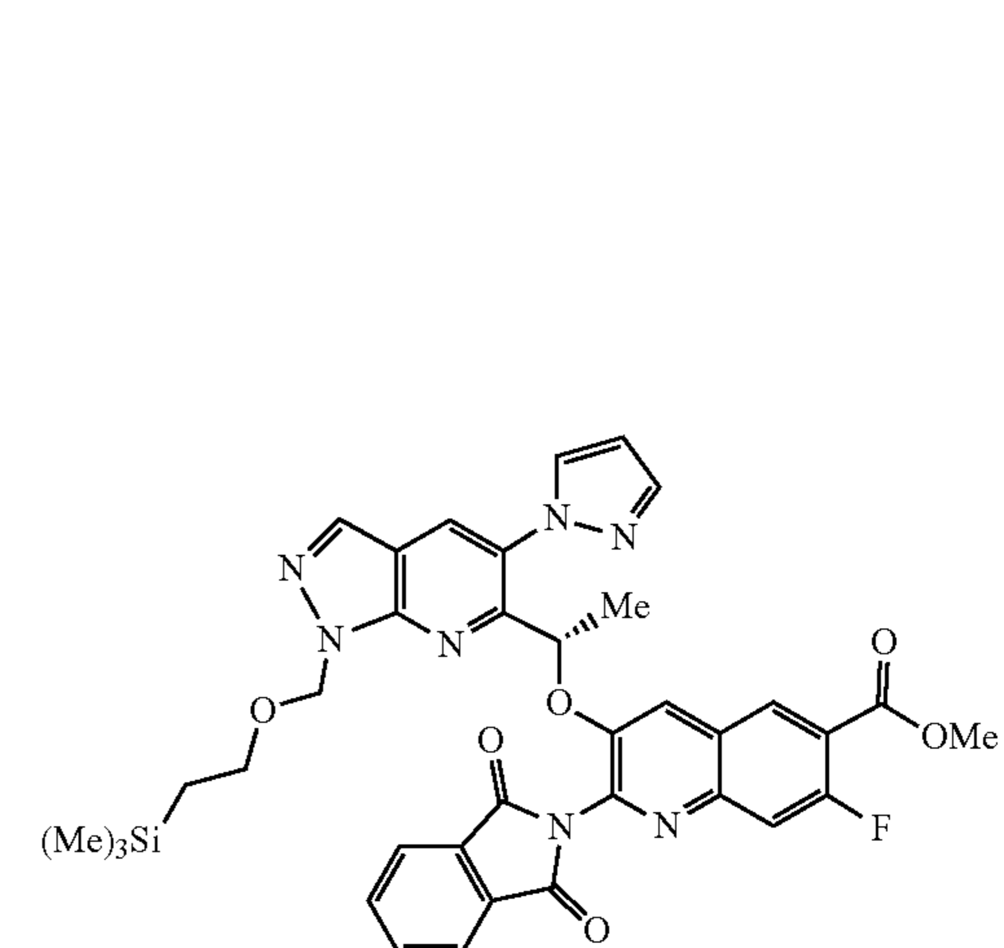
tert-butyl (7-methyl-3-{(1S)-1-[5-(1H-pyrazol-1-yl)-1-{2-(trimethylsilyl)ethoxy}methyl]-1H-pyrazolo[3,4-b]pyridin-6-yl}ethoxy)-1,6-naphthyridin-2-yl}carbamate, a yellow gum in quantitative yield. LCMS m/z = 617 [M + H]^+
