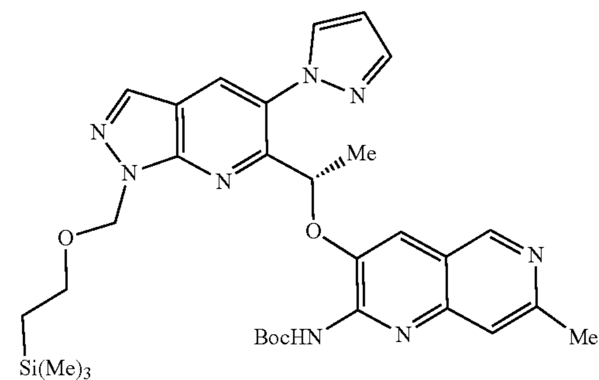
tert-butyl (7-methyl-3-{(1S)-1-[5-(1H-pyrazol-1-yl)-1-{2-(trimethylsilyl)ethoxy}methyl]-1H-pyrazolo[3,4-b]pyridin-6-yl}ethoxy)-1,6-naphthyridin-2-yl}carbamate, a yellow gum in quantitative yield. LCMS m/z = 617 [M + H]^+
