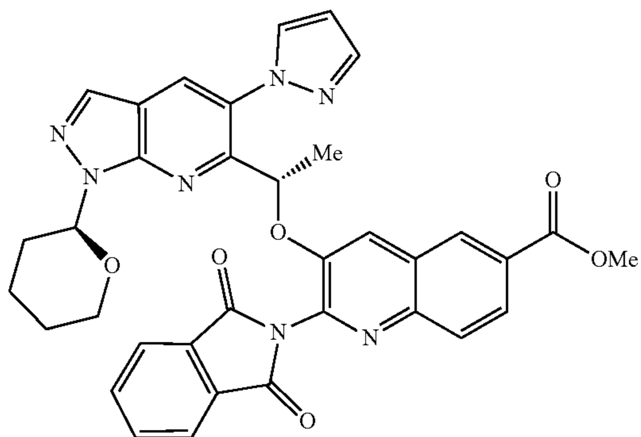
methyl 2-(1,3-dioxo-1,3-dihydro-2H-isoindol-2-yl)-3-[(1S)-1-{5-(1H-pyrazol-1-yl)-1-[(2S)-tetrahydro-2H-pyran-2-yl]-1H-pyrazolo[3,4-b]pyridin-6-yl}ethoxy]quinoline-6-carboxylate, a yellow gum in quantitative yield. LCMS m/z = 644 [M + H]^+
