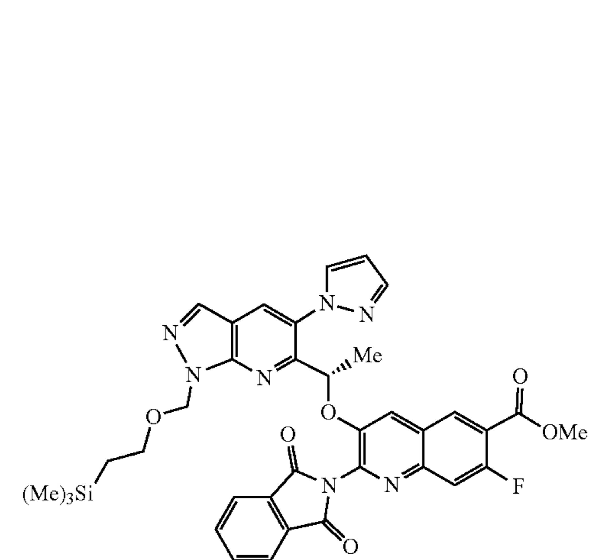
methyl 2-(1,3-dioxo-1,3-dihydro-2H-isoindol-2-yl)-7-fluoro-3-{(1S)-1-[5-(1H-pyrazol-1-yl)-1-{2-(trimethylsilyl)ethoxy}methyl]-1H-pyrazolo[3,4-b]pyridin-6-yl}ethoxy}quinoline-6-carboxylate, a green gum LCMS m/z = 730 [M + Na]^+
