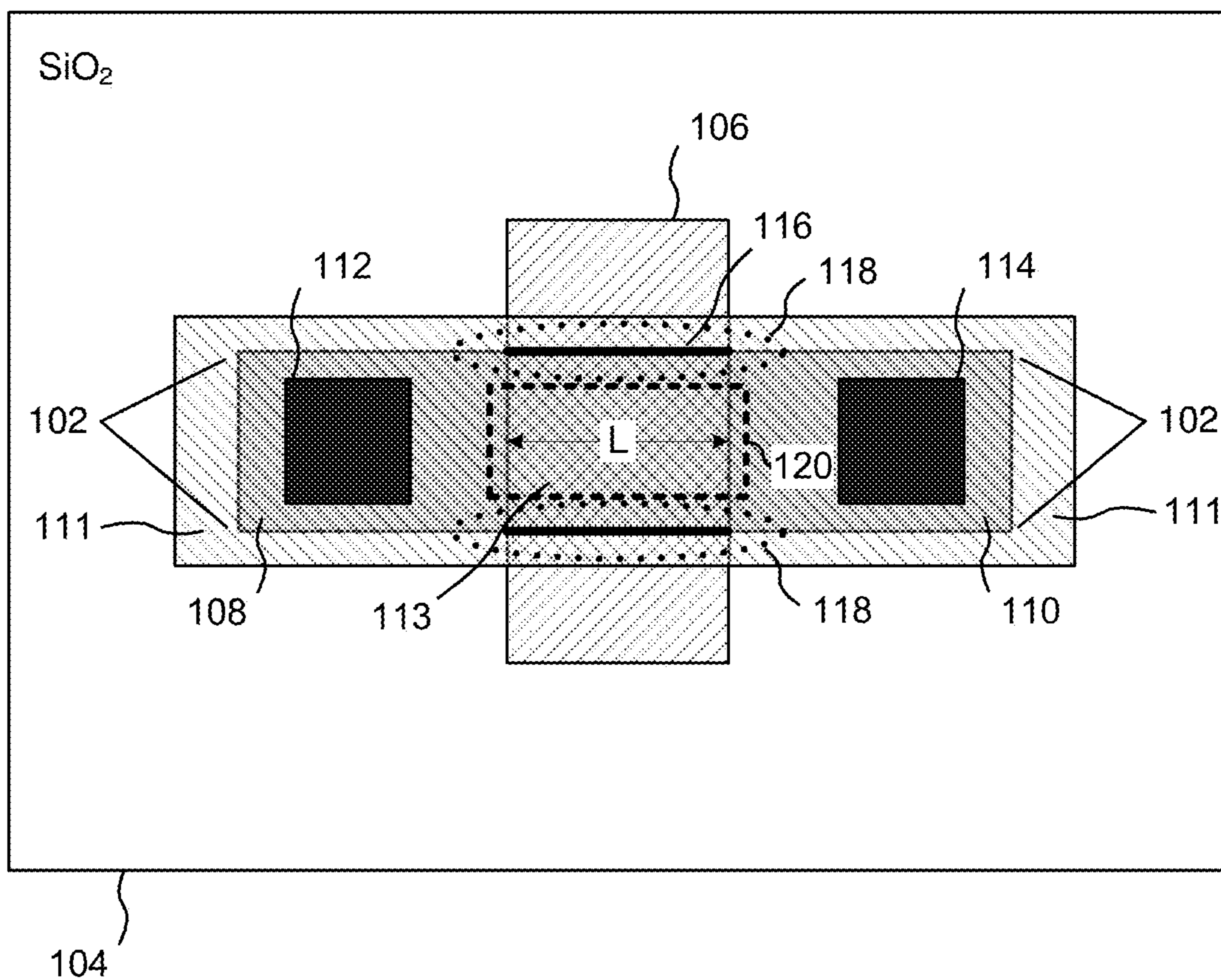
FIG. 1 (Prior Art)
