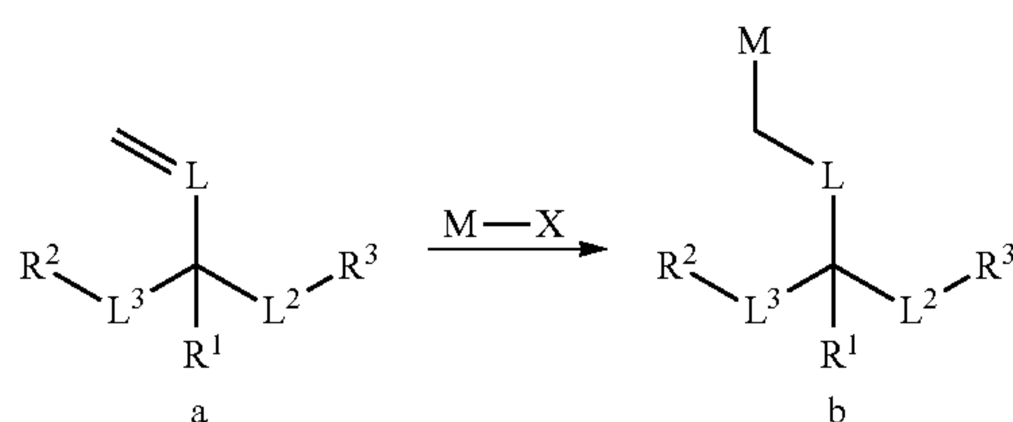
Reaction Scheme I
