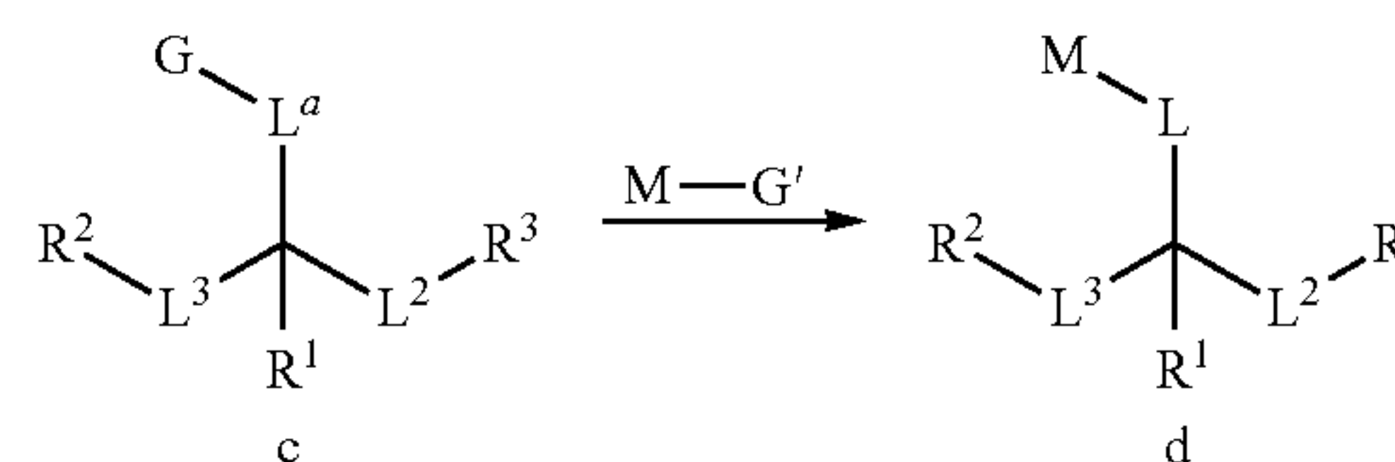
Reaction Scheme II
