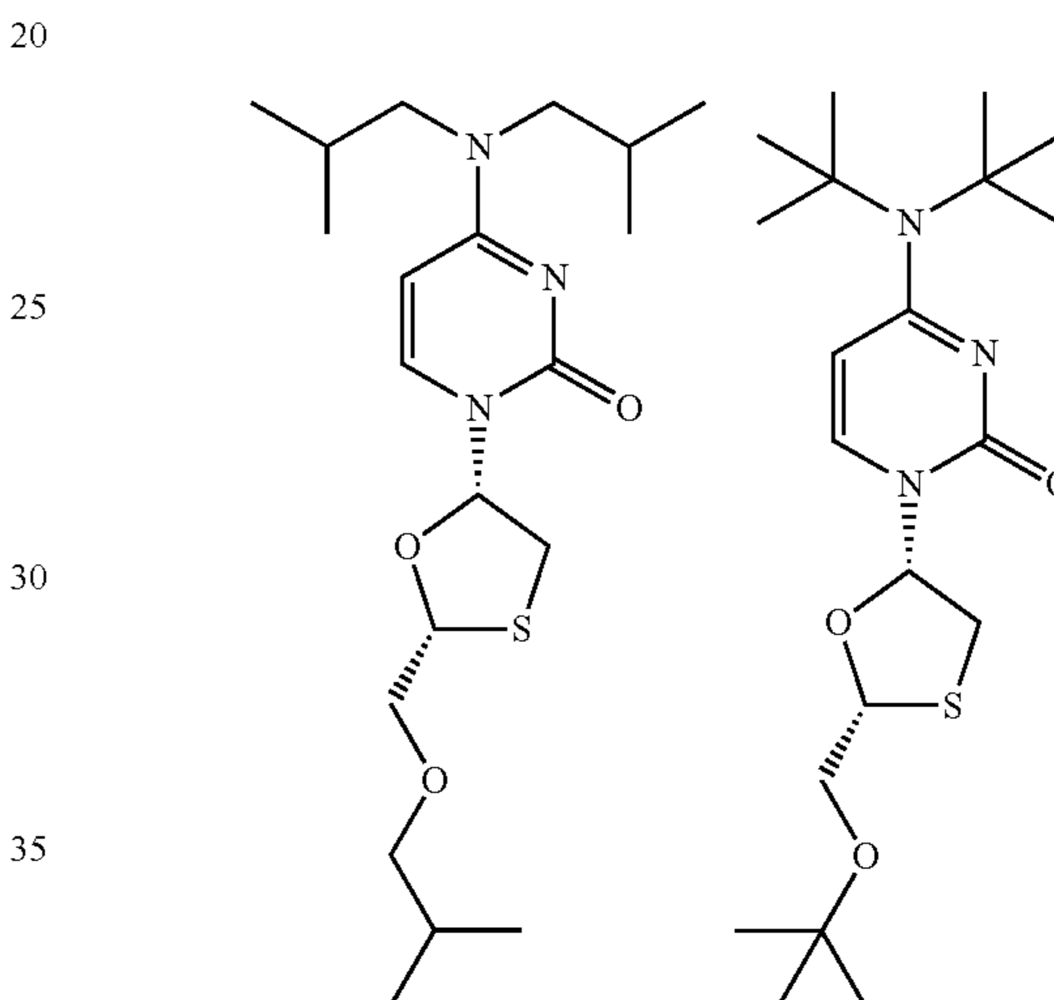
3-Isobutyl-3TC
