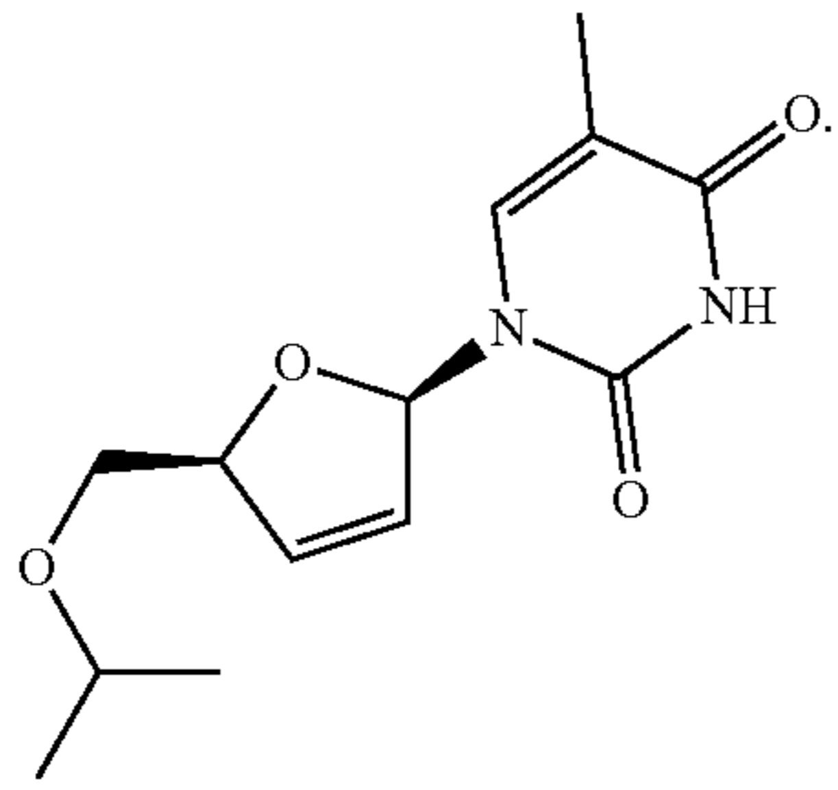
O-isopropyl-d4T
