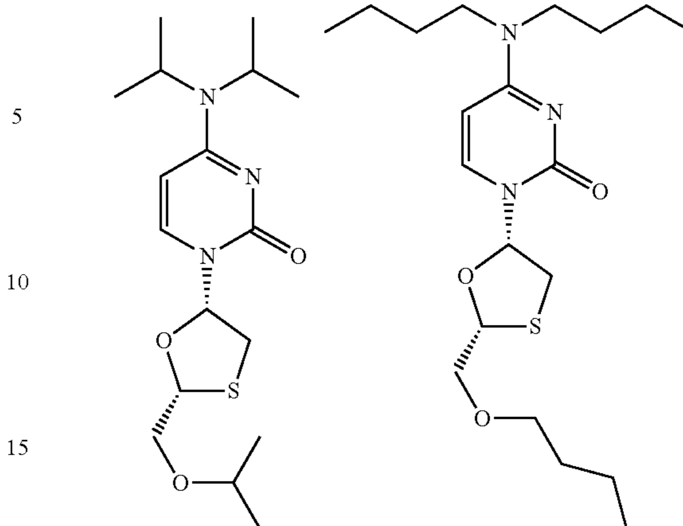
3-Isopropyl-3TC
