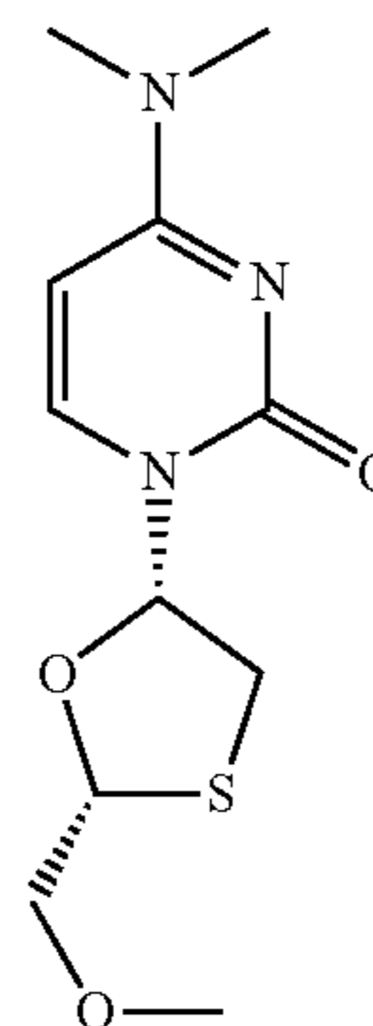
3-Me-3TC
