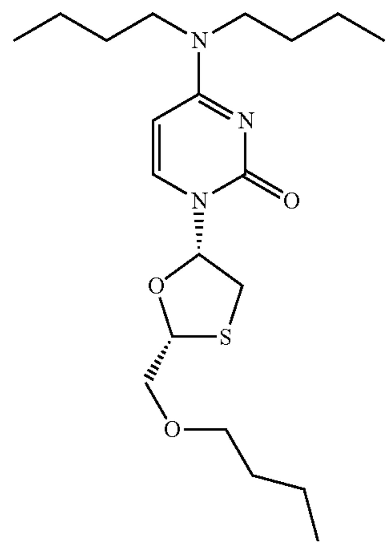
3-Butyl-3TC
