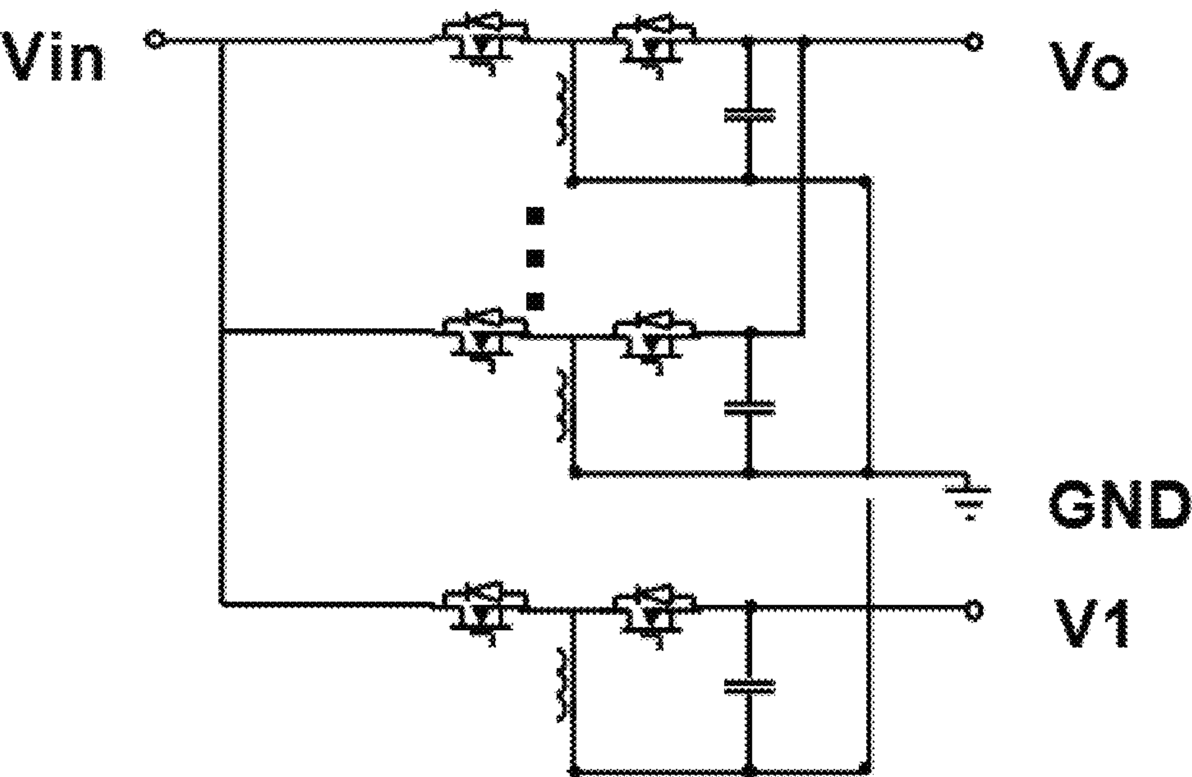
Buck/Boost Circuit
