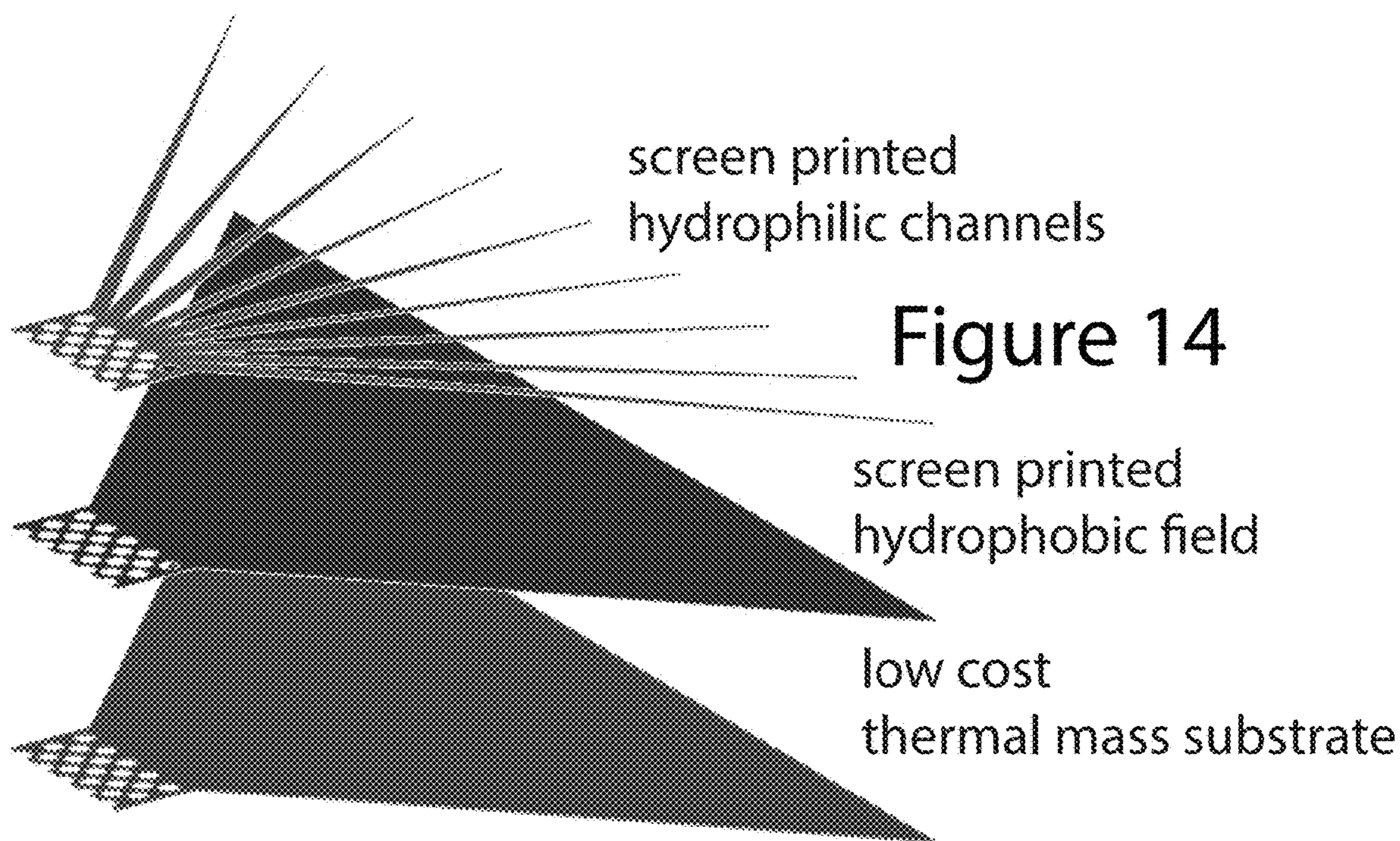
EBC sample collector assembly
